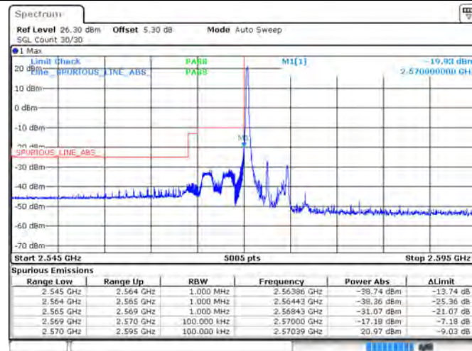
Band38_5MHz_QPSK_37775_1RB#0
