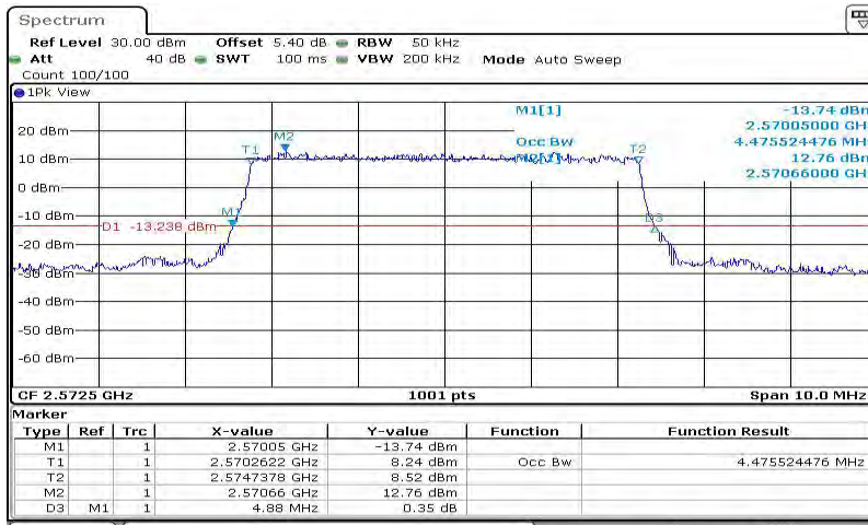
Band38-5MHz-QPSK-37775-25RB#0-4.476
