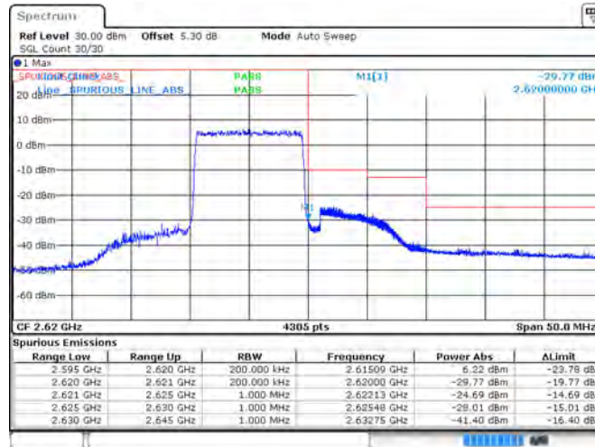
Band38_10MHz_16QAM_38200_50RB#0
