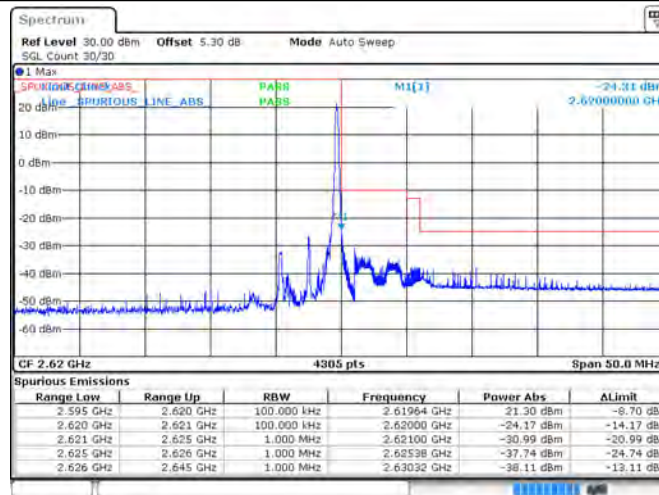
Band38_5MHz_16QAM_38225_25RB#0
