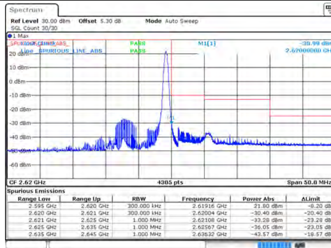
Band38_15MHz_16QAM_38175_75RB#0
