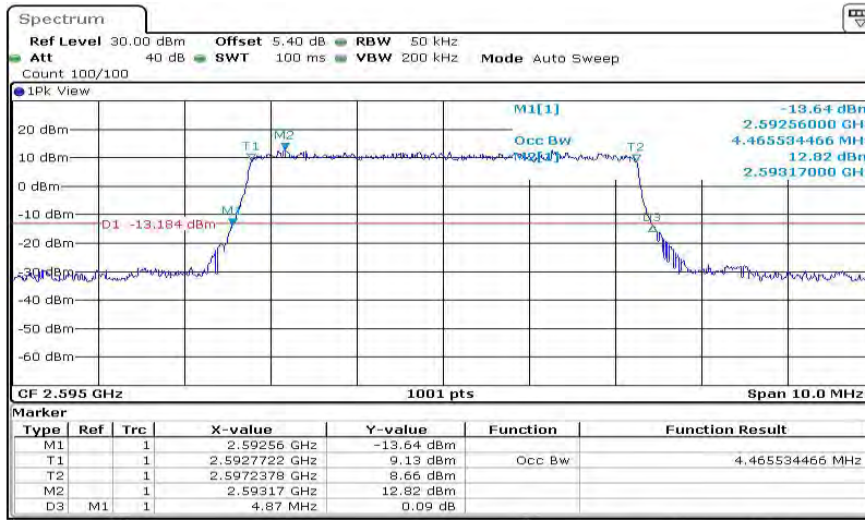
Band38-5MHz-QPSK-38000-25RB#0-4.466
