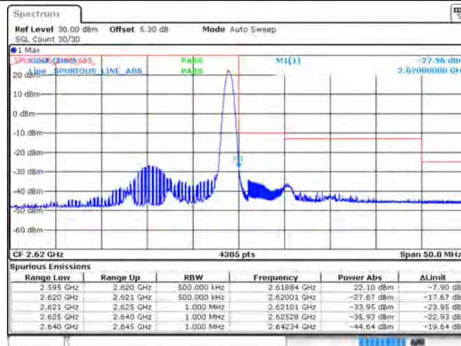
Band38_20MHz_QPSK_38150_100RB#0
