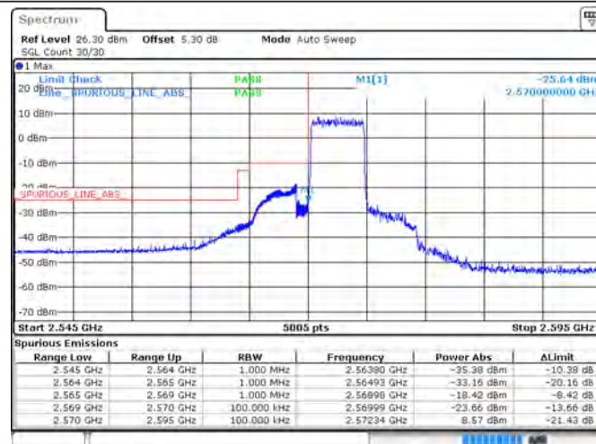
Band38_5MHz_QPSK_37775_25RB#0
