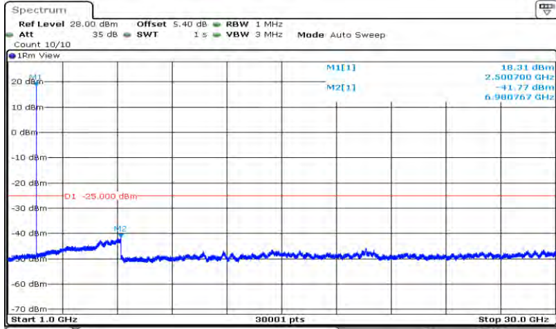
Band7-20MHz-64QAM-20850-1RB#0-Range2:1000~30000MHz
