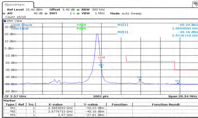
Band7-15MHz-QPSK-21375-75RB#0
