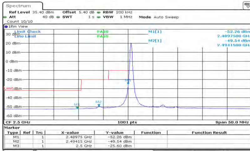
Band7-10MHz-16QAM-20800-50RB#0
