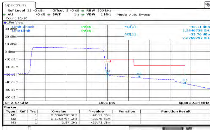
Band7-15MHz-QPSK-21375-75RB#0
