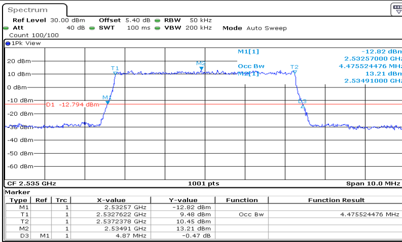
Band7-5MHz-QPSK-21100-25RB#0-4.476
