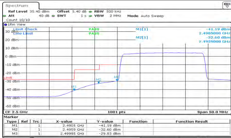
Band7-20MHz-64QAM-20850-100RB#0
