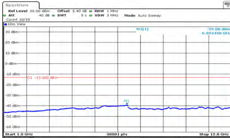
Band5-10MHz-16QAM-20525-1RB#0-Range2:1000~12000MHz
