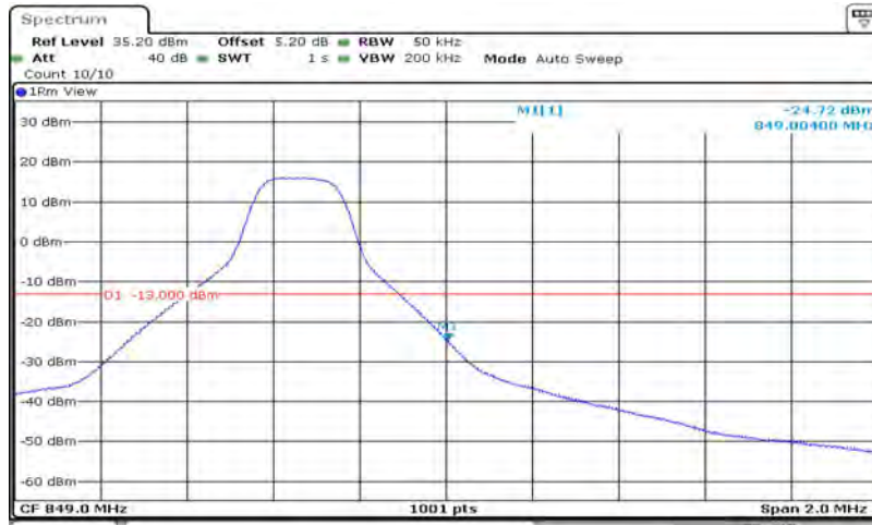
Band5-5MHz-16QAM-20625-25RB#0
