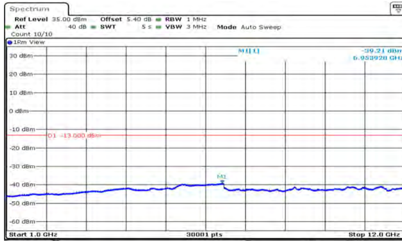
Band5-10MHz-16QAM-20450-1RB#0-Range2:1000~12000MHz
