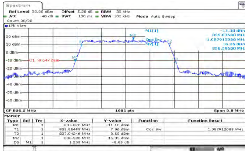
Band5-1.4MHz-QPSK-20525-6RB#0-1.088
