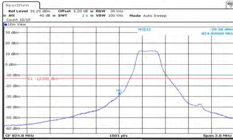
Band5-1.4MHz-64QAM-20407-6RB#0
