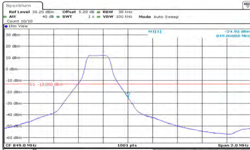
Band5-3MHz-64QAM-20635-15RB#0
