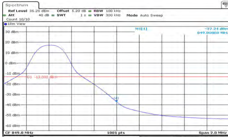
Band5-10MHz-64QAM-20600-50RB#0
