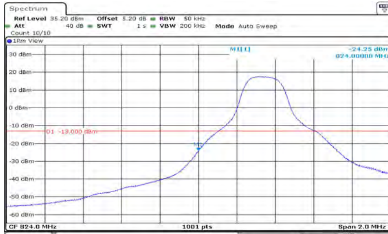
Band5-5MHz-QPSK-20425-25RB#0
