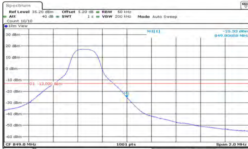
Band5-5MHz-QPSK-20625-25RB#0
