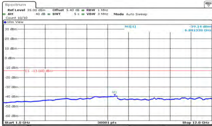
Band5-10MHz-QPSK-20600-1RB#0-Range2:1000~12000MHz
