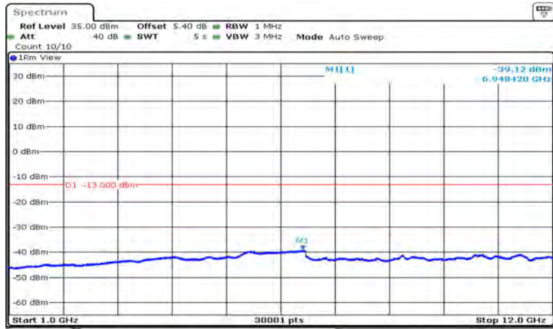
Band5-10MHz-64QAM-20600-1RB#0-Range2:1000~12000MHz
