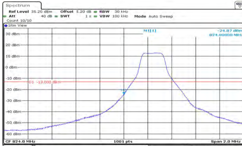
Band5-3MHz-64QAM-20415-15RB#0
