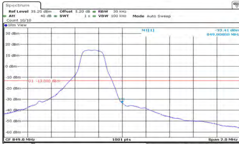
Band5-1.4MHz-QPSK-20643-6RB#0
