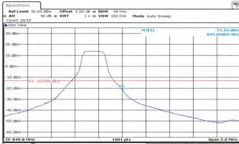
Band5-3MHz-16QAM-20635-15RB#0
