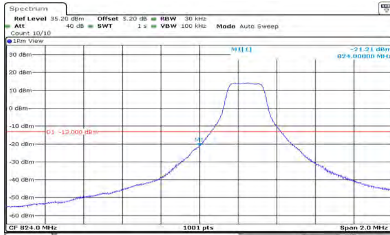
Band5-3MHz-16QAM-20415-15RB#0
