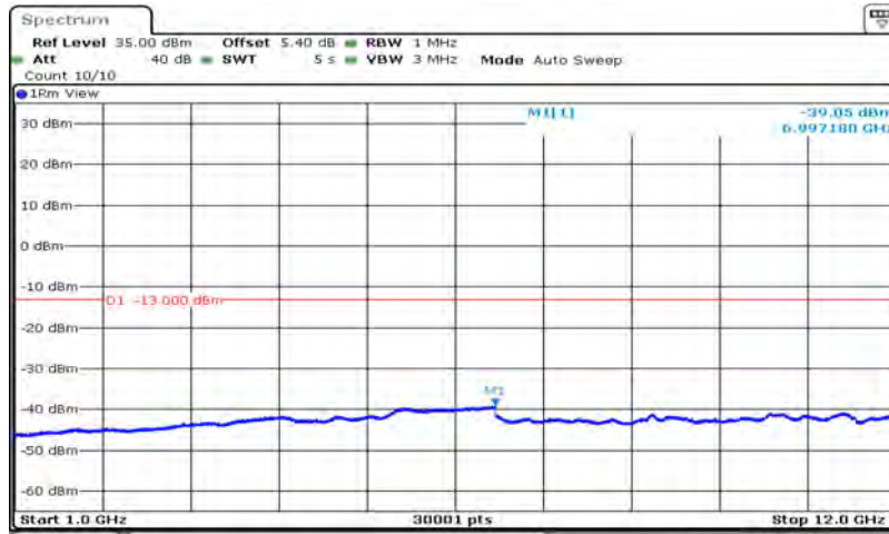
Band5-10MHz-64QAM-20525-1RB#0-Range2:1000~12000MHz
