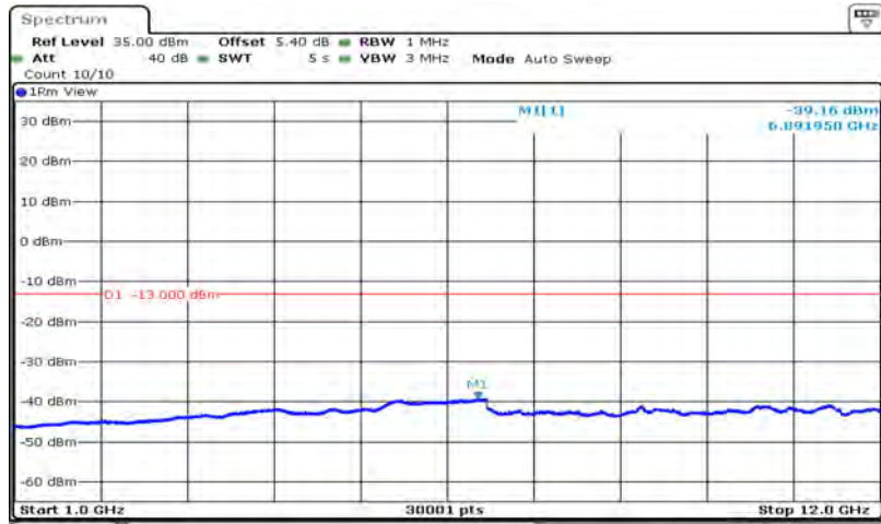
Band5-10MHz-64QAM-20450-1RB#0-Range2:1000~12000MHz
