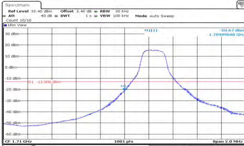
Band4-3MHz-QPSK-19965-15RB#0
