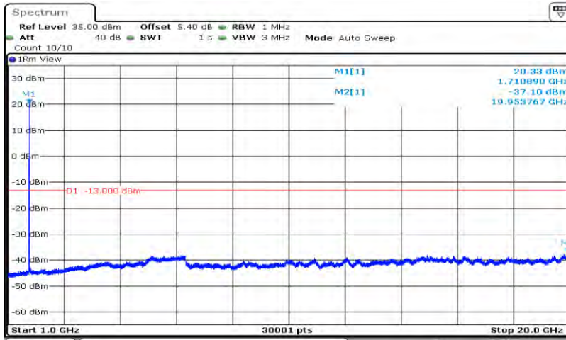
Band4-20MHz-64QAM-20050-1RB#0-Range2:1000~20000MHz
