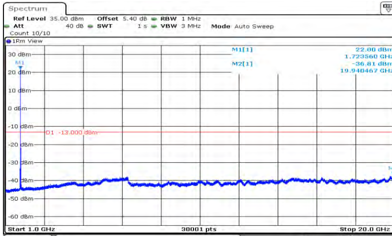
Band4-20MHz-64QAM-20175-1RB#0-Range2:1000~20000MHz
