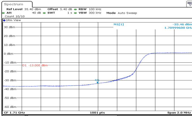
Band4-10MHz-16QAM-20000-50RB#0
