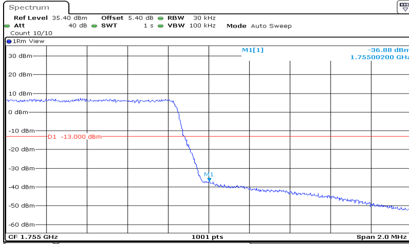
Band4-1.4MHz-QPSK-20393-6RB#0
