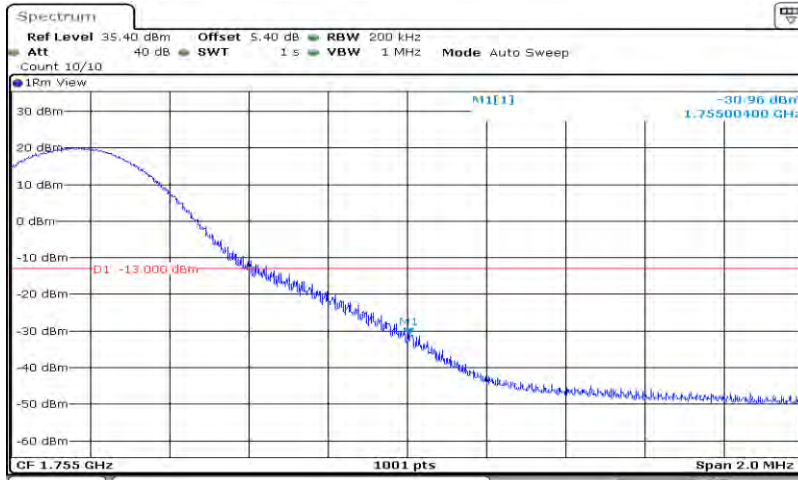
Band4-15MHz-64QAM-20325-75RB#0
