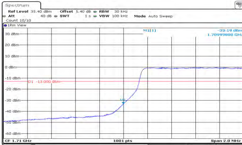
Band4-3MHz-64QAM-19965-15RB#0
