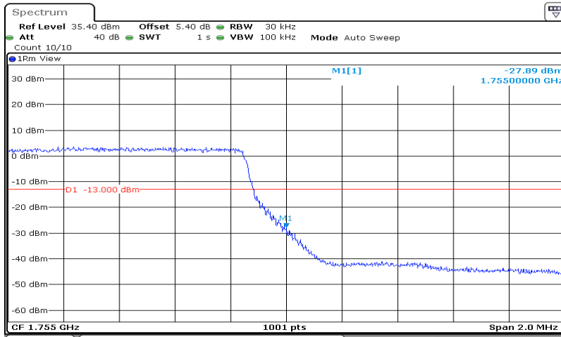
Band4-3MHz-QPSK-20385-15RB#0
