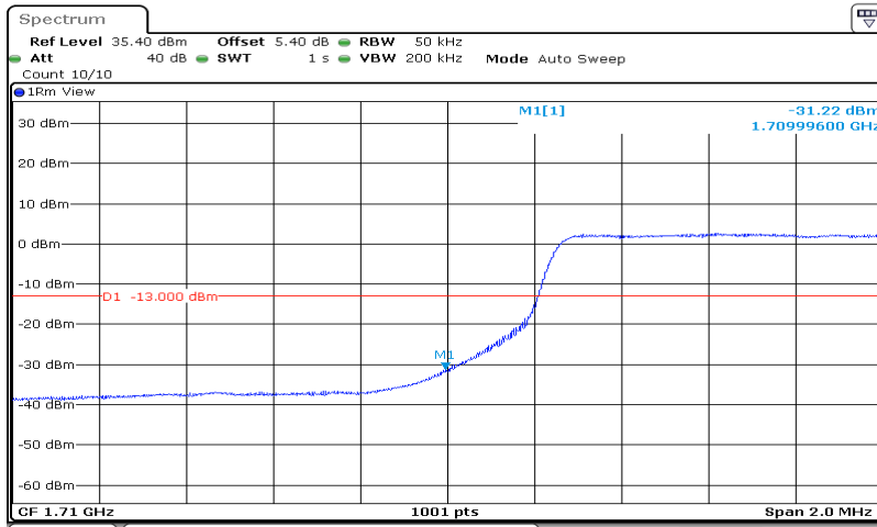
Band4-5MHz-QPSK-19975-25RB#0
