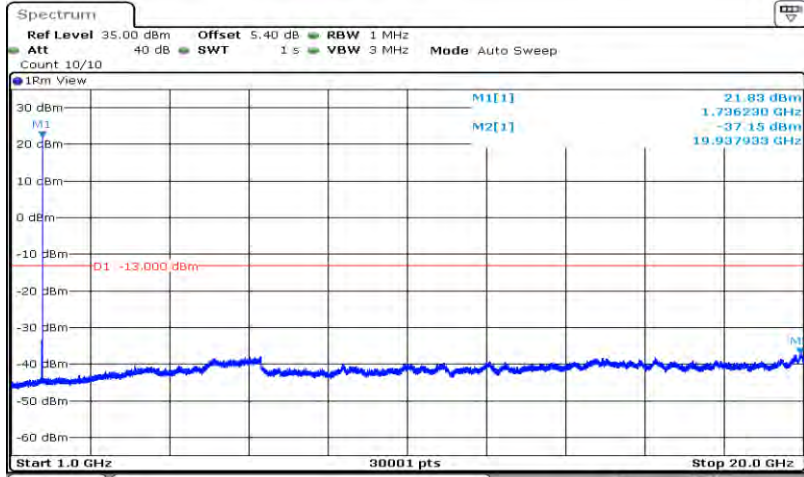
Band4-20MHz-64QAM-20300-1RB#0-Range2:1000~20000MHz
