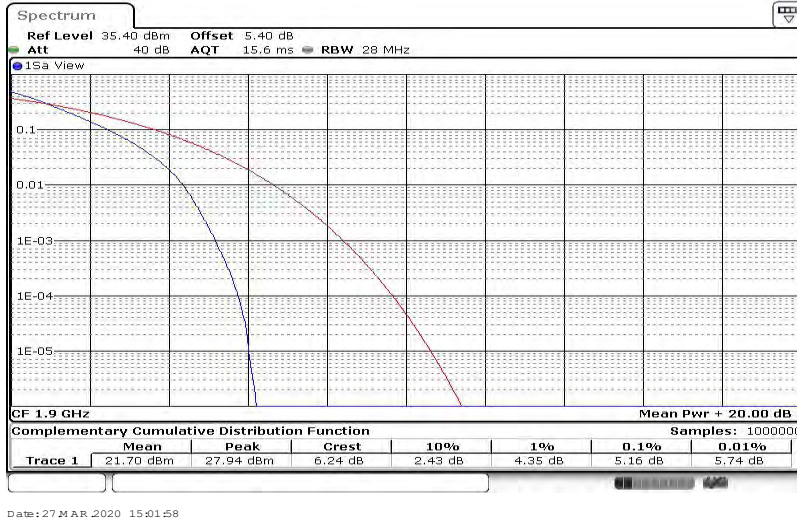
Band2-20MHz-64QAM-18700-100RB#0
