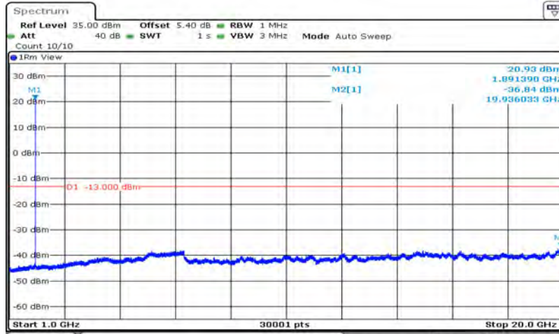
Band2-20MHz-64QAM-19100-1RB#0-Range2:1000~20000MHz
