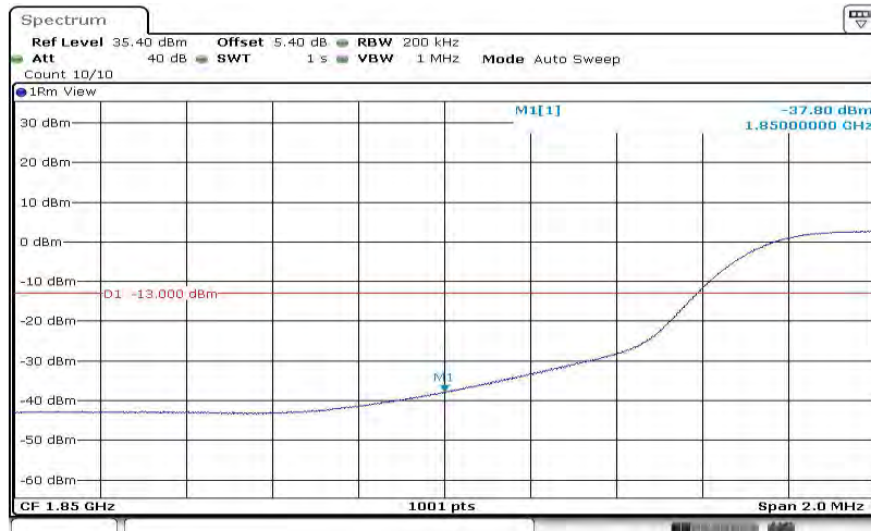
Band2-15MHz-16QAM-18675-75RB#0
