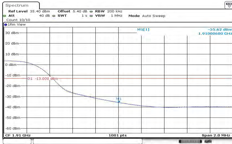
Band2-15MHz-QPSK-19125-75RB#0
