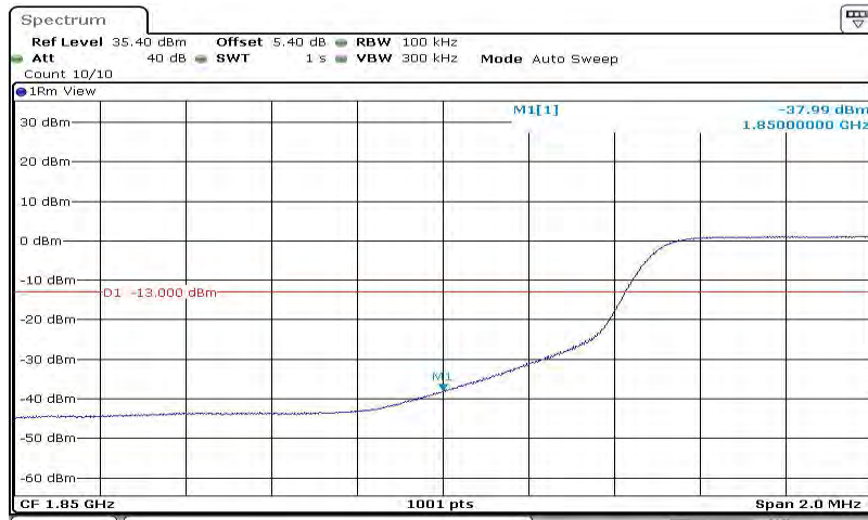
Band2-10MHz-16QAM-18650-50RB#0
