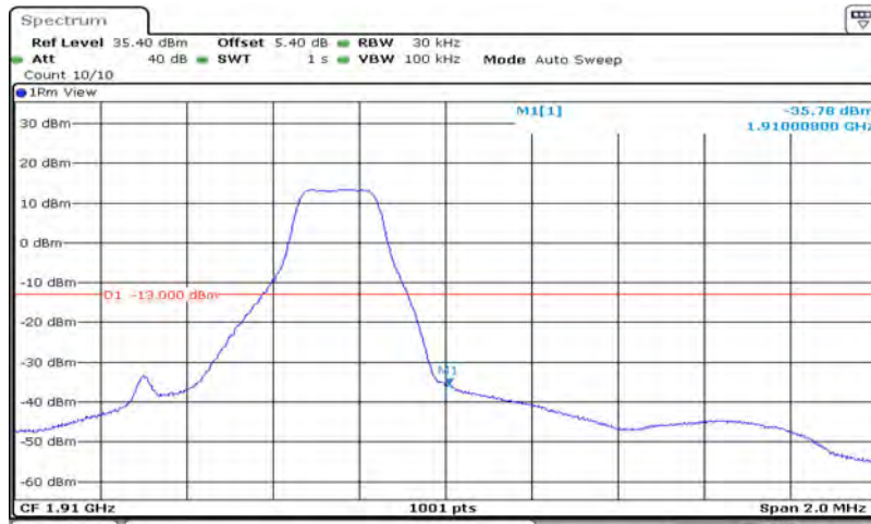
Band2-1.4MHz-64QAM-19193-6RB#0
