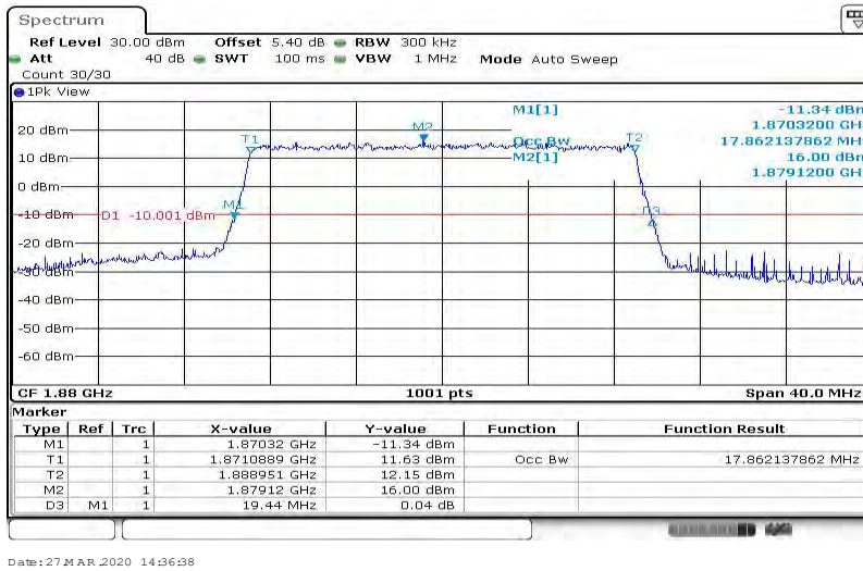
Band2-20MHz-QPSK-19100-100RB#0-17.862
