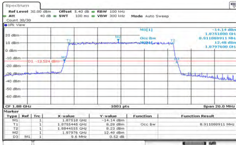
Band2-10MHz-64QAM-18900-50RB#0-8.911
