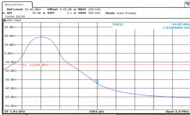
Band2-10MHz-64QAM-19150-50RB#0
