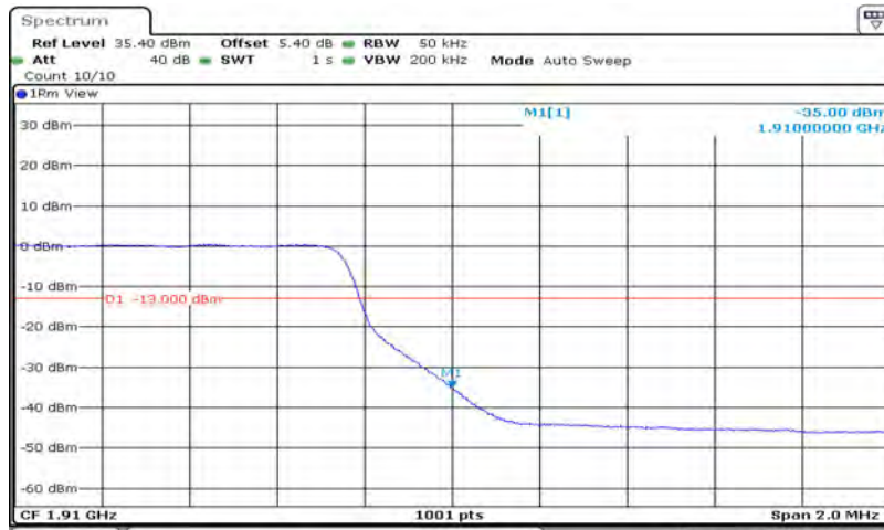
Band2-5MHz-64QAM-19175-25RB#0
