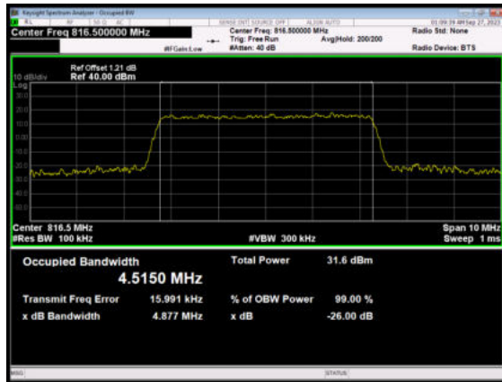
LTE Band 26 QPSK 5MHz CH Middle
