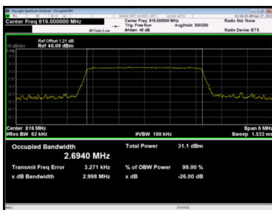
LTE Band 26 64QAM 3MHz CH High
