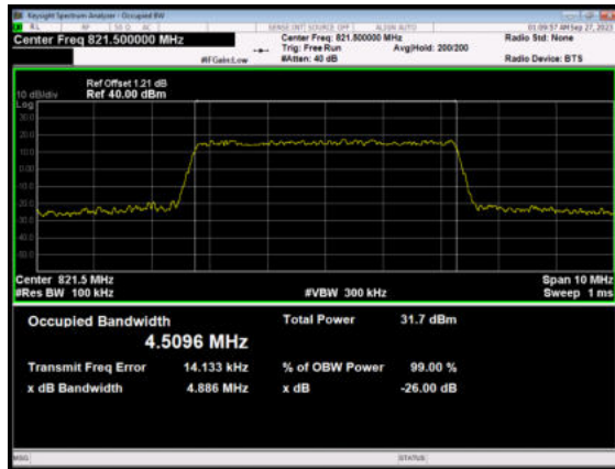
LTE Band 26 QPSK 5MHz CH High
