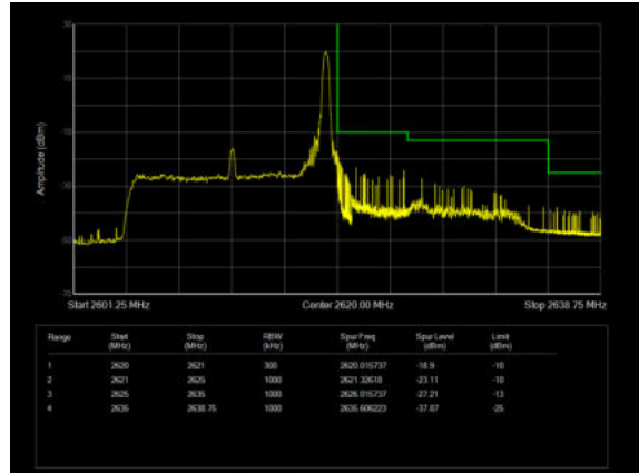
LTE Band 38 16QAM 15MHz CH-High, 100%RB
