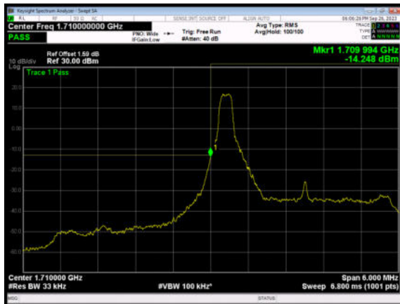
LTE Band 4 64QAM 3MHz CH-Low, 1 RB
