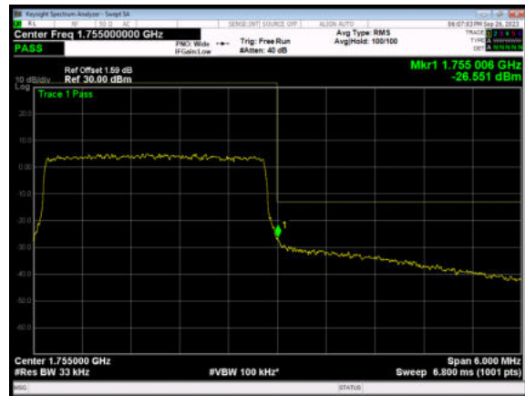
LTE Band 4 64QAM 5MHz CH-High, 1 RB
