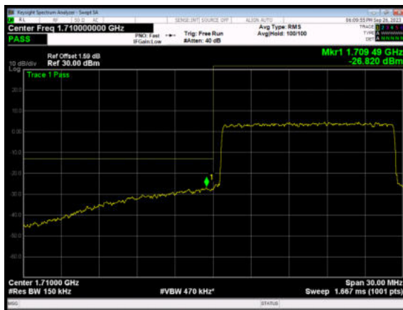
LTE Band 4 64QAM 20MHz CH-Low, 1 RB
