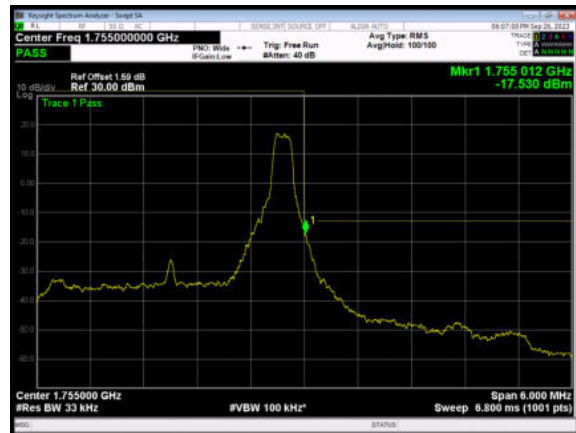
LTE Band 4 64QAM 3MHz CH-High, 1 RB
