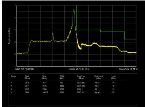
LTE Band 7 64QAM 10MHz CH-High, 100%RB
