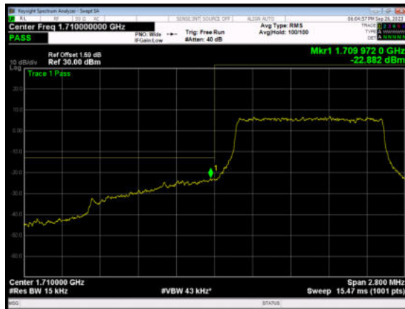
LTE Band 4 QPSK 3MHz CH-Low, 1 RB
