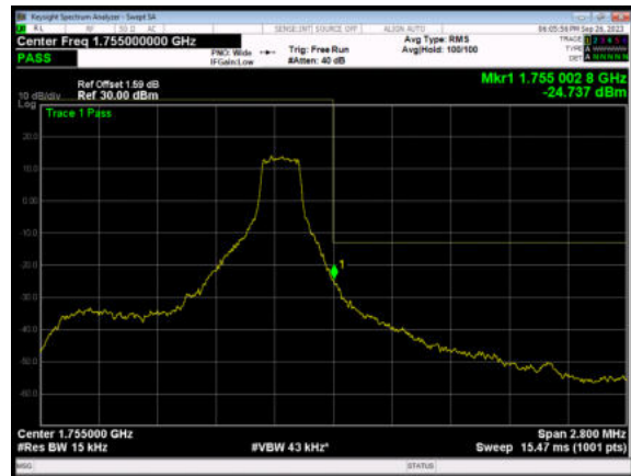
LTE Band 4 64QAM 1.4MHz CH-High, 100%RB
