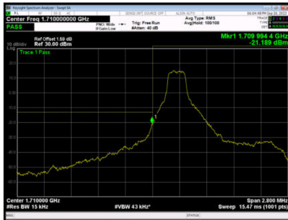
LTE Band 4 QPSK 1.4MHz CH-Low, 100%RB
