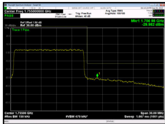
LTE Band 4 64QAM 20MHz CH-High, 1 RB
