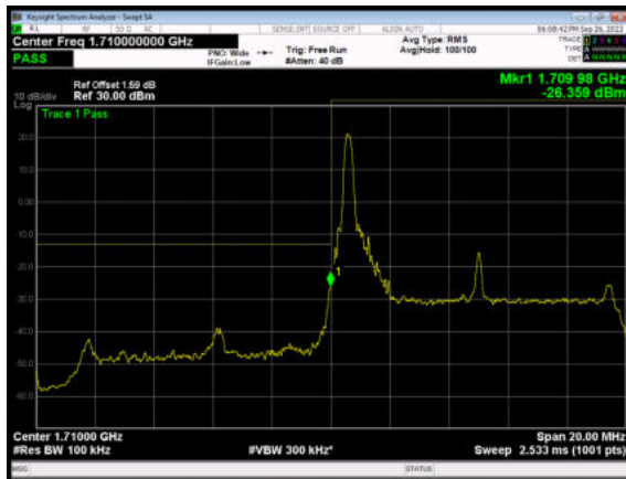
LTE Band 4 64QAM 10MHz CH-Low, 100%RB
