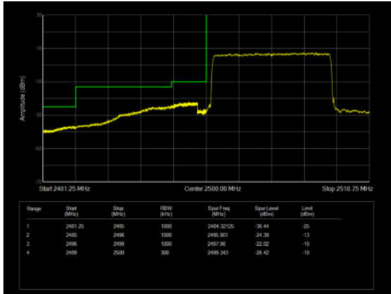
LTE Band 7 64QAM 20MHz CH-Low, 1 RB
