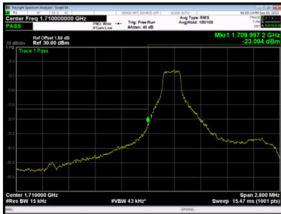
LTE Band 4 64QAM 1.4MHz CH-Low, 100%RB
