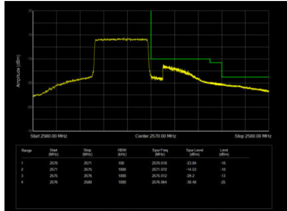
LTE Band 7 16QAM 10MHz CH-High, 1 RB
