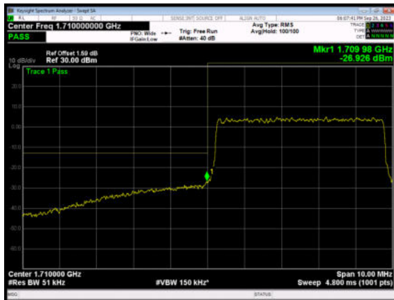
LTE Band 4 64QAM 5MHz CH-Low, 100%RB
