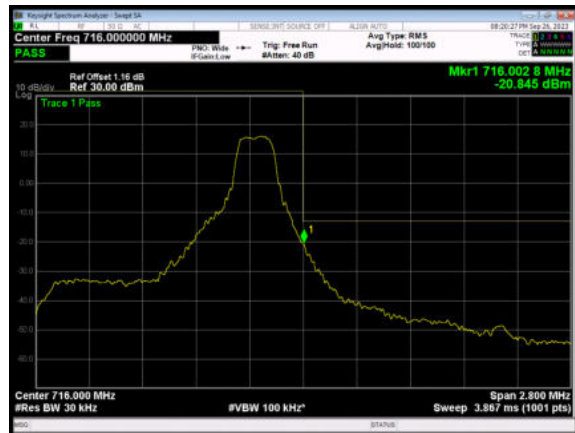
LTE Band 12 64QAM 1.4MHz CH-High, 100%RB
