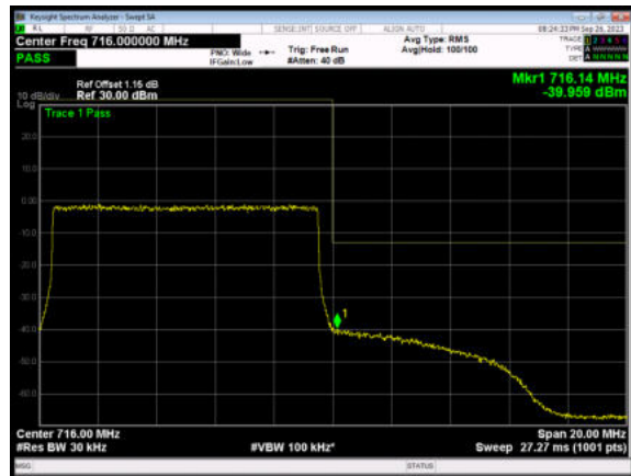
LTE Band 12 64QAM 1.4MHz CH-High, 1 RB
