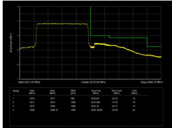
LTE Band 7 64QAM 20MHz CH-High, 1 RB
