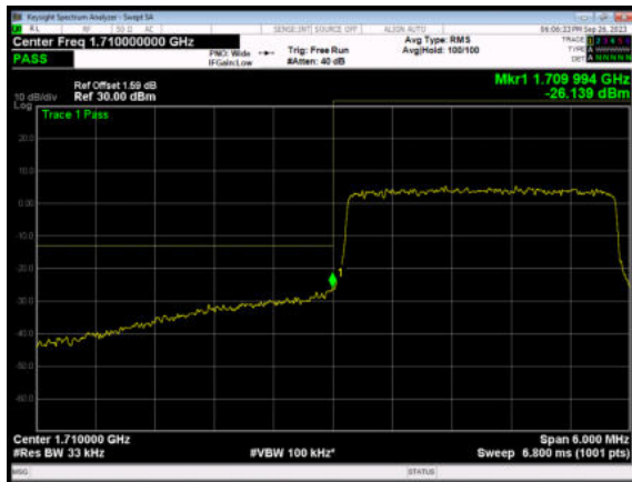
LTE Band 4 64QAM 5MHz CH-Low, 1 RB
