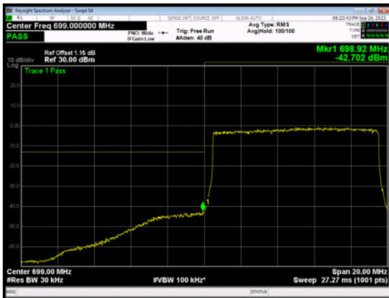
LTE Band 12 64QAM 1.4MHz CH-Low, 1 RB
