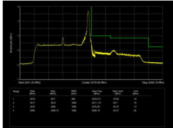
LTE Band 7 16QAM 15MHz CH-High, 100%RB
