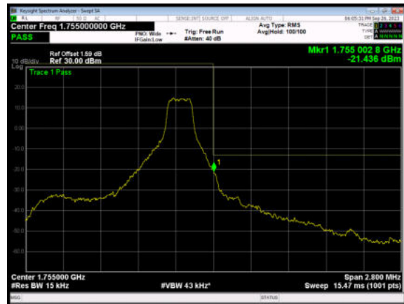
LTE Band 4 QPSK 1.4MHz CH-High, 100%RB
