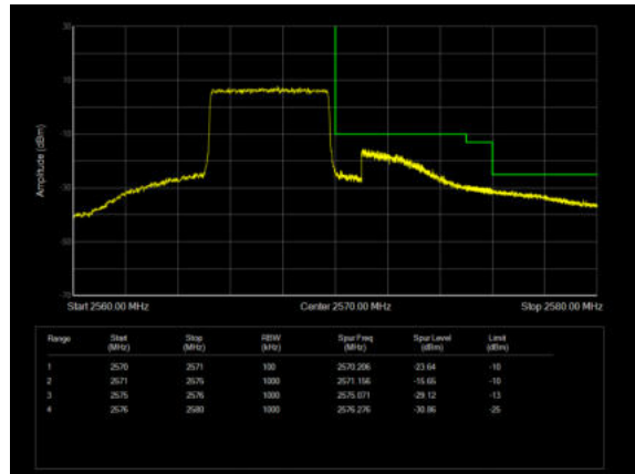
LTE Band 7 64QAM 5MHz CH-High, 100%RB
