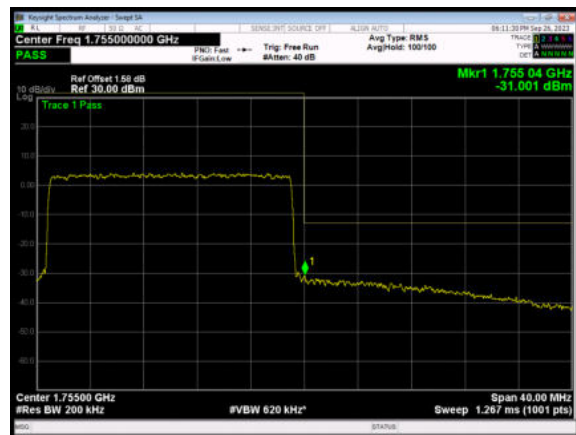
LTE Band 4 64QAM 20MHz CH-High, 100%RB
