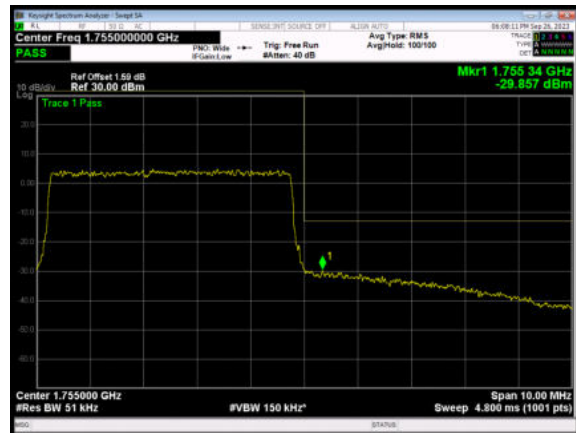
LTE Band 4 64QAM 5MHz CH-High, 100%RB
