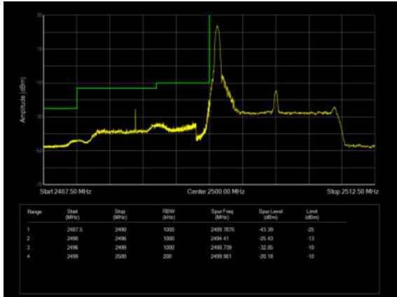
LTE Band 7 64QAM 10MHz CH-Low, 100%RB
