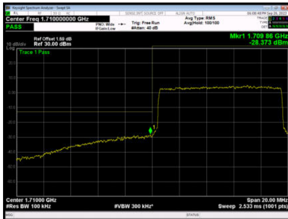
LTE Band 4 64QAM 15MHz CH-Low, 1 RB
