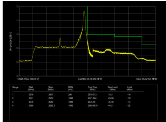
LTE Band 7 16QAM 10MHz CH-High, 100%RB
