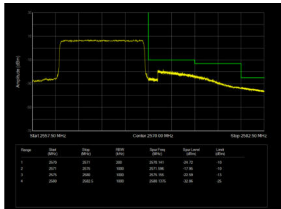
LTE Band 7 64QAM 15MHz CH-High, 1 RB
