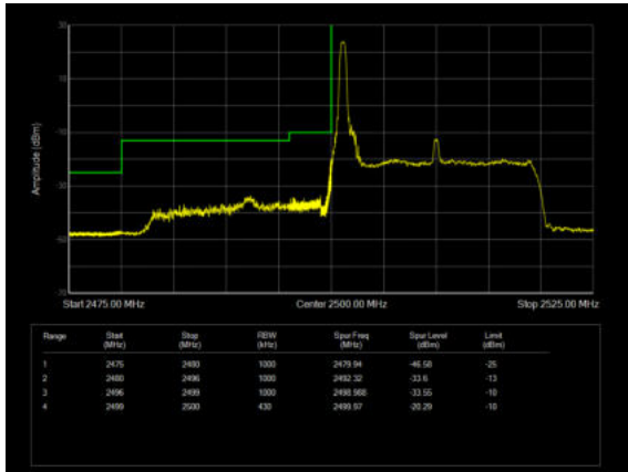
LTE Band 7 64QAM 20MHz CH-Low, 100%RB
