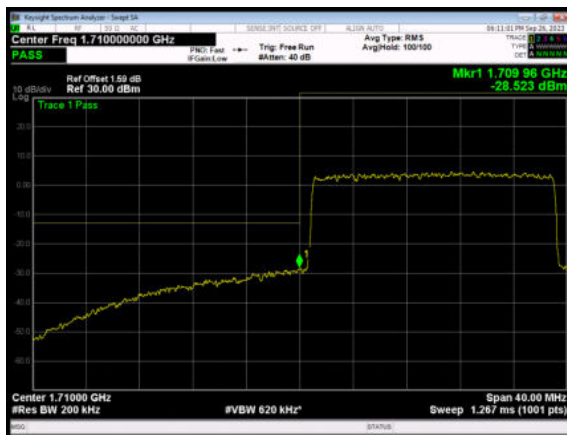
LTE Band 4 64QAM 20MHz CH-Low, 100%RB
