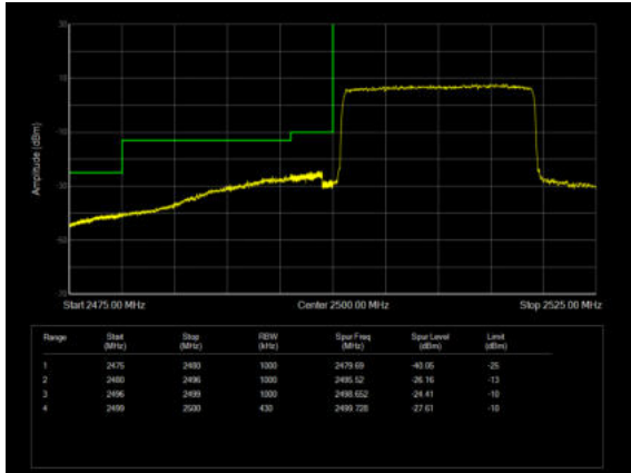
LTE Band 7 64QAM 5MHz CH-Low, 1 RB
