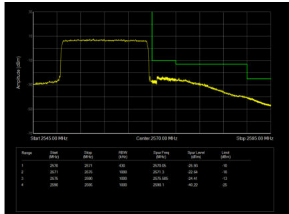
LTE Band 7 64QAM 20MHz CH-High, 100%RB
