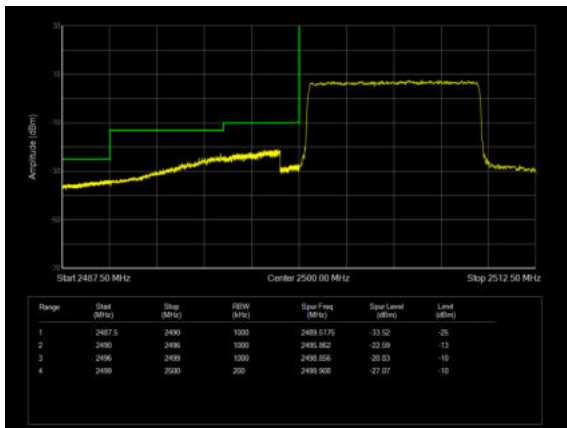
LTE Band 7 64QAM 15MHz CH-Low, 1 RB
