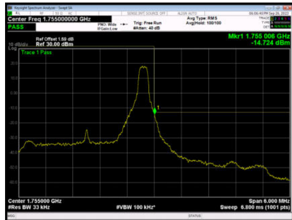
LTE Band 4 QPSK 3MHz CH-High, 1 RB
