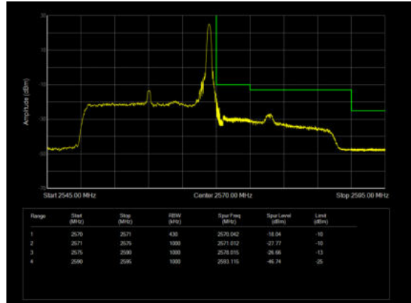
LTE Band 7 QPSK 20MHz CH-High, 100%RB
