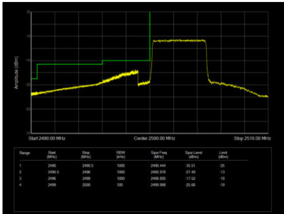
LTE Band 7 64QAM 5MHz CH-Low, 100%RB
