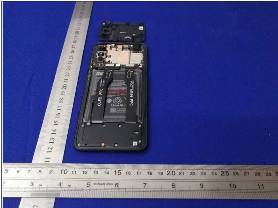
DIV Antenna
