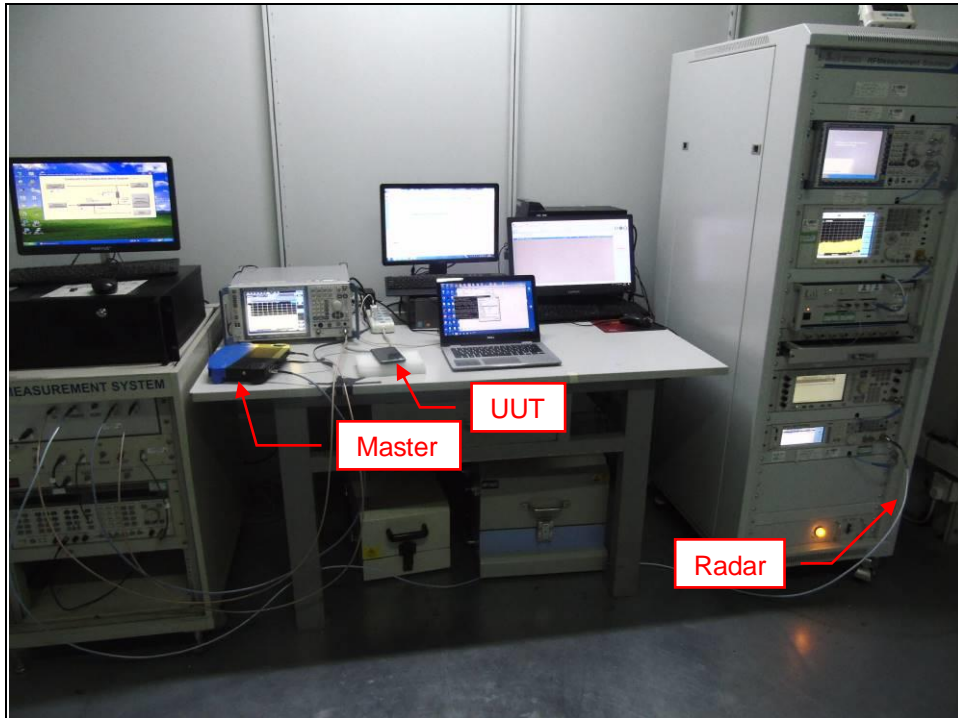
Set UUT as Client mode (Radar injected into Master)
