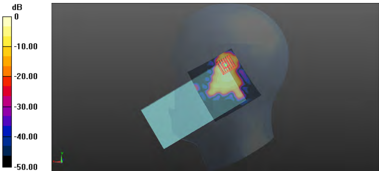
0 dB = 0.500 W/kg
