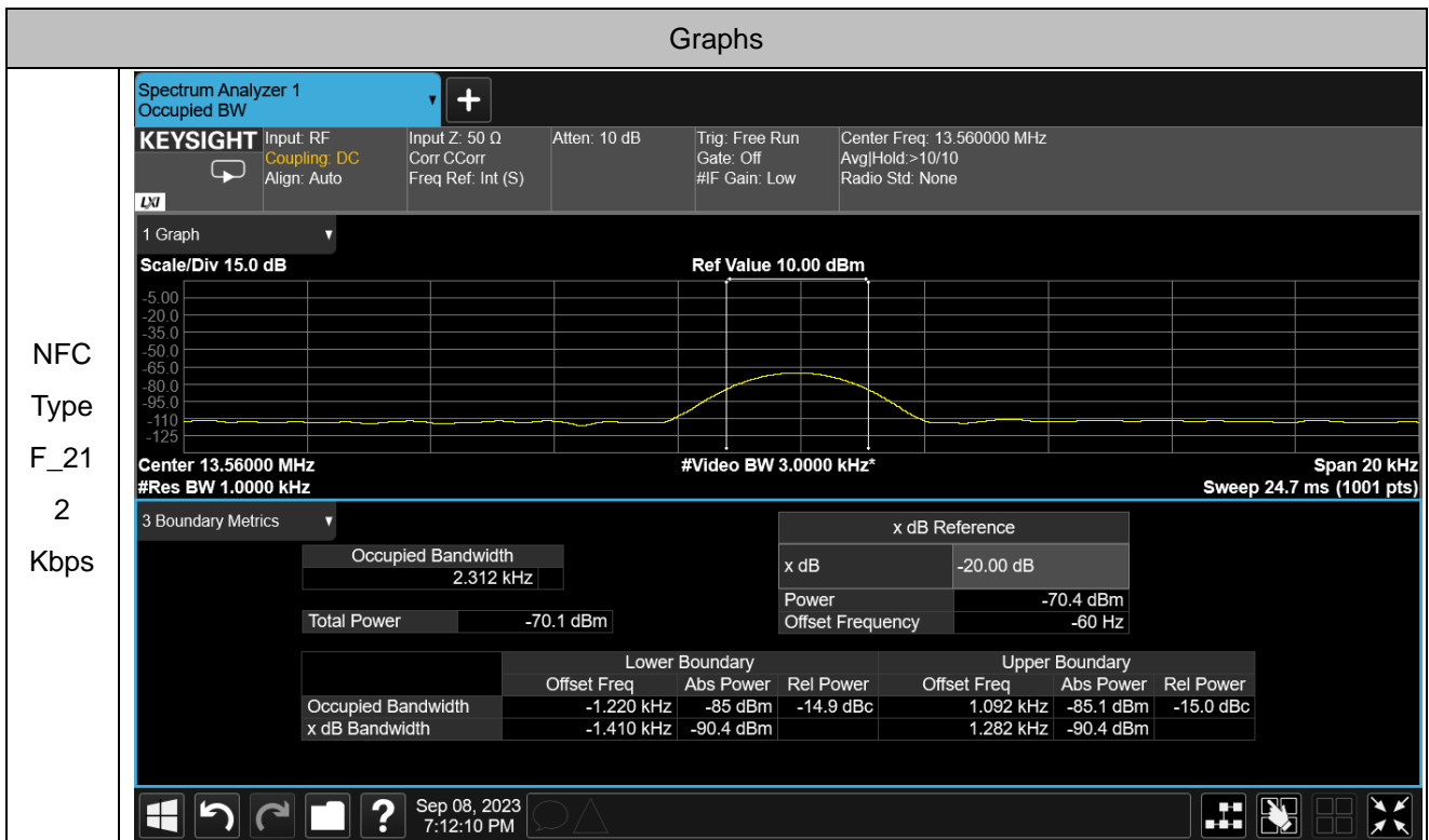
20dB Bandwidth & 99% Bandwidth Plot
