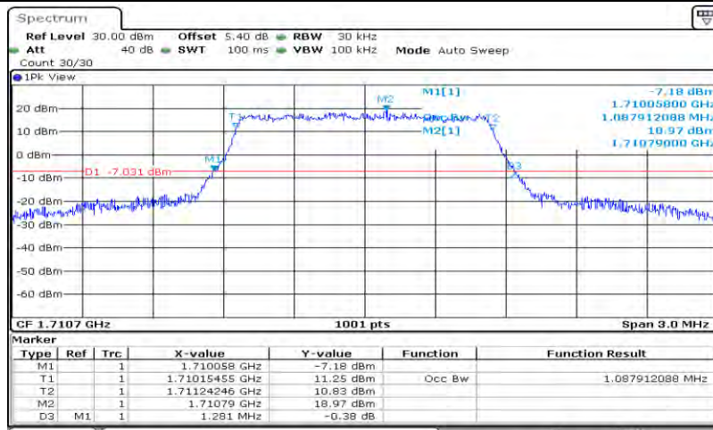
Band4-1.4MHz-QPSK-19957-6RB#0-1.088
