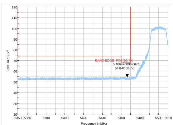
802.11a-Channel 100: Average
