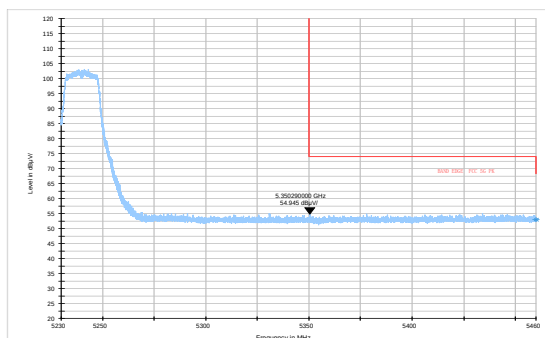
802.11a-Channel 48: Peak
