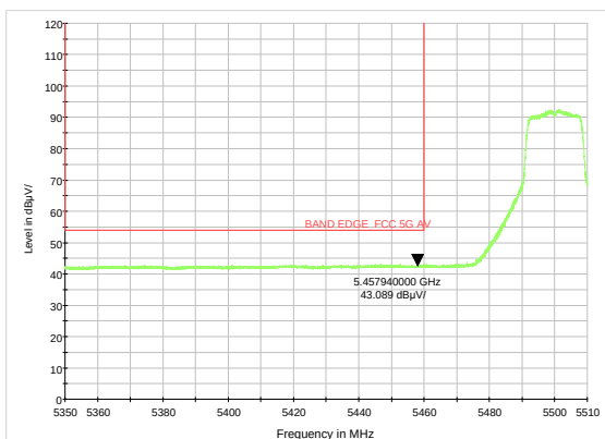
802.11a-Channel 100: Average
