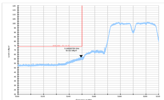
802.11n HT40-Channel 38: Peak
