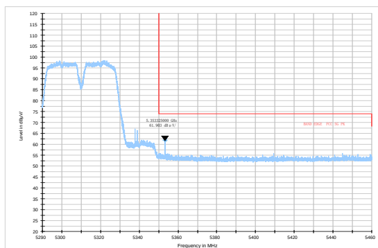
802.11n HT40-Channel 62: Average
