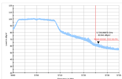
802.11a-Channel 140: Peak
