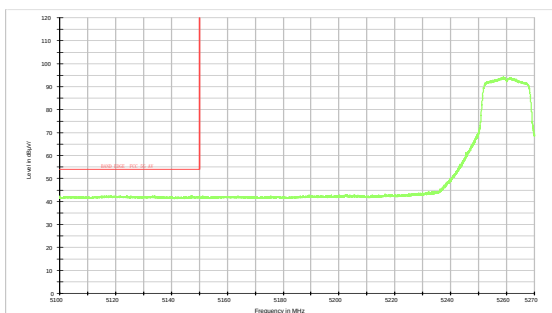
802.11n HT20-Channel 52: Peak
