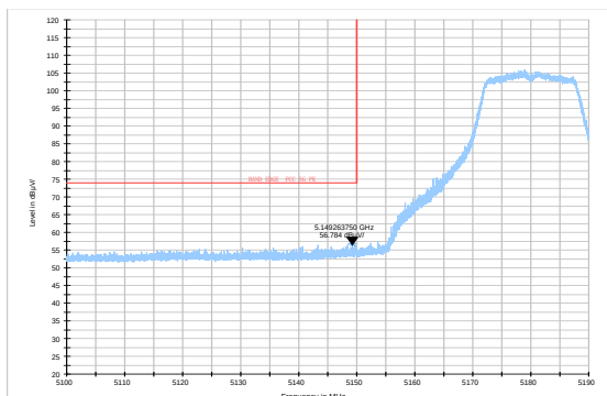
802.11a-Channel 36: Average
