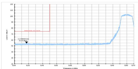
802.11a-Channel 52: Average
