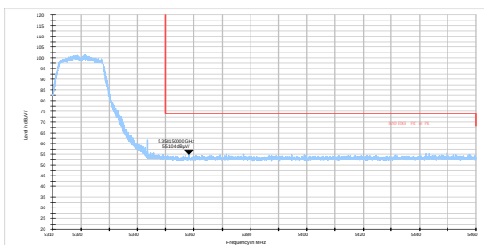
802.11a-Channel 64: Average
