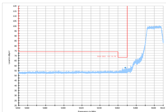
802.11n HT20-Channel 100: Peak
