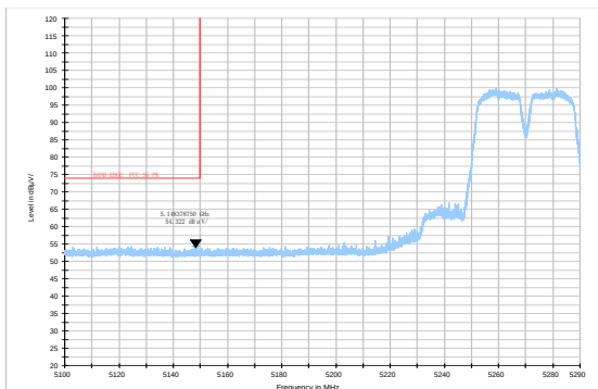
802.11n HT40-Channel 54: Average
