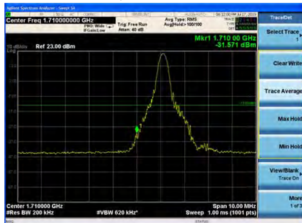
LTE Band 4 16QAM 20MHz CH-Low, 1 RB
