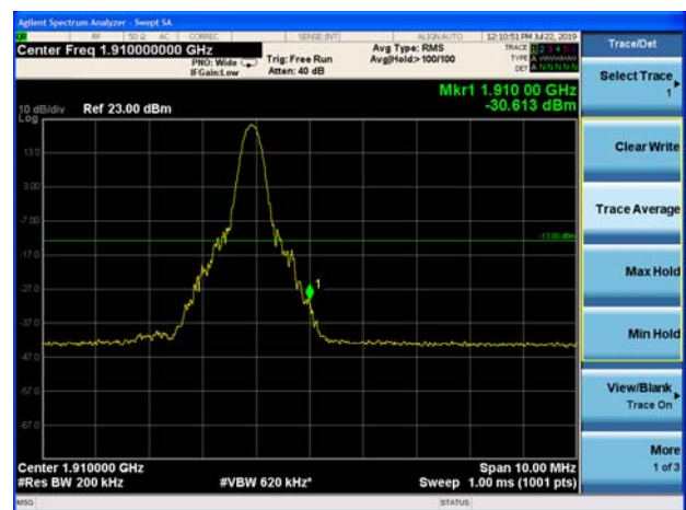
LTE Band 2 20MHz 64QAM 1RB CH-High
