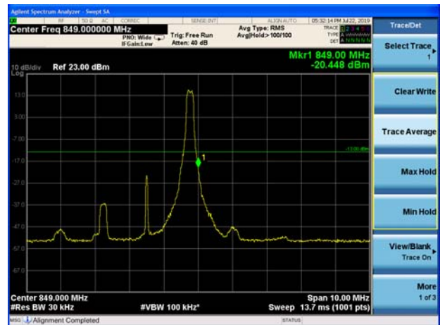
LTE Band 5 64QAM 3MHz CH-High 100%RB
