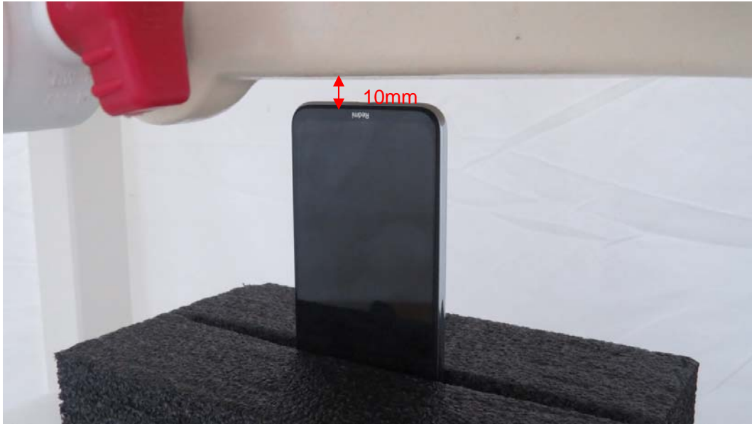
Picture 11: Bottom Side, the distance from handset to the bottom of the Phantom is 10mm
