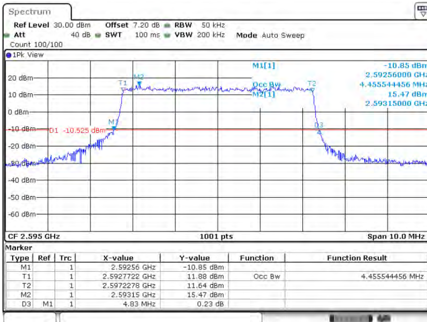
Band38-5MHz-QPSK-38000-25RB#0-4.456
