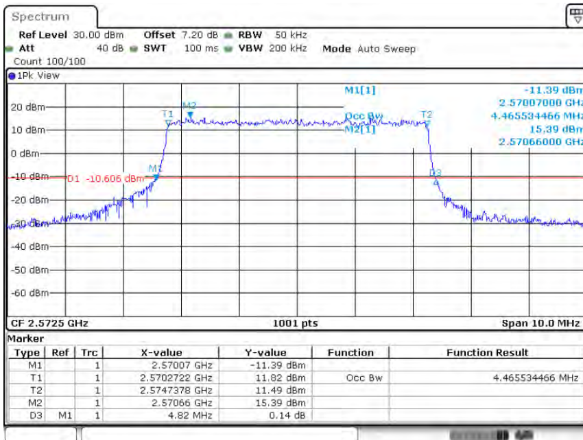
Band38-5MHz-QPSK-37775-25RB#0-4.466
