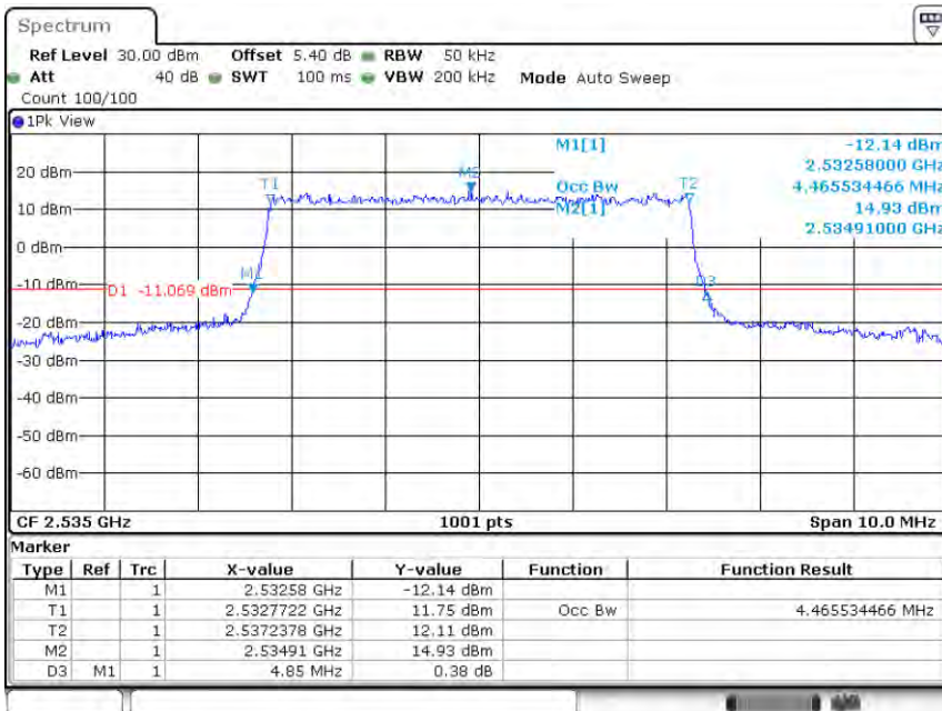
Band7-5MHz-QPSK-21100-25RB#0-4.466
