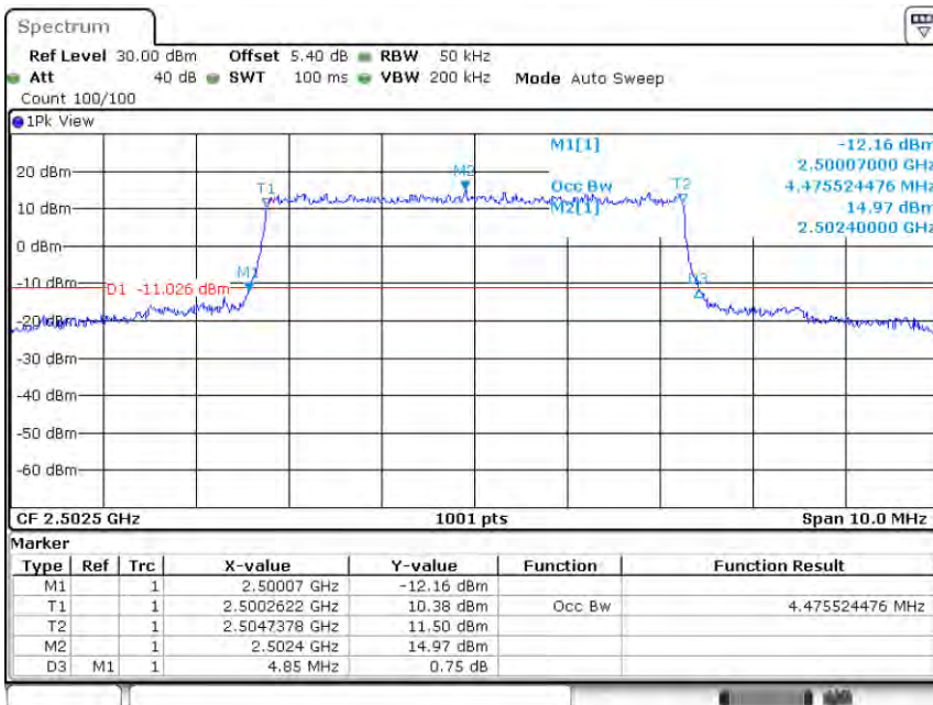
Band7-5MHz-QPSK-20775-25RB#0-4.476
