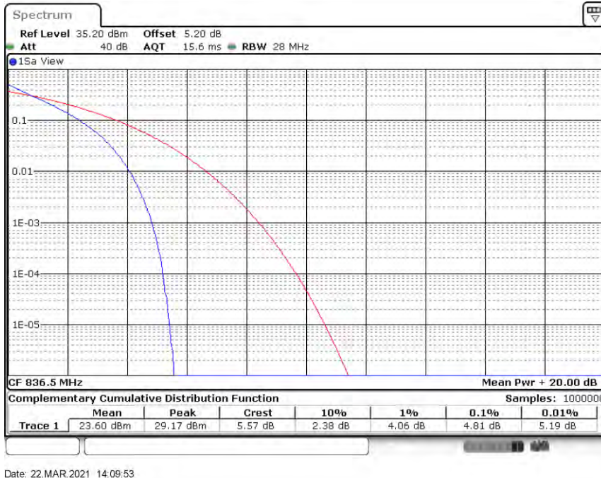
Band5-10MHz-QPSK-20525-50RB#0
