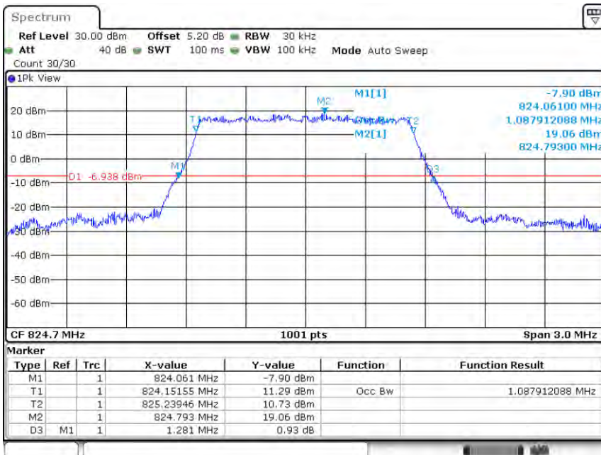
Band5-1.4MHz-QPSK-20407-6RB#0-1.088
