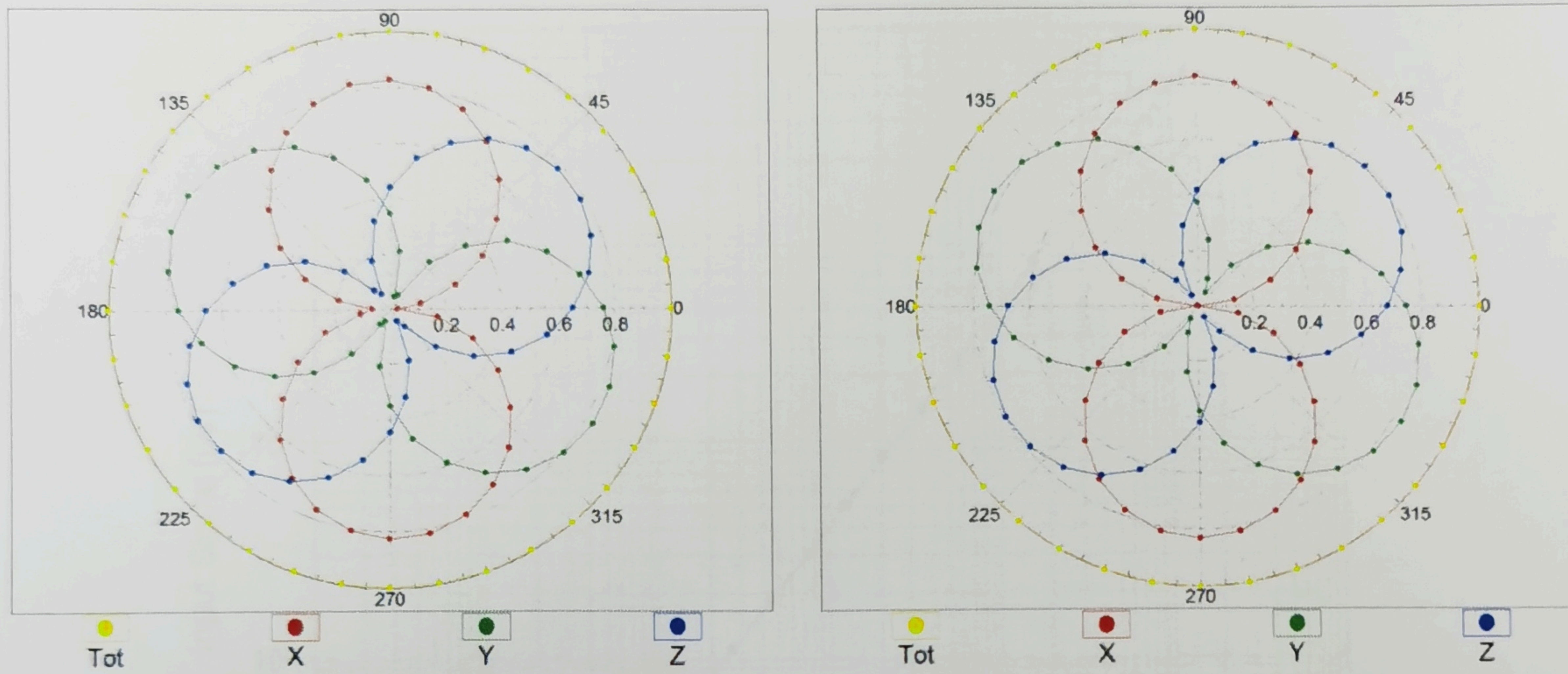
f=600 MHz,TEM
