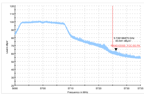
802.11a-Channel 140: Peak
