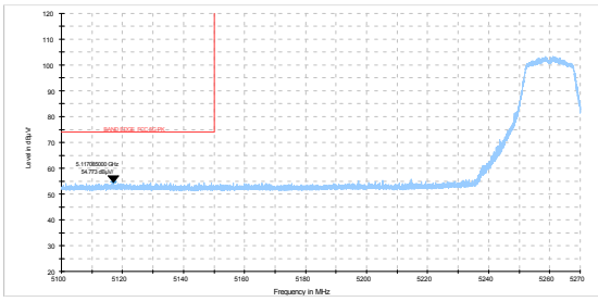
802.11a-Channel 52: Average
