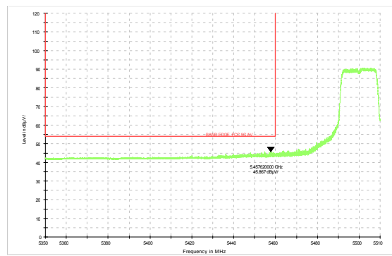
802.11n HT20-Channel 100: Average
