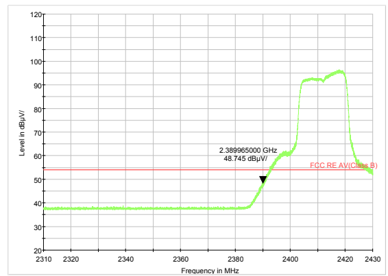
802.11g-Channel 1 Average
