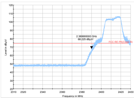
802.11g-Channel 1 Peak
