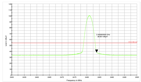
3DH5-Channel 78: Average
