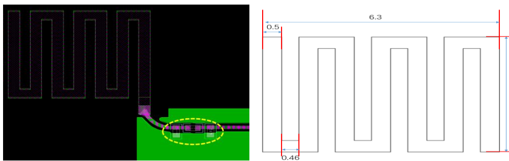
BT Antenna
