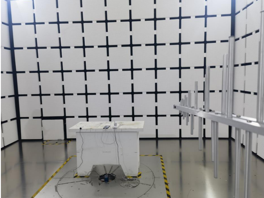
30MHz-1GHz-RF
