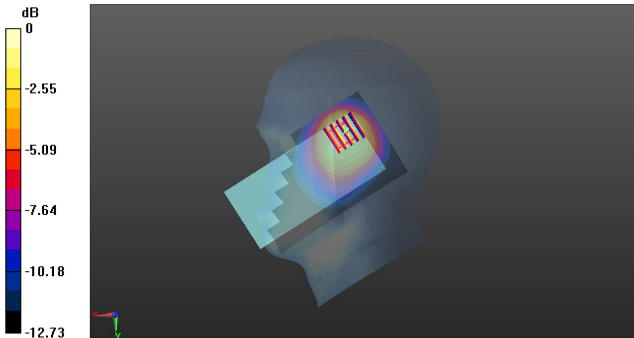
0 dB = 0.778 W/kg
