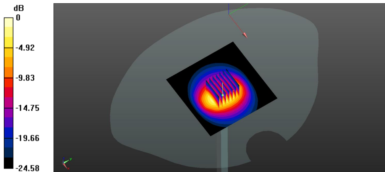
0 dB = 5.87 W/kg
