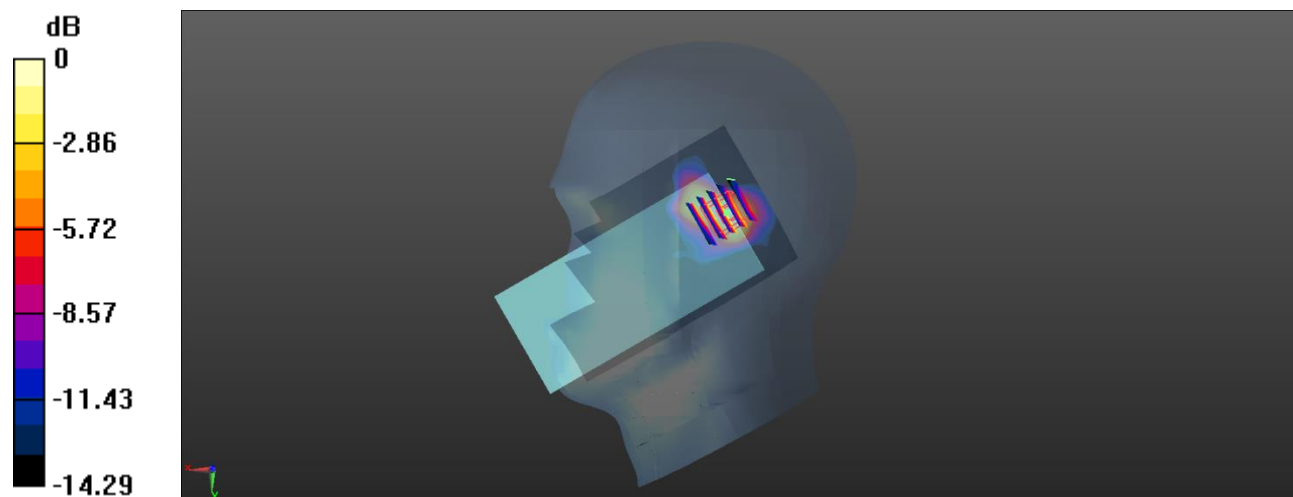
0 dB = 0.792 W/kg
