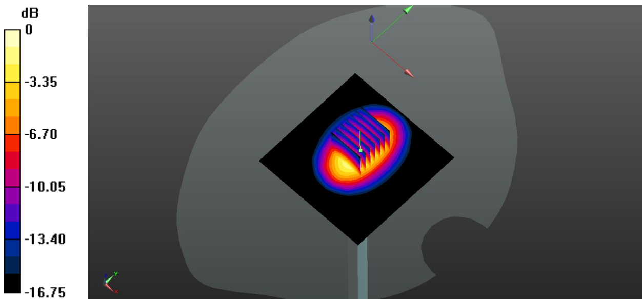
0 dB = 4.52 W/kg
