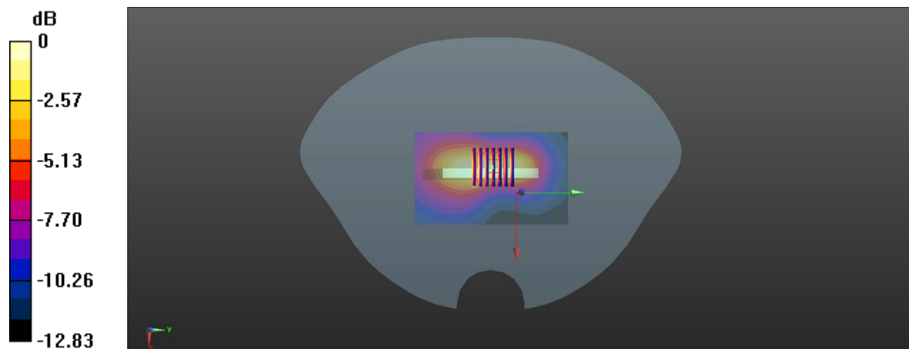
0 dB = 0.667 W/kg
