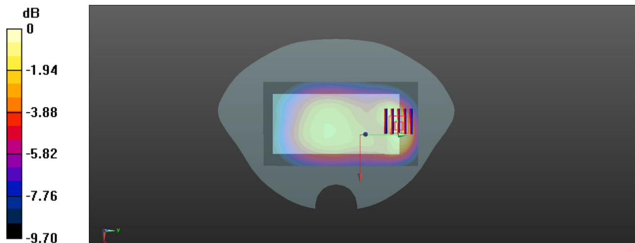
0 dB = 0.181 W/kg
