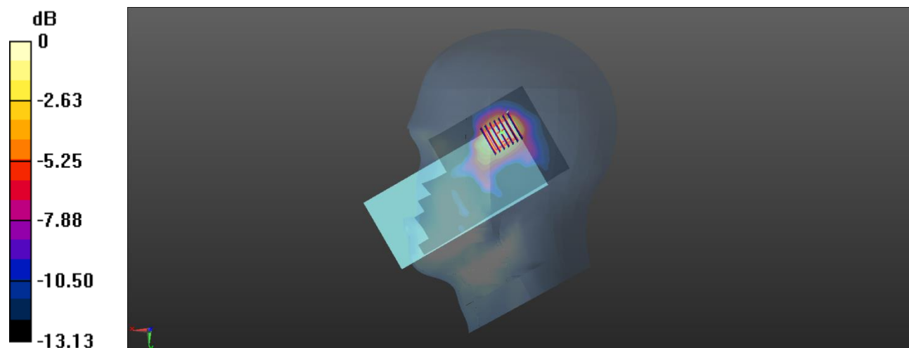
0 dB = 0.579 W/kg
