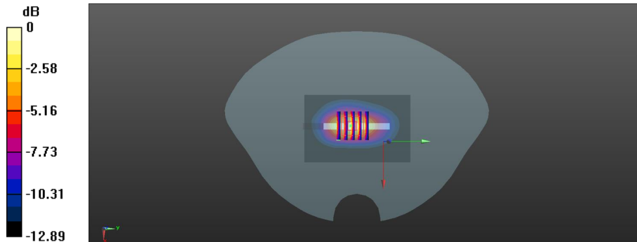
0 dB = 0.624 W/kg
