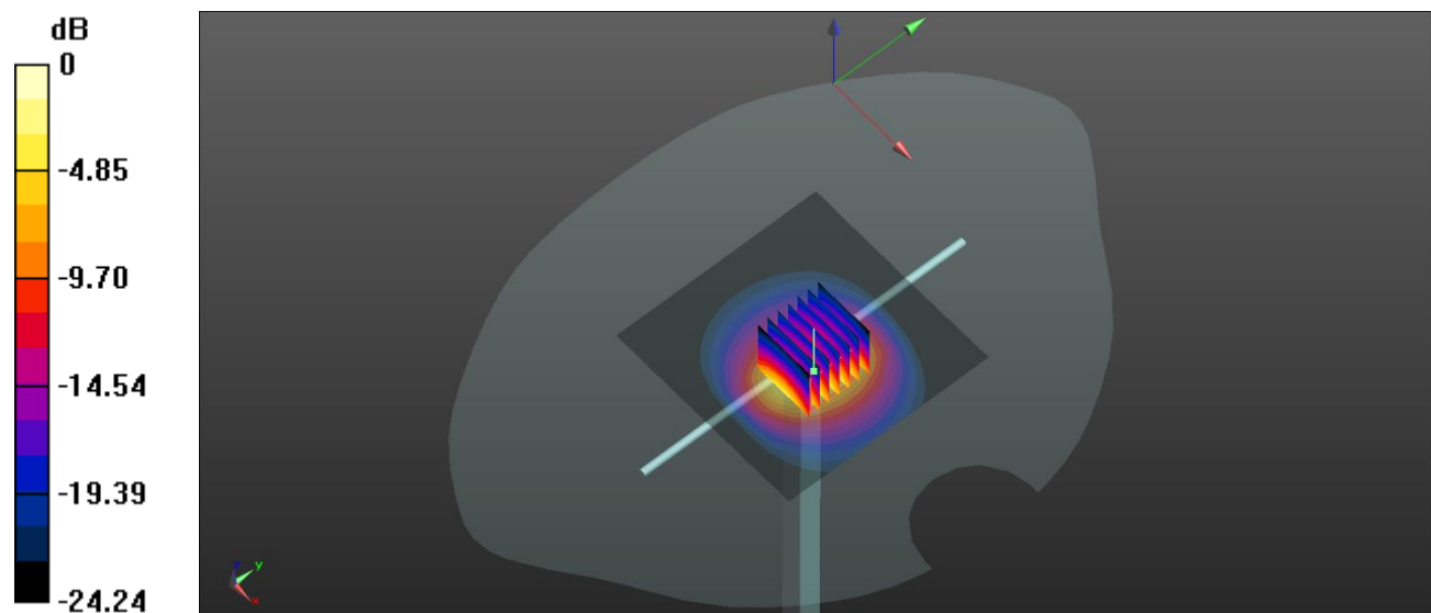
0 dB = 6.57 W/kg
