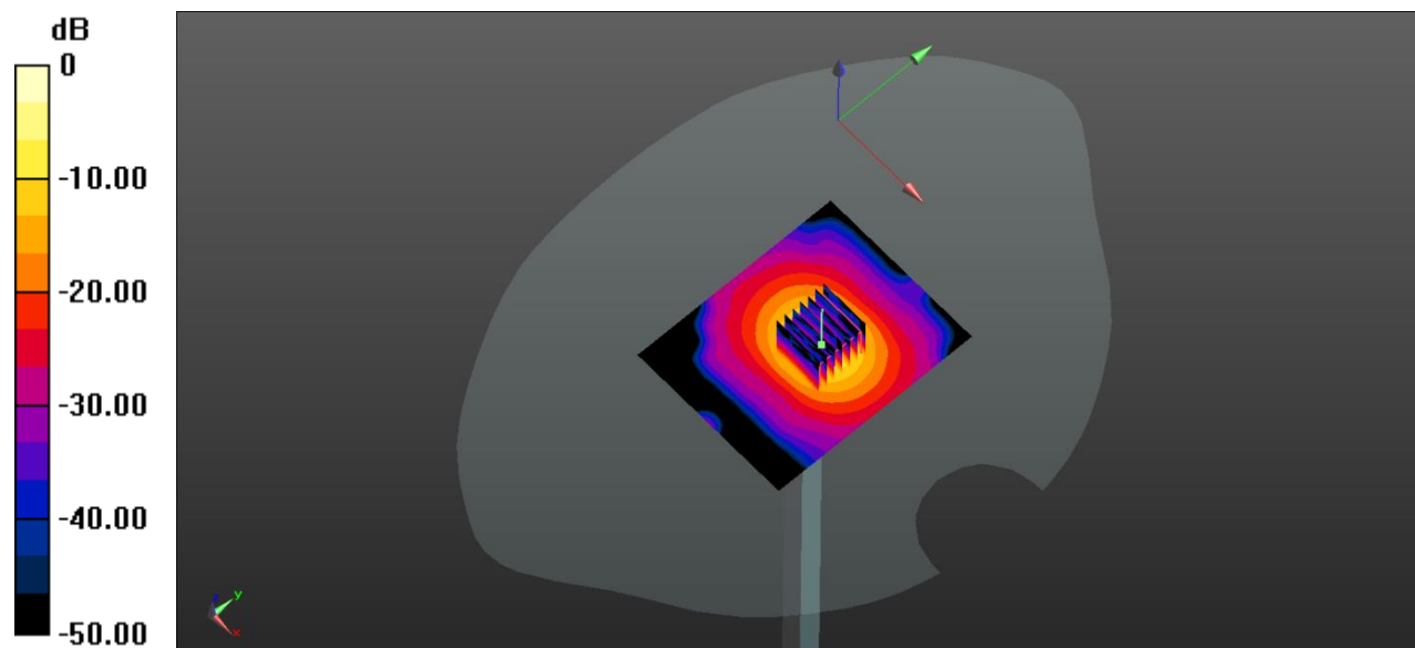
0 dB = 19.3 W/kg
