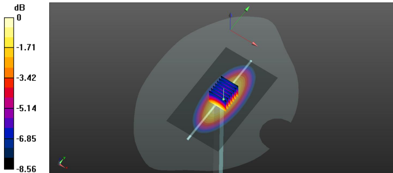
0 dB = 0.951 W/kg
