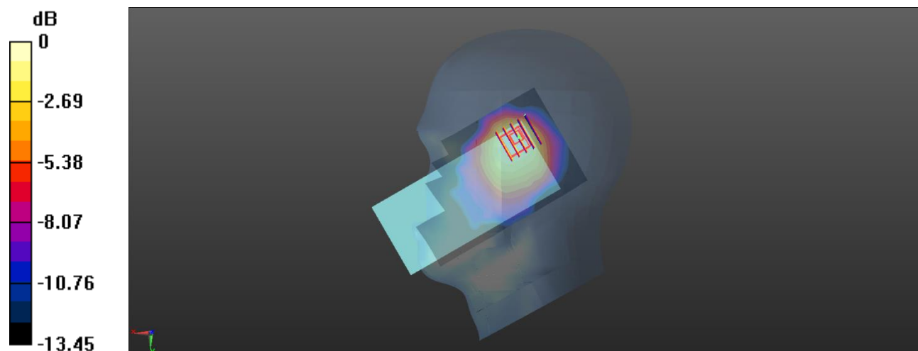
0 dB = 0.545 W/kg
