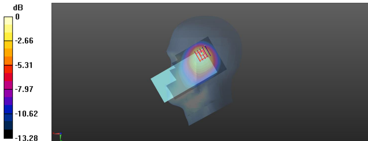
0 dB = 0.635 W/kg
