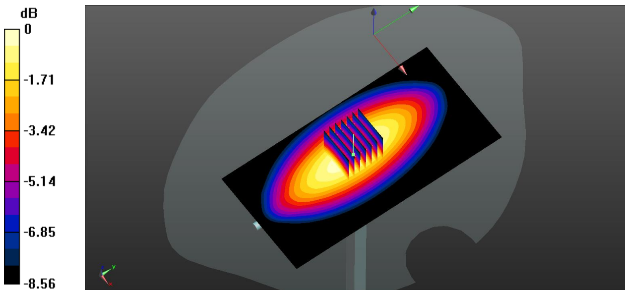
0 dB = 0.932 W/kg
