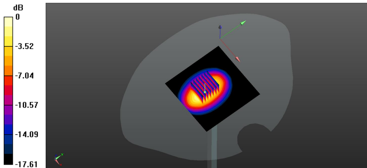
0 dB = 4.21 W/kg
