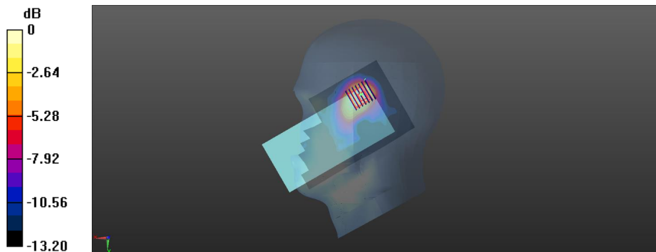
0 dB = 0.742 W/kg
