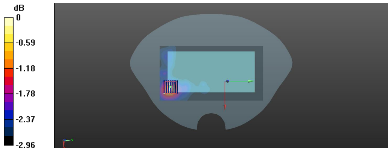
0 dB = 0.221 W/kg
