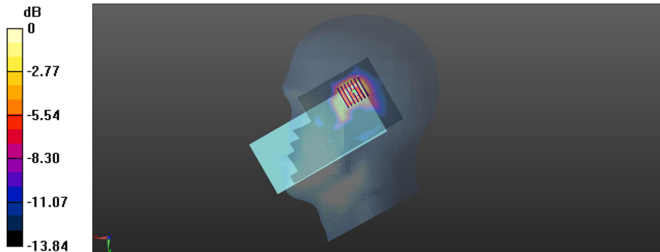
0 dB = 0.682 W/kg
