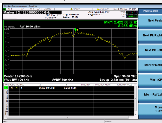
802.11b CHANNEL 3, CARRIER LEVEL
