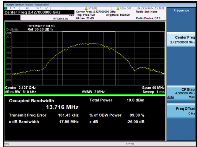
802.11b CHANNEL 4
