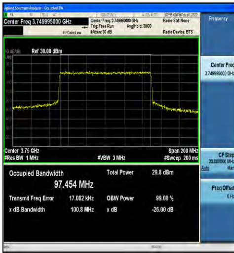
1-N78-3700-3800-30-100-H-7-CP-16QAM-Outer_Ful I-273@0-Ant4-97.454-100.8-≤100-PASS
