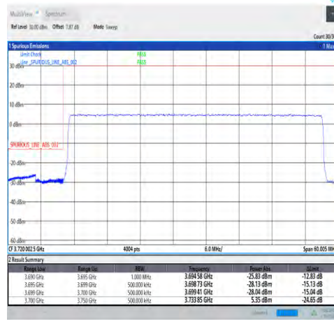
1-N78-3700-3800-30-50-L-3-DFT-PI2BPSK-Outer _Full-128@0-Ant4-PASS-see graph
