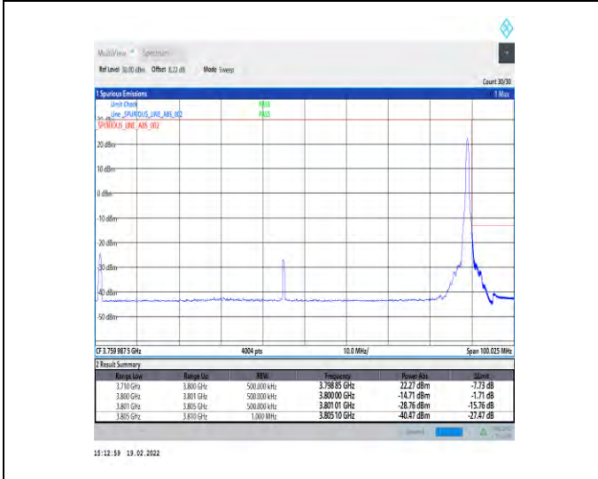
1-N78-3700-3800-30-90-H-5-CP-QPSK-Edge_1RB_Right-1@244-Ant4-PASS-see graph
