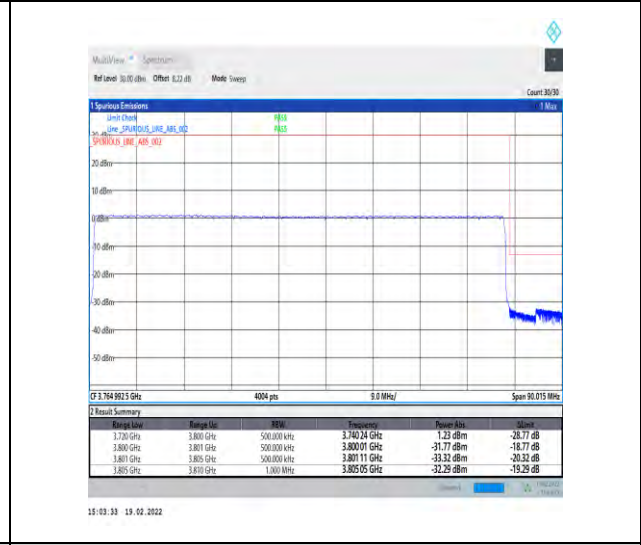
1-N78-3700-3800-30-80-H-6-CP-QPSK-Outer_Full-217@0-Ant4-PASS-see graph
