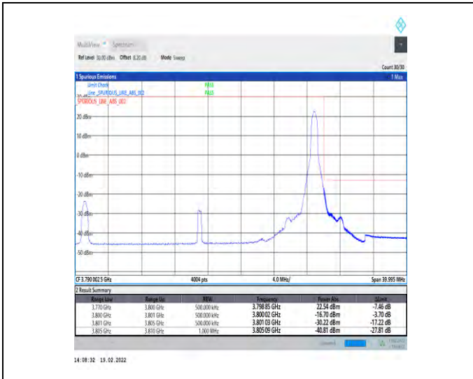
1-N78-3700-3800-30-30-H-2-DFT-PI2BPSK-Edge_1R B_Right-1@77-Ant4-PASS-see graph
