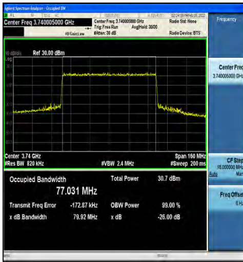
1-N78-3700-3800-30-80-L-3-DFT-16QAM-Outer_Full -216@0-Ant4-77.031-79.92-<math>\leq 80</math>-PASS
