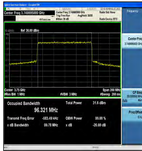
1-N78-3700-3800-30-100-L-2-DFT-PI2BPSK-Outer_Full Full-270@0-Ant4-96.321-99.78-≤100-PASS
