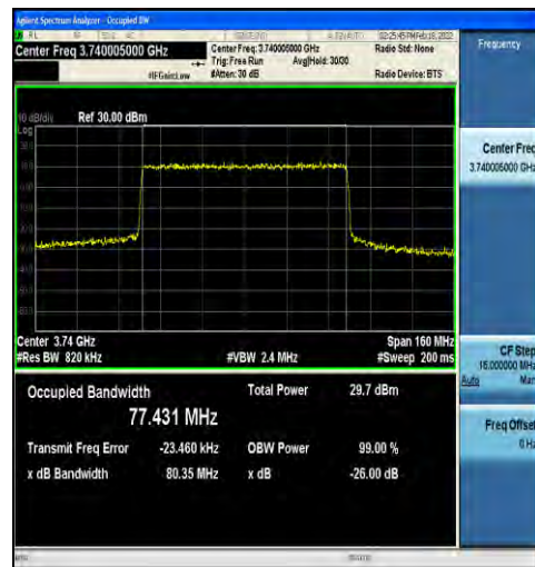
1-N78-3700-3800-30-80-L-6-CP-QPSK-Outer_Full-2 17@0-Ant4-77.431-80.35-<math>\leq 80</math>-PASS
