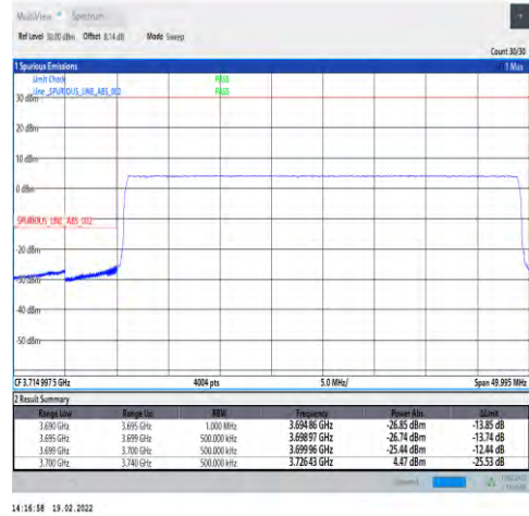
1-N78-3700-3800-30-40-L-6-CP-QPSK-Outer_Full-106@0-Ant4-PASS-see graph
