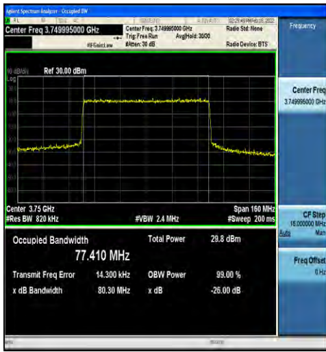
1-N78-3700-3800-30-80-M-6-CP-QPSK-Outer_Full-2 17@0-Ant4-77.410-80.30-≤80-PASS
