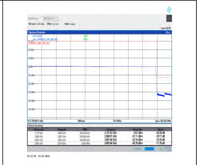
1-N78-3700-3800-30-90-H-6-CP-QPSK-Outer_Full-245@0-Ant4-PASS-see graph
