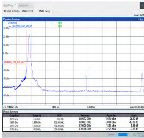
1-N78-3700-3800-30-50-L-4-CP-QPSK-Edge_1RB_Lef t-1@0-Ant4-PASS-see graph
