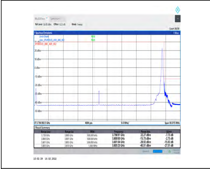
1-N78-3700-3800-30-80-H-5-CP-QPSK-Edge_1RB_Right-1@216-Ant4-PASS-see graph
