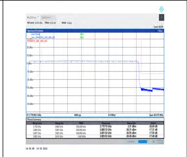
1-N78-3700-3800-30-50-H-6-CP-QPSK-Outer_Full-133@0-Ant4-PASS-see graph
