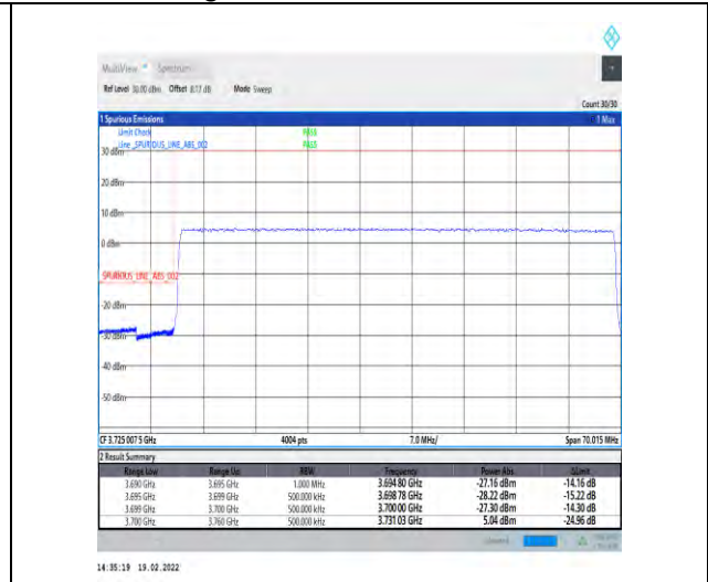
1-N78-3700-3800-30-60-L-3-DFT-PI2BPSK-Outer _Full-162@0-Ant4-PASS-see graph
