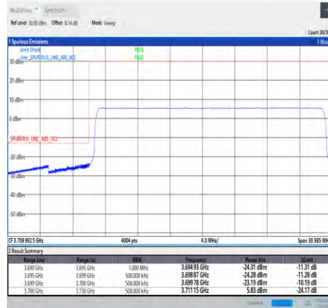
1-N78-3700-3800-30-30-L-6-CP-QPSK-Outer_Full -78@0-Ant4-PASS-see graph
