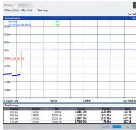
1-N78-3700-3800-30-70-L-6-CP-QPSK-Outer_Full -189@0-Ant4-PASS-see graph
