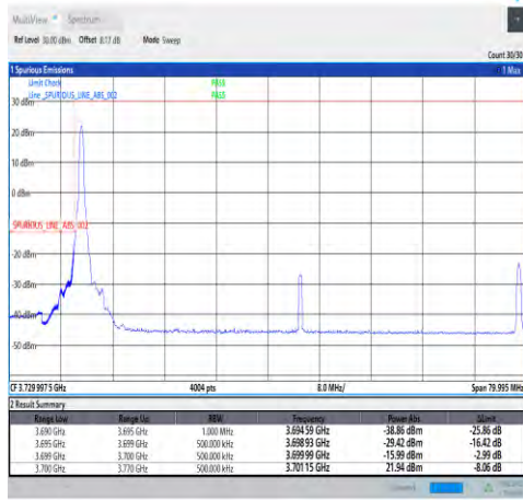
1-N78-3700-3800-30-70-L-4-CP-QPSK-Edge_1RB_Lef t-1@0-Ant4-PASS-see graph
