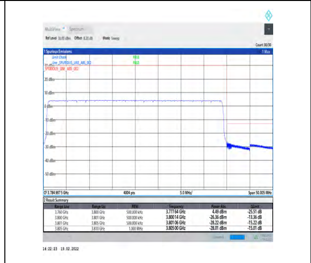
1-N78-3700-3800-30-40-H-6-CP-QPSK-Outer_Full-106@0-Ant4-PASS-see graph
