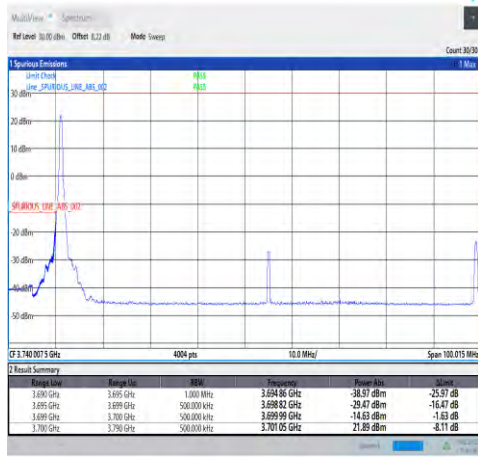
1-N78-3700-3800-30-90-L-4-CP-QPSK-Edge_1RB_Lef t-1@0-Ant4-PASS-see graph
