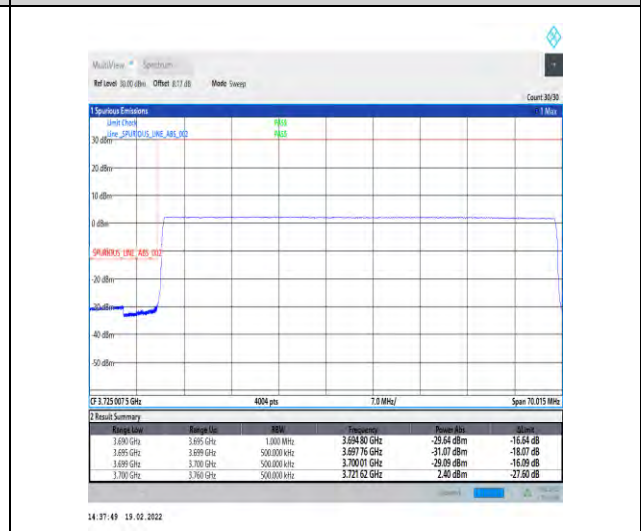
1-N78-3700-3800-30-60-L-6-CP-QPSK-Outer_Full -162@0-Ant4-PASS-see graph
