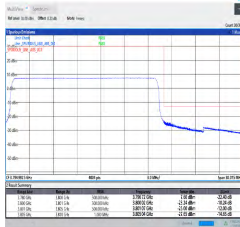
1-N78-3700-3800-30-20-H-6-CP-QPSK-Outer_Full-51@0-Ant4-PASS-see graph
