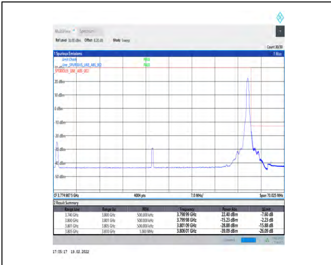
1-N78-3700-3800-30-60-H-2-DFT-PI2BPSK-Edge_1R_B_Right-1@161-Ant4-PASS-see graph
