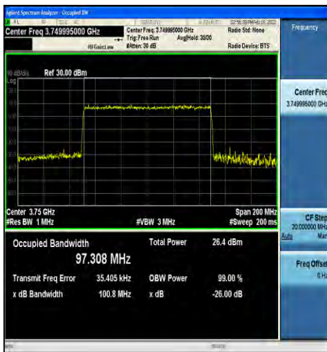
1-N78-3700-3800-30-100-H-9-CP-256QAM-Outer_F ull-273@0-Ant4-97.308-100.8-≤100-PASS
