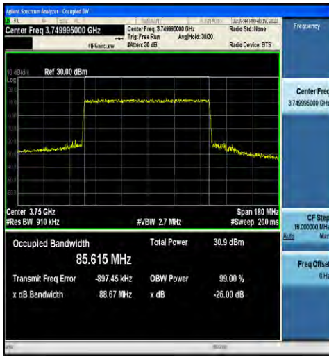
1-N78-3700-3800-30-90-M-3-DFT-16QAM-Outer_Ful I-240@0-Ant4-85.615-88.67- \leq 90 -PASS
