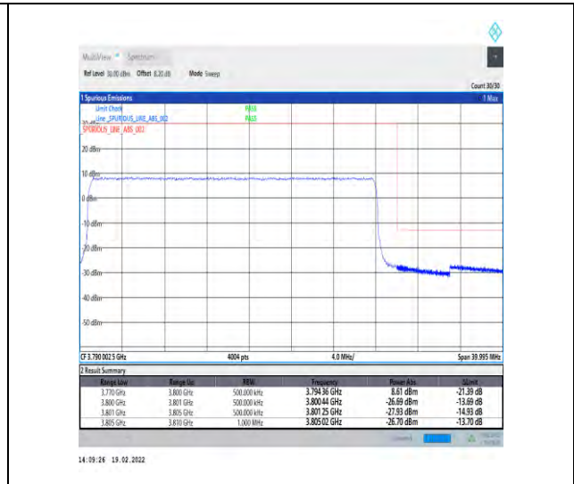
1-N78-3700-3800-30-30-H-3-DFT-PI2BPSK-Outer_Full-75@0-Ant4-PASS-see graph
