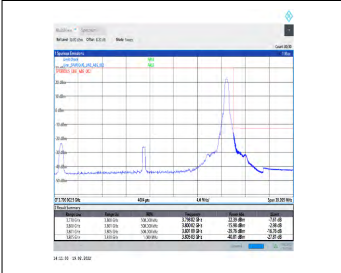
1-N78-3700-3800-30-30-H-5-CP-QPSK-Edge_1RB_Right-1@77-Ant4-PASS-see graph
