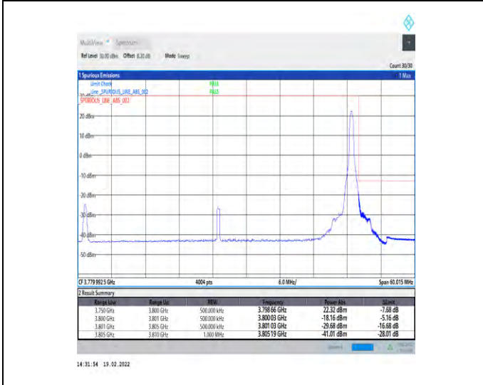
1-N78-3700-3800-30-50-H-5-CP-QPSK-Edge_1RB_Right-1@132-Ant4-PASS-see graph
