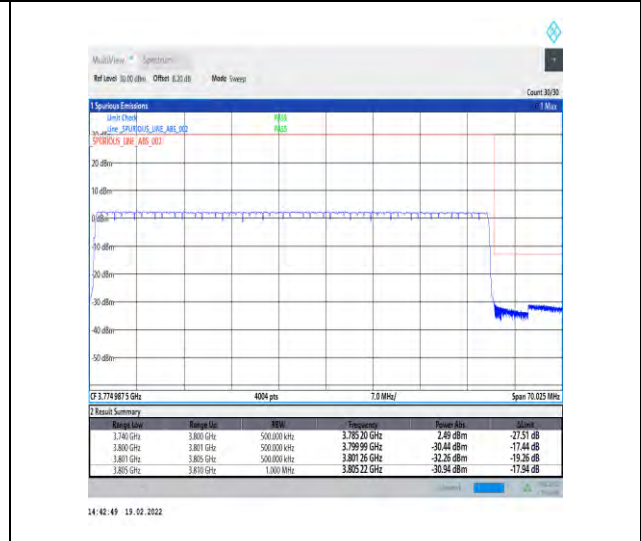
1-N78-3700-3800-30-60-H-6-CP-QPSK-Outer_Full-162@0-Ant4-PASS-see graph
