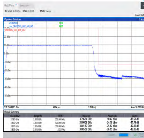
1-N78-3700-3800-30-20-H-3-DFT-PI2BPSK-Outer_Full-50@0-Ant4-PASS-see graph
