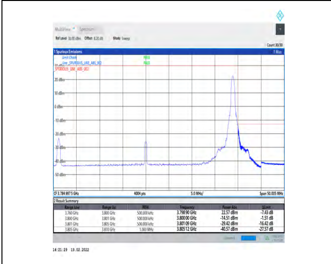
1-N78-3700-3800-30-40-H-5-CP-QPSK-Edge_1RB_Right-1@105-Ant4-PASS-see graph
