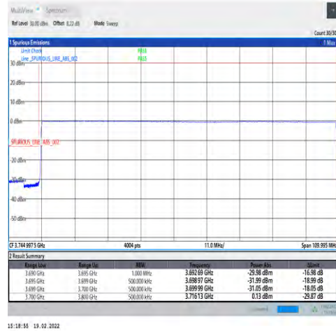
1-N78-3700-3800-30-100-L-6-CP-QPSK-Outer_Ful I-273@0-Ant4-PASS-see graph
