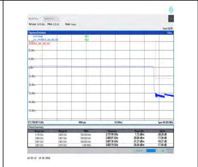
1-N78-3700-3800-30-70-H-6-CP-QPSK-Outer_Full-189@0-Ant4-PASS-see graph
