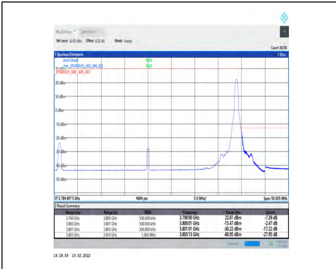
1-N78-3700-3800-30-40-H-2-DFT-PI2BPSK-Edge_1R_B_Right-1@105-Ant4-PASS-see graph
