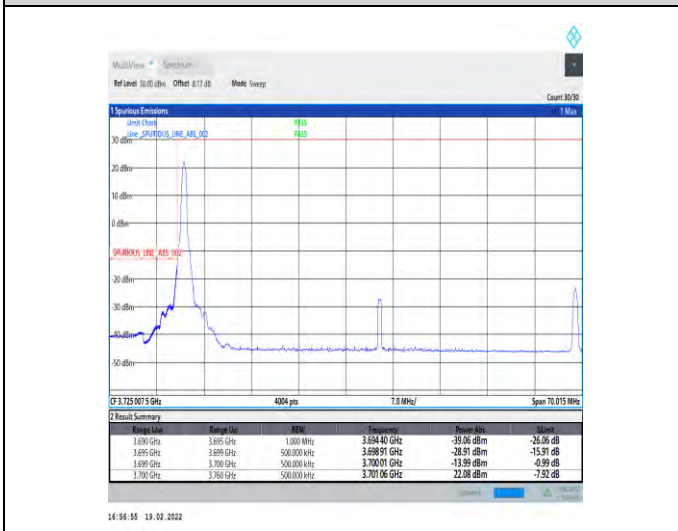
1-N78-3700-3800-30-60-L-4-CP-QPSK-Edge_1RB_Lef t-1@0-Ant4-PASS-see graph
