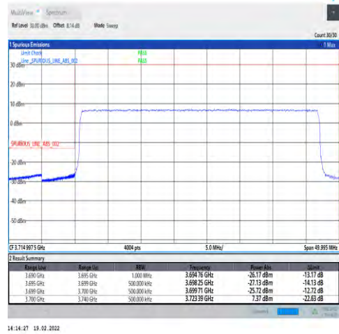
1-N78-3700-3800-30-40-L-3-DFT-PI2BPSK-Outer_Full-100@0-Ant4-PASS-see graph
