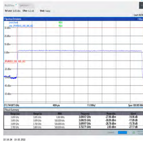
1-N78-3700-3800-30-100-L-3-DFT-PI2BPSK-Outer_Full-270@0-Ant4-PASS-see graph
