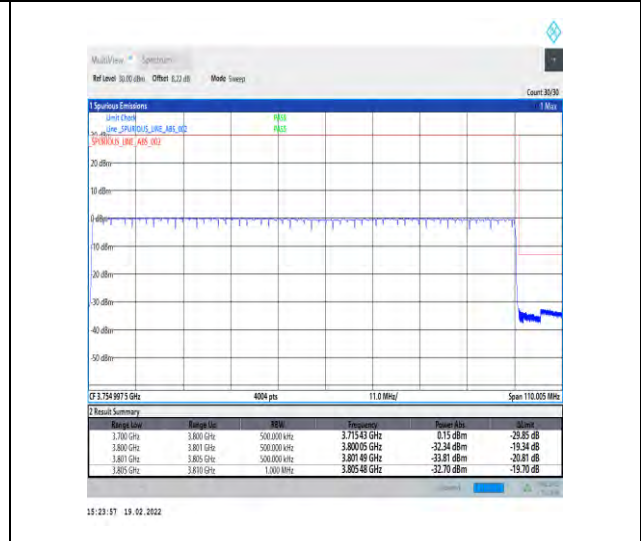
1-N78-3700-3800-30-100-H-6-CP-QPSK-Outer_Full-273@0-Ant4-PASS-see graph
