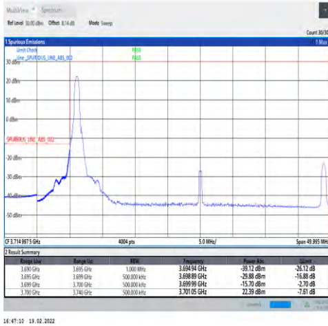
1-N78-3700-3800-30-40-L-4-CP-QPSK-Edge_1RB_Left-1@0-Ant4-PASS-see graph
