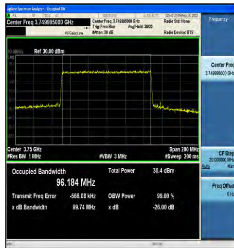
1-N78-3700-3800-30-100-L-4-DFT-64QAM-Outer_Full ull-270@0-Ant4-96.184-99.74-≤100-PASS
