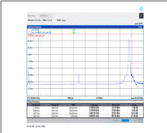
1-N78-3700-3800-30-80-H-2-DFT-PI2BPSK-Edge_1R_B_Right-1@216-Ant4-PASS-see graph
