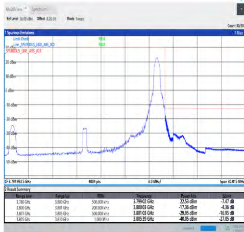
1-N78-3700-3800-30-20-H-5-CP-QPSK-Edge_1RB_Right-1@50-Ant4-PASS-see graph
