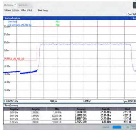
1-N78-3700-3800-30-30-L-3-DFT-PI2BPSK-Outer _Full-75@0-Ant4-PASS-see graph
