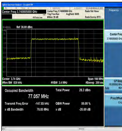
1-N78-3700-3800-30-80-L-5-DFT-256QAM-Outer_Fu II-216@0-Ant4-77.057-79.85-<math>\leq 80</math>-PASS
