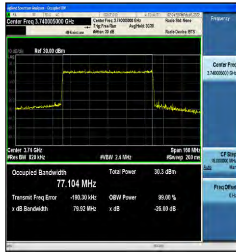
1-N78-3700-3800-30-80-L-4-DFT-64QAM-Outer_Full -216@0-Ant4-77.104-79.92-<math>\leq 80</math>-PASS
