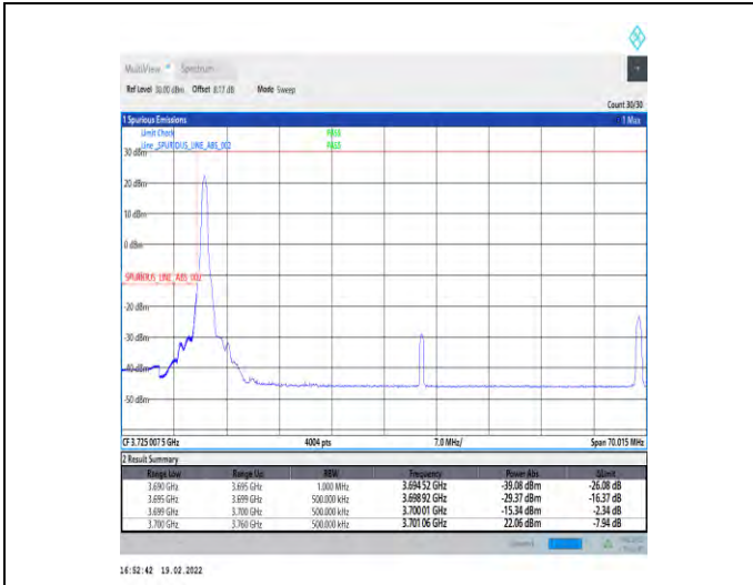
1-N78-3700-3800-30-60-L-1-DFT-PI2BPSK-Edge_1RB _Left-1@0-Ant4-PASS-see graph
