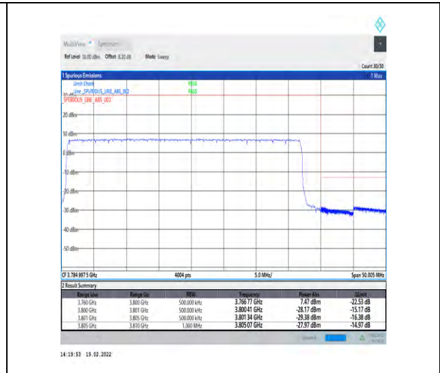
1-N78-3700-3800-30-40-H-3-DFT-PI2BPSK-Outer_Full-100@0-Ant4-PASS-see graph
