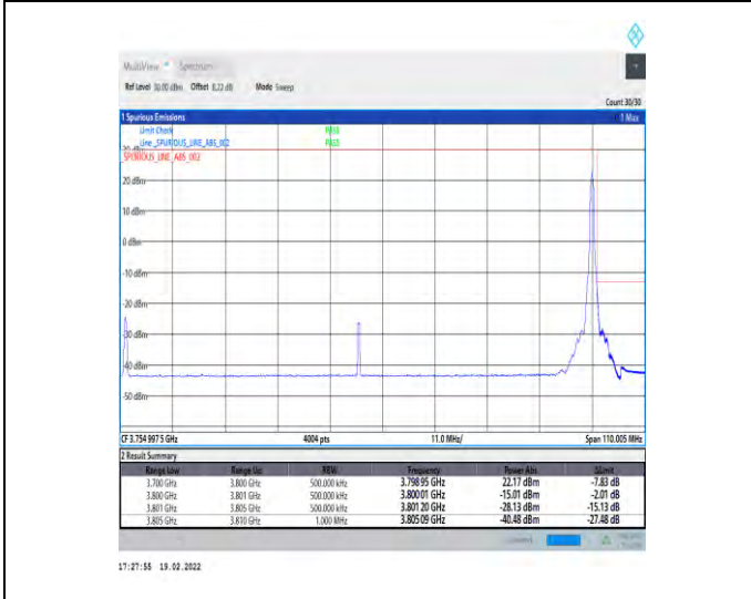
1-N78-3700-3800-30-100-H-5-CP-QPSK-Edge_1RB_Right-1@272-Ant4-PASS-see graph
