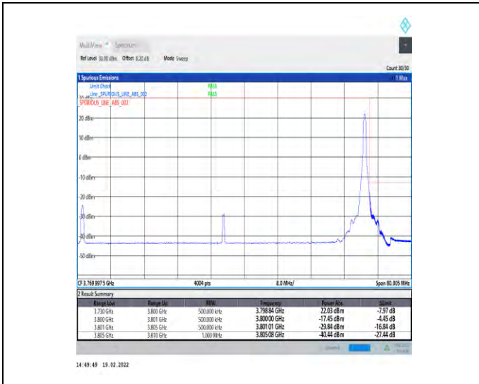
1-N78-3700-3800-30-70-H-2-DFT-PI2BPSK-Edge_1R_B_Right-1@188-Ant4-PASS-see graph
