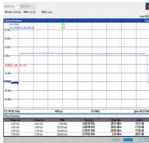
1-N78-3700-3800-30-90-L-3-DFT-PI2BPSK-Outer _Full-240@0-Ant4-PASS-see graph
