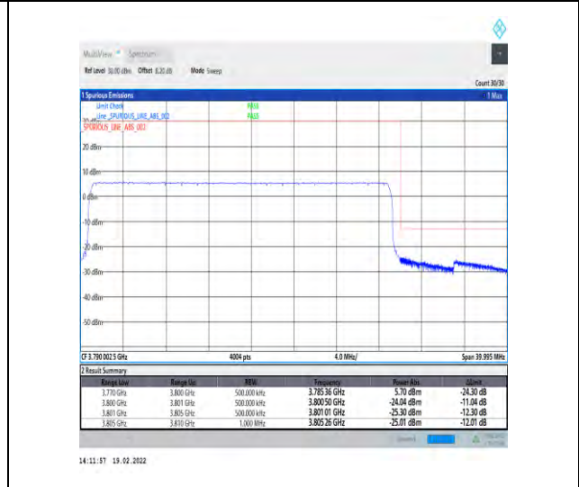
1-N78-3700-3800-30-30-H-6-CP-QPSK-Outer_Full-78@0-Ant4-PASS-see graph
