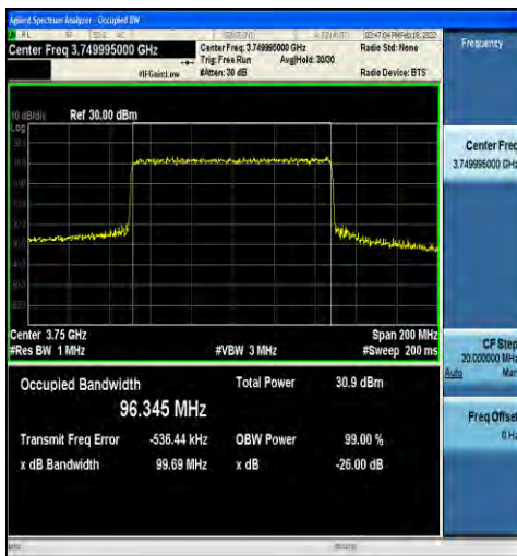
1-N78-3700-3800-30-100-L-3-DFT-16QAM-Outer_Full II-270@0-Ant4-96.345-99.69-≤100-PASS
