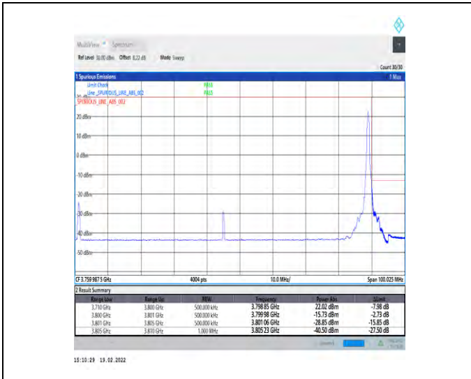
1-N78-3700-3800-30-90-H-2-DFT-PI2BPSK-Edge_1R_B_Right-1@244-Ant4-PASS-see graph
