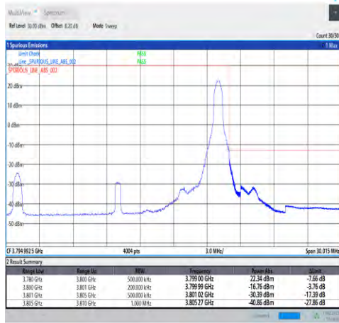
1-N78-3700-3800-30-20-H-2-DFT-PI2BPSK-Edge_1R_B_Right-1@50-Ant4-PASS-see graph
