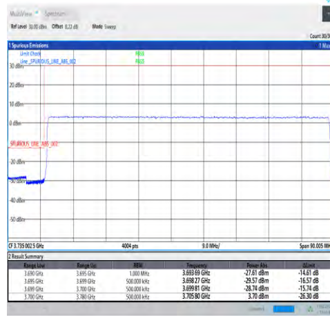
1-N78-3700-3800-30-80-L-3-DFT-PI2BPSK-Outer _Full-216@0-Ant4-PASS-see graph
