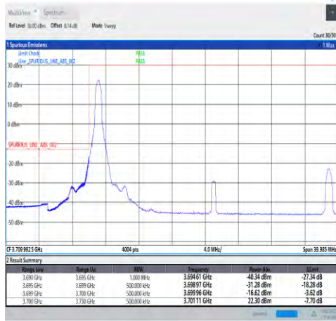
1-N78-3700-3800-30-30-L-1-DFT-PI2BPSK-Edge_1RB _Left-1@0-Ant4-PASS-see graph
