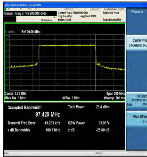
1-N78-3700-3800-30-100-H-8-CP-64QAM-Outer_Ful I-273@0-Ant4-97.429-100.7-≤100-PASS
