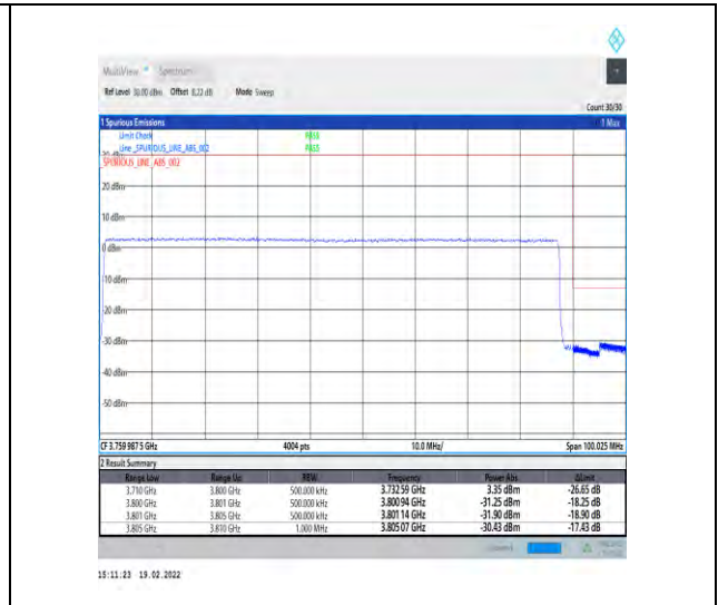
1-N78-3700-3800-30-90-H-3-DFT-PI2BPSK-Outer_Full-240@0-Ant4-PASS-see graph
