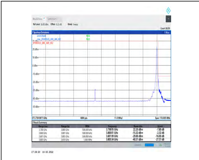
1-N78-3700-3800-30-100-H-2-DFT-PI2BPSK-Edge_1R_B_Right-1@272-Ant4-PASS-see graph
