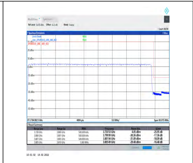
1-N78-3700-3800-30-80-H-3-DFT-PI2BPSK-Outer_Full-216@0-Ant4-PASS-see graph
