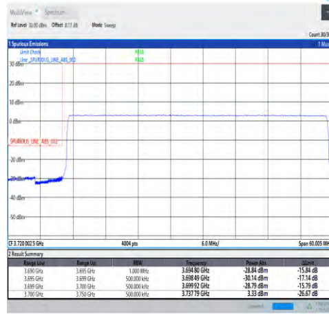
1-N78-3700-3800-30-50-L-6-CP-QPSK-Outer_Full -133@0-Ant4-PASS-see graph
