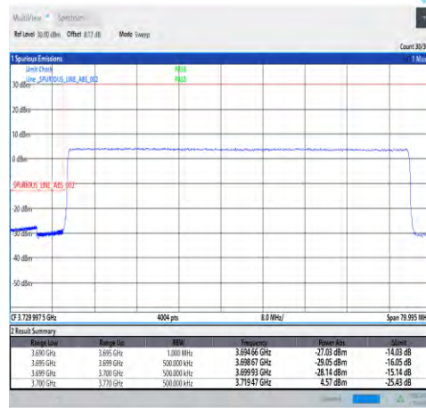
1-N78-3700-3800-30-70-L-3-DFT-PI2BPSK-Outer_Full-180@0-Ant4-PASS-see graph
