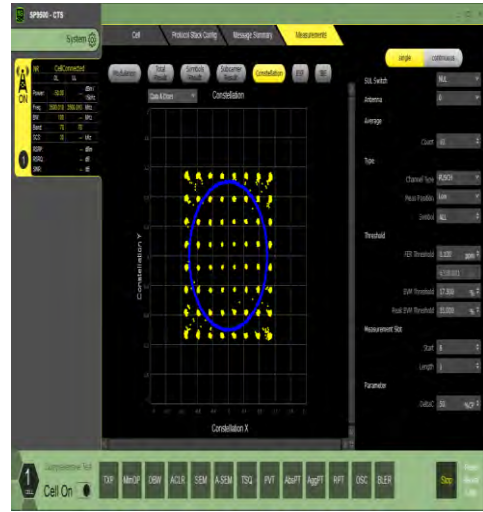
1-N78-3450-3550-30-100-M-4-DFT-64QAM-Outer_Full-270@0-Ant4-see graph-PASS
