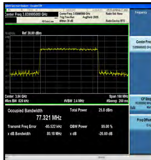
1-N77-3700-3980-30-80-M-9-CP-256QAM-Outer_Fu II-217@0-Ant4-77.321-80.18-≤80-PASS
