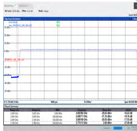
1-N77-3700-3980-30-80-L-3-DFT-PI2BPSK-Outer _Full-216@0-Ant4-PASS-see graph
