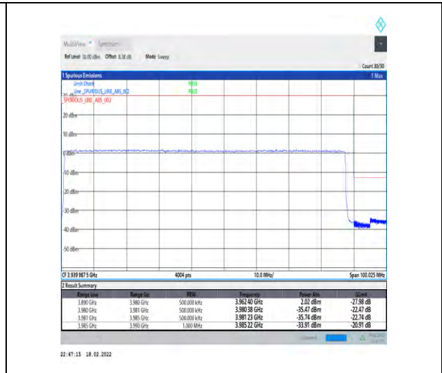
1-N77-3700-3980-30-90-H-3-DFT-PI2BPSK-Outer_Full-240@0-Ant4-PASS-see graph
