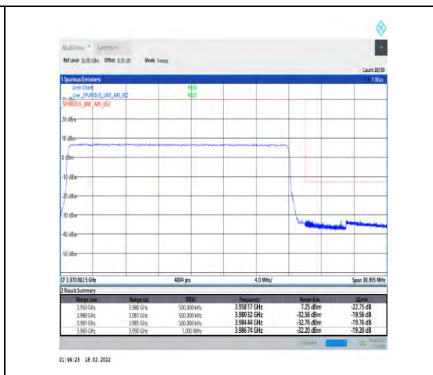
1-N77-3700-3980-30-30-H-3-DFT-PI2BPSK-Outer_Full-75@0-Ant4-PASS-see graph
