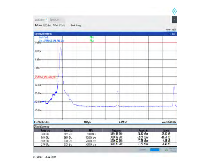
1-N77-3700-3980-30-50-L-1-DFT-PI2BPSK-Edge_1RB_Left-1@0-Ant4-PASS-see graph
