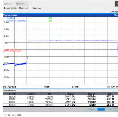
1-N77-3700-3980-30-40-L-6-CP-QPSK-Outer_Full-106@0-Ant4-PASS-see graph
