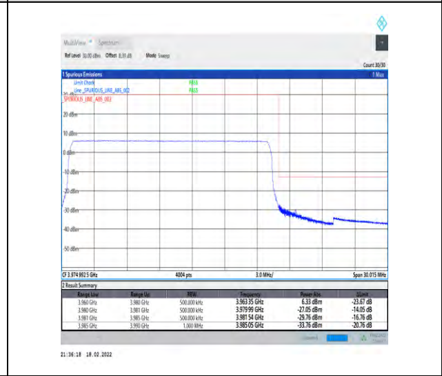
1-N77-3700-3980-30-20-H-6-CP-QPSK-Outer_Full-51@0-Ant4-PASS-see graph
