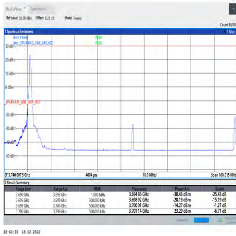
1-N77-3700-3980-30-90-L-1-DFT-PI2BPSK-Edge_1RB _Left-1@0-Ant4-PASS-see graph
