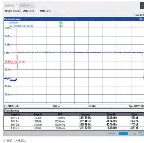
1-N77-3700-3980-30-100-L-3-DFT-PI2BPSK-Outer_Full-270@0-Ant4-PASS-see graph
