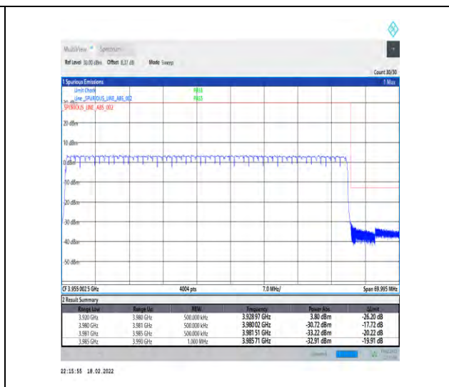
1-N77-3700-3980-30-60-H-3-DFT-PI2BPSK-Outer_Full-162@0-Ant4-PASS-see graph
