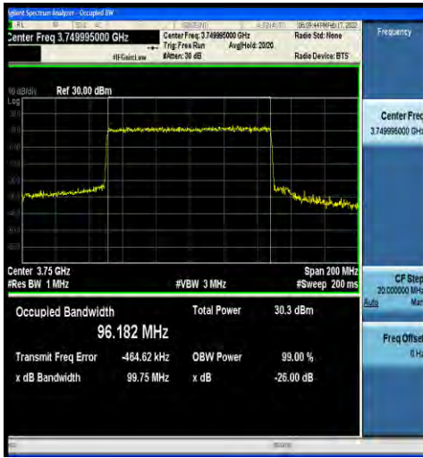
1-N77-3700-3980-30-100-L-1-DFT-QPSK-Outer_Full -270@0-Ant4-96.182-99.75-≤100-PASS
