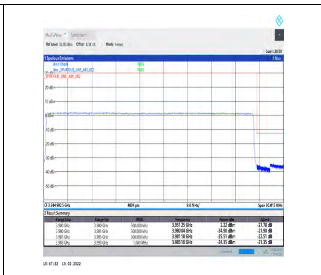
1-N77-3700-3980-30-80-H-3-DFT-PI2BPSK-Outer_Full-216@0-Ant4-PASS-see graph
