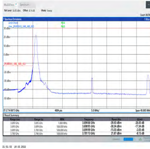
1-N77-3700-3980-30-40-L-4-CP-QPSK-Edge_1RB_Left-1@0-Ant4-PASS-see graph
