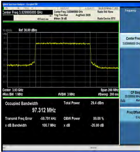
1-N77-3700-3980-30-100-H-7-CP-16QAM-Outer_Ful I-273@0-Ant4-97.312-100.7-≤100-PASS
