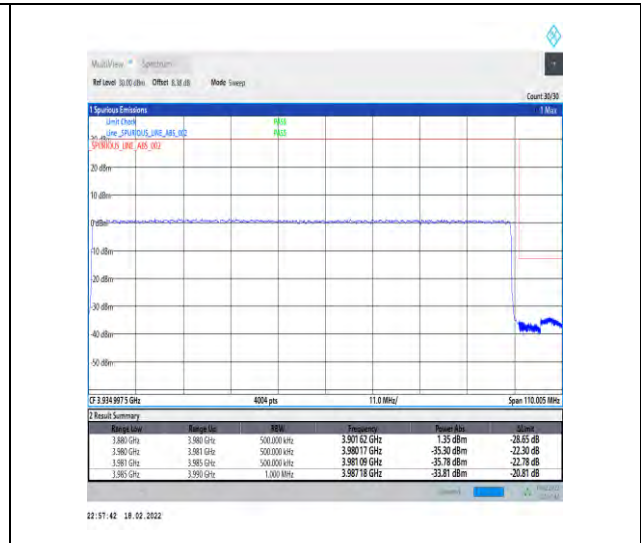
1-N77-3700-3980-30-100-H-3-DFT-PI2BPSK-Outer_Full-270@0-Ant4-PASS-see graph
