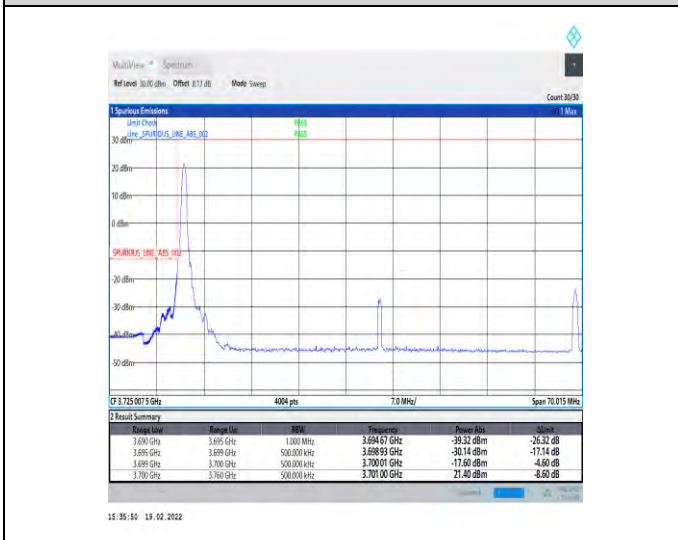
1-N77-3700-3980-30-60-L-4-CP-QPSK-Edge_1RB_Lef t-1@0-Ant4-PASS-see graph
