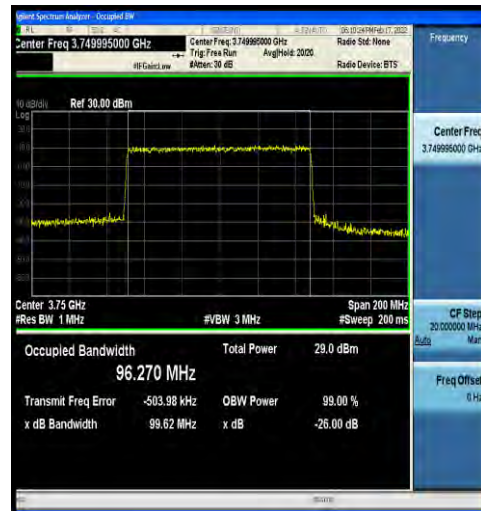
1-N77-3700-3980-30-100-L-4-DFT-64QAM-Outer_Full -270@0-Ant4-96.270-99.62-≤100-PASS
