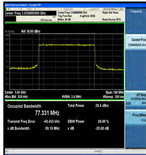
1-N77-3700-3980-30-80-M-7-CP-16QAM-Outer_Full -217@0-Ant4-77.331-80.19-≤80-PASS
