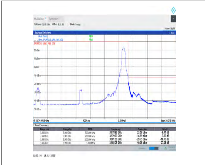
1-N77-3700-3980-30-20-H-2-DFT-PI2BPSK-Edge_1R_B_Right-1@50-Ant4-PASS-see graph
