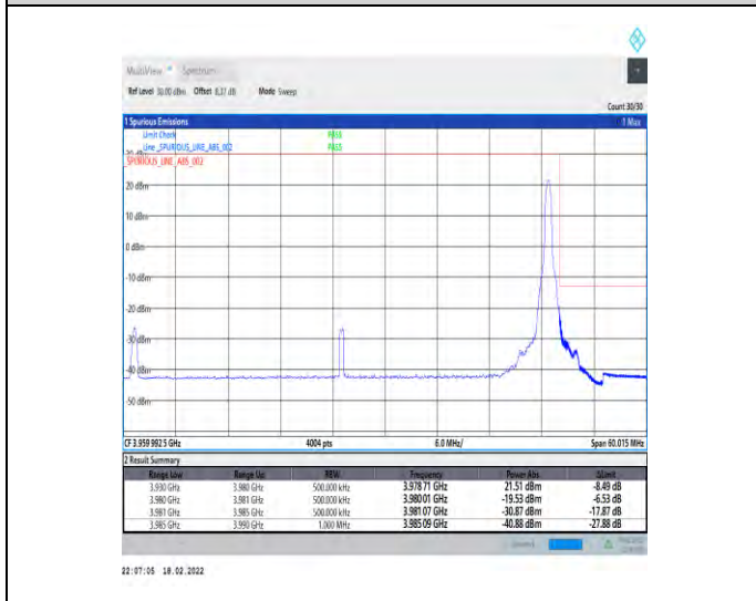
1-N77-3700-3980-30-50-H-5-CP-QPSK-Edge_1RB_Right-1@132-Ant4-PASS-see graph
