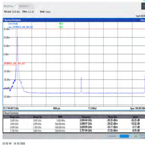
1-N77-3700-3980-30-100-L-4-CP-QPSK-Edge_1RB_L_eft-1@0-Ant4-PASS-see graph
