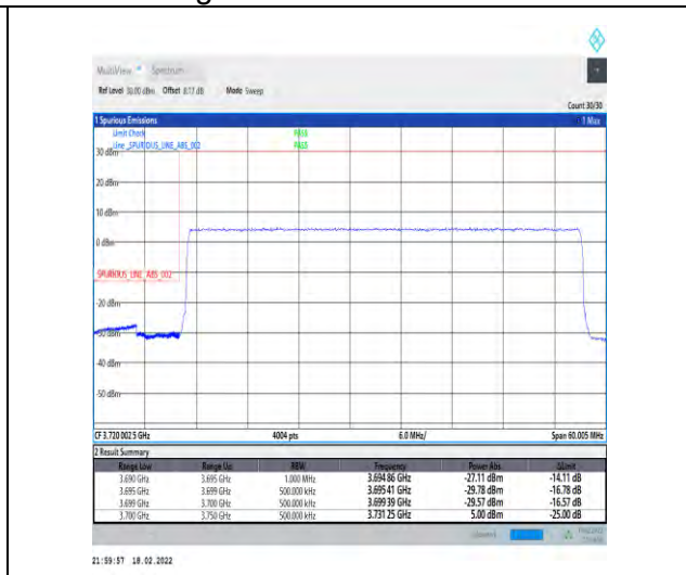
1-N77-3700-3980-30-50-L-3-DFT-PI2BPSK-Outer_Full-128@0-Ant4-PASS-see graph
