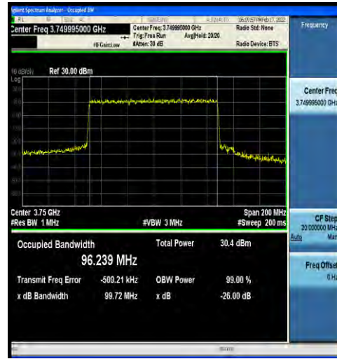
1-N77-3700-3980-30-100-L-2-DFT-PI2BPSK-Outer_Full -270@0-Ant4-96.239-99.72-≤100-PASS
