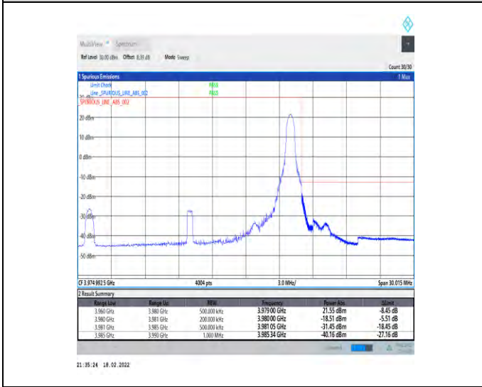
1-N77-3700-3980-30-20-H-5-CP-QPSK-Edge_1RB_Right-1@50-Ant4-PASS-see graph
