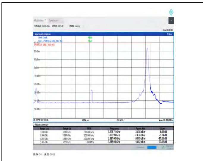
1-N77-3700-3980-30-50-H-2-DFT-PI2BPSK-Edge_1R_B_Right-1@132-Ant4-PASS-see graph
