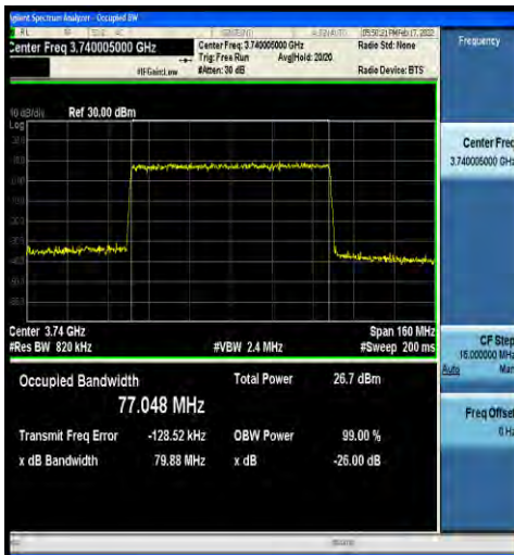
1-N77-3700-3980-30-80-L-5-DFT-256QAM-Outer_Fu II-216@0-Ant4-77.048-79.88-<math>\leq 80</math>-PASS
