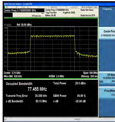
1-N77-3700-3980-30-80-L-6-CP-QPSK-Outer_Full-2 17@0-Ant4-77.455-80.15-<math>\leq 80</math>-PASS
