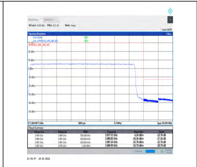
1-N77-3700-3980-30-40-H-3-DFT-PI2BPSK-Outer_Full-100@0-Ant4-PASS-see graph
