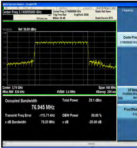
1-N77-3700-3980-30-80-L-3-DFT-16QAM-Outer_Full -216@0-Ant4-76.945-79.93-<math>\leq 80</math>-PASS
