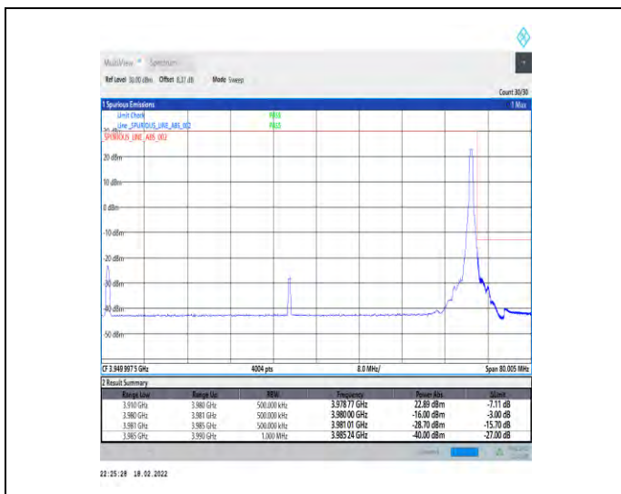
1-N77-3700-3980-30-70-H-2-DFT-PI2BPSK-Edge_1R_B_Right-1@188-Ant4-PASS-see graph
