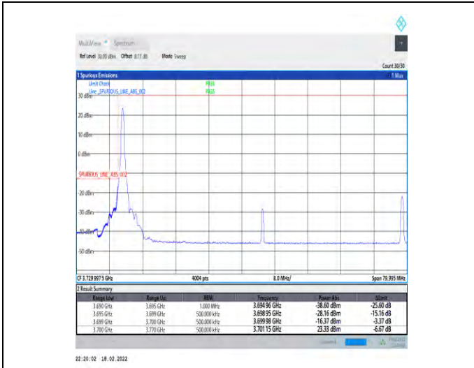
1-N77-3700-3980-30-70-L-1-DFT-PI2BPSK-Edge_1RB _Left-1@0-Ant4-PASS-see graph
