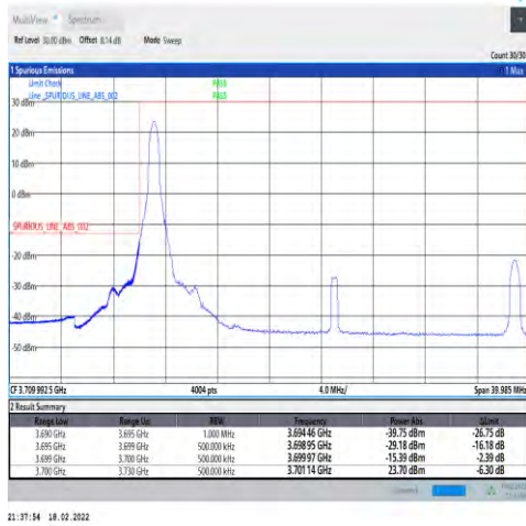
1-N77-3700-3980-30-30-L-1-DFT-PI2BPSK-Edge_1RB _Left-1@0-Ant4-PASS-see graph
