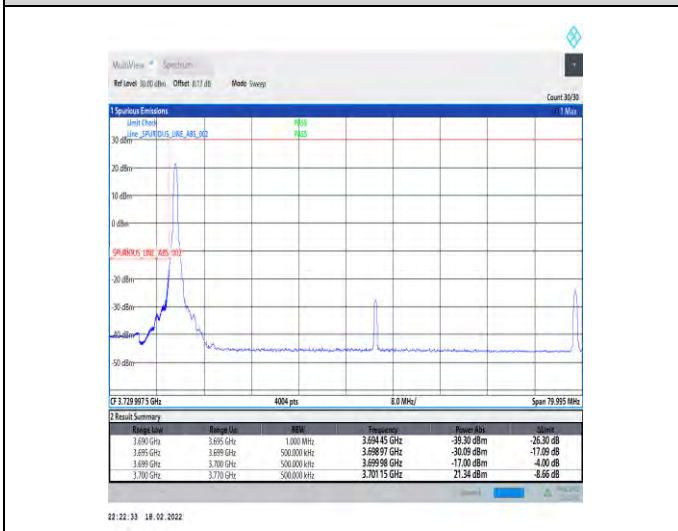
1-N77-3700-3980-30-70-L-4-CP-QPSK-Edge_1RB_Lef t-1@0-Ant4-PASS-see graph
