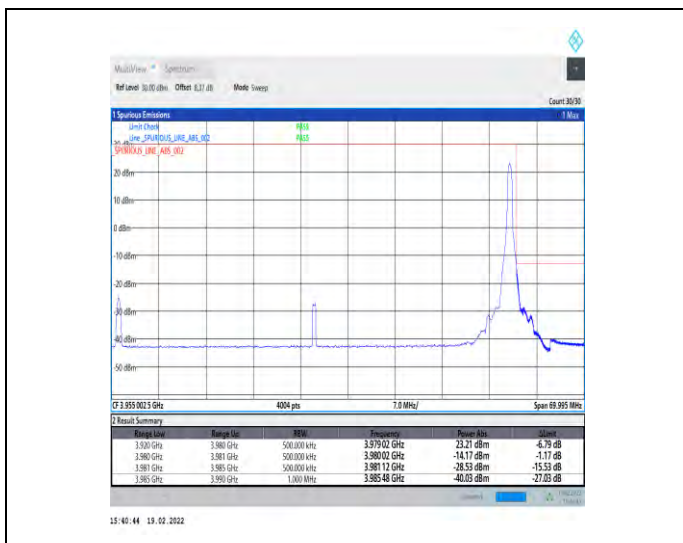
1-N77-3700-3980-30-60-H-2-DFT-PI2BPSK-Edge_1R_B_Right-1@161-Ant4-PASS-see graph
