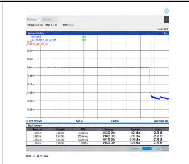
1-N77-3700-3980-30-70-H-6-CP-QPSK-Outer_Full-189@0-Ant4-PASS-see graph
