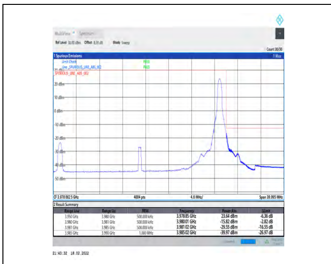
1-N77-3700-3980-30-30-H-2-DFT-PI2BPSK-Edge_1R_B_Right-1@77-Ant4-PASS-see graph
