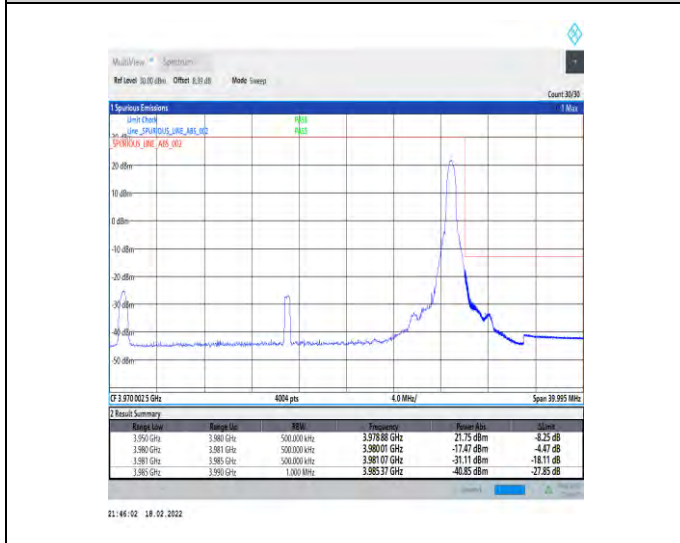
1-N77-3700-3980-30-30-H-5-CP-QPSK-Edge_1RB_Right-1@77-Ant4-PASS-see graph
