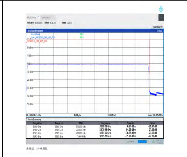
1-N77-3700-3980-30-90-H-6-CP-QPSK-Outer_Full-245@0-Ant4-PASS-see graph
