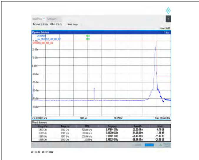
1-N77-3700-3980-30-90-H-2-DFT-PI2BPSK-Edge_1R_B_Right-1@244-Ant4-PASS-see graph
