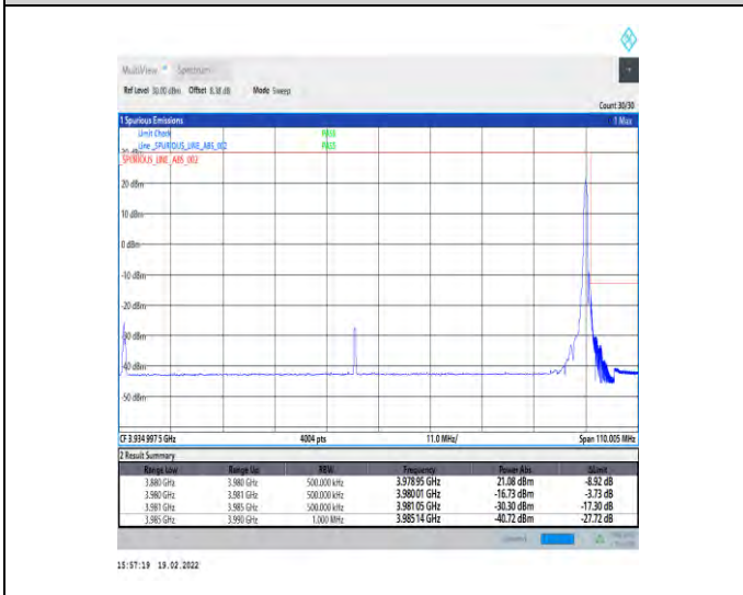
1-N77-3700-3980-30-100-H-5-CP-QPSK-Edge_1RB_Right-1@272-Ant4-PASS-see graph
