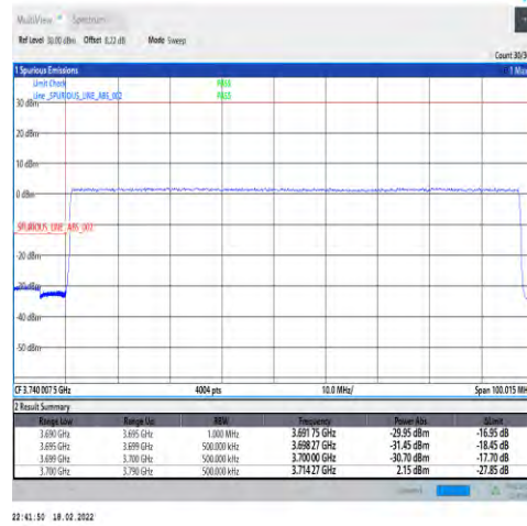
1-N77-3700-3980-30-90-L-3-DFT-PI2BPSK-Outer _Full-240@0-Ant4-PASS-see graph
