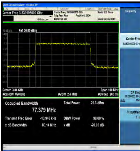
1-N77-3700-3980-30-80-M-6-CP-QPSK-Outer_Full-2 17@0-Ant4-77.379-80.14-≤80-PASS
