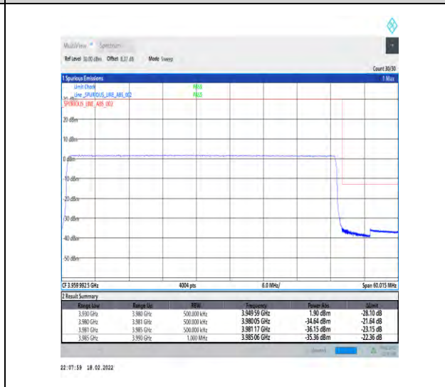
1-N77-3700-3980-30-50-H-6-CP-QPSK-Outer_Full-133@0-Ant4-PASS-see graph
