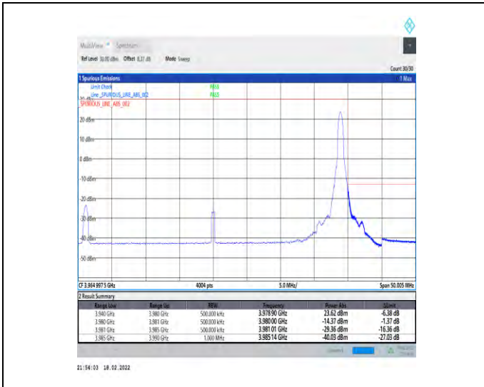
1-N77-3700-3980-30-40-H-2-DFT-PI2BPSK-Edge_1R_B_Right-1@105-Ant4-PASS-see graph
