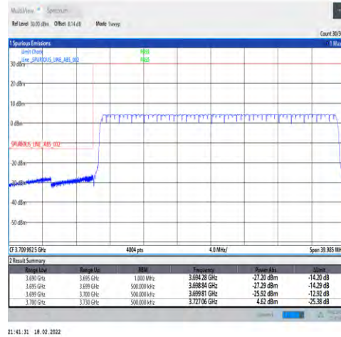
1-N77-3700-3980-30-30-L-6-CP-QPSK-Outer_Full -78@0-Ant4-PASS-see graph
