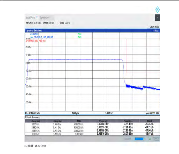
1-N77-3700-3980-30-30-H-6-CP-QPSK-Outer_Full-78@0-Ant4-PASS-see graph
