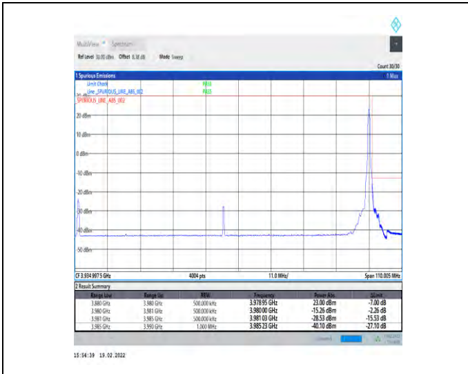
1-N77-3700-3980-30-100-H-2-DFT-PI2BPSK-Edge_1R_B_Right-1@272-Ant4-PASS-see graph
