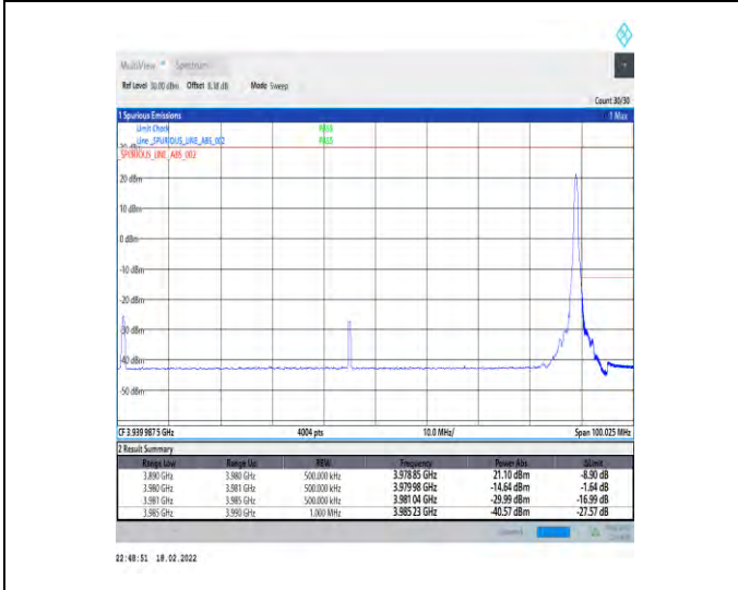
1-N77-3700-3980-30-90-H-5-CP-QPSK-Edge_1RB_Right-1@244-Ant4-PASS-see graph
