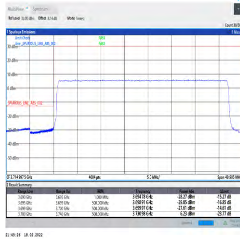
1-N77-3700-3980-30-40-L-3-DFT-PI2BPSK-Outer_Full-100@0-Ant4-PASS-see graph
