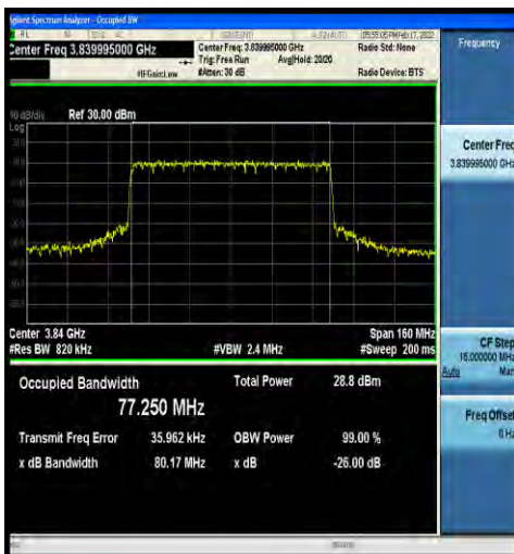
1-N77-3700-3980-30-80-M-8-CP-64QAM-Outer_Full- 217@0-Ant4-77.250-80.17-≤80-PASS
