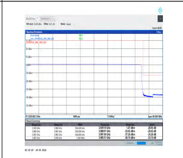
1-N77-3700-3980-30-60-H-6-CP-QPSK-Outer_Full-162@0-Ant4-PASS-see graph
