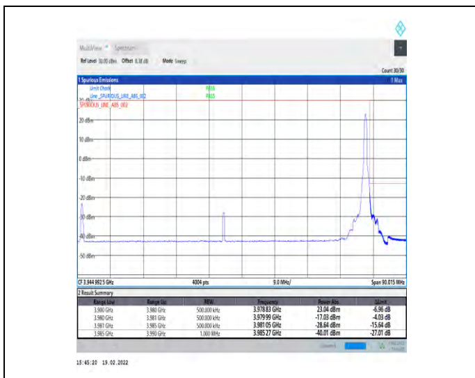
1-N77-3700-3980-30-80-H-2-DFT-PI2BPSK-Edge_1R_B_Right-1@216-Ant4-PASS-see graph
