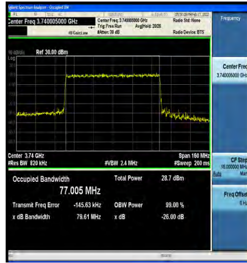
1-N77-3700-3980-30-80-L-4-DFT-64QAM-Outer_Full -216@0-Ant4-77.005-79.61-<math>\leq 80</math>-PASS
