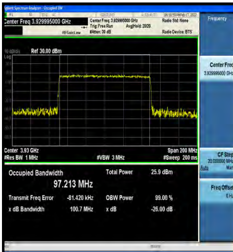
1-N77-3700-3980-30-100-H-9-CP-256QAM-Outer_F ull-273@0-Ant4-97.213-100.7-≤100-PASS
