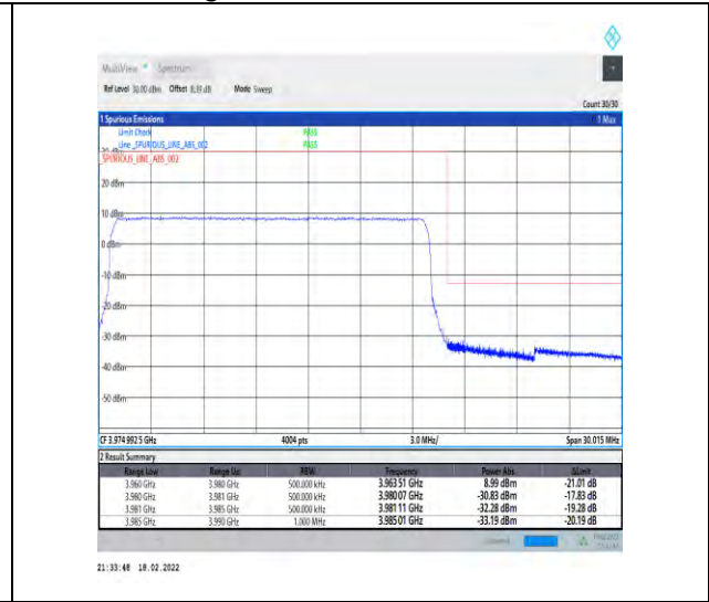
1-N77-3700-3980-30-20-H-3-DFT-PI2BPSK-Outer_Full-50@0-Ant4-PASS-see graph
