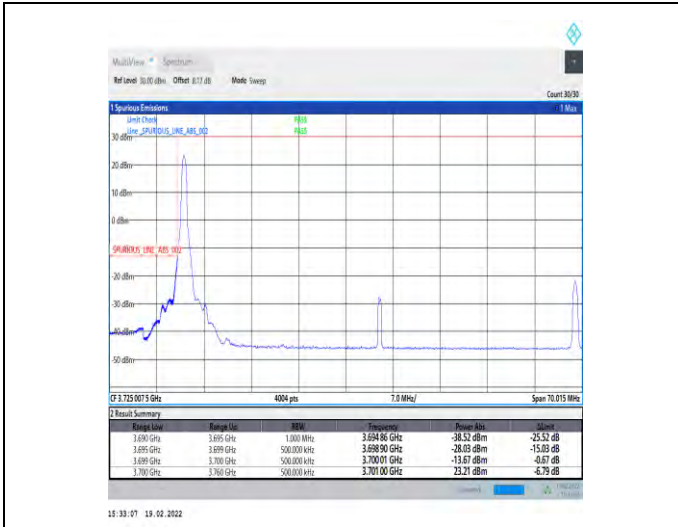
1-N77-3700-3980-30-60-L-1-DFT-PI2BPSK-Edge_1RB _Left-1@0-Ant4-PASS-see graph
