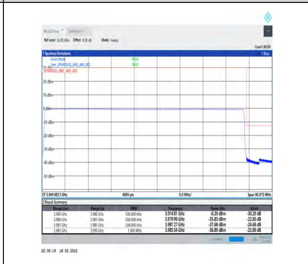
1-N77-3700-3980-30-80-H-6-CP-QPSK-Outer_Full-217@0-Ant4-PASS-see graph
