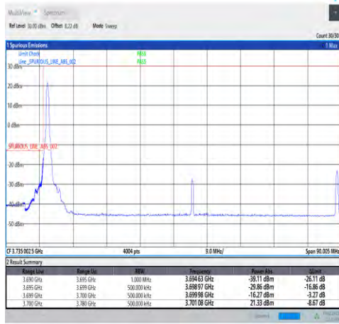
1-N77-3700-3980-30-80-L-4-CP-QPSK-Edge_1RB_Lef t-1@0-Ant4-PASS-see graph
