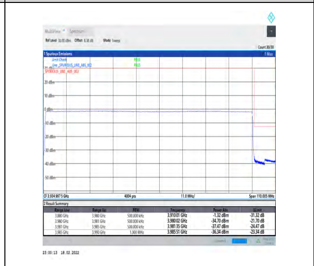
1-N77-3700-3980-30-100-H-6-CP-QPSK-Outer_Full-273@0-Ant4-PASS-see graph
