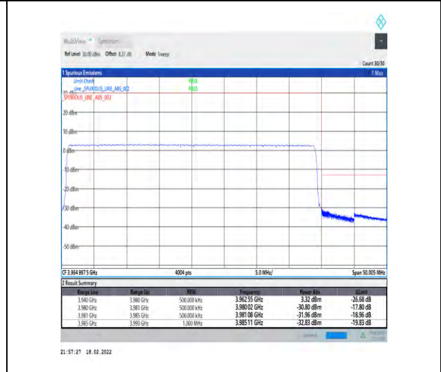
1-N77-3700-3980-30-40-H-6-CP-QPSK-Outer_Full-106@0-Ant4-PASS-see graph
