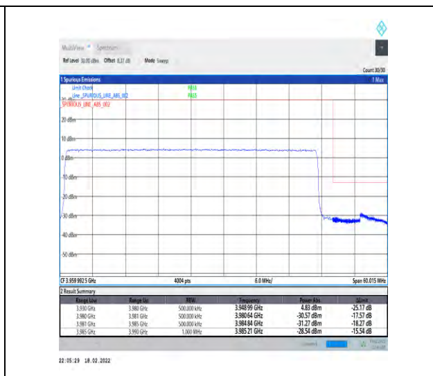
1-N77-3700-3980-30-50-H-3-DFT-PI2BPSK-Outer_Full-128@0-Ant4-PASS-see graph
