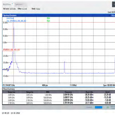
1-N77-3700-3980-30-100-L-1-DFT-PI2BPSK-Edge_1R_B_Left-1@0-Ant4-PASS-see graph
