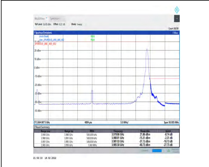
1-N77-3700-3980-30-40-H-5-CP-QPSK-Edge_1RB_Right-1@105-Ant4-PASS-see graph
