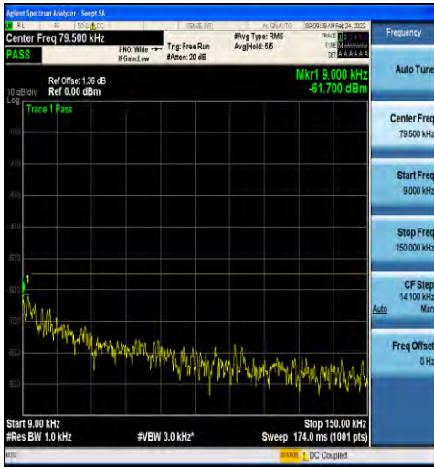
1-N38-30-40-H-1-DFT-PI2BPSK-Inner_1RB_Left-1 @1-0.009-0.15-Ant2--61.70--55-PASS
