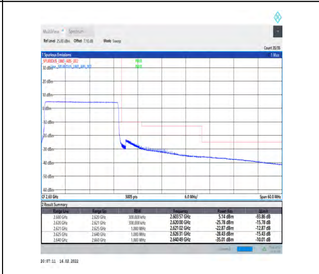
1-N38-30-20-H-6-CP-QPSK-Outer_Full-51@0-Ant2-PASS-see graph
