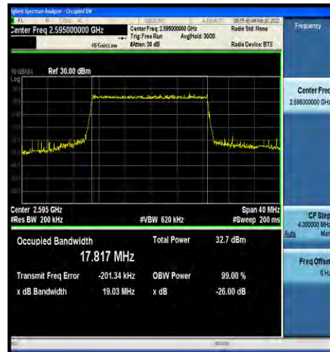
1-N38-30-20-M-1-DFT-QPSK-Outer_Full-50@0-Ant2 -17.817-19.03-≤20-PASS
