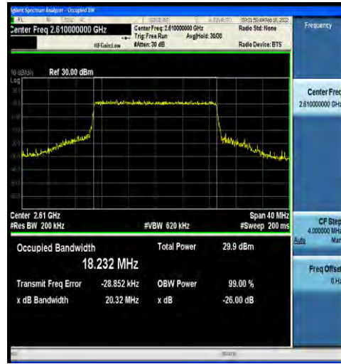
1-N38-30-20-H-8-CP-64QAM-Outer_Full-51@0-Ant2 -18.232-20.32-≤20-PASS
