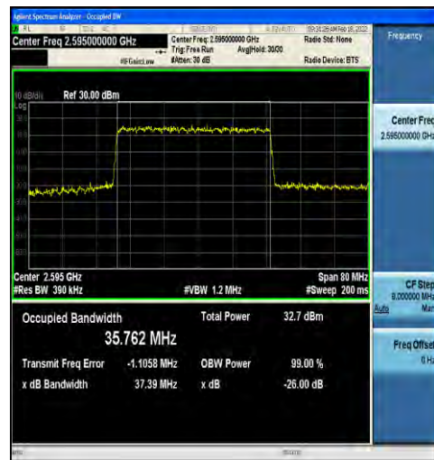
1-N38-30-40-M-1-DFT-QPSK-Outer_Full-100@0-Ant 2-35.762-37.39-≤40-PASS
