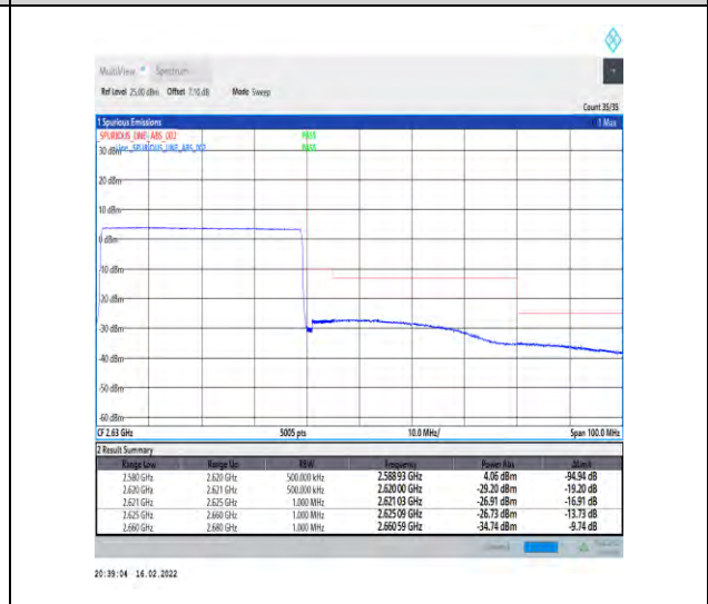
1-N38-30-40-H-6-CP-QPSK-Outer_Full-106@0-Ant2-PASS-see graph
