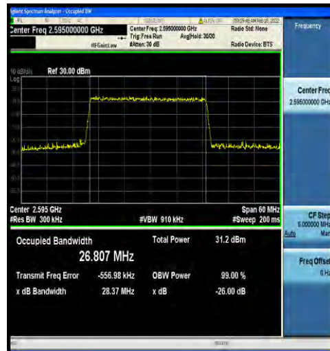
1-N38-30-30-M-4-DFT-64QAM-Outer_Full-75@0-Ant 2-26.807-28.37-≤30-PASS
