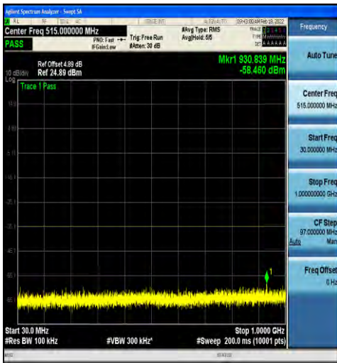
1-N38-30-40-H-1-DFT-PI2BPSK-Inner_1RB_Left-1 @1-30-1000-Ant2--58.46--35-PASS
