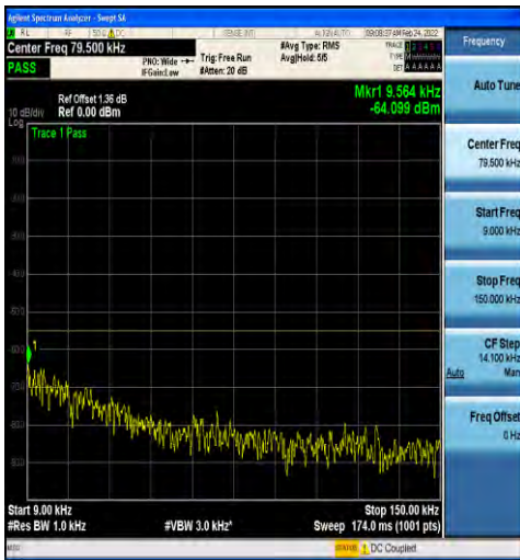
1-N38-30-40-M-1-DFT-PI2BPSK-Inner_1RB_Left-1 @1-0.009-0.15-Ant2--64.10--55-PASS
