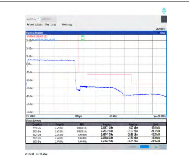
1-N38-30-30-H-3-DFT-PI2BPSK-Outer_Full-75@0-Ant2-PASS-see graph
