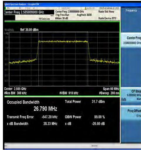
1-N38-30-30-L-3-DFT-16QAM-Outer_Full-75@0-Ant 2-26.790-28.33-≤30-PASS
