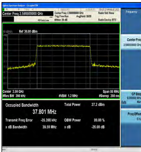
1-N38-30-40-L-9-CP-256QAM-Outer_Full-106@0-Ant t2-37.801-39.59-≤40-PASS
