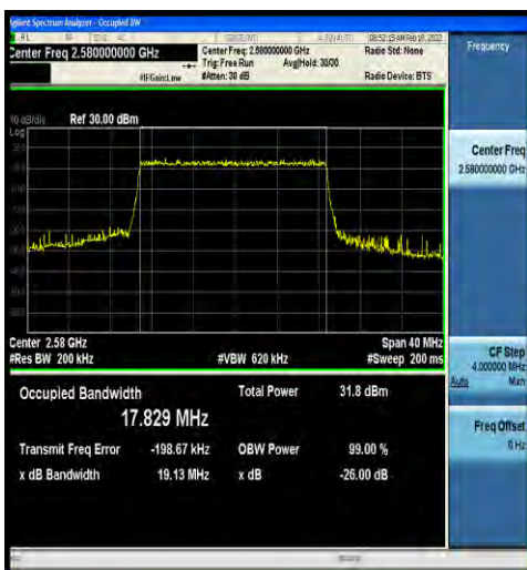
1-N38-30-20-L-3-DFT-16QAM-Outer_Full-50@0-Ant 2-17.829-19.13-≤20-PASS
