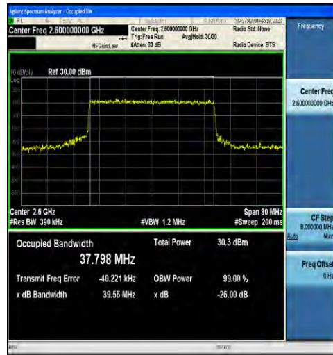
1-N38-30-40-H-8-CP-64QAM-Outer_Full-106@0-Ant 2-37.798-39.56-≤40-PASS
