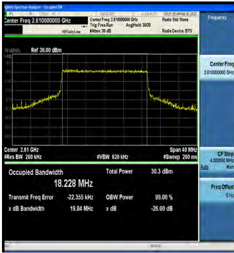
1-N38-30-20-H-7-CP-16QAM-Outer_Full-51@0-Ant2 -18.228-19.84-≤20-PASS
