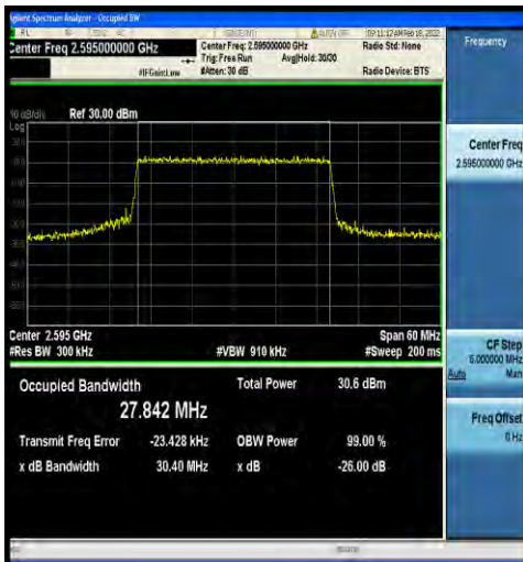
1-N38-30-30-M-7-CP-16QAM-Outer_Full-78@0-Ant2 -27.842-30.40-≤30-PASS
