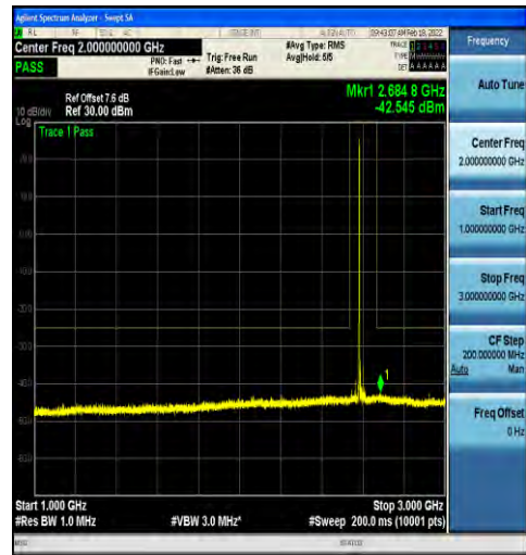
1-N38-30-40-H-1-DFT-PI2BPSK-Inner_1RB_Left-1@ 1-1000-3000-Ant2--42.55--25-PASS
