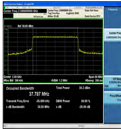
1-N38-30-40-L-8-CP-64QAM-Outer_Full-106@0-Ant 2-37.787-39.95-≤40-PASS
