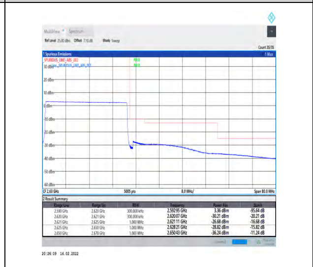
1-N38-30-30-H-6-CP-QPSK-Outer_Full-78@0-Ant2-PASS-see graph
