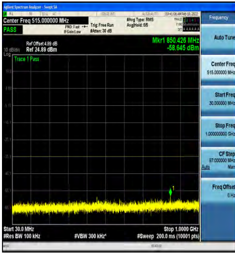
1-N38-30-40-M-1-DFT-PI2BPSK-Inner_1RB_Left-1 @1-30-1000-Ant2--58.65--35-PASS
