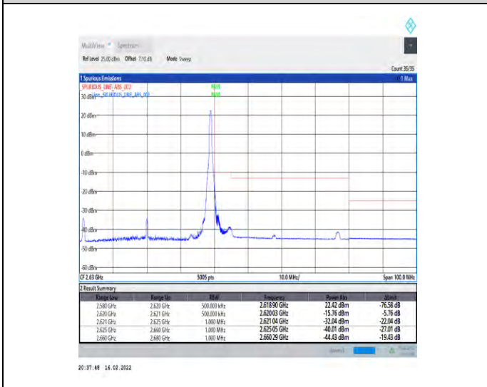
1-N38-30-40-H-5-CP-QPSK-Edge_1RB_Right-1@105-Ant2-PASS-see graph
