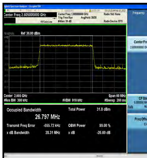
1-N38-30-30-H-3-DFT-16QAM-Outer_Full-75@0-Ant 2-26.797-28.31-≤30-PASS
