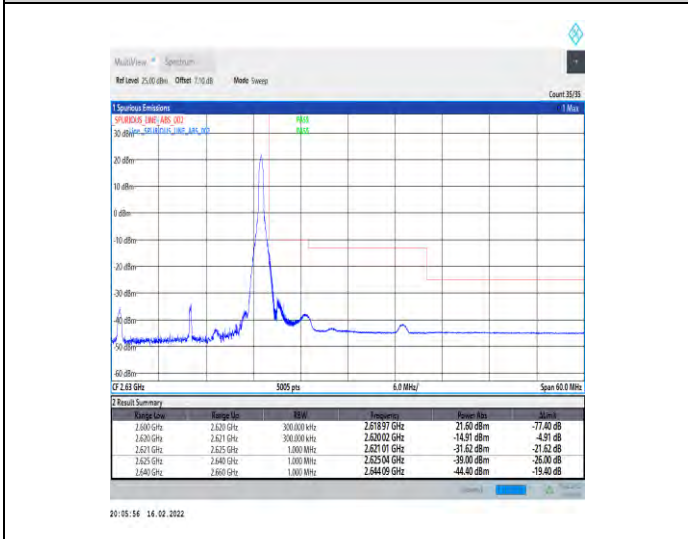
1-N38-30-20-H-5-CP-QPSK-Edge_1RB_Right-1@50-Ant2-PASS-see graph
