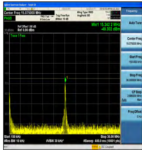
1-N38-30-40-M-1-DFT-PI2BPSK-Inner_1RB_Left-1@ 1-0.15-30-Ant2--49.30--45-PASS
