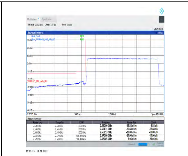
1-N38-30-40-L-3-DFT-PI2BPSK-Outer_Full-100@0-Ant2-PASS-see graph
