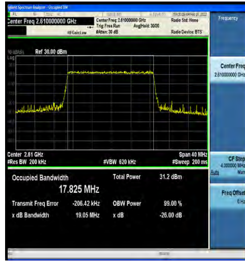
1-N38-30-20-H-4-DFT-64QAM-Outer_Full-50@0-Ant 2-17.825-19.05-≤20-PASS
