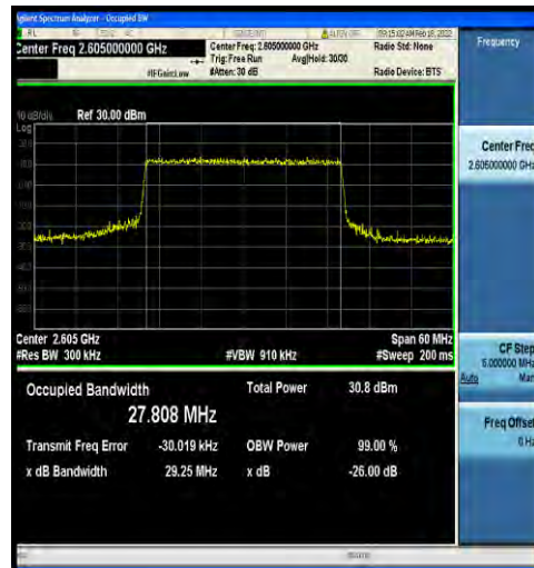
1-N38-30-30-H-7-CP-16QAM-Outer_Full-78@0-Ant2 -27.808-29.25-≤30-PASS
