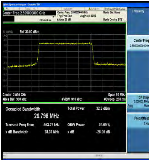
1-N38-30-30-M-1-DFT-QPSK-Outer_Full-75@0-Ant2 -26.798-28.37-≤30-PASS
