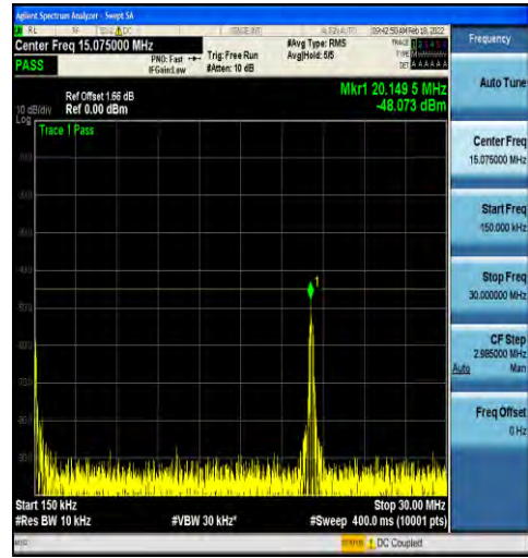
1-N38-30-40-H-1-DFT-PI2BPSK-Inner_1RB_Left-1@ 1-0.15-30-Ant2--48.07--45-PASS
