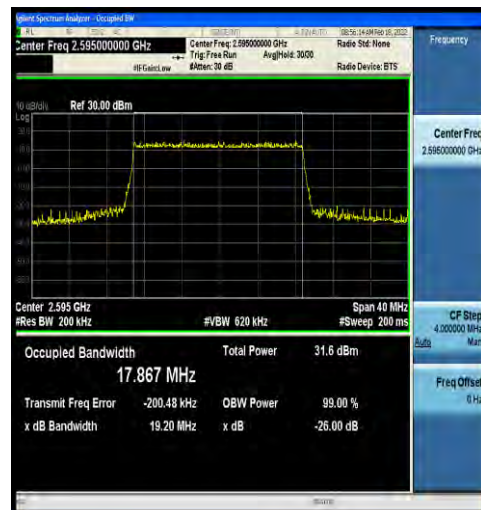
1-N38-30-20-M-3-DFT-16QAM-Outer_Full-50@0-Ant 2-17.867-19.20-≤20-PASS
