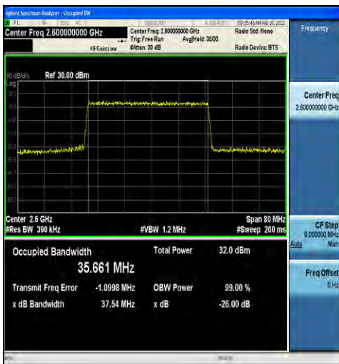
1-N38-30-40-H-3-DFT-16QAM-Outer_Full-100@0-Ant nt2-35.661-37.54-≤40-PASS
