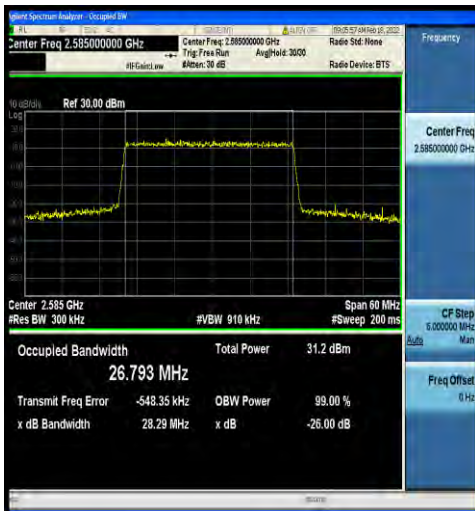
1-N38-30-30-L-4-DFT-64QAM-Outer_Full-75@0-Ant 2-26.793-28.29-≤30-PASS
