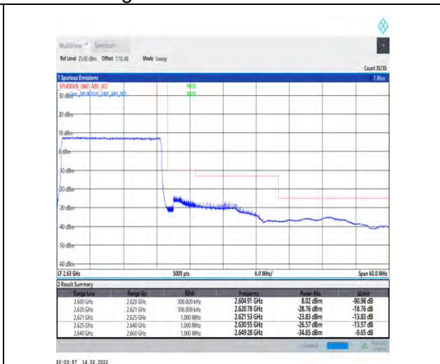
1-N38-30-20-H-3-DFT-PI2BPSK-Outer_Full-50@0-Ant2-PASS-see graph
