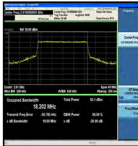
1-N38-30-20-H-6-CP-QPSK-Outer_Full-51@0-Ant 2-18.202-19.60-≤20-PASS
