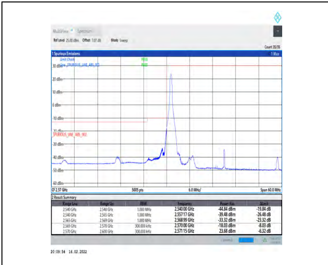
1-N38-30-30-L-1-DFT-PI2BPSK-Edge_1RB_Left-1@0-Ant2-PASS-see graph
