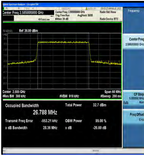
1-N38-30-30-L-2-DFT-PI2BPSK-Outer_Full-75@0-A nt2-26.788-28.36-≤30-PASS
