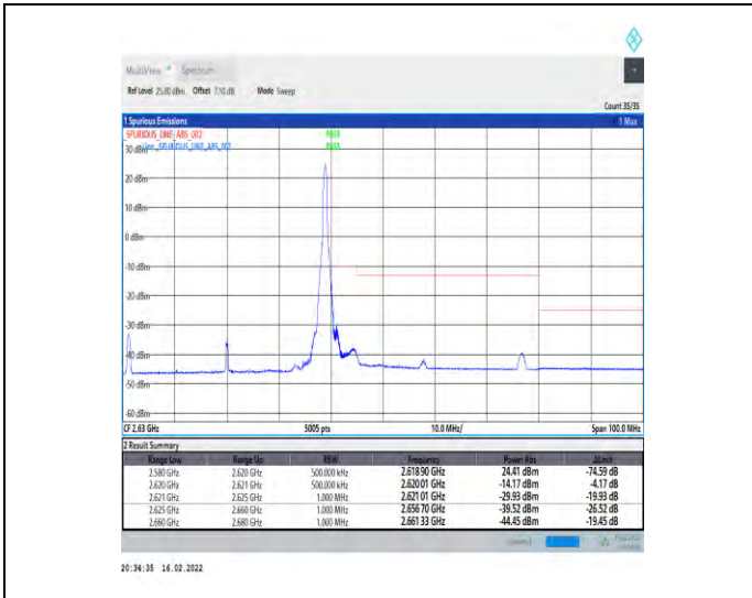
1-N38-30-40-H-2-DFT-PI2BPSK-Edge_1RB_Right-1@105-Ant2-PASS-see graph
