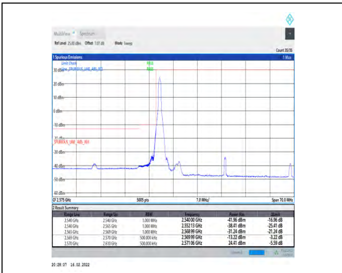
1-N38-30-40-L-1-DFT-PI2BPSK-Edge_1RB_Left-1@0-Ant2-PASS-see graph
