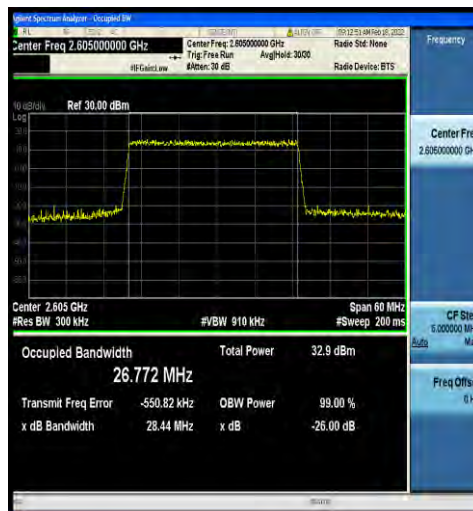
1-N38-30-30-H-1-DFT-QPSK-Outer_Full-75@0-Ant2 -26.772-28.44-≤30-PASS
