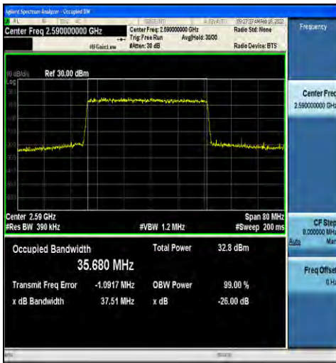
1-N38-30-40-L-1-DFT-QPSK-Outer_Full-100@0-Ant 2-35.680-37.51-≤40-PASS
