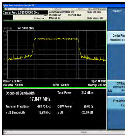
1-N38-30-20-L-4-DFT-64QAM-Outer_Full-50@0-Ant 2-17.847-18.98-≤20-PASS
