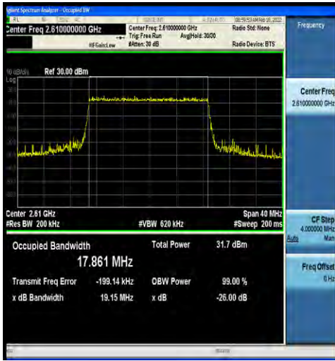
1-N38-30-20-H-3-DFT-16QAM-Outer_Full-50@0-Ant 2-17.861-19.15-≤20-PASS
