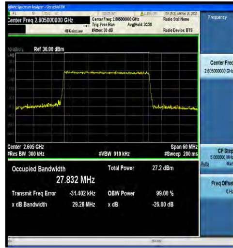
1-N38-30-30-H-9-CP-256QAM-Outer_Full-78@0-Ant 2-27.832-29.28-≤30-PASS
