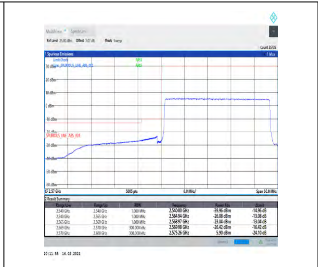
1-N38-30-30-L-3-DFT-PI2BPSK-Outer_Full-75@0-Ant2-PASS-see graph
