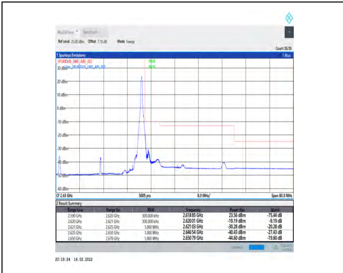
1-N38-30-30-H-2-DFT-PI2BPSK-Edge_1RB_Right-1@77-Ant2-PASS-see graph
