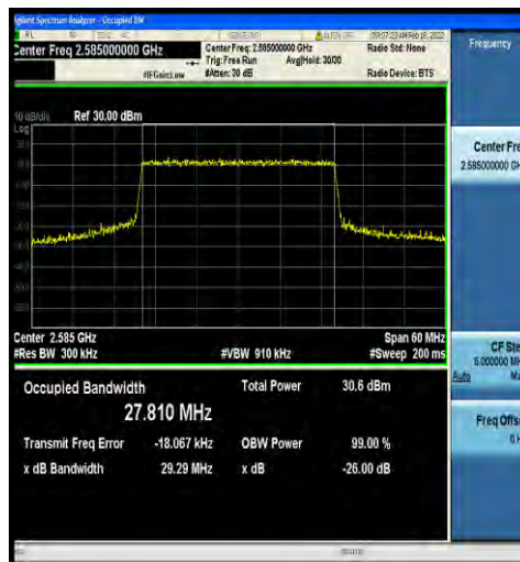
1-N38-30-30-L-7-CP-16QAM-Outer_Full-78@0-Ant2 -27.810-29.29-≤30-PASS
