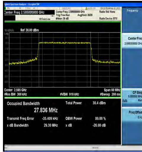
1-N38-30-30-M-6-CP-QPSK-Outer_Full-78@0-Ant2- 27.836-29.30-≤30-PASS
