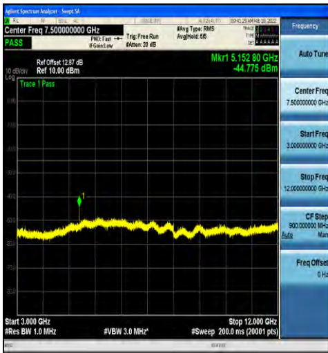
1-N38-30-40-M-1-DFT-PI2BPSK-Inner_1RB_Left-1 @1-3000-12000-Ant2--44.77--25-PASS
