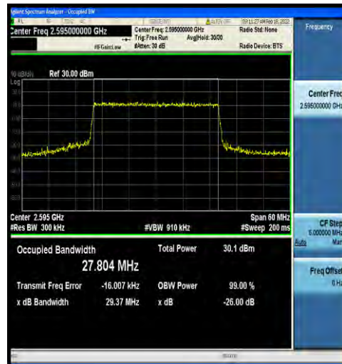
1-N38-30-30-M-8-CP-64QAM-Outer_Full-78@0-Ant 2-27.804-29.37-≤30-PASS
