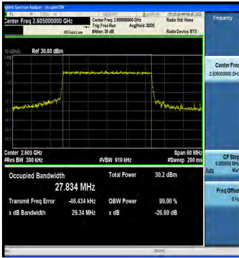
1-N38-30-30-H-8-CP-64QAM-Outer_Full-78@0-Ant2 -27.834-29.34-≤30-PASS
