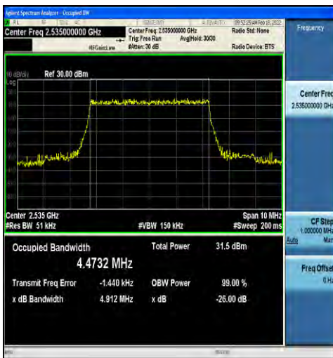
1-N7-15-5-M-2-DFT-PI2BPSK-Outer_Full-25@0-Ant 2-4.4732-4.912-≤5-PASS
