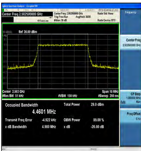
1-N7-15-5-L-7-CP-16QAM-Outer_Full-25@0-Ant2-4.4601-4.900-≤5-PASS
