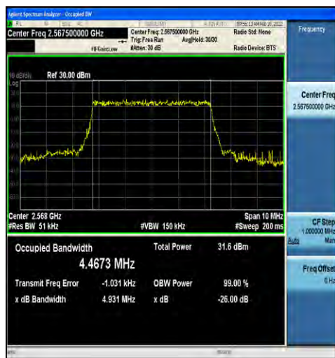
1-N7-15-5-H-2-DFT-PI2BPSK-Outer_Full-25@0-Ant2-4 2-4.4673-4.931-≤5-PASS
