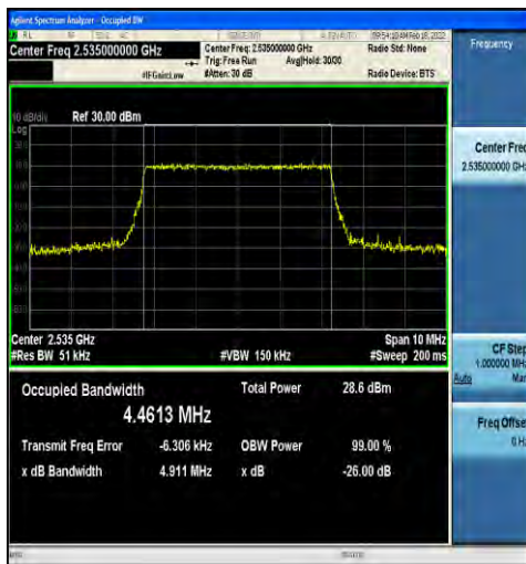
1-N7-15-5-M-6-CP-QPSK-Outer_Full-25@0-Ant2-4.4613-4.911-≤5-PASS
