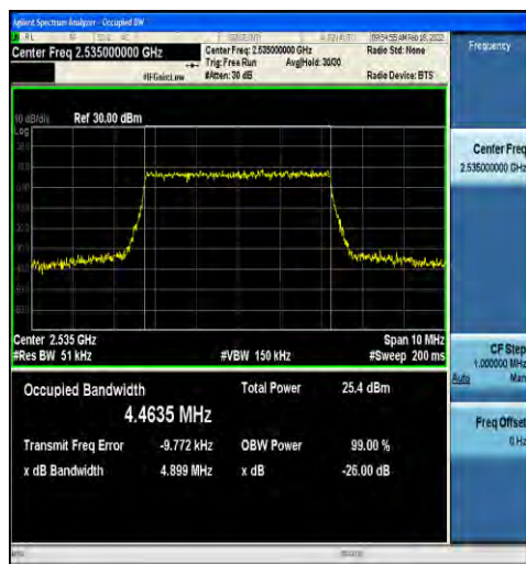
1-N7-15-5-M-9-CP-256QAM-Outer_Full-25@0-Ant2-4 4.4635-4.899-≤5-PASS
