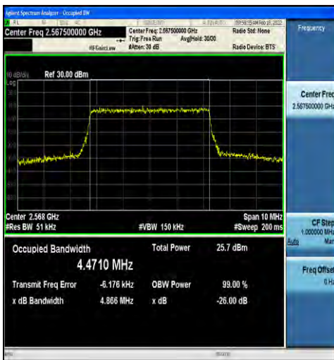
1-N7-15-5-H-9-CP-256QAM-Outer_Full-25@0-Ant2- 4.4710-4.866-≤5-PASS
