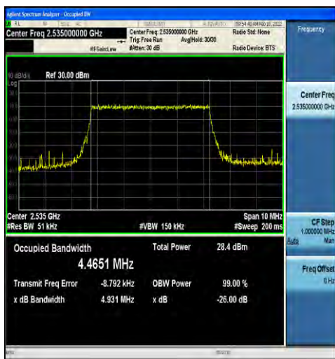
1-N7-15-5-M-8-CP-64QAM-Outer_Full-25@0-Ant2-4 .4651-4.931-≤5-PASS
