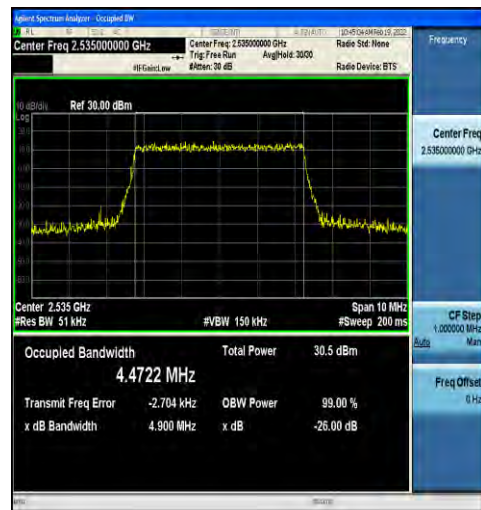
1-N7-15-5-M-3-DFT-16QAM-Outer_Full-25@0-Ant2- 4.4722-4.900-≤5-PASS
