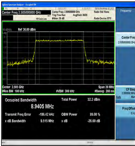
1-N7-15-10-L-2-DFT-PI2BPSK-Outer_Full-50@0-Ant 2-8.9405-9.515-≤10-PASS
