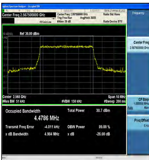
1-N7-15-5-H-3-DFT-16QAM-Outer_Full-25@0-Ant2- 4.4786-4.904-≤5-PASS
