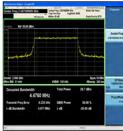
1-N7-15-5-H-8-CP-64QAM-Outer_Full-25@0-Ant2-4. 4760-4.871-≤5-PASS
