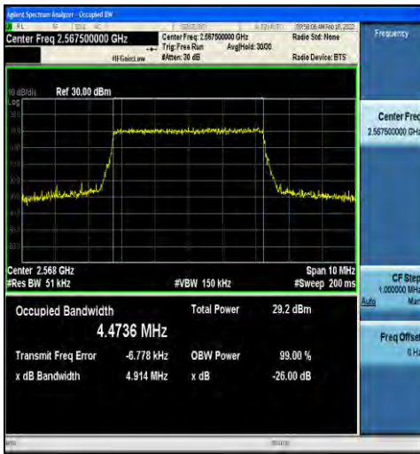
1-N7-15-5-H-7-CP-16QAM-Outer_Full-25@0-Ant2-4. 4736-4.914-≤5-PASS
