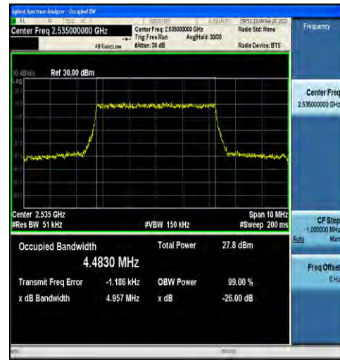
1-N7-15-5-M-5-DFT-256QAM-Outer_Full-25@0-Ant2-4.4830-4.957-≤5-PASS
