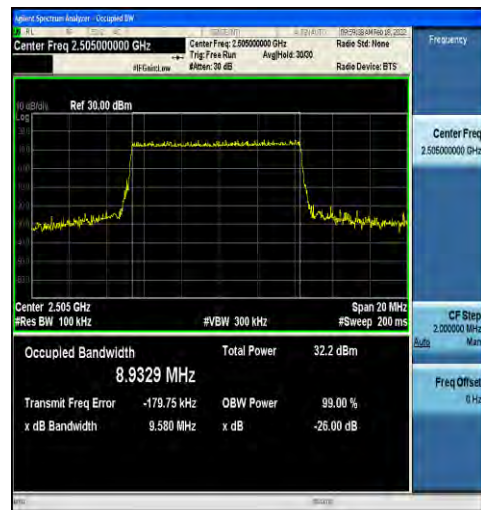
1-N7-15-10-L-1-DFT-QPSK-Outer_Full-50@0-Ant2-8 .9329-9.580-≤10-PASS
