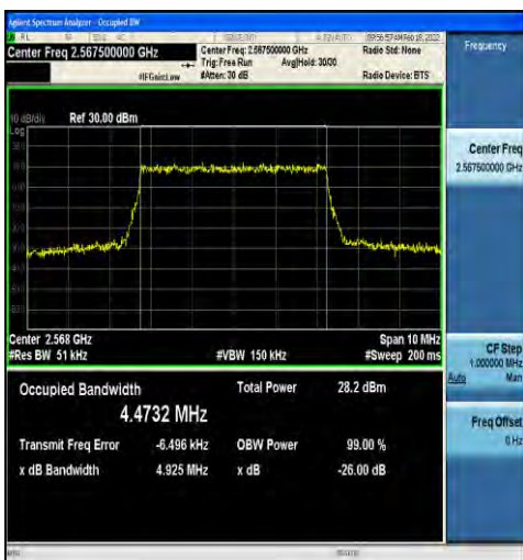
1-N7-15-5-H-5-DFT-256QAM-Outer_Full-25@0-Ant2 -4.4732-4.925-≤5-PASS
