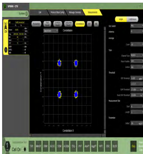
1-N7-15-40-M-6-CP-QPSK-Outer_Full-216@0-Ant2 -see graph-PASS
