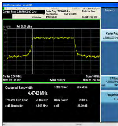
1-N7-15-5-L-8-CP-64QAM-Outer_Full-25@0-Ant2-4.4742-4.867-≤5-PASS
