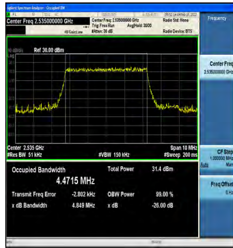
1-N7-15-5-M-1-DFT-QPSK-Outer_Full-25@0-Ant2-4. 4.715-4.849-≤5-PASS
