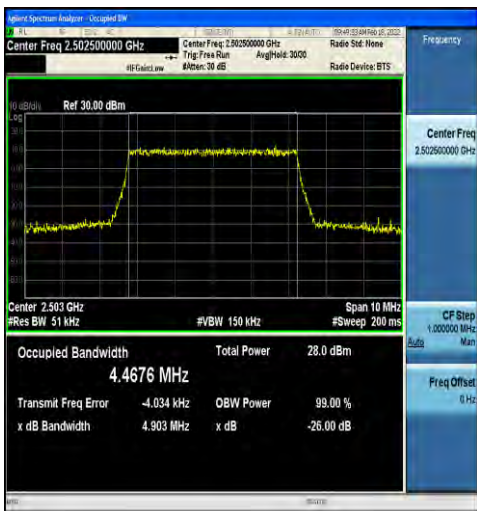
1-N7-15-5-L-5-DFT-256QAM-Outer_Full-25@0-Ant2-4.4676-4.903-≤5-PASS
