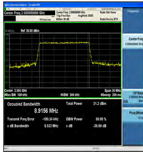
1-N7-15-10-L-3-DFT-16QAM-Outer_Full-50@0-Ant2- 8.9156-9.532-≤10-PASS
