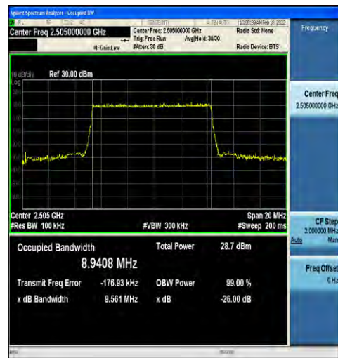
1-N7-15-10-L-5-DFT-256QAM-Outer_Full-50@0-Ant 2-8.9408-9.561-≤10-PASS
