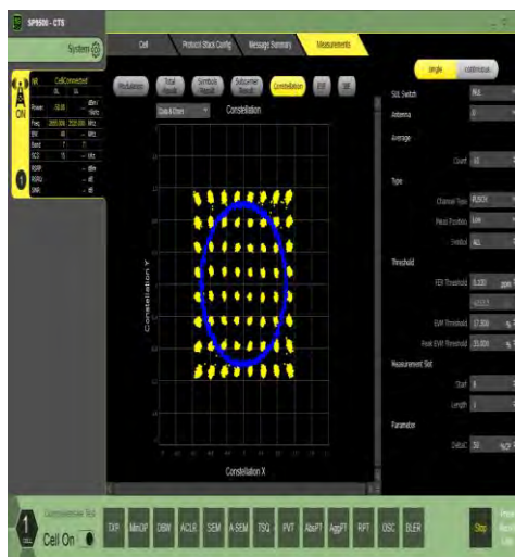
1-N7-15-40-M-4-DFT-64QAM-Outer_Full-216@0-An t2-see graph-PASS
