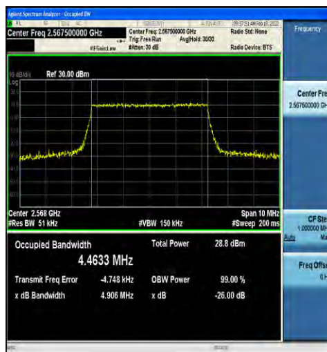
1-N7-15-5-H-6-CP-QPSK-Outer_Full-25@0-Ant2-4.4 633-4.906-≤5-PASS
