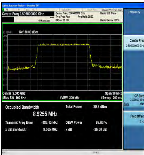
1-N7-15-10-L-4-DFT-64QAM-Outer_Full-50@0-Ant2- 8.9255-9.565-≤10-PASS
