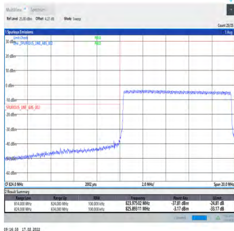
1-N5-15-10-L-6-CP-QPSK-Outer_Full-52@0-Ant0-seegraph-PASS-see graph
