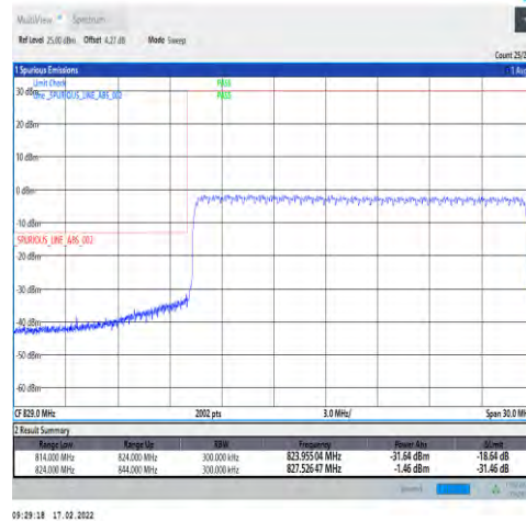
1-N5-15-20-L-6-CP-QPSK-Outer_Full-106@0-Ant0-seegraph-PASS-see graph
