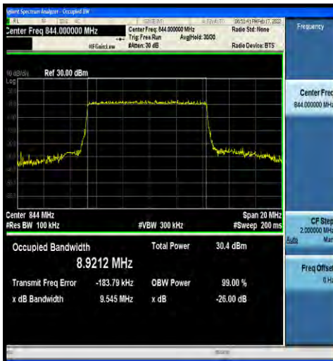
1-N5-15-10-H-4-DFT-64QAM-Outer_Full-50@0-Ant0 -8.9212-9.545-≤10-PASS
