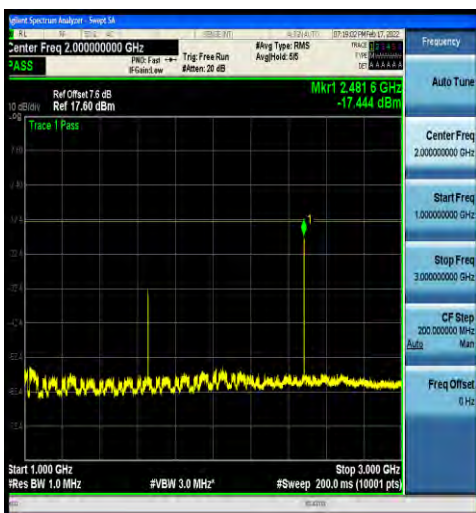
1-N5-15-20-M-1-DFT-PI2BPSK-Inner_1RB_Left-1@ 1-1000-3000-ANT0--17.44--13-PASS
