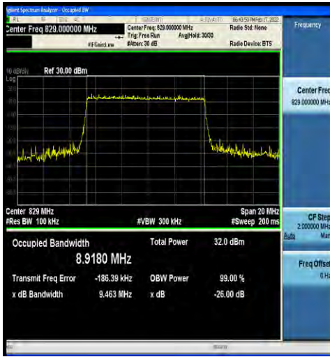
1-N5-15-10-L-2-DFT-PI2BPSK-Outer_Full-50@0-Ant 0-8.9180-9.463-≤10-PASS
