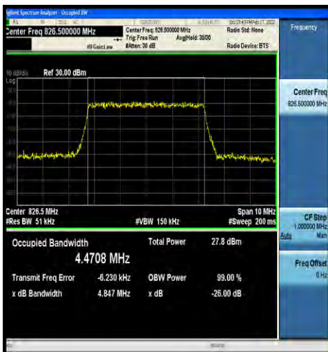
1-N5-15-5-L-5-DFT-256QAM-Outer_Full-25@0-Ant0 -4.4708-4.847-≤5-PASS
