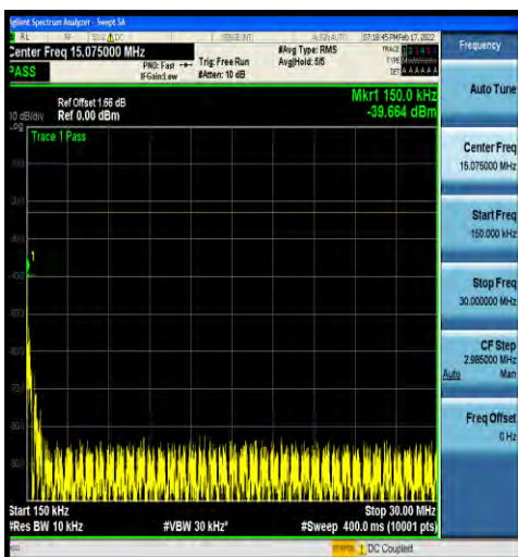
1-N5-15-20-M-1-DFT-PI2BPSK-Inner_1RB_Left-1@ 1-0.15-30-ANT0--39.66--23-PASS
