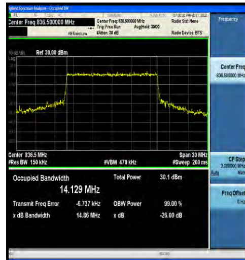
1-N5-15-15-M-7-CP-16QAM-Outer_Full-79@0-Ant0- 14.129-14.86-≤15-PASS
