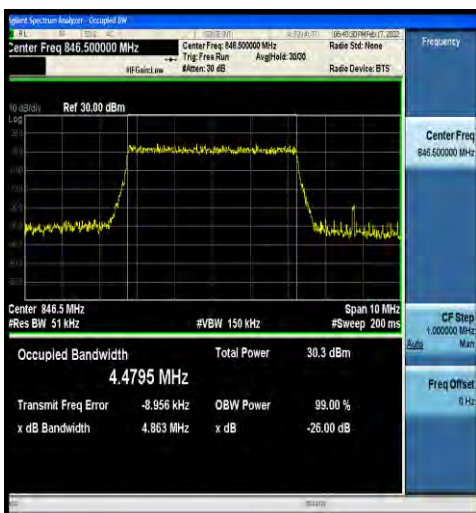
1-N5-15-5-H-3-DFT-16QAM-Outer_Full-25@0-Ant0-4.4795-4.863-≤5-PASS
