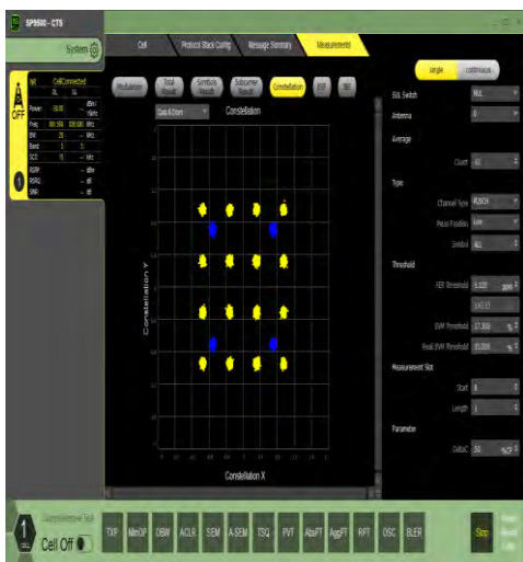
1-N5-15-20-M-7-CP-16QAM-Outer_Full-106@0-Ant0-see graph-PASS
