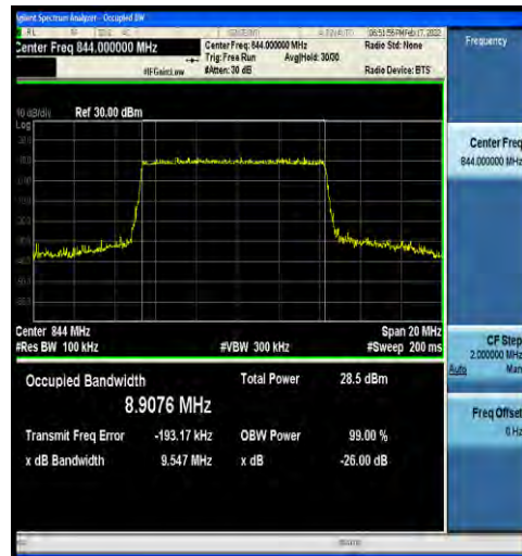
1-N5-15-10-H-5-DFT-256QAM-Outer_Full-50@0-Ant0 0-8.9076-9.547-≤10-PASS
