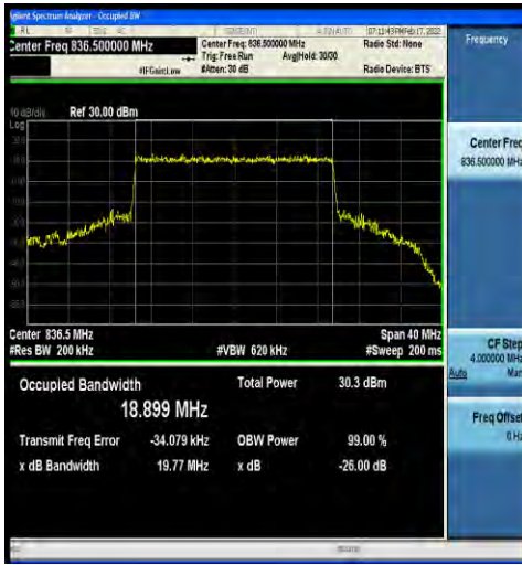
1-N5-15-20-M-7-CP-16QAM-Outer_Full-106@0-Ant0-18.899-19.77-≤20-PASS
