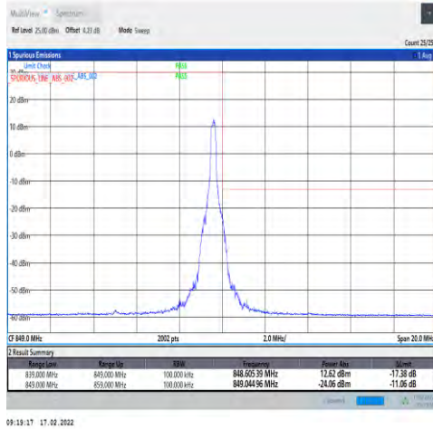
1-N5-15-10-H-5-CP-QPSK-Edge_1RB_Right-1@51-Ant0-seegraph-PASS-see graph
