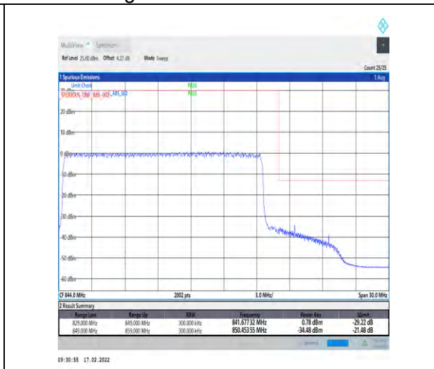
1-N5-15-20-H-3-DFT-PI2BPSK-Outer_Full-100@0-Ant0-seegraph-PASS-see graph
