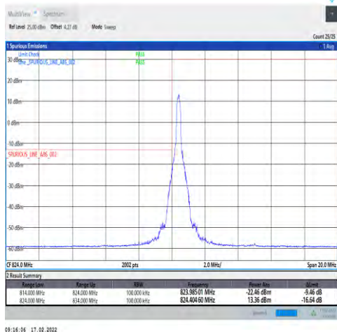
1-N5-15-10-L-4-CP-QPSK-Edge_1RB_Left-1@0-Ant0-seegraph-PASS-see graph
