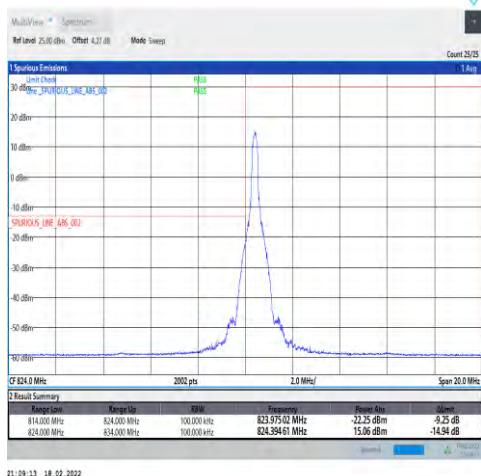
1-N5-15-10-L-1-DFT-PI2BPSK-Edge_1RB_Left-1@0-A nt0-seegraph-PASS-see graph
