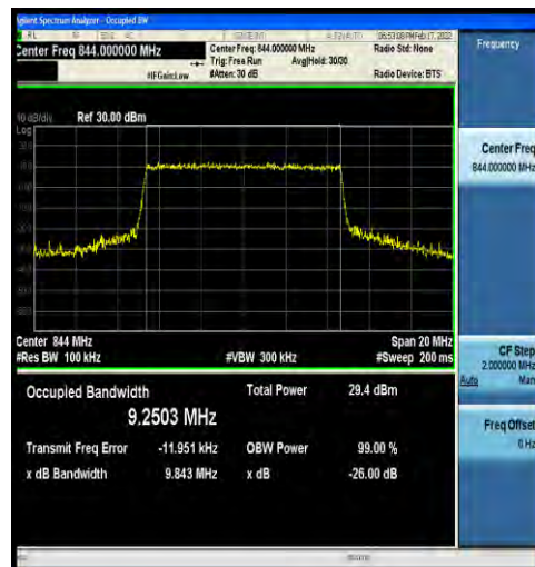
1-N5-15-10-H-7-CP-16QAM-Outer_Full-52@0-Ant0-9 9.2503-9.843-≤10-PASS
