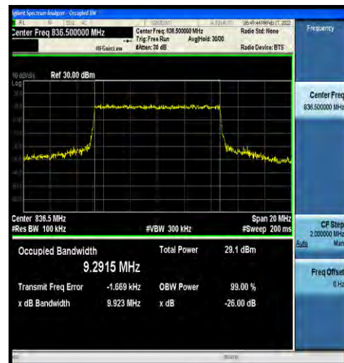
1-N5-15-10-M-8-CP-64QAM-Outer_Full-52@0-Ant0- 9.2915-9.923-≤10-PASS
