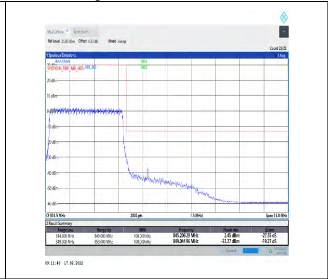
1-N5-15-5-H-3-DFT-PI2BPSK-Outer_Full-25@0-Ant0-seegraph-PASS-see graph
