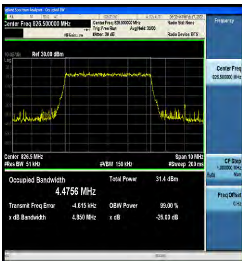
1-N5-15-5-L-1-DFT-QPSK-Outer_Full-25@0-Ant0-4. 4756-4.850-≤5-PASS
