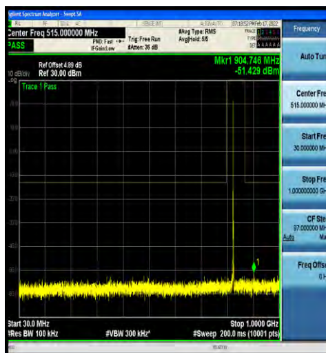
1-N5-15-20-M-1-DFT-PI2BPSK-Inner_1RB_Left-1@ 1-30-1000-ANT0--51.43--13-PASS
