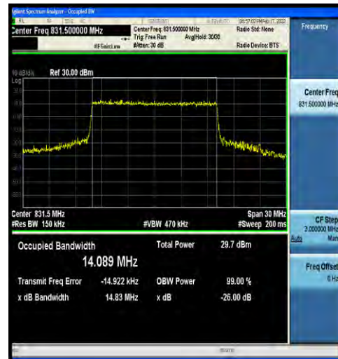
1-N5-15-15-L-8-CP-64QAM-Outer_Full-79@0-Ant0-14.089-14.83-≤15-PASS
