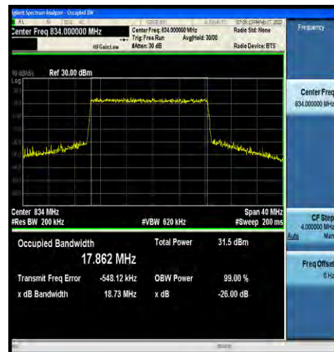
1-N5-15-20-L-3-DFT-16QAM-Outer_Full-100@0-Ant0 17.862-18.73≤20-PASS
