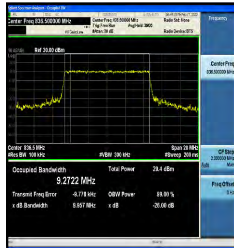
1-N5-15-10-M-6-CP-QPSK-Outer_Full-52@0-Ant0-9. 2722-9.957-≤10-PASS
