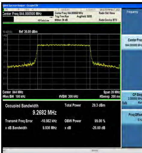
1-N5-15-10-H-6-CP-QPSK-Outer_Full-52@0-Ant0-9. 2682-9.936-≤10-PASS
