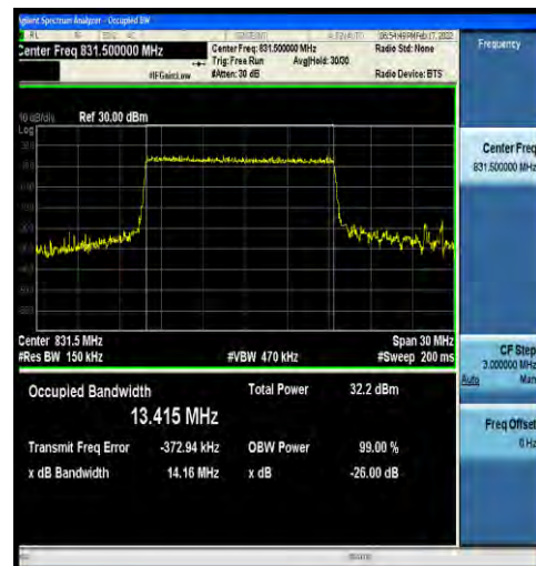
1-N5-15-15-L-2-DFT-PI2BPSK-Outer_Full-75@0-Ant0-13.415-14.16-≤15-PASS
