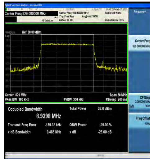
1-N5-15-10-L-1-DFT-QPSK-Outer_Full-50@0-Ant0-8 .9298-9.485-≤10-PASS
