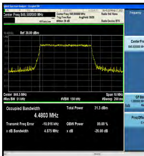
1-N5-15-5-H-2-DFT-PI2BPSK-Outer_Full-25@0-Ant0 -4.4803-4.875-≤5-PASS
