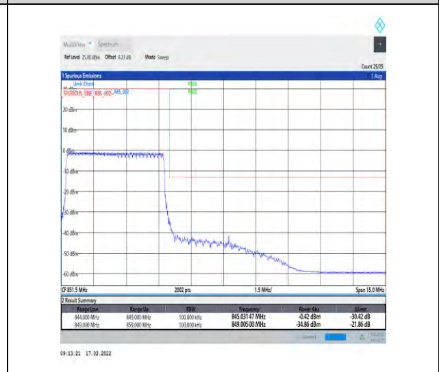
1-N5-15-5-H-6-CP-QPSK-Outer_Full-25@0-Ant0-seegraph-PASS-see graph
