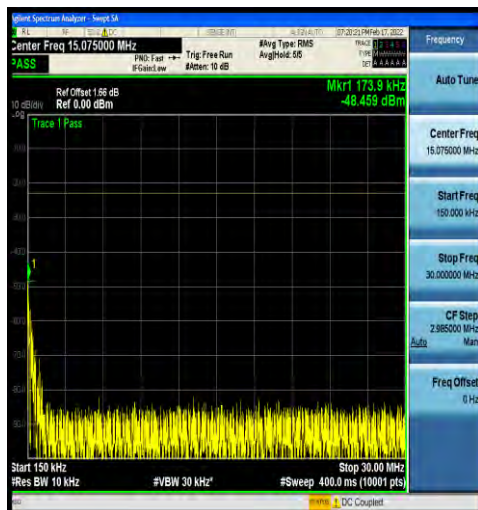
1-N5-15-20-H-1-DFT-PI2BPSK-Inner_1RB_Left-1@1 -0.15-30-ANT0--48.46--23-PASS
