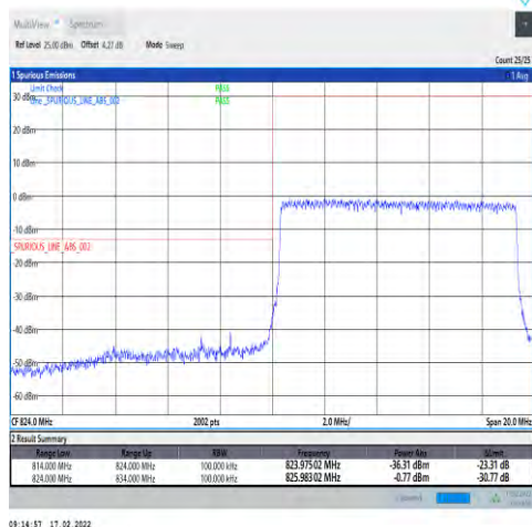
1-N5-15-10-L-3-DFT-PI2BPSK-Outer_Full-50@0-Ant0-seegraph-PASS-see graph
