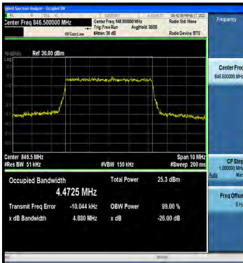
1-N5-15-5-H-9-CP-256QAM-Outer_Full-25@0-Ant0- 4.4725-4.880-≤5-PASS
