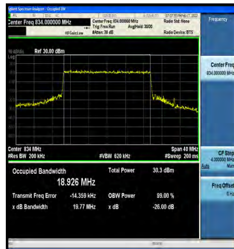
1-N5-15-20-L-7-CP-16QAM-Outer_Full-106@0-Ant0 18.926-19.77-≤20-PASS
