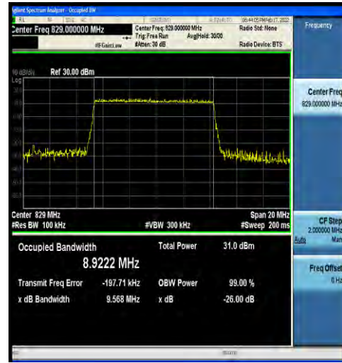
1-N5-15-10-L-3-DFT-16QAM-Outer_Full-50@0-Ant0- 8.9222-9.568-≤10-PASS
