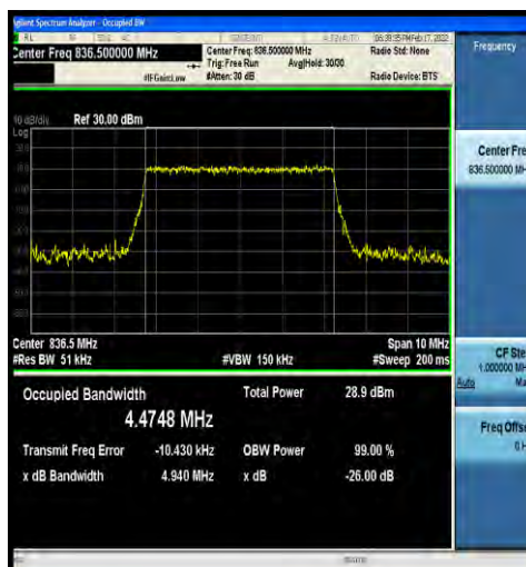
1-N5-15-5-M-7-CP-16QAM-Outer_Full-25@0-Ant0-4.4748-4.940-≤5-PASS
