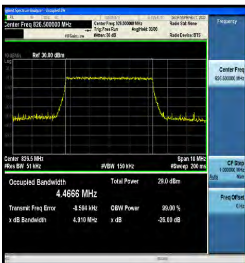
1-N5-15-5-L-7-CP-16QAM-Outer_Full-25@0-Ant0-4. 4666-4.910-≤5-PASS
