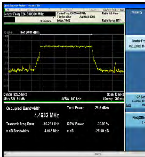
1-N5-15-5-L-6-CP-QPSK-Outer_Full-25@0-Ant0-4.4 632-4.945-≤5-PASS
