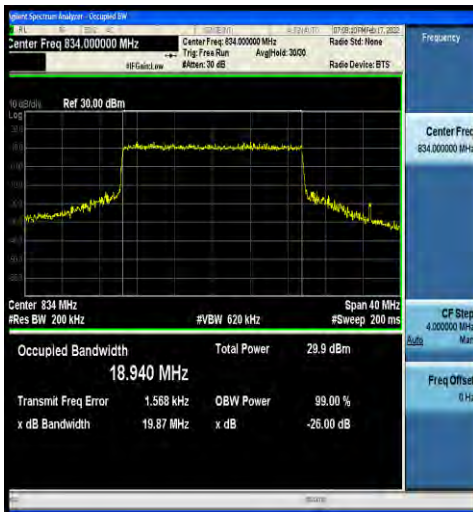
1-N5-15-20-L-8-CP-64QAM-Outer_Full-106@0-Ant0 -18.940-19.87-≤20-PASS
