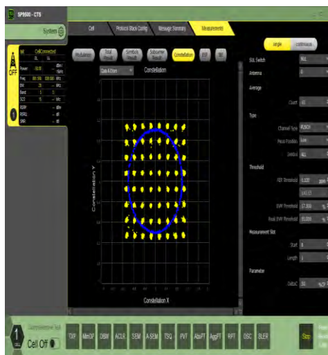
1-N5-15-20-M-4-DFT-64QAM-Outer_Full-100@0-An t0-see graph-PASS
