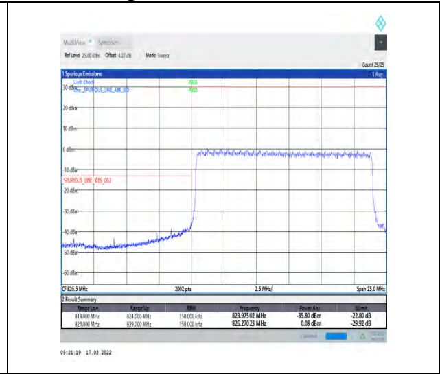
1-N5-15-15-L-3-DFT-PI2BPSK-Outer_Full-75@0-Ant0-seegraph-PASS-see graph
