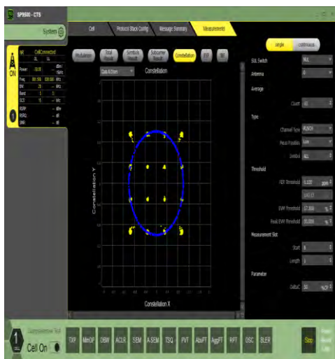
1-N5-15-20-M-3-DFT-16QAM-Outer_Full-100@0-Ant 0-see graph-PASS
