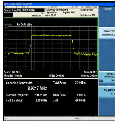
1-N5-15-10-L-5-DFT-256QAM-Outer_Full-50@0-Ant 0-8.9217-9.469-≤10-PASS
