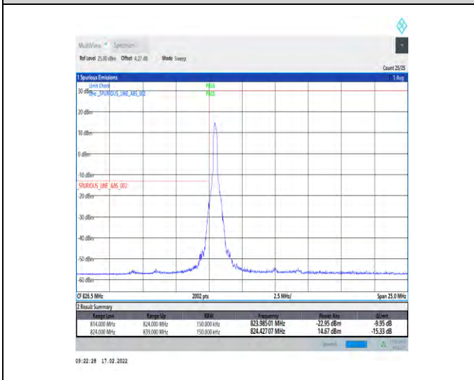
1-N5-15-15-L-4-CP-QPSK-Edge_1RB_Left-1@0-Ant0-seegraph-PASS-see graph
