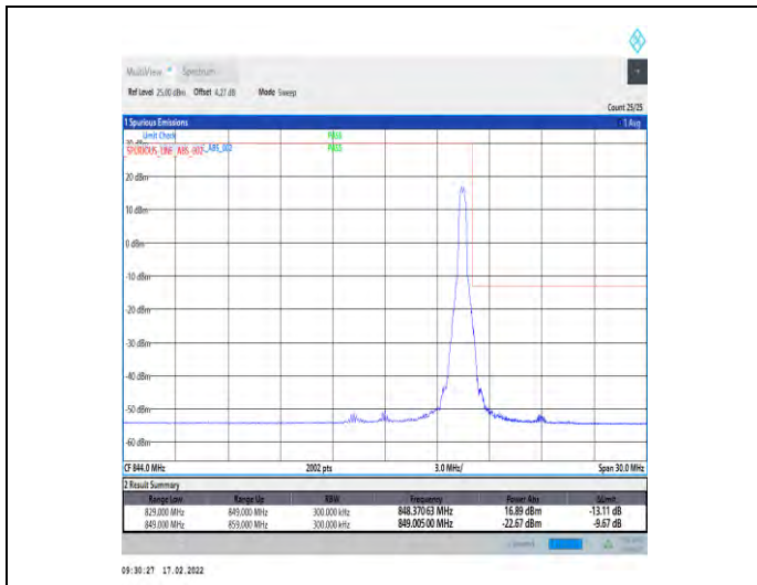
1-N5-15-20-H-2-DFT-PI2BPSK-Edge_1RB_Right-1@105-Ant0-seegraph-PASS-see graph
