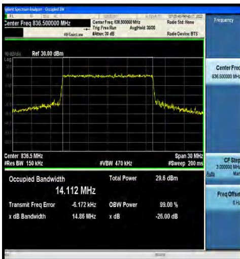
1-N5-15-15-M-8-CP-64QAM-Outer_Full-79@0-Ant0- 14.112-14.86-≤15-PASS
