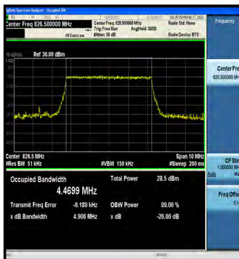
1-N5-15-5-L-8-CP-64QAM-Outer_Full-25@0-Ant0-4. 4699-4.906-≤5-PASS
