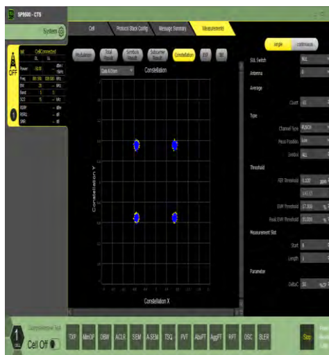
1-N5-15-20-M-6-CP-QPSK-Outer_Full-106@0-Ant0 -see graph-PASS
