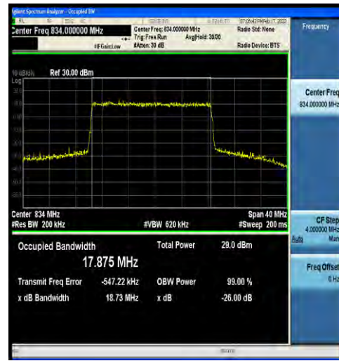
1-N5-15-20-L-5-DFT-256QAM-Outer_Full-100@0-An t0-17.875-18.73-≤20-PASS
