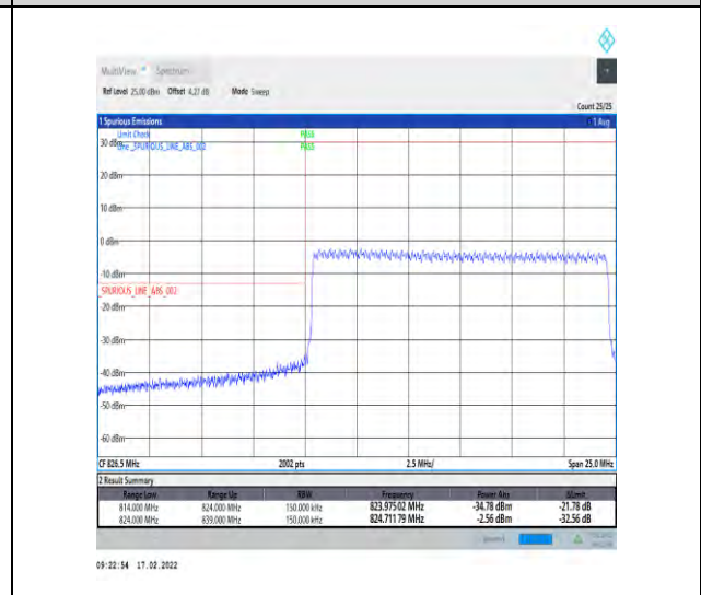
1-N5-15-15-L-6-CP-QPSK-Outer_Full-79@0-Ant0-seegraph-PASS-see graph
