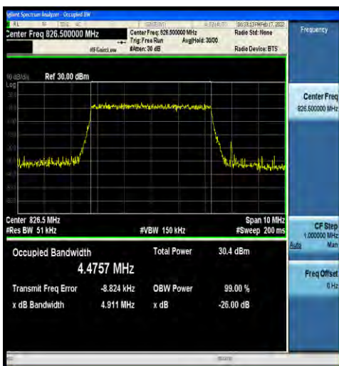
1-N5-15-5-L-3-DFT-16QAM-Outer_Full-25@0-Ant0- 4.4757-4.911-≤5-PASS
