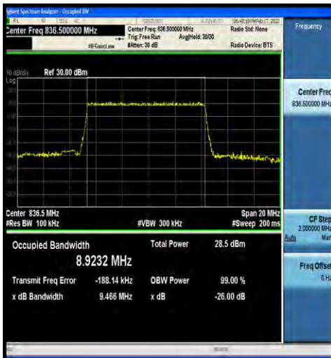
1-N5-15-10-M-5-DFT-256QAM-Outer_Full-50@0-Ant 0-8.9232-9.466-≤10-PASS
