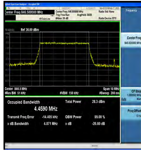
1-N5-15-5-H-8-CP-64QAM-Outer_Full-25@0-Ant0-4. 4590-4.871-≤5-PASS
