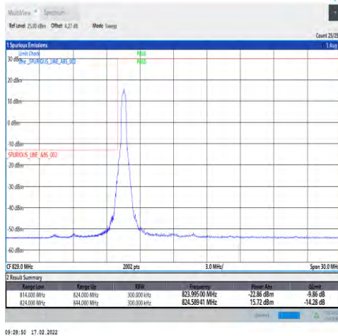
1-N5-15-20-L-4-CP-QPSK-Edge_1RB_Left-1@0-Ant0-seegraph-PASS-see graph
