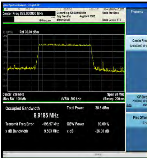
1-N5-15-10-L-4-DFT-64QAM-Outer_Full-50@0-Ant0 -8.9185-9.503-≤10-PASS
