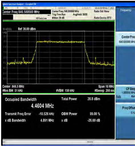
1-N5-15-5-H-7-CP-16QAM-Outer_Full-25@0-Ant0-4. 4604-4.891-≤5-PASS
