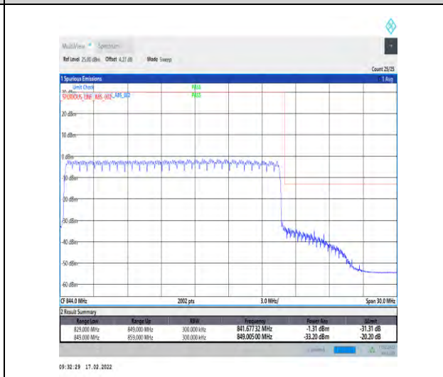
1-N5-15-20-H-6-CP-QPSK-Outer_Full-106@0-Ant0-seegraph-PASS-see graph
