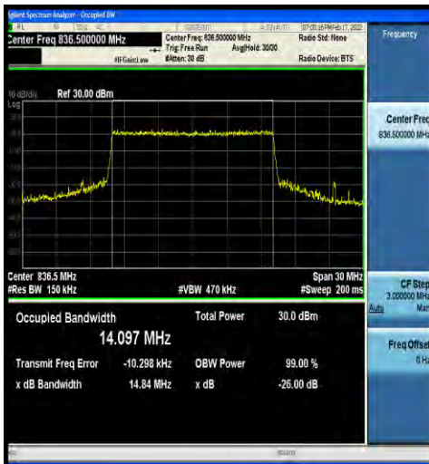
1-N5-15-15-M-6-CP-QPSK-Outer_Full-79@0-Ant0-1 4.097-14.84-≤15-PASS
