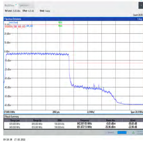
1-N5-15-10-H-3-DFT-PI2BPSK-Outer_Full-50@0-Ant0-seegraph-PASS-see graph
