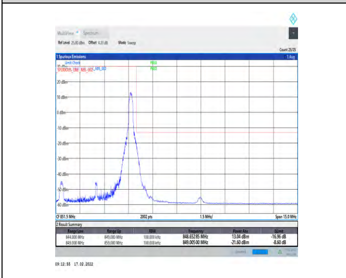
1-N5-15-5-H-5-CP-QPSK-Edge_1RB_Right-1@24-Ant0-seegraph-PASS-see graph
