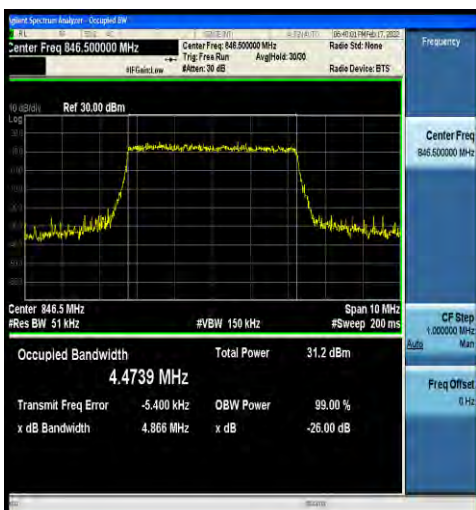
1-N5-15-5-H-1-DFT-QPSK-Outer_Full-25@0-Ant0-4. 4739-4.866-≤5-PASS
