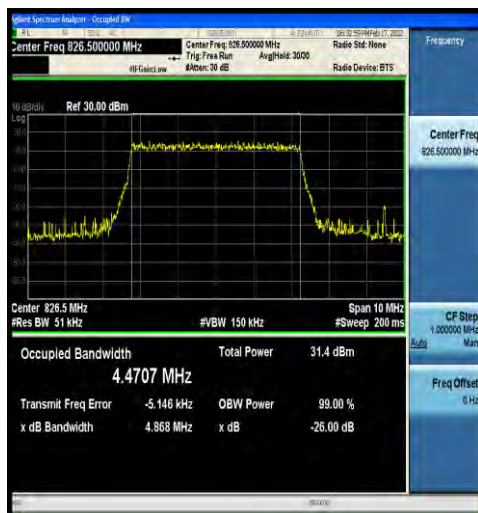
1-N5-15-5-L-2-DFT-P12BPSK-Outer_Full-25@0-Ant0 -4.4707-4.868-≤5-PASS
