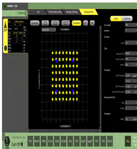
1-N5-15-20-M-8-CP-64QAM-Outer_Full-106@0-Ant 0-see graph-PASS
