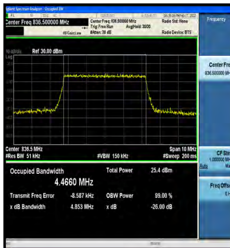
1-N5-15-5-M-9-CP-256QAM-Outer_Full-25@0-Ant0-4 4.4660-4.853-≤5-PASS
