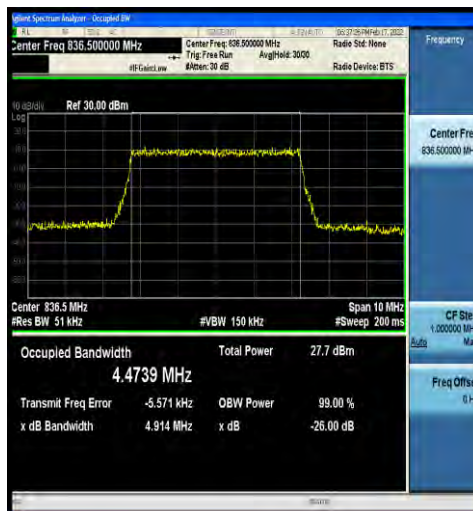
1-N5-15-5-M-5-DFT-256QAM-Outer_Full-25@0-Ant0-4.4739-4.914-≤5-PASS
