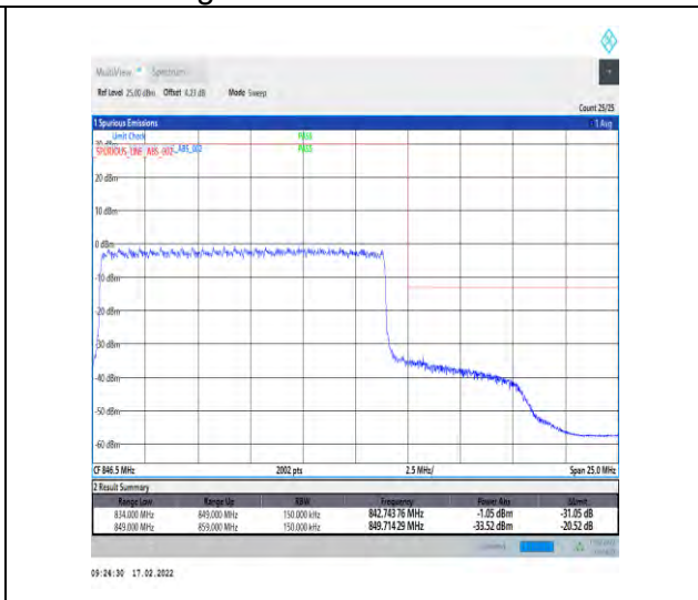
1-N5-15-15-H-3-DFT-PI2BPSK-Outer_Full-75@0- Ant0-seegraph-PASS-see graph
