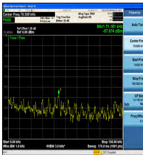
1-N5-15-20-M-1-DFT-PI2BPSK-Inner_1RB_Left-1@ 1-0.009-0.15-ANT0--57.67--33-PASS
