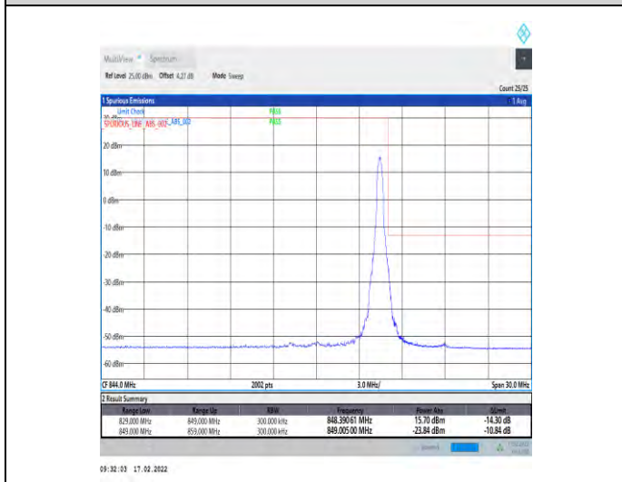
1-N5-15-20-H-5-CP-QPSK-Edge_1RB_Right-1@105-Ant0-seegraph-PASS-see graph
