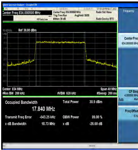
1-N5-15-20-L-4-DFT-64QAM-Outer_Full-100@0-Ant 0-17.840-18.73-≤20-PASS
