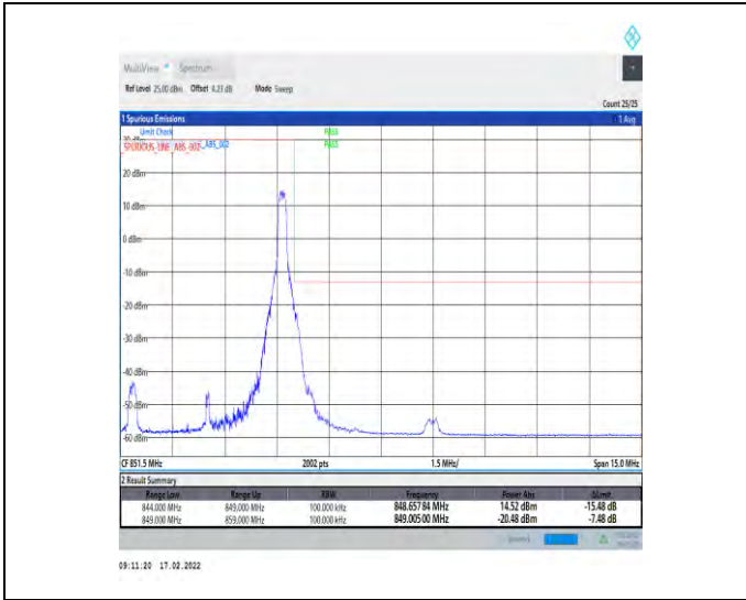
1-N5-15-5-H-2-DFT-PI2BPSK-Edge_1RB_Right-1@24-Ant0-seegraph-PASS-see graph
