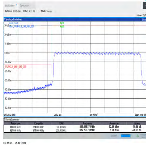
1-N5-15-20-L-3-DFT-PI2BPSK-Outer_Full-100@0-Ant0-seegraph-PASS-see graph
