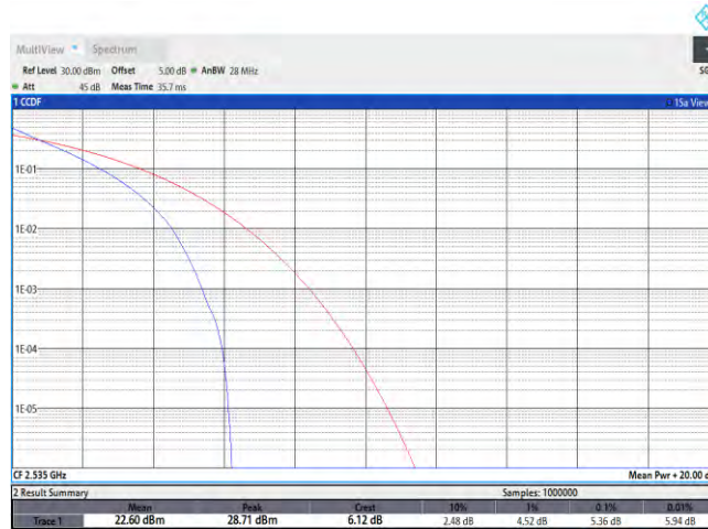
Band7-20MHz-QPSK-21100-100RB#0
