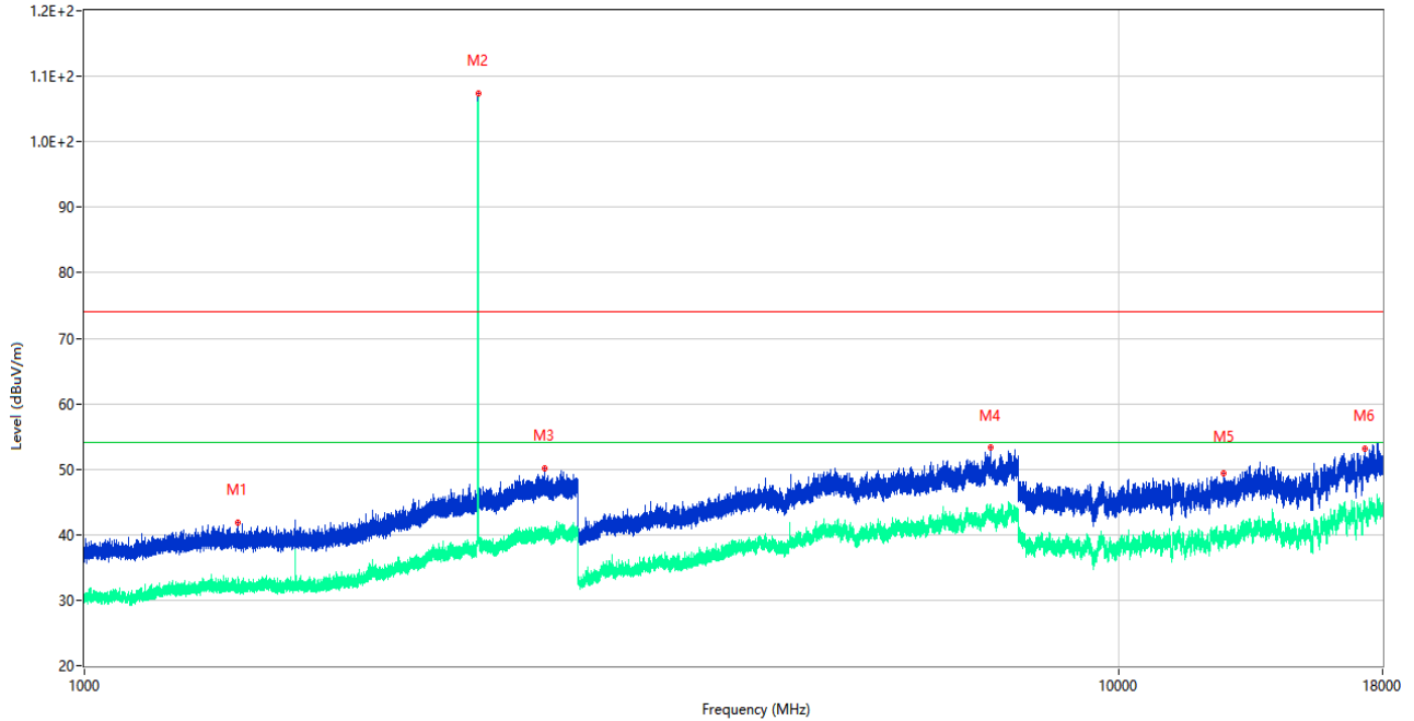
RSE (SRD)_FCC Part 15C_FCC 15.247(2.4G)_1GHz-18GHz
