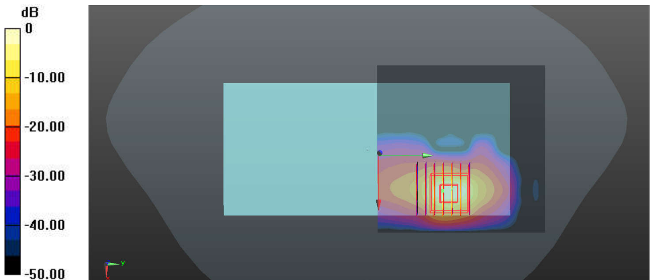
0 dB = 13.6 W/kg
