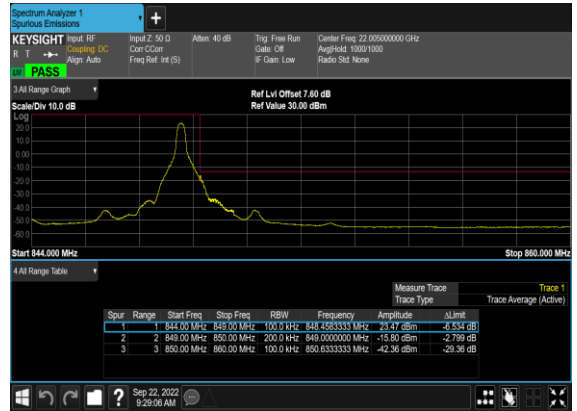
N5(20M)_DFT-s-OFDM_BPSK_Edge_1RB_Right_High_CH
