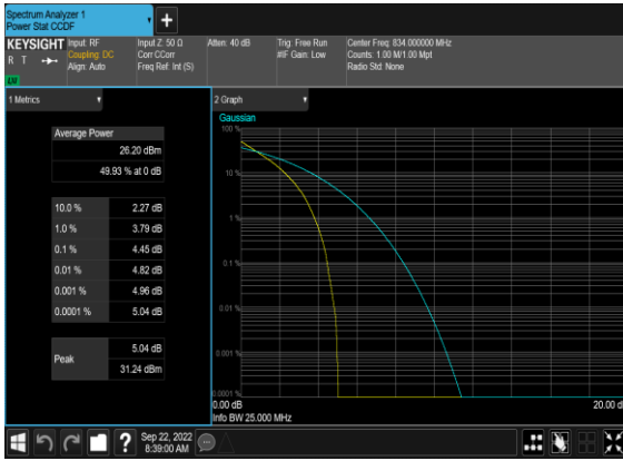
N5(20M)_DFT-s-OFDM_QPSK_Outer_Full_Low_CH
