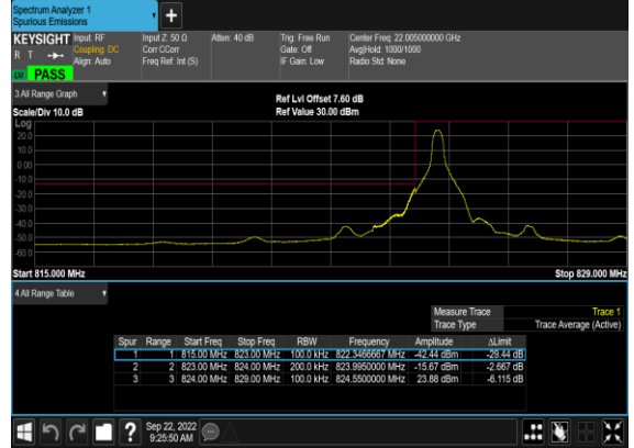
N5(20M)_DFT-s-OFDM_BPSK_Edge_1RB_Left_Low_CH
