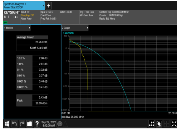
N5(20M)_DFT-s-OFDM_PI_2-BPSK_Edge_1RB_Left_High_CH
