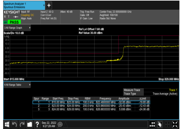
N5(20M)_DFT-s-OFDM_BPSK_Outer_Full_Low_CH
