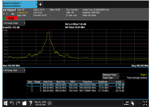
N5(10M)_DFT-s-OFDM_QPSK_Edge_1RB_Right_High_CH
