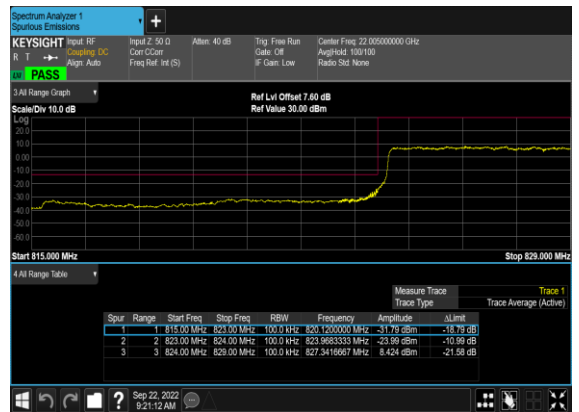
N5(10M)_DFT-s-OFDM_BPSK_Outer_Full_Low_CH
