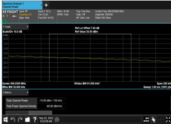
N5(10M)_DFT-s-OFDM_BPSK_Edge_1RB_Right_High_CH_CHP_PASS
