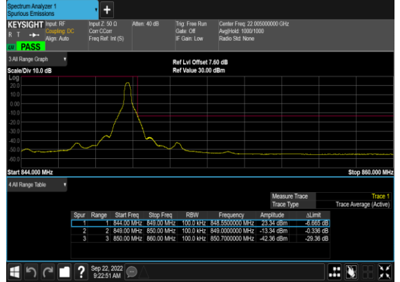
N5(10M)_DFT-s-OFDM_BPSK_Edge_1RB_Right_High_CH
