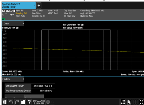
N5(10M)_DFT-s-OFDM_QPSK_Edge_1RB_Right_High_CH_CHP_PASS
