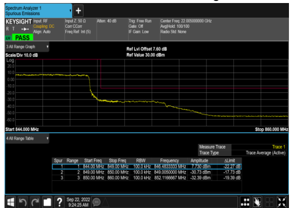
N5(10M)_DFT-s-OFDM_BPSK_Outer_Full_High_CH
