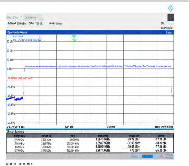
1-N78-3700-3800-PASS-30-90-L-6-CP-QPSK-Outer_Full-245@0-Ant1-1--PASS-see graph
