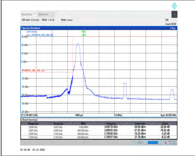
1-N78-3700-3800-PASS-30-20-L-4-CP-QPSK-Edge_1RB_Left-1@0-Ant1-1--PASS-see graph
