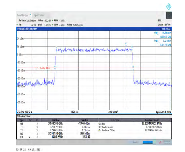
1-N78-3700-3800-PASS-30-100-L-9-CP-256QAM-Out uter_Full-273@0-Ant1-97.239-100.800-≤100-PASS
