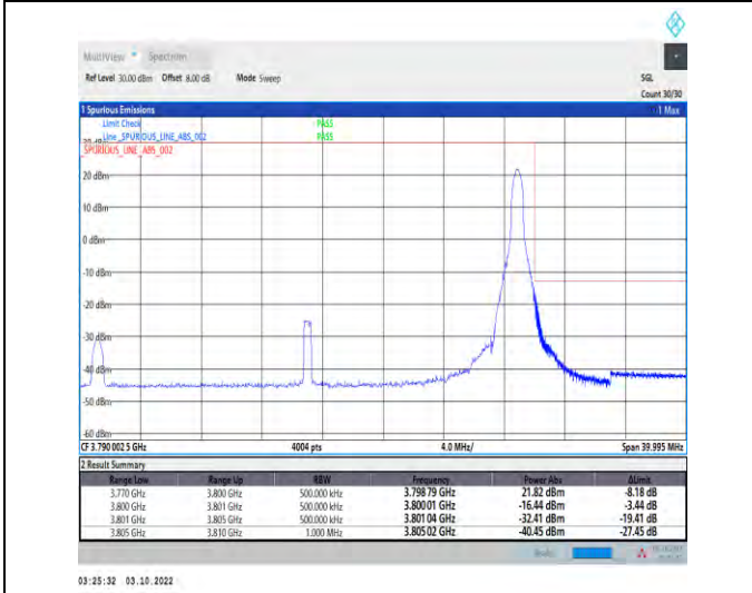
1-N78-3700-3800-PASS-30-30-H-5-CP-QPSK-Edge_1RB_Right-1@77-Ant1-1--PASS-see graph
