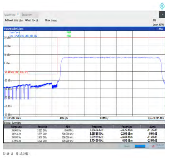
1-N78-3700-3800-PASS-30-20-L-6-CP-QPSK-Outer_Full-51@0-Ant1-1--PASS-see graph
