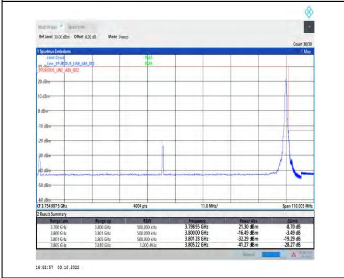
1-N78-3700-3800-PASS-30-100-H-5-CP-QPSK-Edge_1RB_Right-1@272-Ant1-1--PASS-see graph
