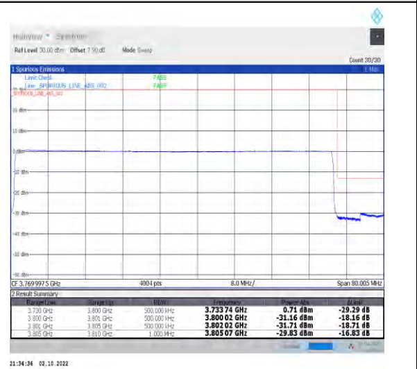
1-N78-3700-3800-PASS-30-70-H-6-CP-QPSK-Outer_Full-189@0-Ant1-1--PASS-see graph
