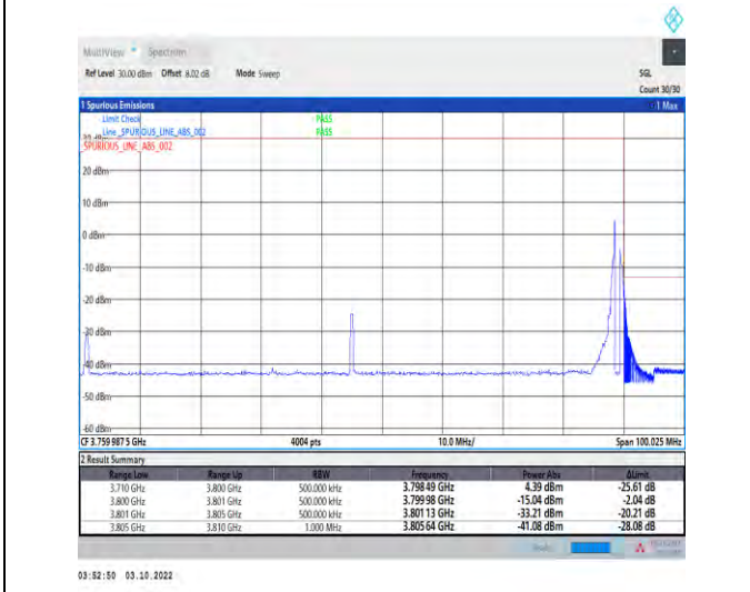
1-N78-3700-3800-PASS-30-90-H-5-CP-QPSK-Edge_1RB_Right-1@244-Ant1-1--PASS-see graph
