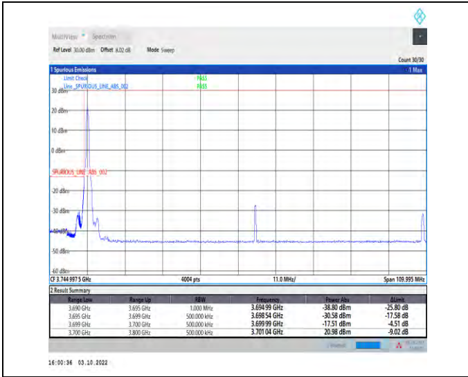
1-N78-3700-3800-PASS-30-100-L-1-DFT-PI2BPSK-Edge_1RB_Left-1@0-Ant1-1--PASS-see graph
