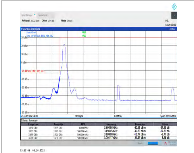
1-N78-3700-3800-PASS-30-30-L-1-DFT-PI2BPSK-Edge_e_1RB_Left-1@0-Ant1-1--PASS-see graph
