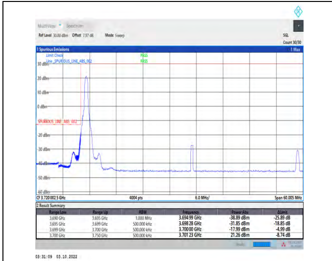
1-N78-3700-3800-PASS-30-50-L-1-DFT-PI2BPSK-Edge_1_RB_Left-1@0-Ant1-1--PASS-see graph
