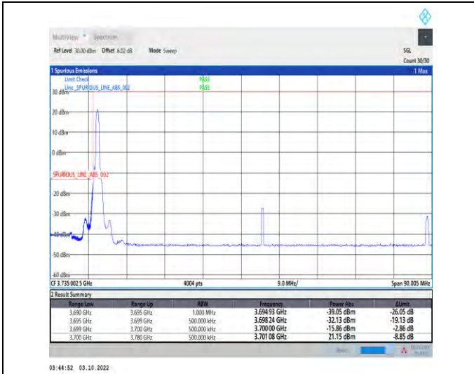
1-N78-3700-3800-PASS-30-80-L-1-DFT-PI2BPSK-Edge_e_1RB_Left-1@0-Ant1-1--PASS-see graph
