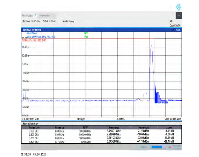
1-N78-3700-3800-PASS-30-50-H-2-DFT-PI2BPSK-Edge_1RB_Right-1@132-Ant1-1--PASS-see graph
