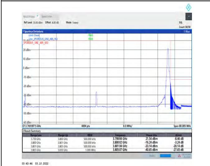
1-N78-3700-3800-PASS-30-70-H-5-CP-QPSK-Edge_1RB_Right-1@188-Ant1-1--PASS-see graph
