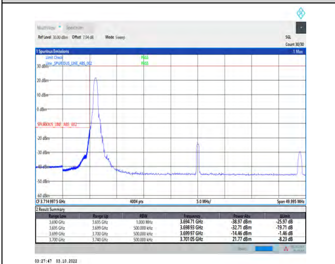
1-N78-3700-3800-PASS-30-40-L-4-CP-QPSK-Edge_1_RB_Left-1@0-Ant1-1--PASS-see graph
