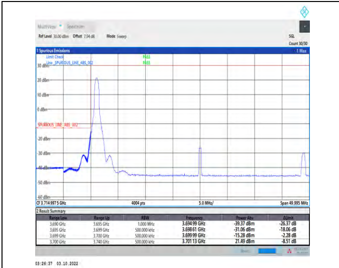
1-N78-3700-3800-PASS-30-40-L-1-DFT-PI2BPSK-Edge_1_RB_Left-1@0-Ant1-1--PASS-see graph
