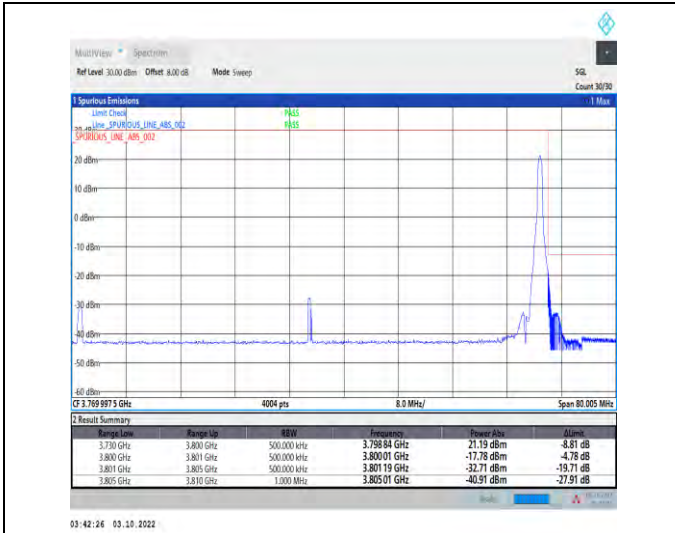
1-N78-3700-3800-PASS-30-70-H-2-DFT-PI2BPSK-Edge_1RB_Right-1@188-Ant1-1--PASS-see graph
