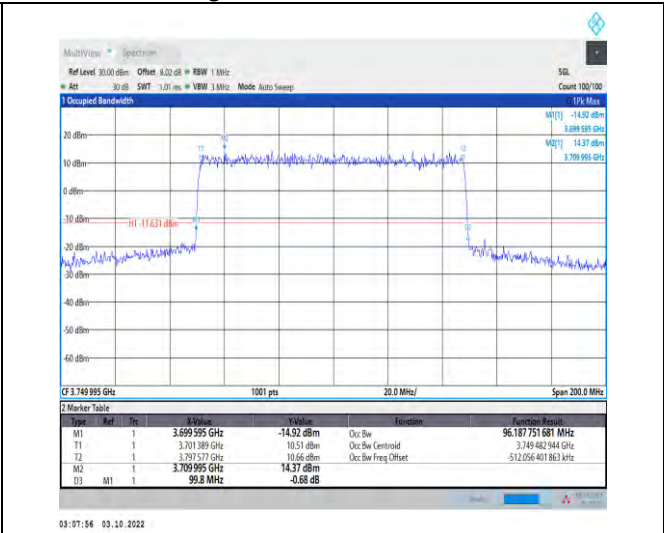
1-N78-3700-3800-PASS-30-100-M-1-DFT-QPSK-Out er_Full-270@0-Ant1-96.188-99.800-≤100-PASS
