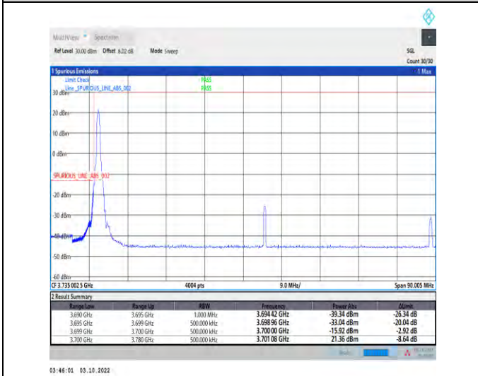
1-N78-3700-3800-PASS-30-80-L-4-CP-QPSK-Edge_1RB_Left-1@0-Ant1-1--PASS-see graph
