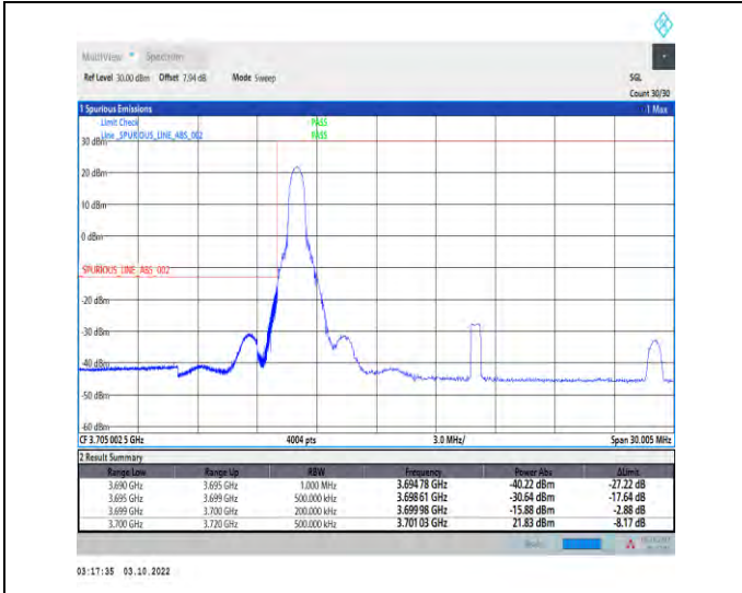
1-N78-3700-3800-PASS-30-20-L-1-DFT-PI2BPSK-Edge_e_1RB_Left-1@0-Ant1-1--PASS-see graph
