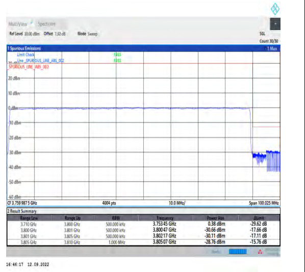
1-N78-3700-3800-PASS-30-90-H-6-CP-QPSK-Outer_Full-245@0-Ant1-1--PASS-see graph
