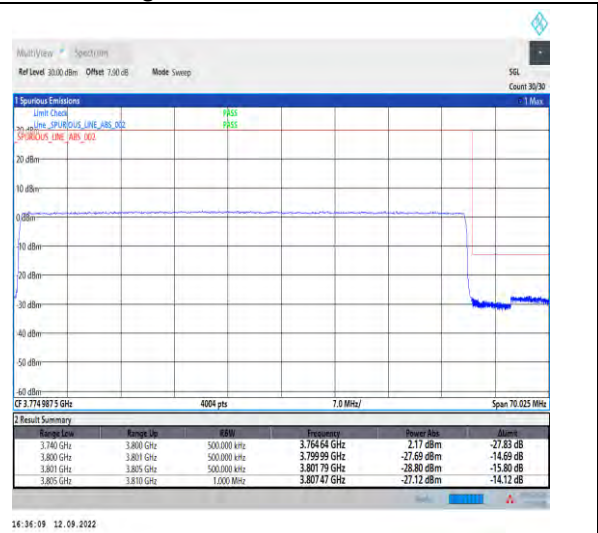
1-N78-3700-3800-PASS-30-60-H-3-DFT-PI2BPSK-Outer_Full-162@0-Ant1-1--PASS-see graph
