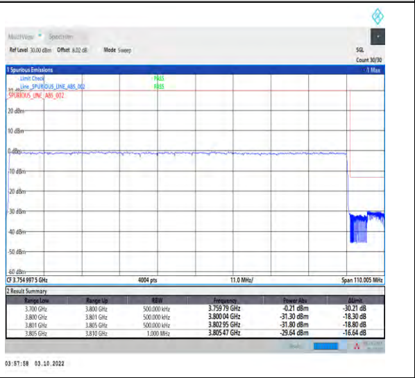
1-N78-3700-3800-PASS-30-100-H-6-CP-QPSK-Outer_Full-273@0-Ant1-1--PASS-see graph
