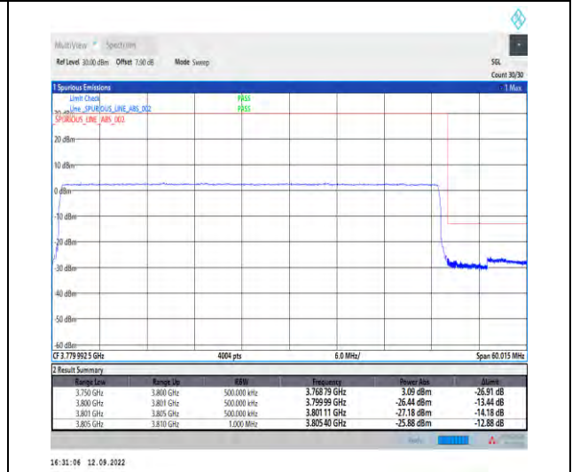
1-N78-3700-3800-PASS-30-50-H-6-CP-QPSK-Outer_Full-133@0-Ant1-1--PASS-see graph
