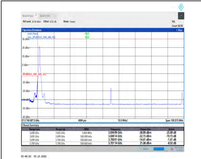
1-N78-3700-3800-PASS-30-90-L-1-DFT-PI2BPSK-Edge_e_1RB_Left-1@0-Ant1-1--PASS-see graph
