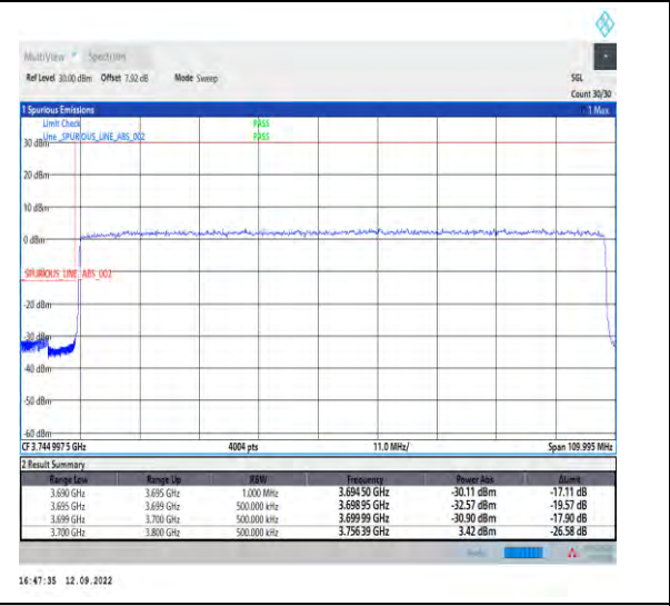
1-N78-3700-3800-PASS-30-100-L-6-CP-QPSK-Outer_Full-273@0-Ant1-1--PASS-see graph
