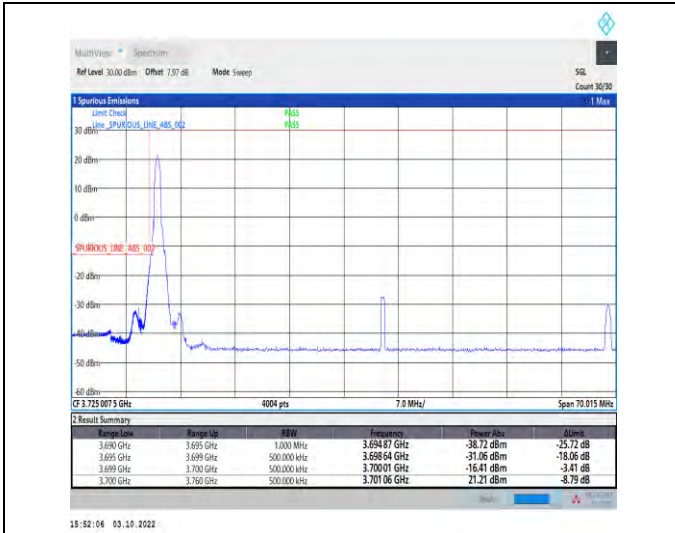
1-N78-3700-3800-PASS-30-60-L-1-DFT-PI2BPSK-Edge_1_RB_Left-1@0-Ant1-1--PASS-see graph
