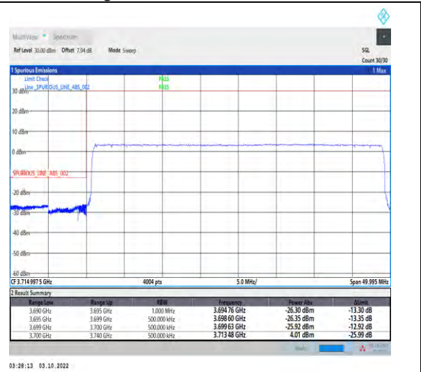
1-N78-3700-3800-PASS-30-40-L-3-DFT-PI2BPSK-Outer_Full-100@0-Ant1-1--PASS-see graph
