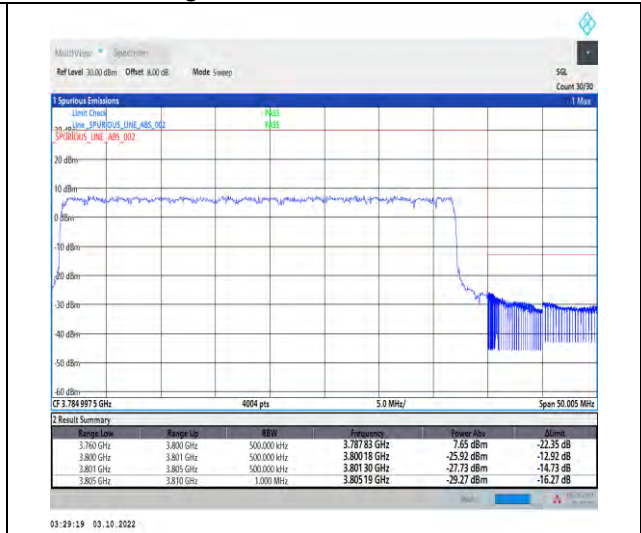
1-N78-3700-3800-PASS-30-40-H-3-DFT-PI2BPSK-Outer_Full-100@0-Ant1-1--PASS-see graph
