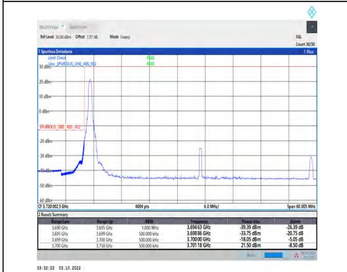
1-N78-3700-3800-PASS-30-50-L-4-CP-QPSK-Edge_1_RB_Left-1@0-Ant1-1--PASS-see graph
