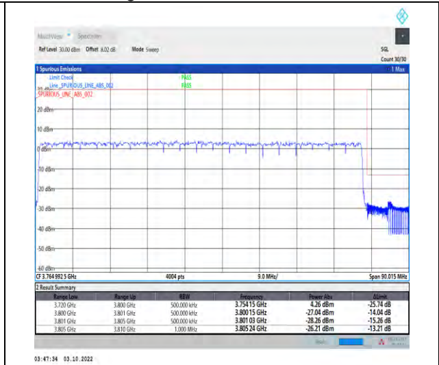
1-N78-3700-3800-PASS-30-80-H-3-DFT-PI2BPSK-Outer_Full-216@0-Ant1-1--PASS-see graph
