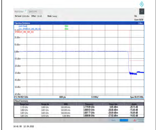
1-N78-3700-3800-PASS-30-80-H-6-CP-QPSK-Outer_Full-217@0-Ant1-1--PASS-see graph
