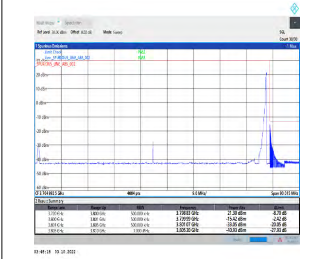
1-N78-3700-3800-PASS-30-80-H-5-CP-QPSK-Edge_1RB_Right-1@216-Ant1-1--PASS-see graph
