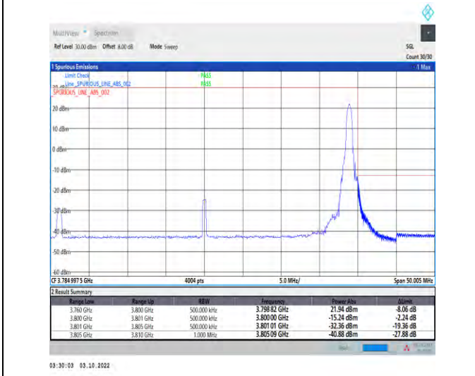
1-N78-3700-3800-PASS-30-40-H-5-CP-QPSK-Edge_1RB_Right-1@105-Ant1-1--PASS-see graph
