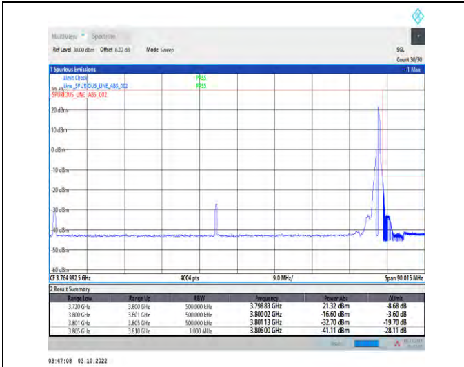
1-N78-3700-3800-PASS-30-80-H-2-DFT-PI2BPSK-Edge_1RB_Right-1@216-Ant1-1--PASS-see graph
