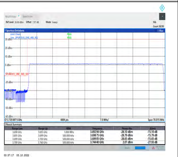
1-N78-3700-3800-PASS-30-60-L-6-CP-QPSK-Outer_Full-162@0-Ant1-1--PASS-see graph
