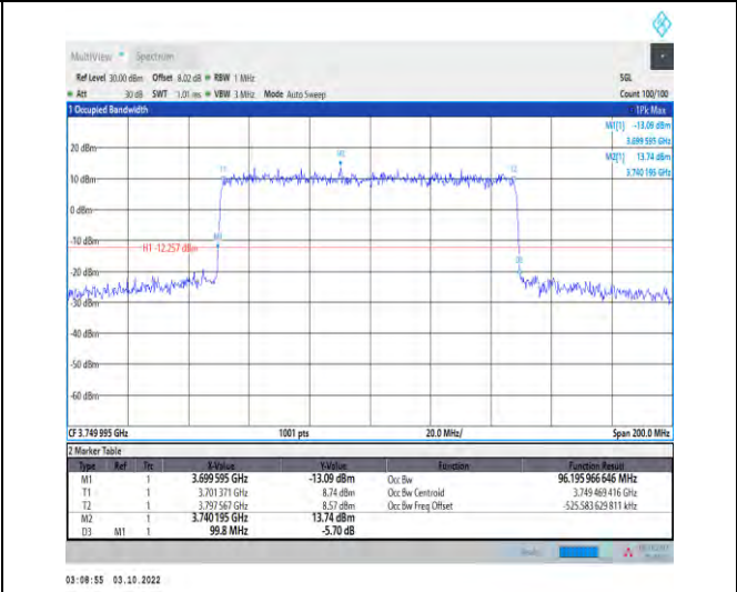
1-N78-3700-3800-PASS-30-100-M-3-DFT-16QAM-Outer uter_Full-270@0-Ant1-96.196-99.800-≤100-PASS
