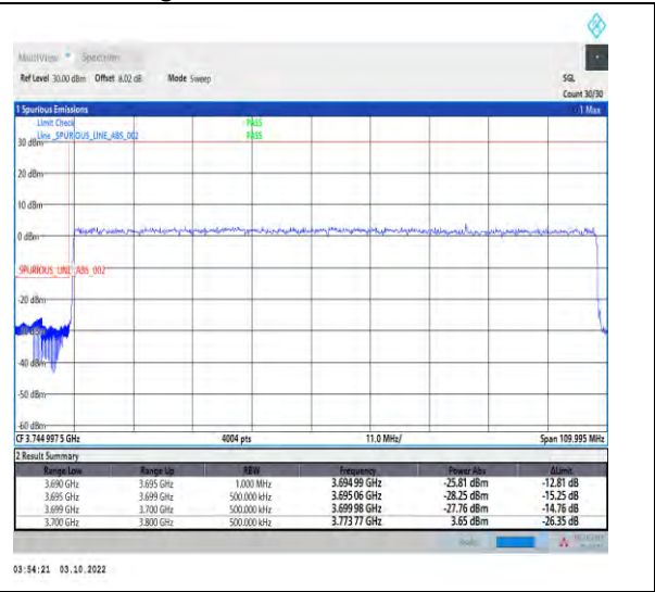
1-N78-3700-3800-PASS-30-100-L-3-DFT-PI2BPSK-K-Outer_Full-270@0-Ant1-1--PASS-see graph
