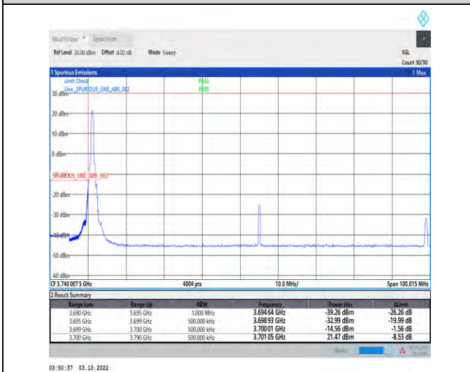
1-N78-3700-3800-PASS-30-90-L-4-CP-QPSK-Edge_1RB_Left-1@0-Ant1-1--PASS-see graph
