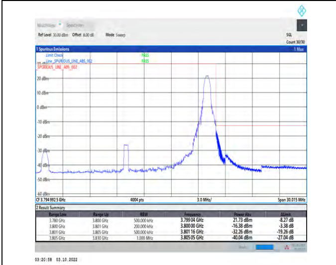
1-N78-3700-3800-PASS-30-20-H-5-CP-QPSK-Edge_1RB_Right-1@50-Ant1-1--PASS-see graph
