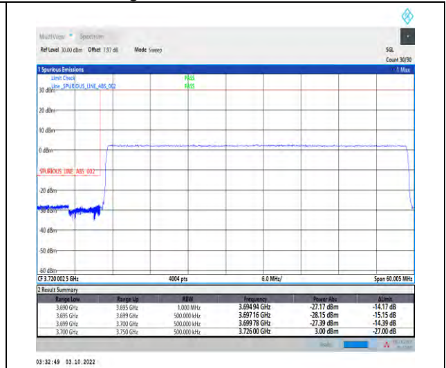
1-N78-3700-3800-PASS-30-50-L-3-DFT-PI2BPSK-Outer_Full-128@0-Ant1-1--PASS-see graph
