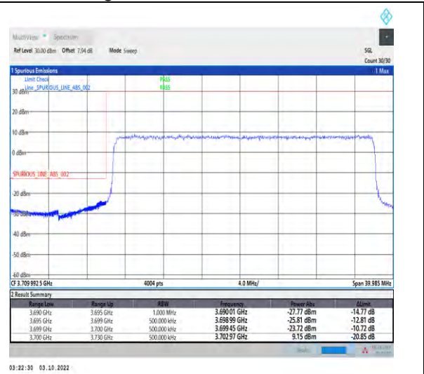
1-N78-3700-3800-PASS-30-30-L-3-DFT-PI2BPSK-Outer_Full-75@0-Ant1-1--PASS-see graph
