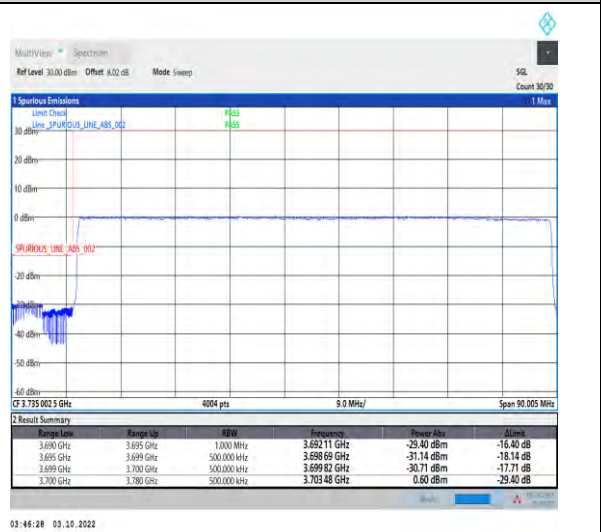
1-N78-3700-3800-PASS-30-80-L-6-CP-QPSK-Outer_Full-217@0-Ant1-1--PASS-see graph
