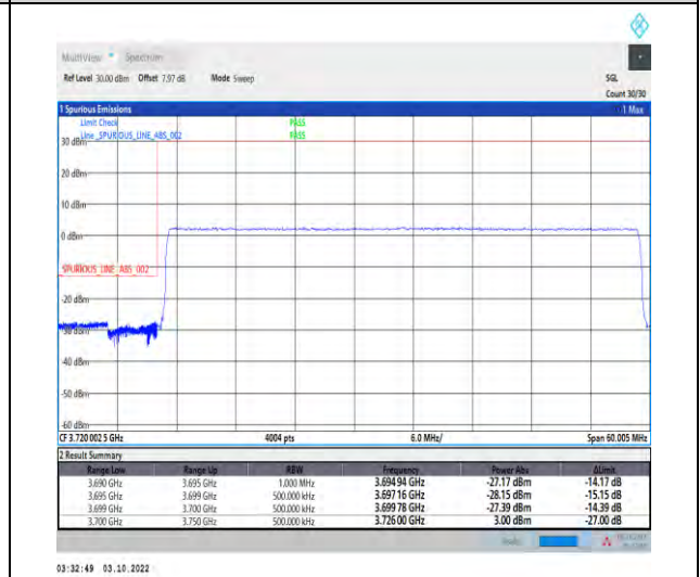
1-N78-3700-3800-PASS-30-50-L-6-CP-QPSK-Outer_Full-133@0-Ant1-1--PASS-see graph
