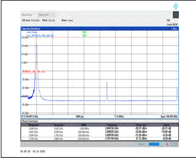
1-N78-3700-3800-PASS-30-100-L-4-CP-QPSK-Edge_1RB_Left-1@0-Ant1-1--PASS-see graph
