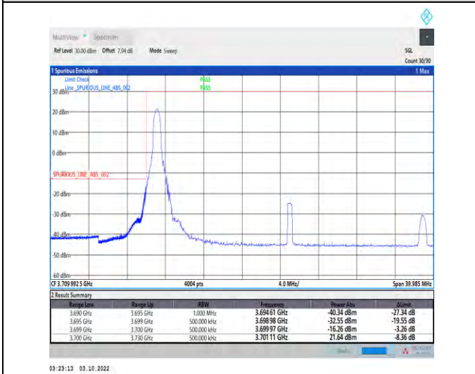
1-N78-3700-3800-PASS-30-30-L-4-CP-QPSK-Edge_1RB_Left-1@0-Ant1-1--PASS-see graph
