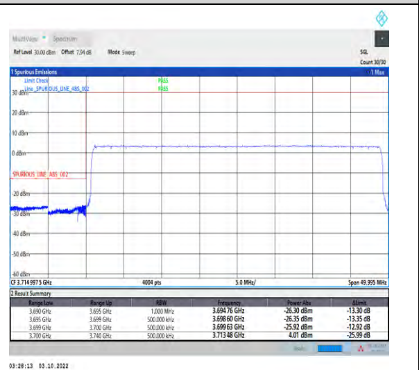
1-N78-3700-3800-PASS-30-40-L-6-CP-QPSK-Outer_Full-106@0-Ant1-1--PASS-see graph
