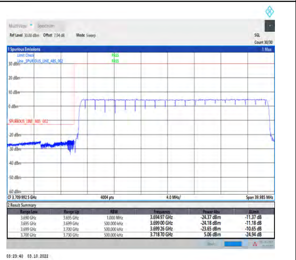
1-N78-3700-3800-PASS-30-30-L-6-CP-QPSK-Outer_Full-78@0-Ant1-1--PASS-see graph
