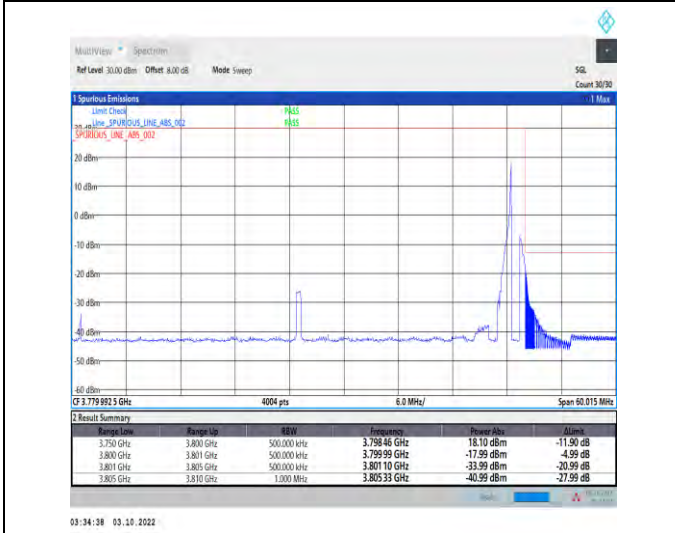
1-N78-3700-3800-PASS-30-50-H-5-CP-QPSK-Edge_1RB_Right-1@132-Ant1-1--PASS-see graph
