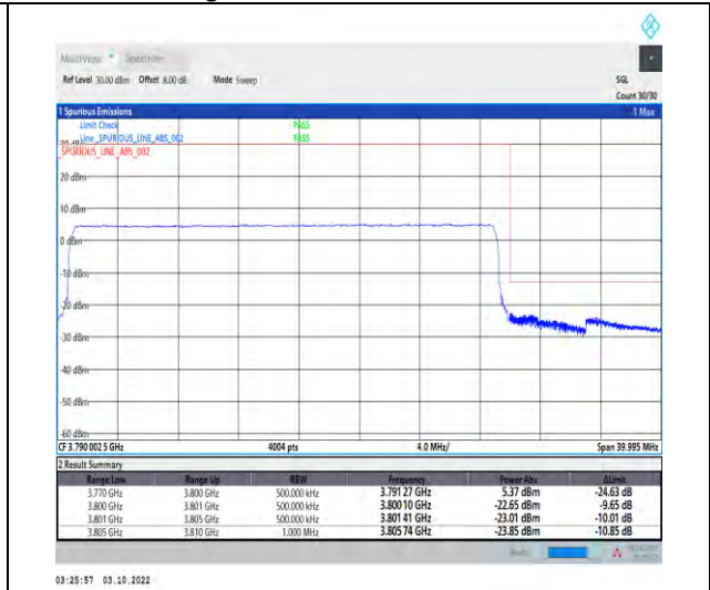
1-N78-3700-3800-PASS-30-30-H-3-DFT-PI2BPSK-Outer_Full-75@0-Ant1-1--PASS-see graph
