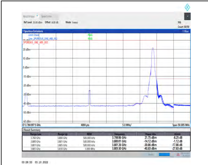
1-N78-3700-3800-PASS-30-40-H-2-DFT-PI2BPSK-Edge_1RB_Right-1@105-Ant1-1--PASS-see graph
