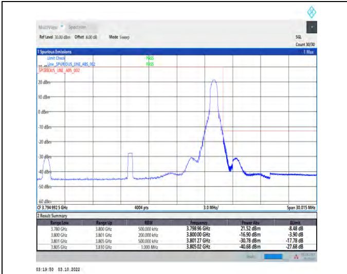
1-N78-3700-3800-PASS-30-20-H-2-DFT-PI2BPSK-Edge_1RB_Right-1@50-Ant1-1--PASS-see graph
