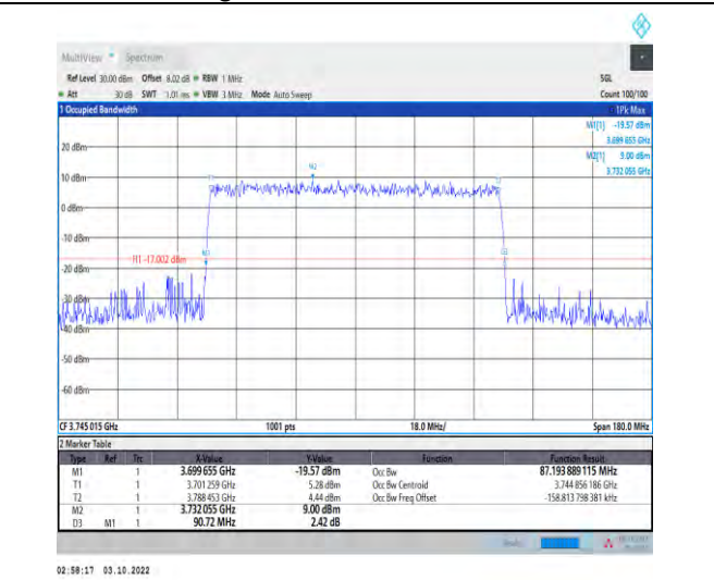
1-N78-3700-3800-PASS-30-90-L-9-CP-256QAM-Out er_Full-245@0-Ant1-87.194-90.720-≤90-PASS
