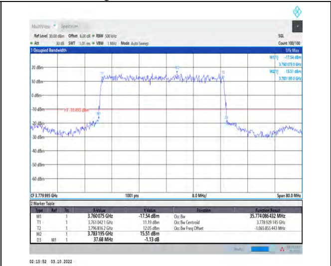
1-N78-3700-3800-PASS-30-40-H-2-DFT-PI2BPSK-O uter_Full-100@0-Ant1-35.774-37.680-≤40-PASS
