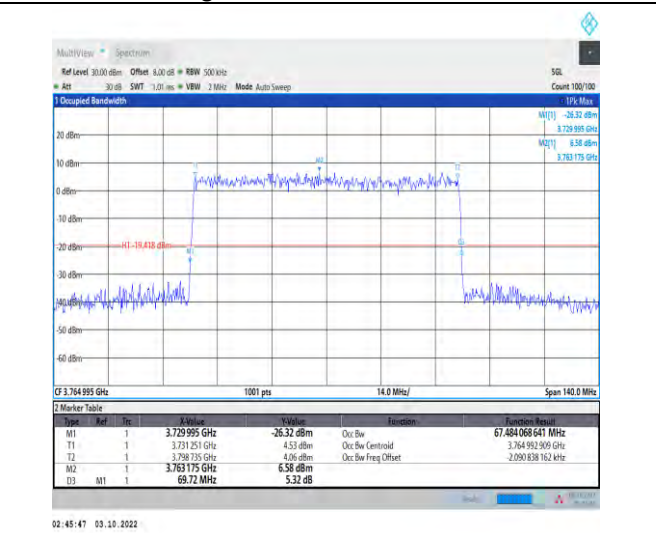
1-N78-3700-3800-PASS-30-70-H-9-CP-256QAM-Out er_Full-189@0-Ant1-67.484-69.720-≤70-PASS
