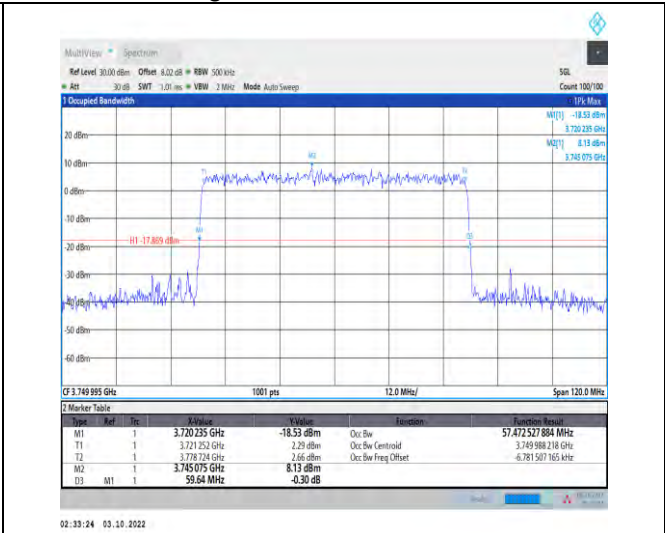
1-N78-3700-3800-PASS-30-60-M-9-CP-256QAM-Out er_Full-162@0-Ant1-57.473-59.640-≤60-PASS
