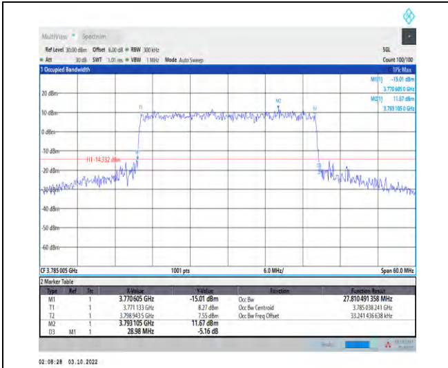
1-N78-3700-3800-PASS-30-30-H-8-CP-64QAM-Out er_Full-78@0-Ant1-27.81-28.980-≤30-PASS
