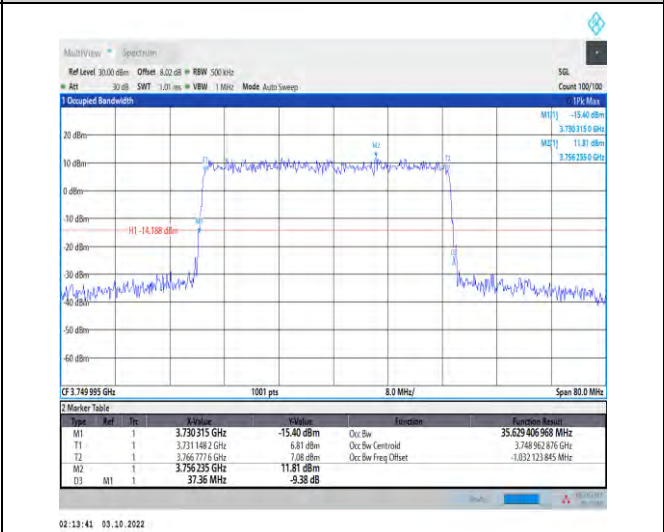
1-N78-3700-3800-PASS-30-40-M-5-DFT-256QAM-O uter_Full-100@0-Ant1-35.629-37.360-≤40-PASS
