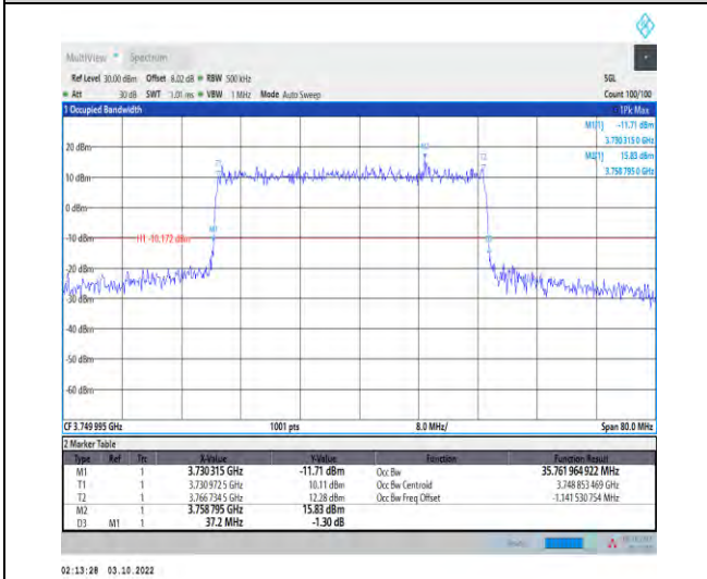
1-N78-3700-3800-PASS-30-40-M-4-DFT-64QAM-Ou ter_Full-100@0-Ant1-35.762-37.200-≤40-PASS
