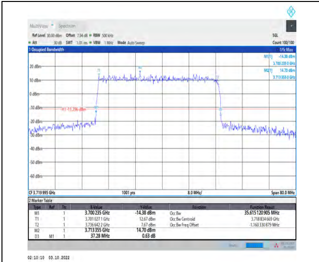
1-N78-3700-3800-PASS-30-40-L-3-DFT-16QAM-Out er_Full-100@0-Ant1-35.615-37.280-≤40-PASS
