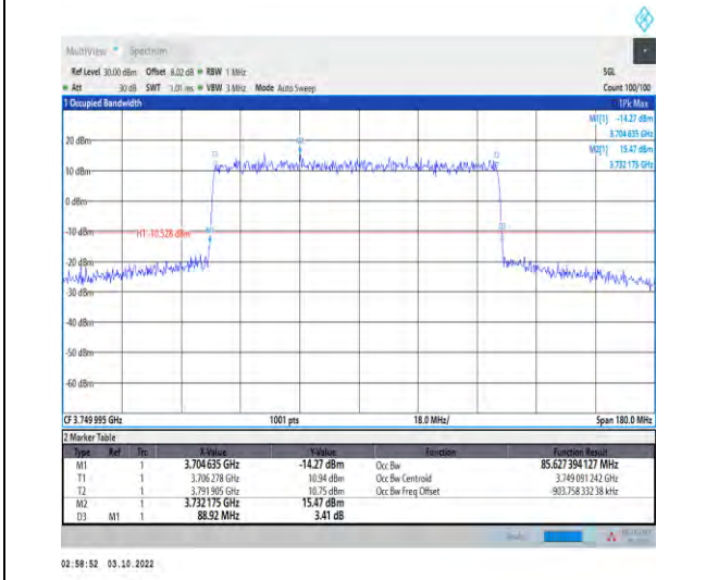
1-N78-3700-3800-PASS-30-90-M-1-DFT-QPSK-Out er_Full-240@0-Ant1-85.627-88.920-≤90-PASS
