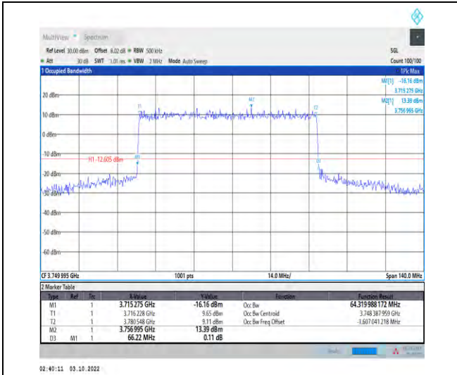
1-N78-3700-3800-PASS-30-70-M-1-DFT-QPSK-Out er_Full-180@0-Ant1-64.32-66.220-≤70-PASS
