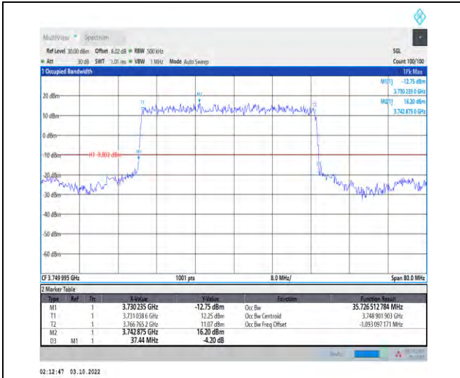
1-N78-3700-3800-PASS-30-40-M-2-DFT-PI2BPSK-Outer_Full-100@0-Ant1-35.727-37.440-≤40-PASS
