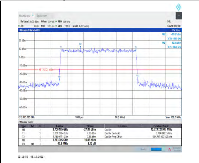
1-N78-3700-3800-PASS-30-50-L-5-DFT-256QAM-Out er_Full-128@0-Ant1-45.774-47.800-≤50-PASS
