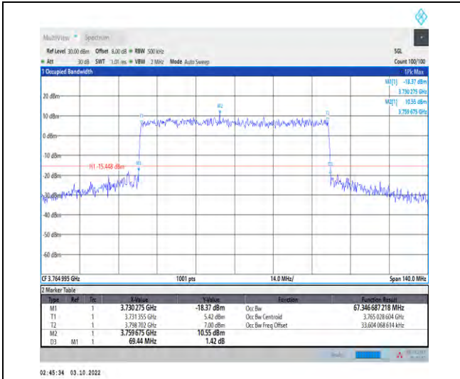
1-N78-3700-3800-PASS-30-70-H-8-CP-64QAM-Out er_Full-189@0-Ant1-67.347-69.440-≤70-PASS
