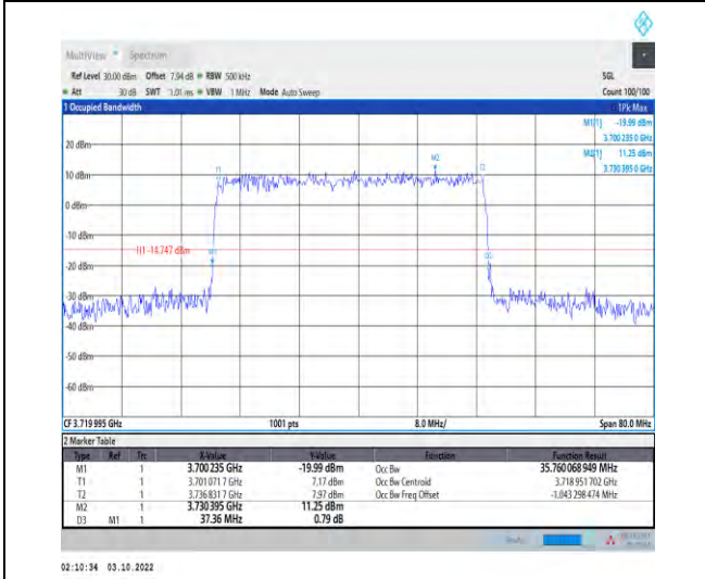
1-N78-3700-3800-PASS-30-40-L-5-DFT-256QAM-Out er_Full-100@0-Ant1-35.76-37.360-≤40-PASS
