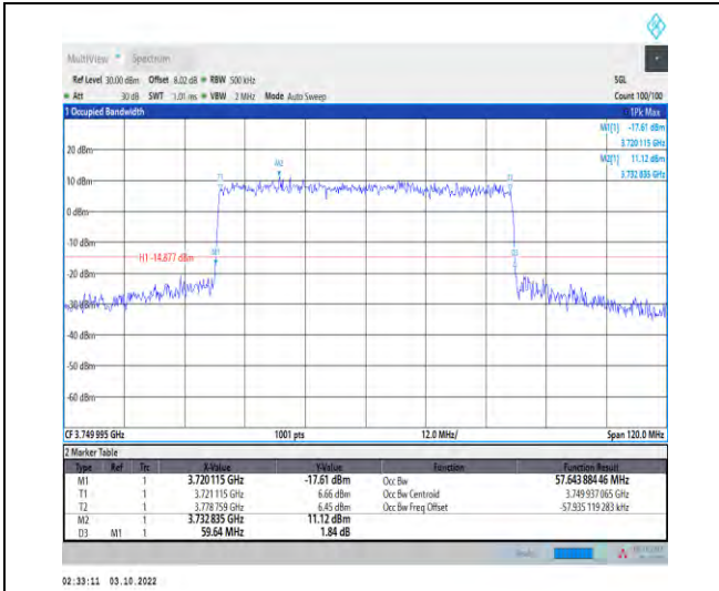
1-N78-3700-3800-PASS-30-60-M-8-CP-64QAM-Out er_Full-162@0-Ant1-57.644-59.640-≤60-PASS
