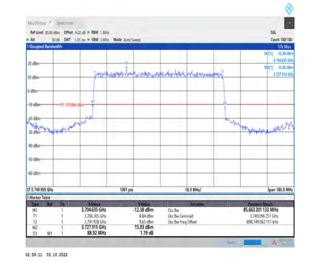
1-N78-3700-3800-PASS-30-90-M-2-DFT-PI2BPSK-Out er_Full-240@0-Ant1-85.663-88.920-≤90-PASS
