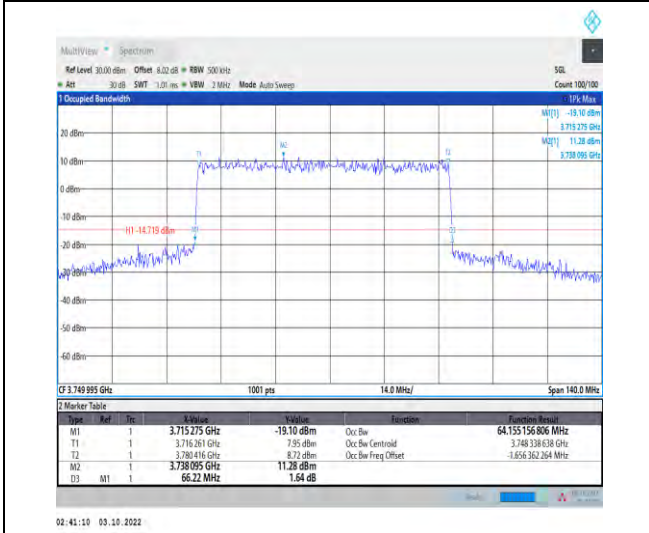
1-N78-3700-3800-PASS-30-70-M-3-DFT-16QAM-Ou ter_Full-180@0-Ant1-64.155-66.220-≤70-PASS
