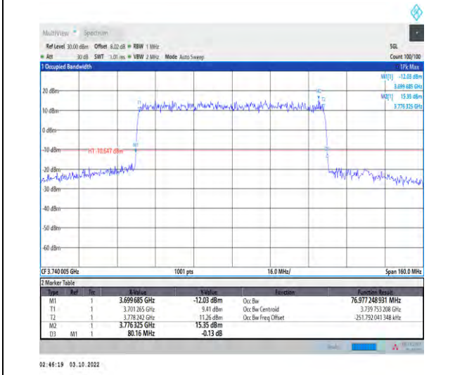
1-N78-3700-3800-PASS-30-80-L-1-DFT-QPSK-Out er_Full-216@0-Ant1-76.977-80.160-≤80-PASS
