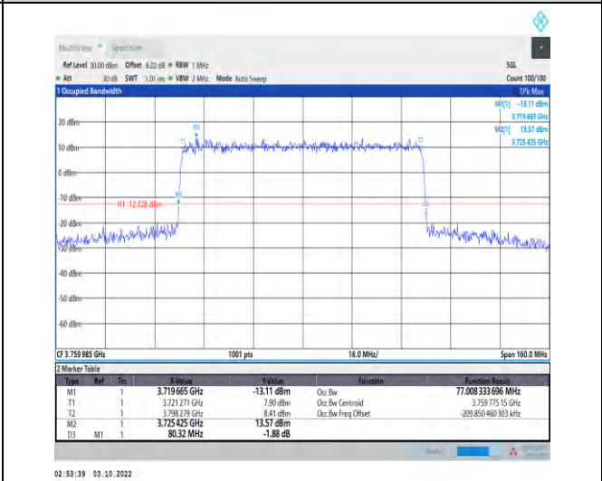
1-N78-3700-3800-PASS-30-80-H-4-DFT-64QAM-Out er_Full-216@0-Ant1-77.008-80.320-≤80-PASS
