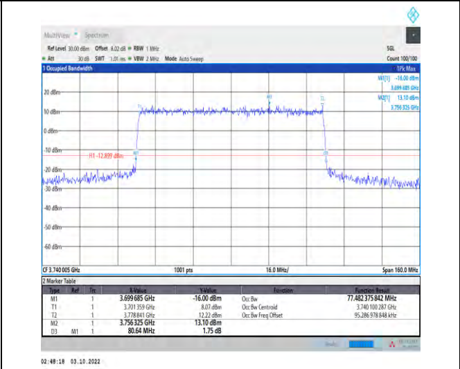
1-N78-3700-3800-PASS-30-80-L-6-CP-QPSK-Outer Full-217@0-Ant1-77.482-80.640-≤80-PASS
