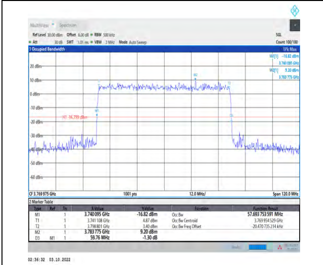
1-N78-3700-3800-PASS-30-60-H-9-CP-256QAM-Out er_Full-162@0-Ant1-57.694-59.760-≤60-PASS
