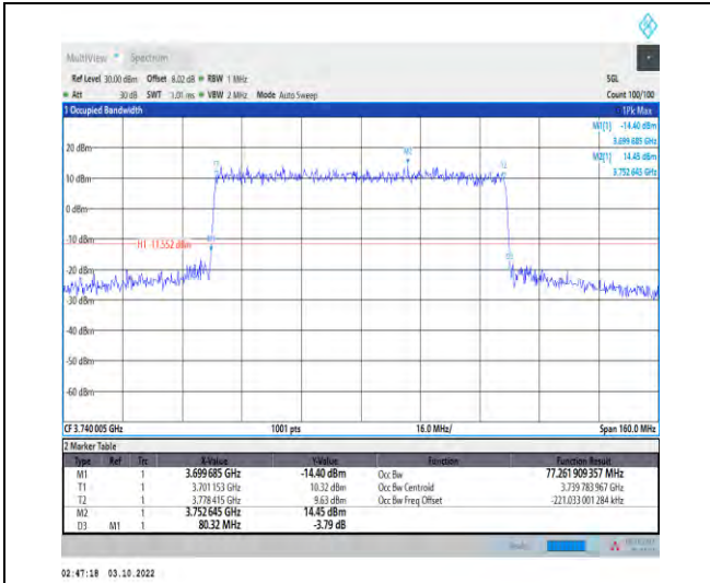
1-N78-3700-3800-PASS-30-80-L-3-DFT-16QAM-Out er_Full-216@0-Ant1-77.262-80.320-≤80-PASS
