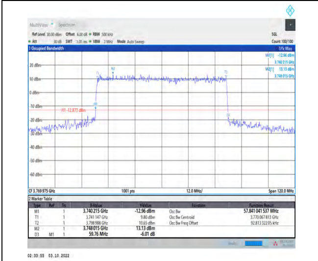
1-N78-3700-3800-PASS-30-60-H-1-DFT-QPSK-Out er_Full-162@0-Ant1-57.841-59.760-≤60-PASS
