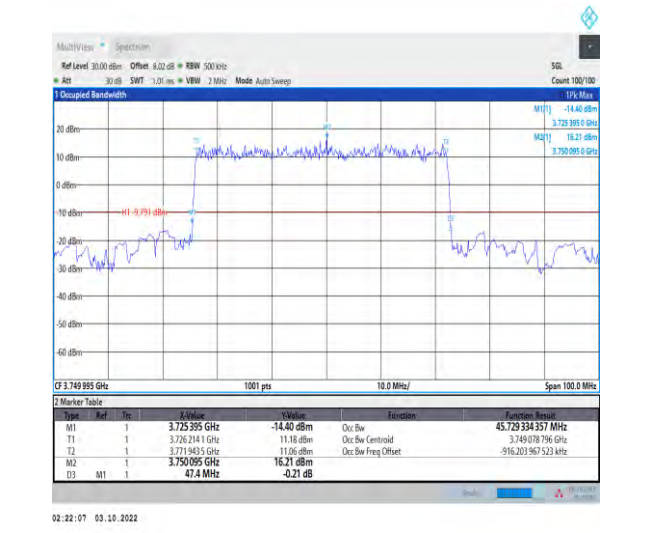
1-N78-3700-3800-PASS-30-50-M-2-DFT-PI2BPSK-Out er_Full-128@0-Ant1-45.729-47.400-≤50-PASS
