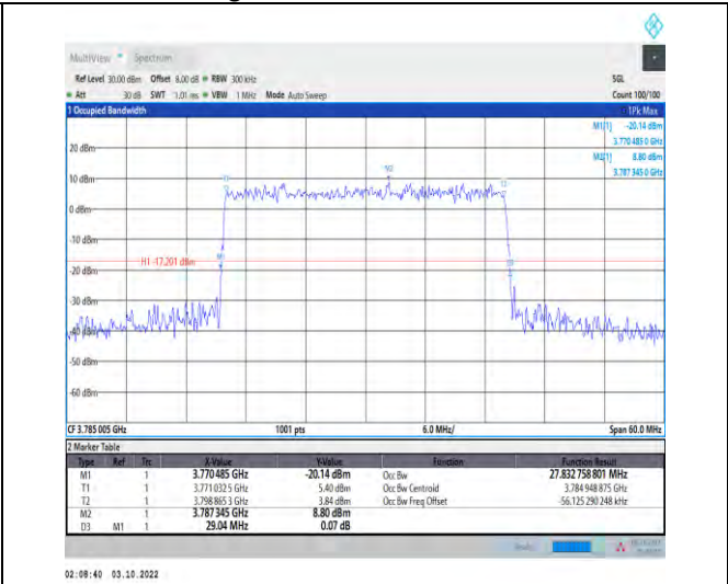
1-N78-3700-3800-PASS-30-30-H-9-CP-256QAM-Out er_Full-78@0-Ant1-27.833-29.040-≤30-PASS
