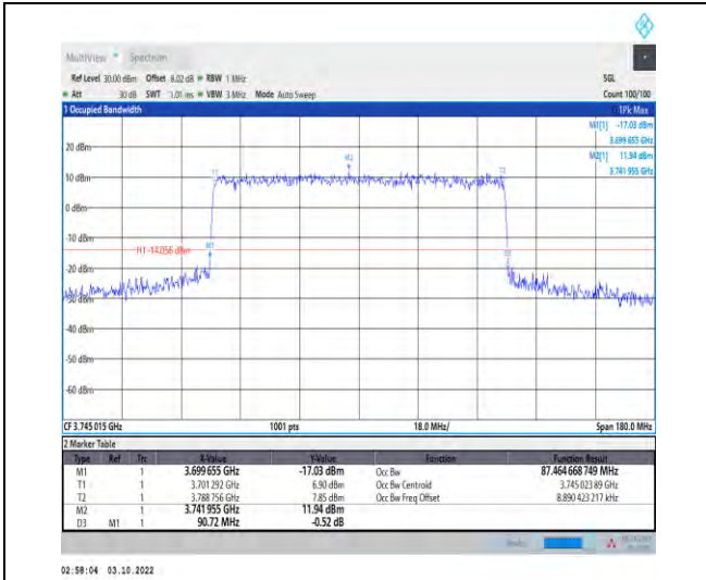
1-N78-3700-3800-PASS-30-90-L-8-CP-64QAM-Out er_Full-245@0-Ant1-87.465-90.720-≤90-PASS
