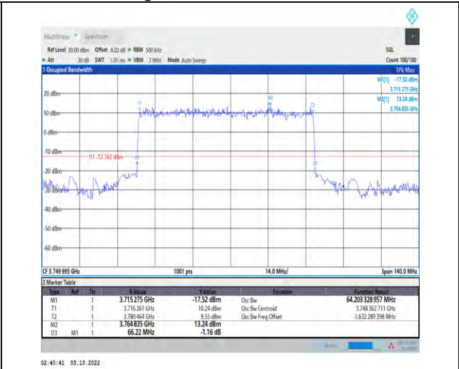
1-N78-3700-3800-PASS-30-70-M-2-DFT-PI2BPSK-O uter_Full-180@0-Ant1-64.203-66.220-≤70-PASS
