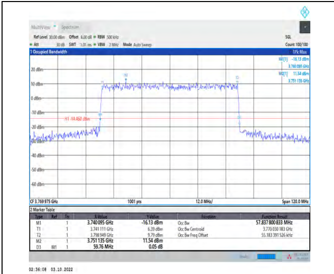
1-N78-3700-3800-PASS-30-60-H-7-CP-16QAM-Out er_Full-162@0-Ant1-57.838-59.760-≤60-PASS
