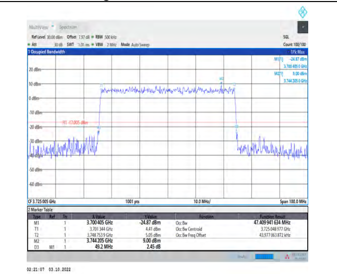
1-N78-3700-3800-PASS-30-50-L-9-CP-256QAM-Out er_Full-133@0-Ant1-47.41-49.200-≤50-PASS
