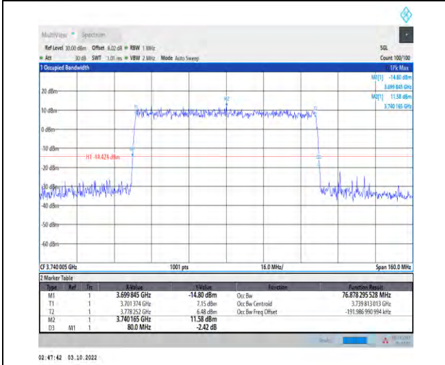
1-N78-3700-3800-PASS-30-80-L-5-DFT-256QAM-Out er_Full-216@0-Ant1-76.878-80.000-≤80-PASS
