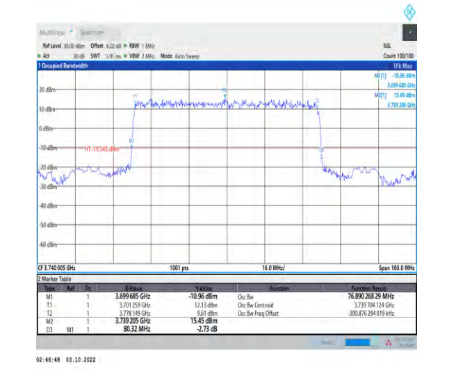
1-N78-3700-3800-PASS-30-80-L-2-DFT-PI2BPSK-Out er_Full-216@0-Ant1-76.89-80.320-≤80-PASS
