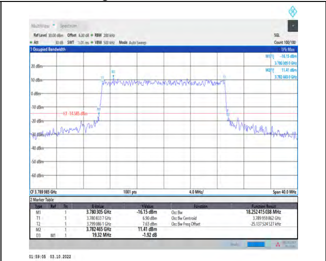
1-N78-3700-3800-PASS-30-20-H-8-CP-64QAM-Out er_Full-51@0-Ant1-18.252-19.320-≤20-PASS
