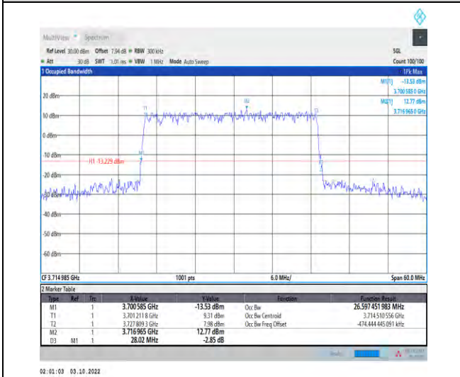
1-N78-3700-3800-PASS-30-30-L-4-DFT-64QAM-Out er_Full-75@0-Ant1-26.597-28.020-≤30-PASS
