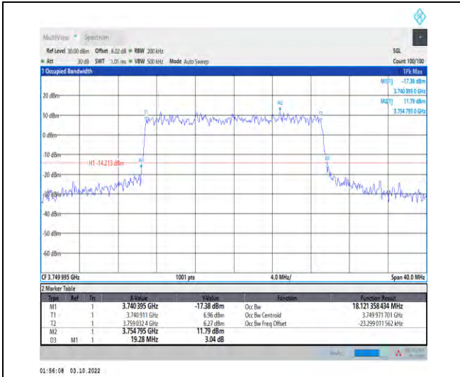
1-N78-3700-3800-PASS-30-20-M-8-CP-64QAM-Out_er_Full-51@0-Ant1-18.121-19.280-≤20-PASS
