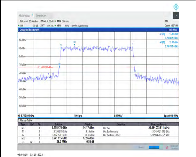
1-N78-3700-3800-PASS-30-30-M-4-DFT-64QAM-Out er_Full-75@0-Ant1-26.684-28.200-≤30-PASS
