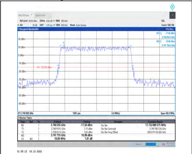
1-N78-3700-3800-PASS-30-20-M-5-DFT-256QAM-Outer_Full-50@0-Ant1-17.732-18.840-≤20-PASS
