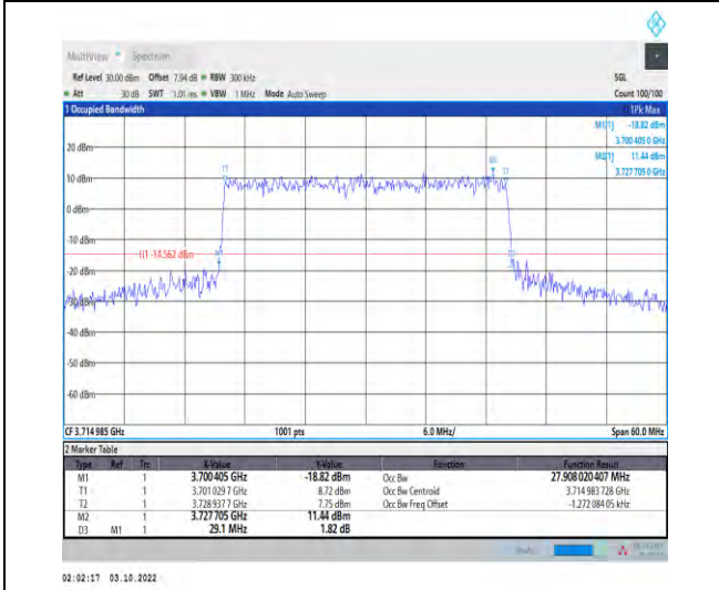
1-N78-3700-3800-PASS-30-30-L-8-CP-64QAM-Outer_Full-78@0-Ant1-27.908-29.100-≤30-PASS
