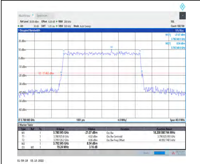
1-N78-3700-3800-PASS-30-20-H-9-CP-256QAM-Out er_Full-51@0-Ant1-18.2-19.240-≤20-PASS
