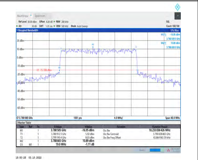
1-N78-3700-3800-PASS-30-20-H-6-CP-QPSK-Outer_Full-51@0-Ant1-18.233-19.000-≤20-PASS
