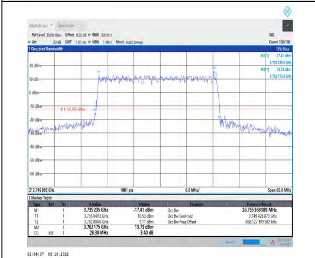
1-N78-3700-3800-PASS-30-30-M-3-DFT-16QAM-Ou ter_Full-75@0-Ant1-26.755-28.380-≤30-PASS
