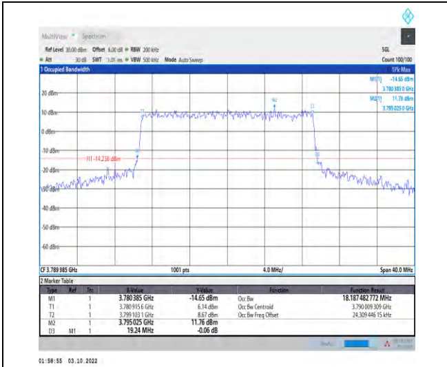
1-N78-3700-3800-PASS-30-20-H-7-CP-16QAM-Out er_Full-51@0-Ant1-18.187-19.240-≤20-PASS
