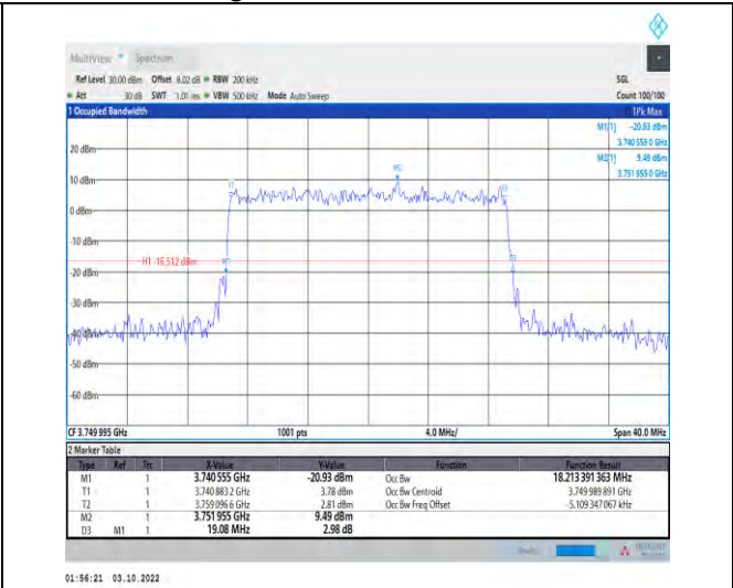
1-N78-3700-3800-PASS-30-20-M-9-CP-256QAM-Out_er_Full-51@0-Ant1-18.213-19.080-≤20-PASS
