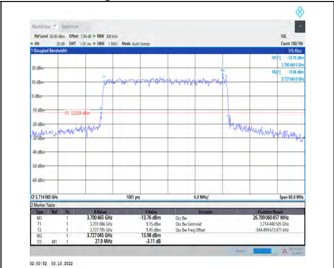
1-N78-3700-3800-PASS-30-30-L-3-DFT-16QAM-Out er_Full-75@0-Ant1-26.709-27.900-≤30-PASS
