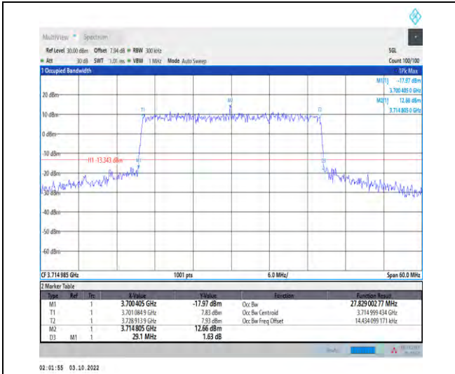
1-N78-3700-3800-PASS-30-30-L-6-CP-QPSK-Outer_Full-78@0-Ant1-27.829-29.100-≤30-PASS
