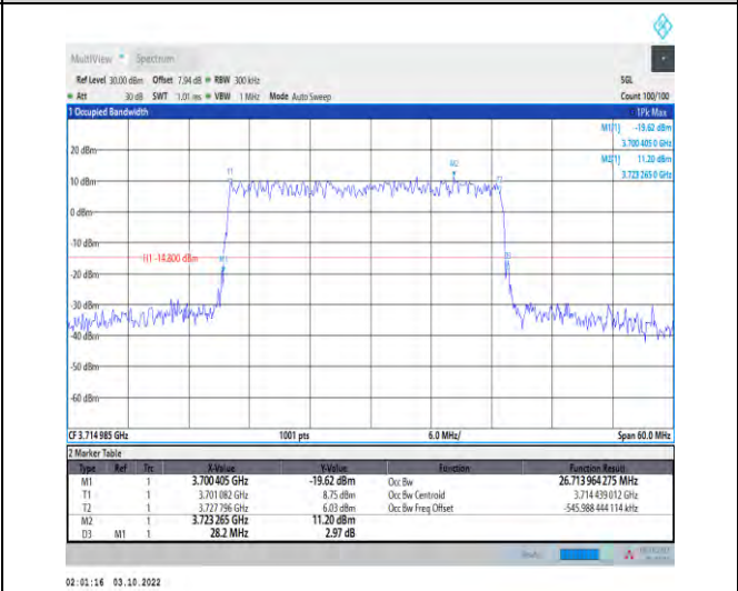
1-N78-3700-3800-PASS-30-30-L-5-DFT-256QAM-Out er_Full-75@0-Ant1-26.714-28.200-≤30-PASS
