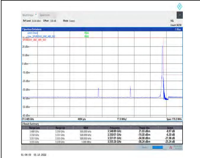
1-N78-3450-3550--30-70-H-5-CP-QPSK-Edge_1RB_R ight-1@188-Ant1-1--PASS-see graph
