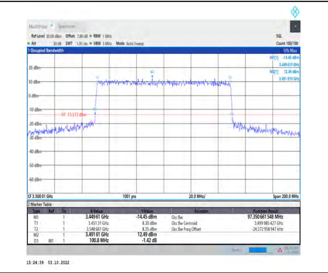
1-N78-3450-3550--30-100-M-7-CP-16QAM-Outer_Full-273@0-Ant1-97.351-100.800-≤100-PASS
