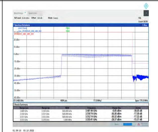
1-N78-3450-3550--30-90-H-6-CP-QPSK-Outer_Full-245@0-Ant1-1--PASS-see graph
