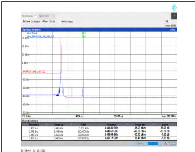
1-N78-3450-3550--30-30-L-1-DFT-PI2BPSK-Edge_1R_B_Left-1@0-Ant1-1--PASS-see graph
