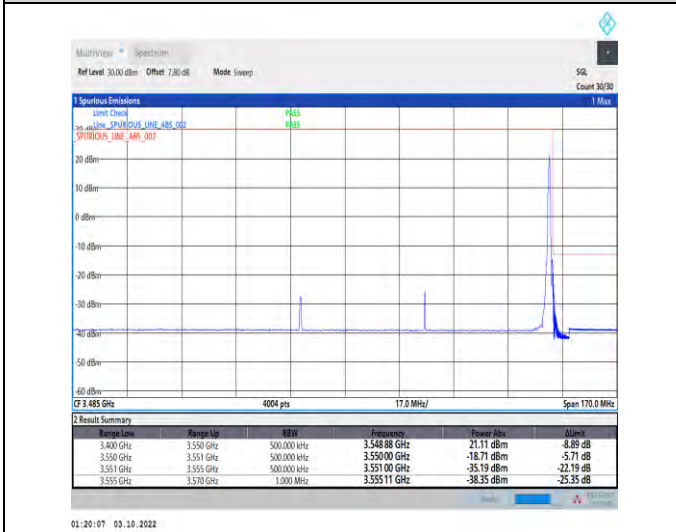
1-N78-3450-3550--30-80-H-5-CP-QPSK-Edge_1RB_R ight-1@216-Ant1-1--PASS-see graph
