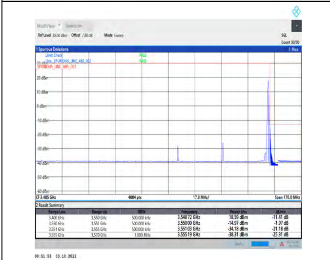
1-N78-3450-3550--30-60-H-5-CP-QPSK-Edge_1RB_Right-1@161-Ant1-1--PASS-see graph
