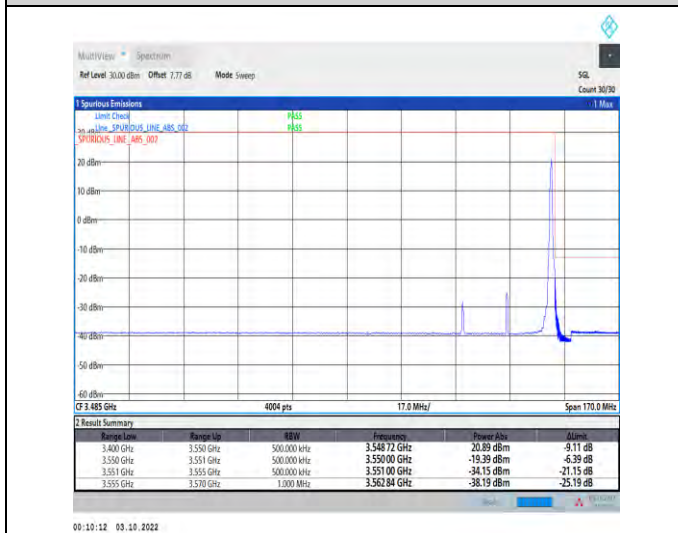
1-N78-3450-3550--30-30-H-5-CP-QPSK-Edge_1RB_R ight-1@77-Ant1-1--PASS-see graph
