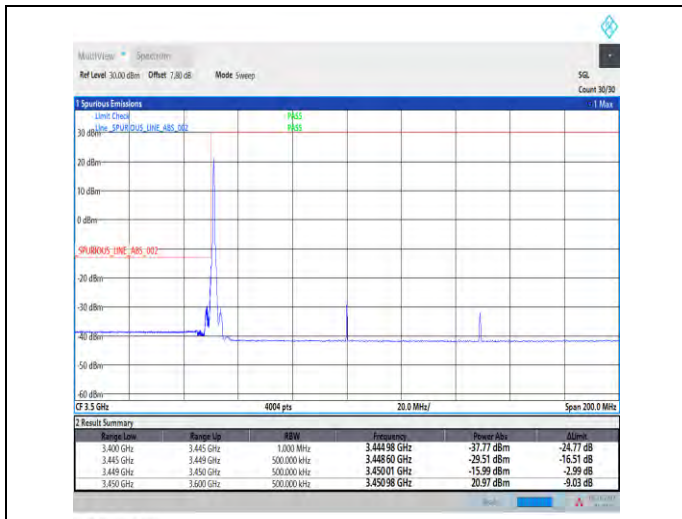
1-N78-3450-3550--30-100-L-1-DFT-PI2BPSK-Edge_1 RB_Left-1@0-Ant1-1--PASS-see graph
