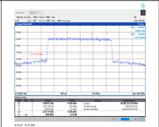
1-N78-3450-3550--30-100-M-3-DFT-16QAM-Outer_F ull-270@0-Ant1-96.003-99.800-<=100-PASS
