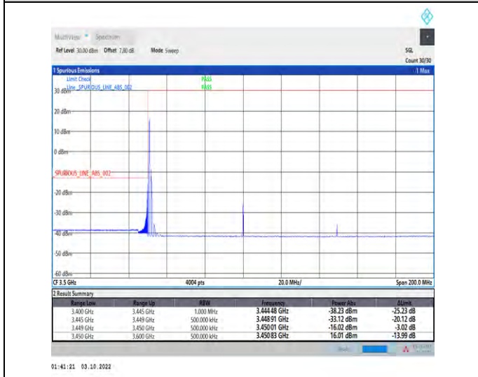
1-N78-3450-3550--30-100-L-4-CP-QPSK-Edge_1RB_Left-1@0-Ant1-1--PASS-see graph
