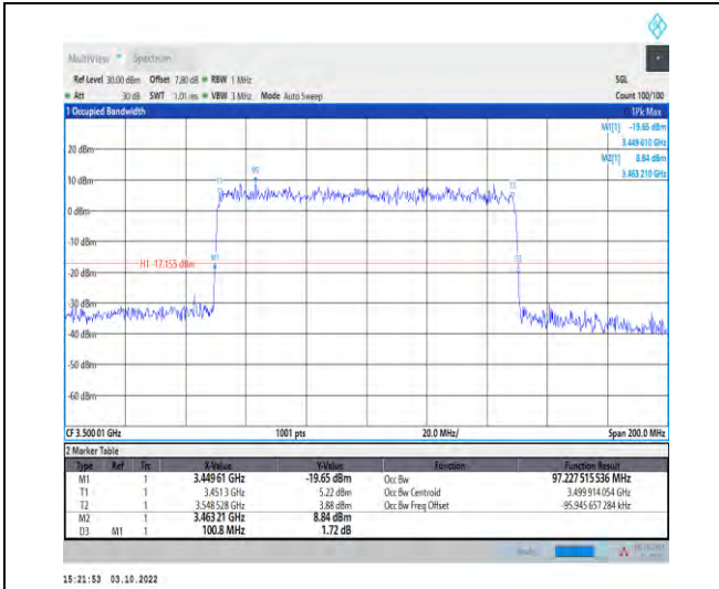
1-N78-3450-3550--30-100-L-9-CP-256QAM-Outer_F ull-273@0-Ant1-97.228-100.800-<=100-PASS
