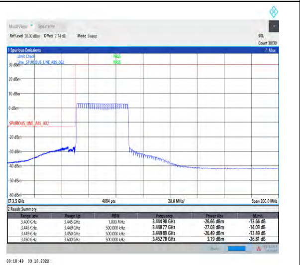
1-N78-3450-3550--30-40-L-6-CP-QPSK-Outer_Full-106@0-Ant1-1--PASS-see graph
