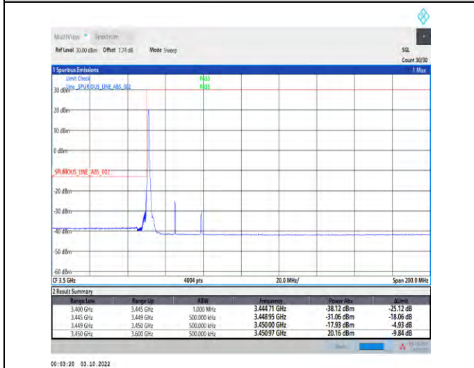
1-N78-3450-3550--30-30-L-4-CP-QPSK-Edge_1RB_Left-1@0-Ant1-1--PASS-see graph
