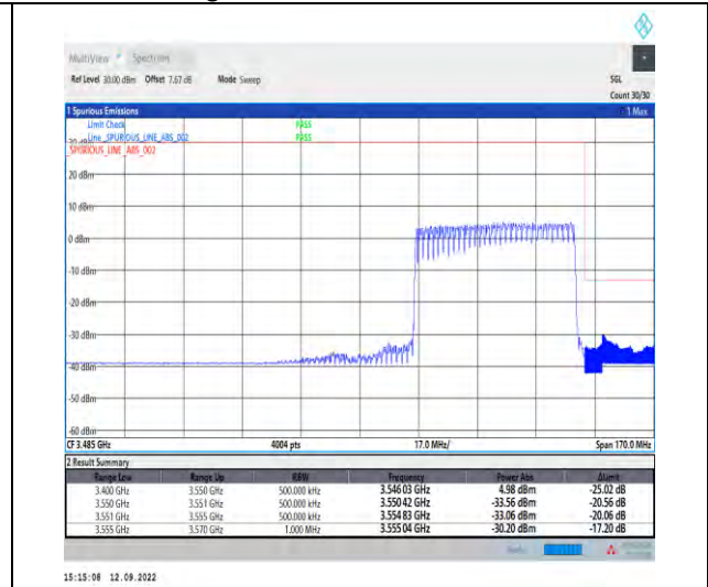
1-N78-3450-3550--30-50-H-3-DFT-PI2BPSK-Outer_Full-128@0-Ant1-1--PASS-see graph
