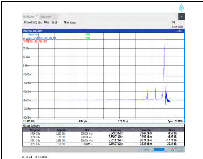
1-N78-3450-3550--30-20-H-2-DFT-PI2BPSK-Edge_1R_B_Right-1@50-Ant1-1--PASS-see graph
