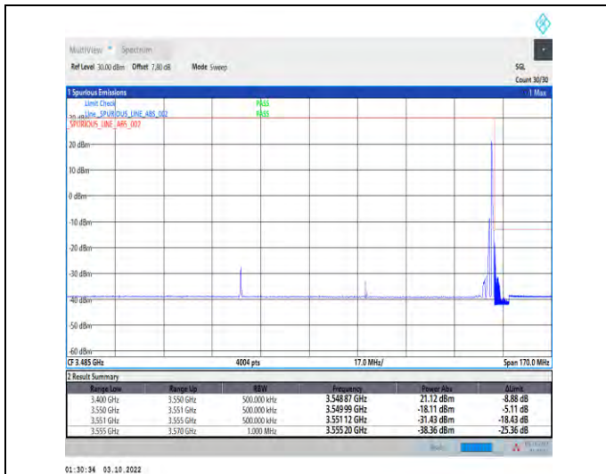
1-N78-3450-3550--30-90-H-2-DFT-PI2BPSK-Edge_1R_B_Right-1@244-Ant1-1--PASS-see graph
