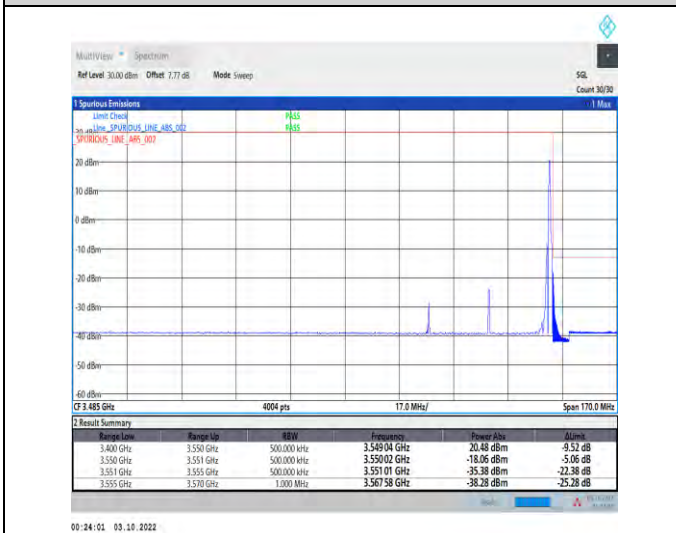
1-N78-3450-3550--30-40-H-5-CP-QPSK-Edge_1RB_Right-1@105-Ant1-1--PASS-see graph
