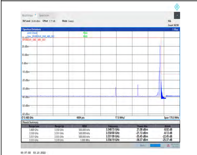
1-N78-3450-3550--30-50-H-5-CP-QPSK-Edge_1RB_Right-1@132-Ant1-1--PASS-see graph
