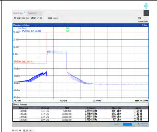
1-N78-3450-3550--30-30-L-6-CP-QPSK-Outer_Full-78@0-Ant1-1--PASS-see graph
