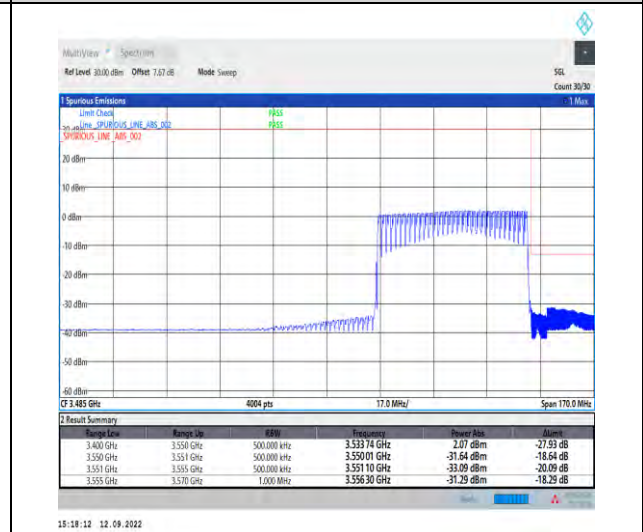
1-N78-3450-3550--30-50-H-6-CP-QPSK-Outer_Full-133@0-Ant1-1--PASS-see graph
