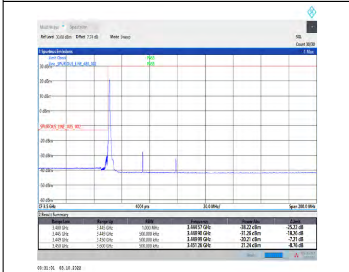
1-N78-3450-3550--30-50-L-4-CP-QPSK-Edge_1RB_Left-1@0-Ant1-1--PASS-see graph
