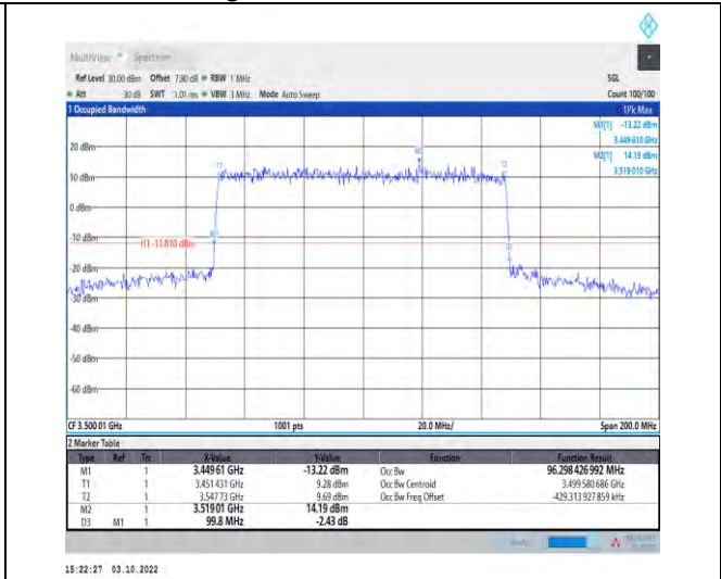
1-N78-3450-3550--30-100-M-1-DFT-QPSK-Outer_Fu ll-270@0-Ant1-96.298-99.800-<=100-PASS
