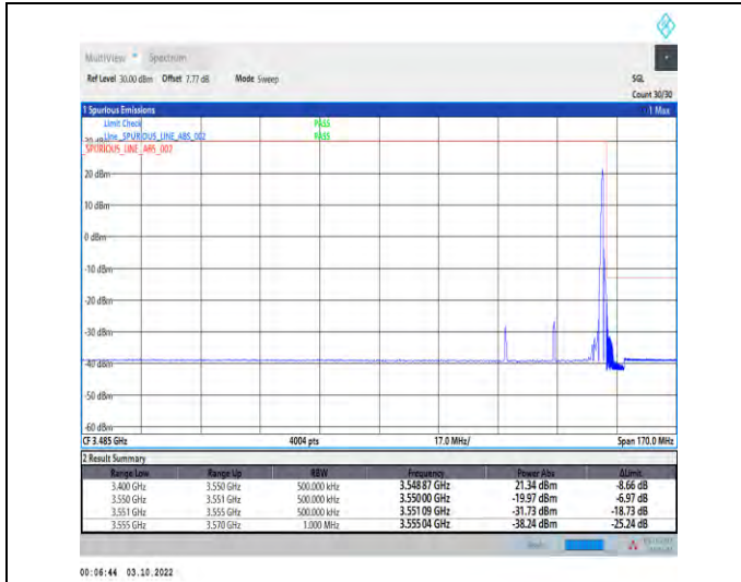
1-N78-3450-3550--30-30-H-2-DFT-PI2BPSK-Edge_1R_B_Right-1@77-Ant1-1--PASS-see graph
