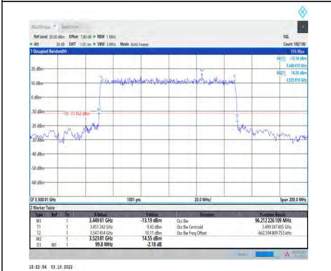
1-N78-3450-3550--30-100-M-2-DFT-PI2BPSK-Outer _Full-270@0-Ant1-96.212-99.800-<=100-PASS
