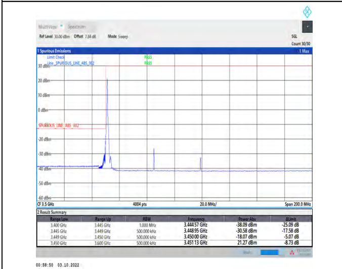
1-N78-3450-3550--30-70-L-4-CP-QPSK-Edge_1RB_Left-1@0-Ant1-1--PASS-see graph
