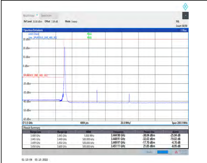
1-N78-3450-3550--30-80-L-4-CP-QPSK-Edge_1RB_Left-1@0-Ant1-1--PASS-see graph
