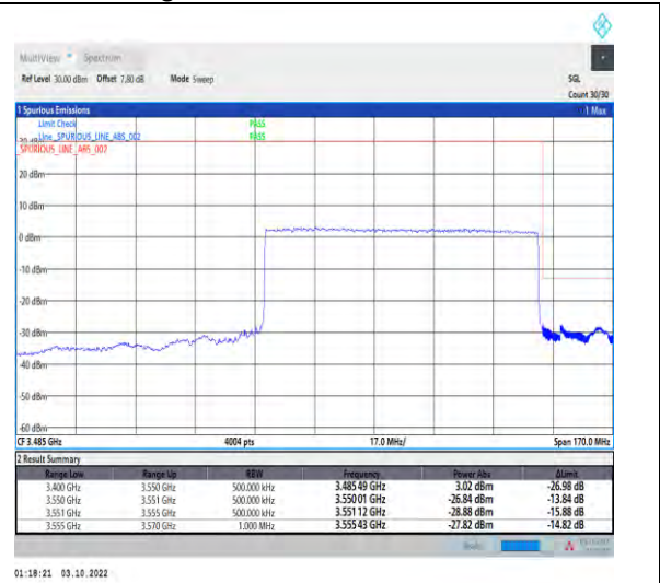
1-N78-3450-3550--30-80-H-3-DFT-PI2BPSK-Outer_Full-216@0-Ant1-1--PASS-see graph
