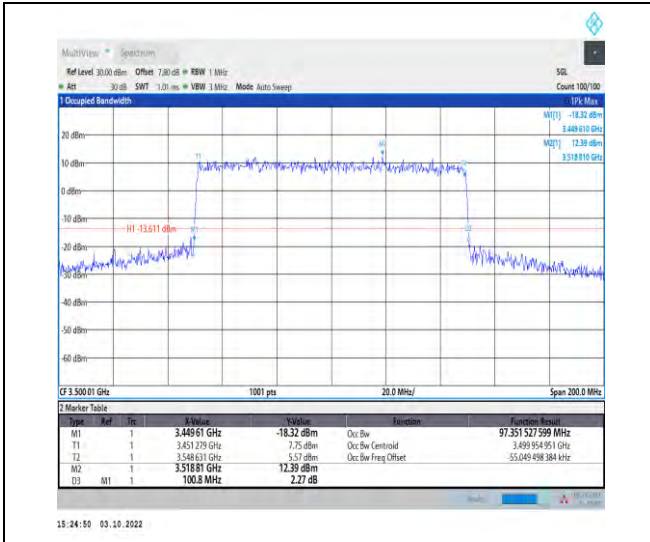
1-N78-3450-3550--30-100-M-8-CP-64QAM-Outer_Full-273@0-Ant1-97.352-100.800-≤100-PASS
