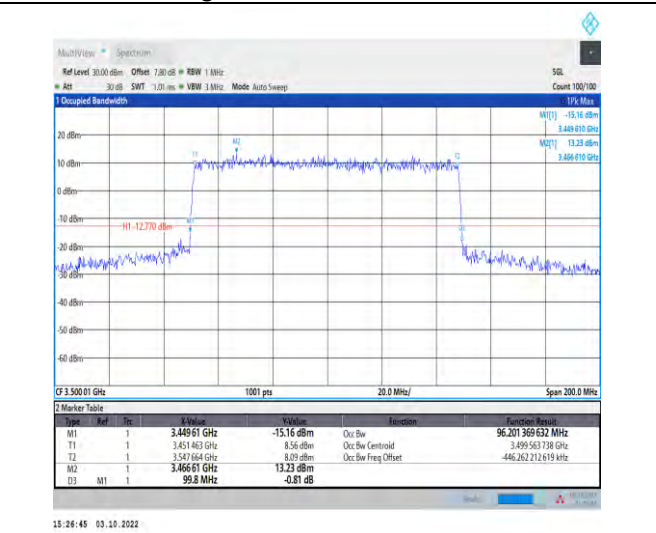
1-N78-3450-3550--30-100-H-4-DFT-64QAM-Outer_Full-270@0-Ant1-96.201-99.800-≤100-PASS
