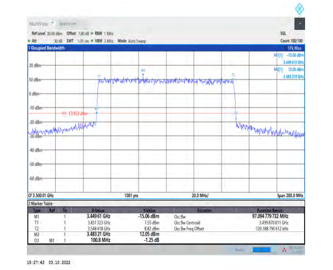
1-N78-3450-3550--30-100-H-6-CP-QPSK-Outer_Full-273@0-Ant1-97.095-100.800-≤100-PASS
