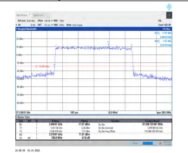
1-N78-3450-3550--30-100-H-8-CP-64QAM-Outer_Full-273@0-Ant1-97.039-100.800-≤100-PASS
