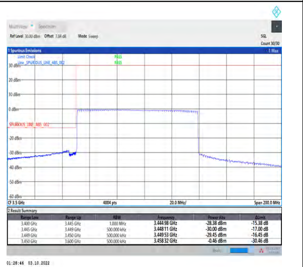
1-N78-3450-3550--30-90-L-6-CP-QPSK-Outer_Full-245@0-Ant1-1--PASS-see graph
