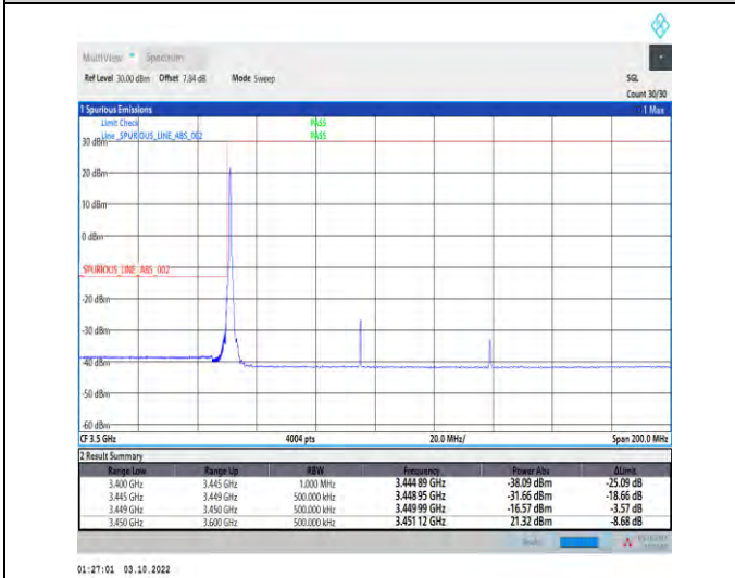
1-N78-3450-3550--30-90-L-4-CP-QPSK-Edge_1RB_Left-1@0-Ant1-1--PASS-see graph
