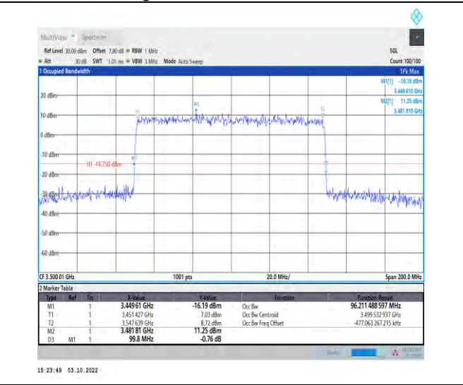
1-N78-3450-3550--30-100-M-5-DFT-256QAM-Outer_Full-270@0-Ant1-96.211-99.800-≤100-PASS
