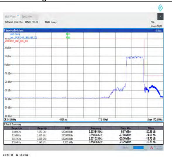
1-N78-3450-3550--30-20-H-3-DFT-PI2BPSK-Outer_Full-50@0-Ant1-1--PASS-see graph
