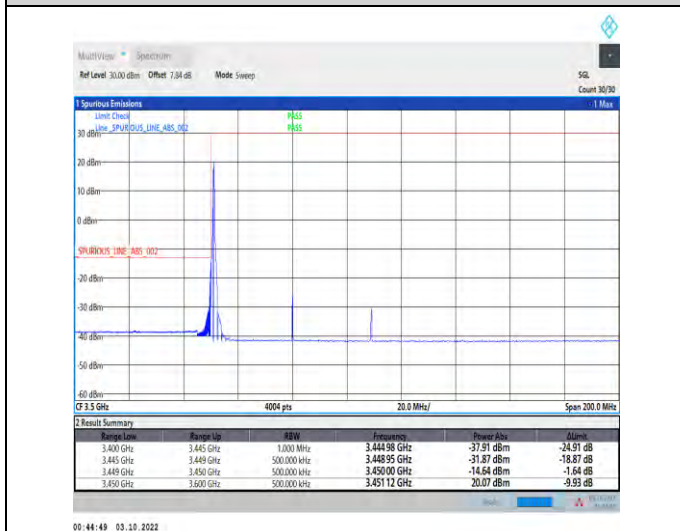
1-N78-3450-3550--30-60-L-4-CP-QPSK-Edge_1RB_Left-1@0-Ant1-1--PASS-see graph
