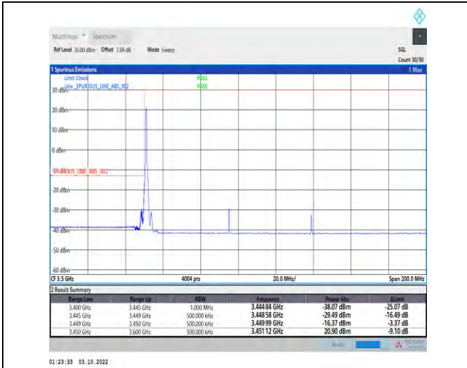
1-N78-3450-3550--30-90-L-1-DFT-PI2BPSK-Edge_1R_B_Left-1@0-Ant1-1--PASS-see graph
