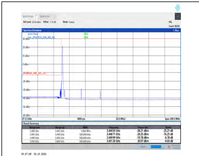
1-N78-3450-3550--30-50-L-1-DFT-PI2BPSK-Edge_1R_B_Left-1@0-Ant1-1--PASS-see graph
