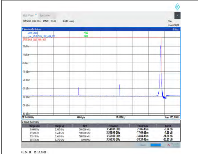
1-N78-3450-3550--30-90-H-5-CP-QPSK-Edge_1RB_Right-1@244-Ant1-1--PASS-see graph
