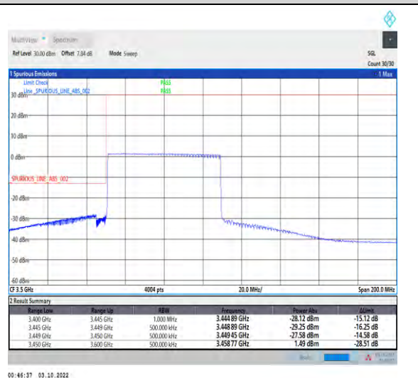
1-N78-3450-3550--30-60-L-6-CP-QPSK-Outer_Full-162@0-Ant1-1--PASS-see graph
