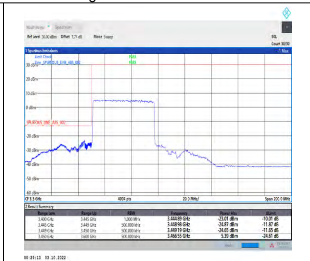
1-N78-3450-3550--30-50-L-3-DFT-PI2BPSK-Outer_Full-128@0-Ant1-1--PASS-see graph
