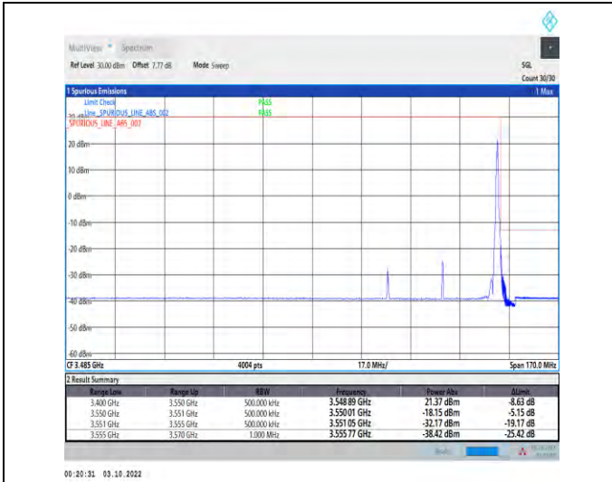
1-N78-3450-3550--30-40-H-2-DFT-PI2BPSK-Edge_1R_B_Right-1@105-Ant1-1--PASS-see graph
