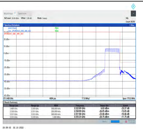
1-N78-3450-3550--30-20-H-6-CP-QPSK-Outer_Ful l-51@0-Ant1-1--PASS-see graph
