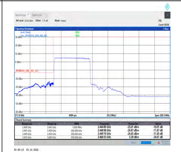
1-N78-3450-3550--30-50-L-6-CP-QPSK-Outer_Full-133@0-Ant1-1--PASS-see graph
