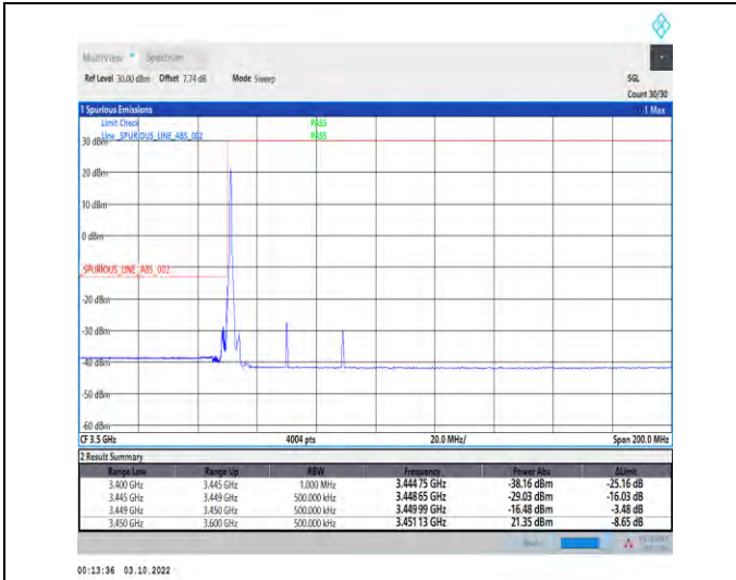
1-N78-3450-3550--30-40-L-1-DFT-PI2BPSK-Edge_1R_B_Left-1@0-Ant1-1--PASS-see graph
