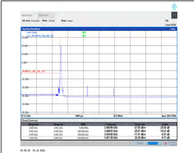
1-N78-3450-3550--30-70-L-1-DFT-PI2BPSK-Edge_1R_B_Left-1@0-Ant1-1--PASS-see graph
