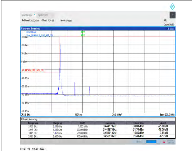
1-N78-3450-3550--30-40-L-4-CP-QPSK-Edge_1RB_Left-1@0-Ant1-1--PASS-see graph
