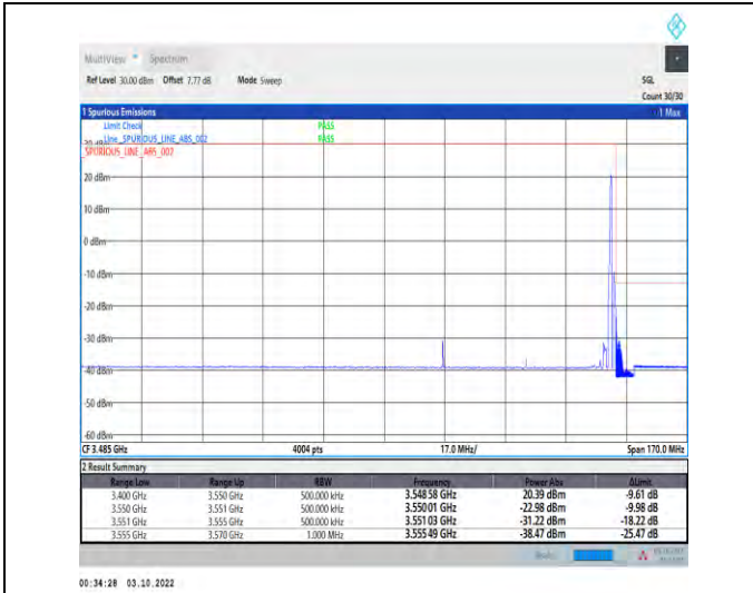
1-N78-3450-3550--30-50-H-2-DFT-PI2BPSK-Edge_1R_B_Right-1@132-Ant1-1--PASS-see graph
