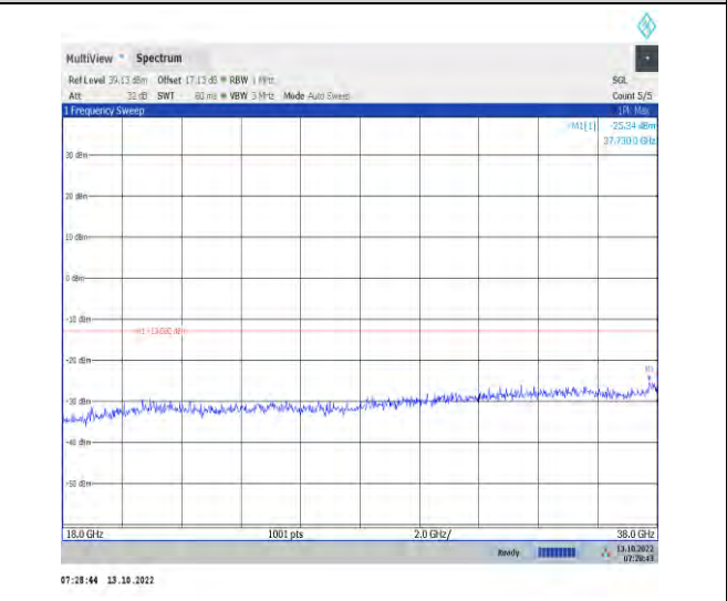
1-N78-3450-3550-PC2-30-100-M-1-DFT-PI2BPSK-In ner_1RB_Left-1@1-18000-40000-Ant1-18000.00--59 .62--13-PASS
