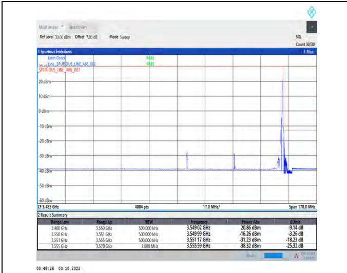
1-N78-3450-3550--30-60-H-2-DFT-PI2BPSK-Edge_1R_B_Right-1@161-Ant1-1--PASS-see graph
