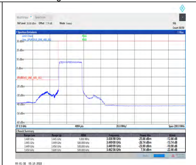
1-N78-3450-3550--30-30-L-3-DFT-PI2BPSK-Outer_Full-75@0-Ant1-1--PASS-see graph
