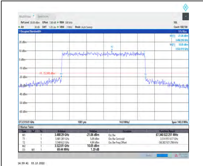
1-N78-3450-3550--30-70-H-8-CP-64QAM-Outer_Full -189@0-Ant1-67.34-69.440-≤70-PASS
