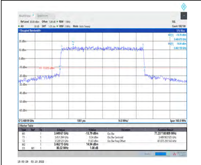
1-N78-3450-3550--30-80-L-1-DFT-QPSK-Outer_Full -216@0-Ant1-77.237-80.320-≤80-PASS
