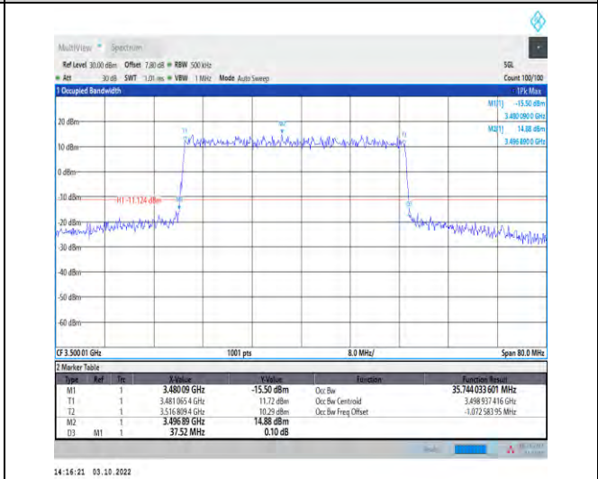
1-N78-3450-3550--30-40-M-1-DFT-QPSK-Outer_Full -100@0-Ant1-35.744-37.520-≤40-PASS
