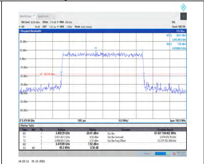
1-N78-3450-3550--30-50-L-9-CP-256QAM-Outer_Ful I-133@0-Ant1-47.431-49.300-≤50-PASS
