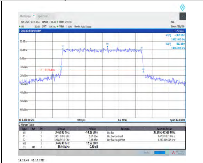
1-N78-3450-3550--30-40-L-8-CP-64QAM-Outer_Full 106@0-Ant1-37.865-39.440-≤40-PASS
