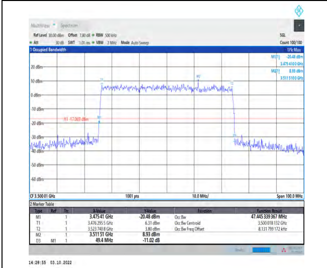
1-N78-3450-3550--30-50-M-9-CP-256QAM-Outer_Full ull-133@0-Ant1-47.445-49.400-≤50-PASS
