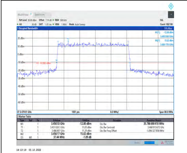
1-N78-3450-3550--30-40-L-1-DFT-QPSK-Outer_Full -100@0-Ant1-35.787-37.440-≤40-PASS
