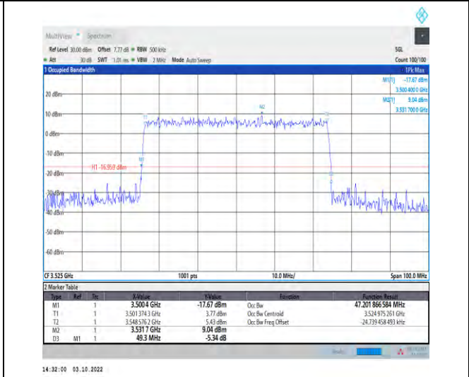
1-N78-3450-3550--30-50-H-9-CP-256QAM-Outer_Fu ll-133@0-Ant1-47.202-49.300-<math>\leq 50</math>-PASS
