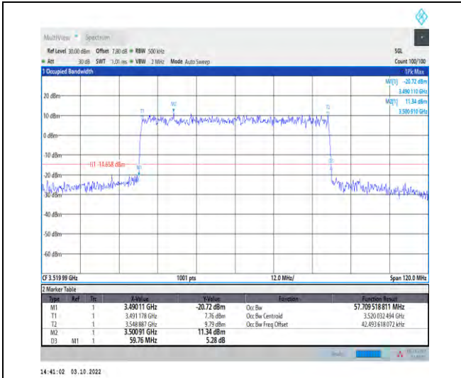
1-N78-3450-3550--30-60-H-7-CP-16QAM-Outer_Full -162@0-Ant1-57.71-59.760-≤60-PASS
