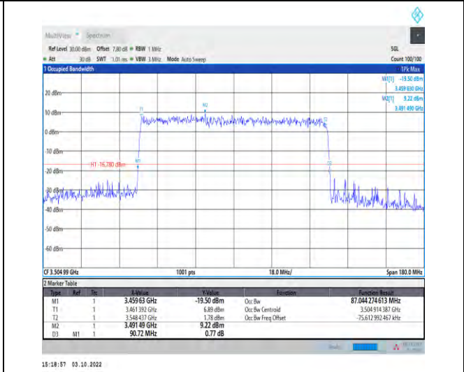
1-N78-3450-3550--30-90-H-9-CP-256QAM-Outer_Fu ll-245@0-Ant1-87.044-90.720-<math>\leq 90</math>-PASS
