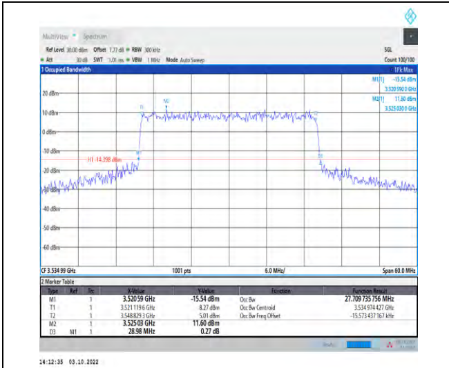
1-N78-3450-3550--30-30-H-8-CP-64QAM-Outer_Full -78@0-Ant1-27.71-28.980-≤30-PASS
