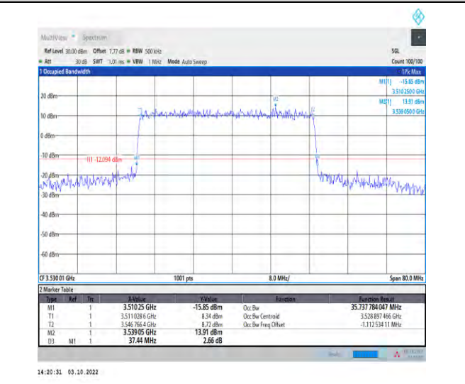
1-N78-3450-3550--30-40-H-4-DFT-64QAM-Outer_Full -100@0-Ant1-35.738-37.440-≤40-PASS
