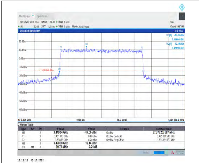
1-N78-3450-3550--30-90-L-8-CP-64QAM-Outer_Full -245@0-Ant1-87.376-90.720-≤90-PASS
