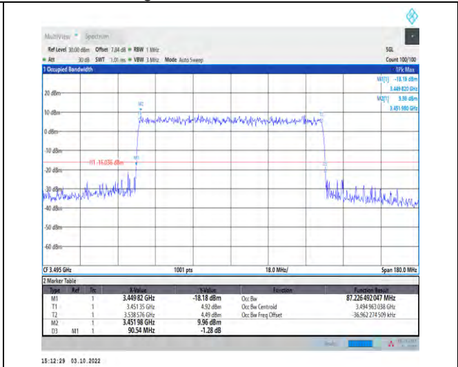
1-N78-3450-3550--30-90-L-9-CP-256QAM-Outer_Ful I-245@0-Ant1-87.226-90.540-≤90-PASS
