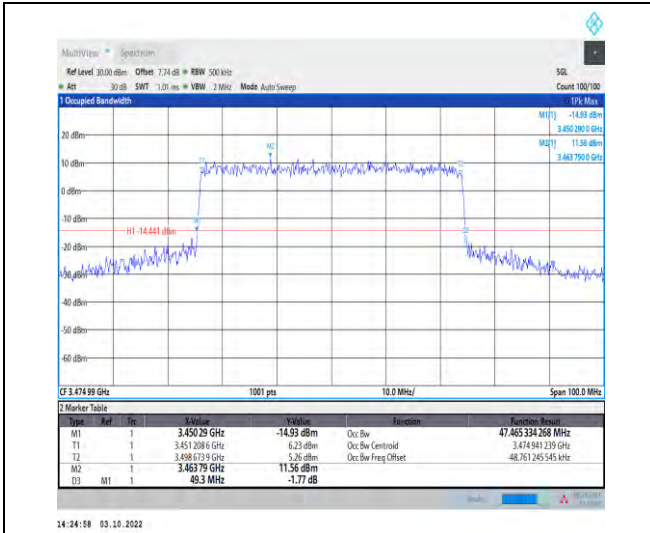
1-N78-3450-3550--30-50-L-8-CP-64QAM-Outer_Full -133@0-Ant1-47.465-49.300-≤50-PASS
