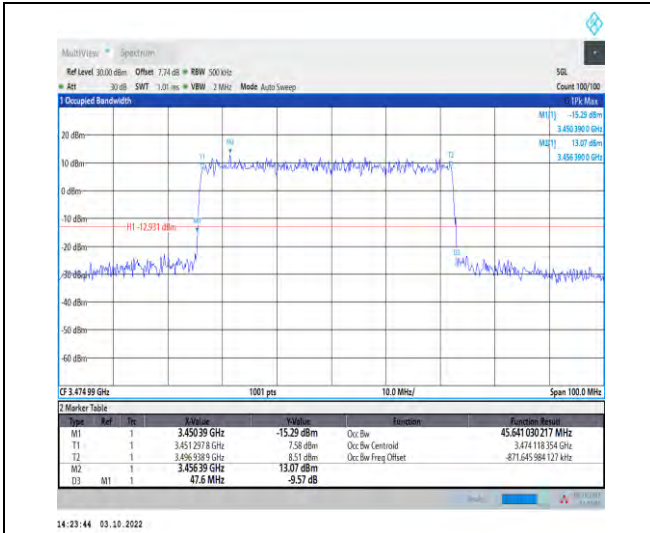
1-N78-3450-3550--30-50-L-4-DFT-64QAM-Outer_Fu II-128@0-Ant1-45.641-47.600-<math>\leq 50</math>-PASS
