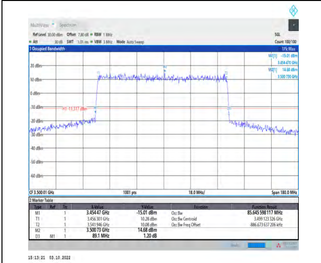
1-N78-3450-3550--30-90-M-1-DFT-QPSK-Outer_Full -240@0-Ant1-85.646-89.100-≤90-PASS
