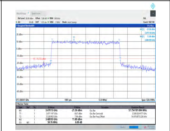
1-N78-3450-3550--30-60-M-1-DFT-QPSK-Outer_Full -162@0-Ant1-57.74-59.760-≤60-PASS
