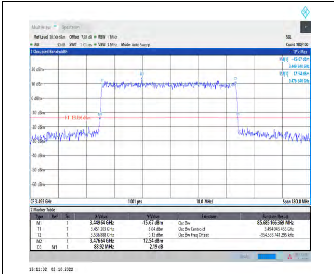
1-N78-3450-3550--30-90-L-4-DFT-64QAM-Outer_Fu II-240@0-Ant1-85.685-88.920-≤90-PASS
