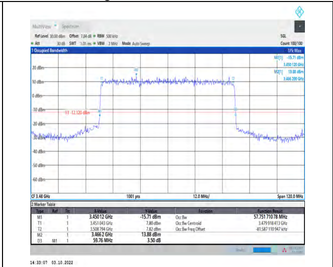
1-N78-3450-3550--30-60-L-2-DFT-PI2BPSK-Outer_Full -162@0-Ant1-57.752-59.760-≤60-PASS
