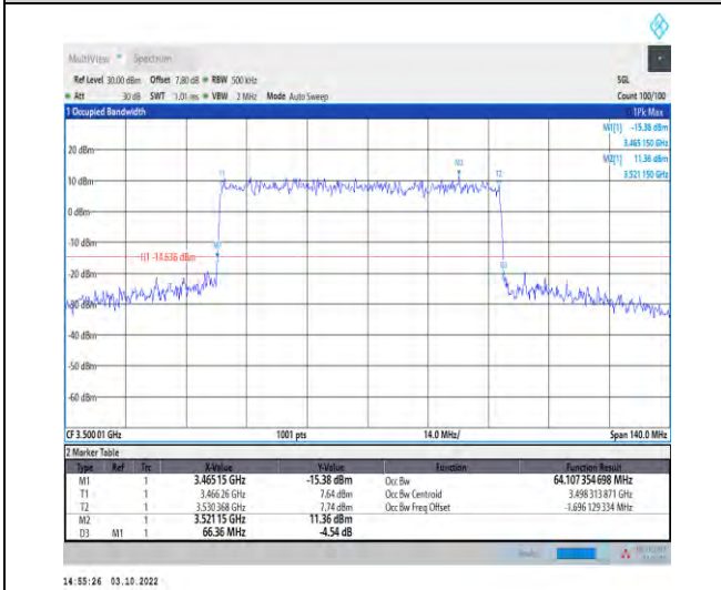
1-N78-3450-3550--30-70-M-3-DFT-16QAM-Outer_Full -180@0-Ant1-64.107-66.360-≤70-PASS
