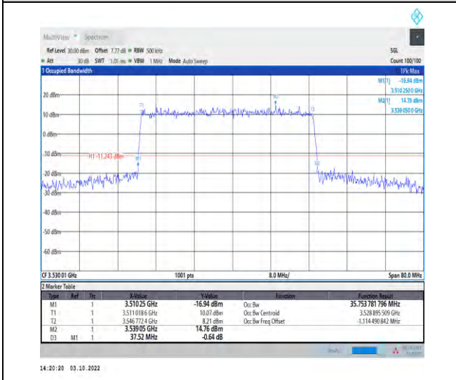
1-N78-3450-3550--30-40-H-3-DFT-16QAM-Outer_Full -100@0-Ant1-35.754-37.520-≤40-PASS
