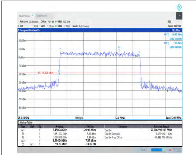
1-N78-3450-3550--30-60-L-9-CP-256QAM-Outer_Fu II-162@0-Ant1-57.707-59.760-≤60-PASS
