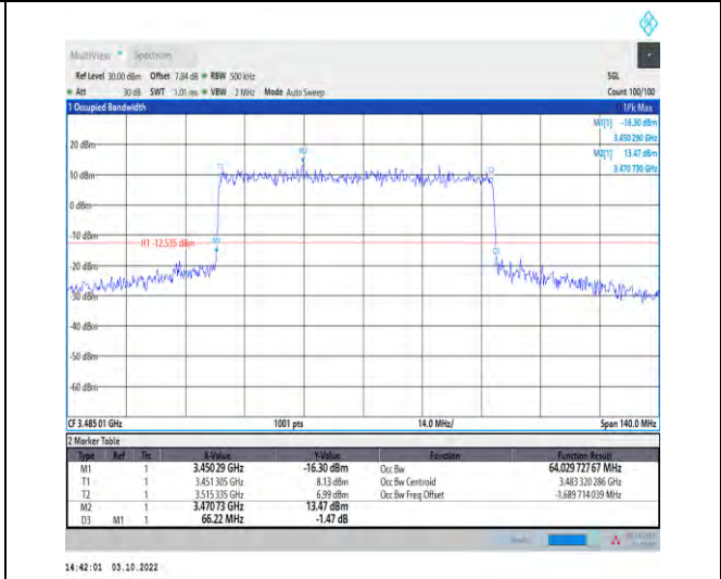
1-N78-3450-3550--30-70-L-1-DFT-QPSK-Outer_Full -180@0-Ant1-64.03-66.220-≤70-PASS
