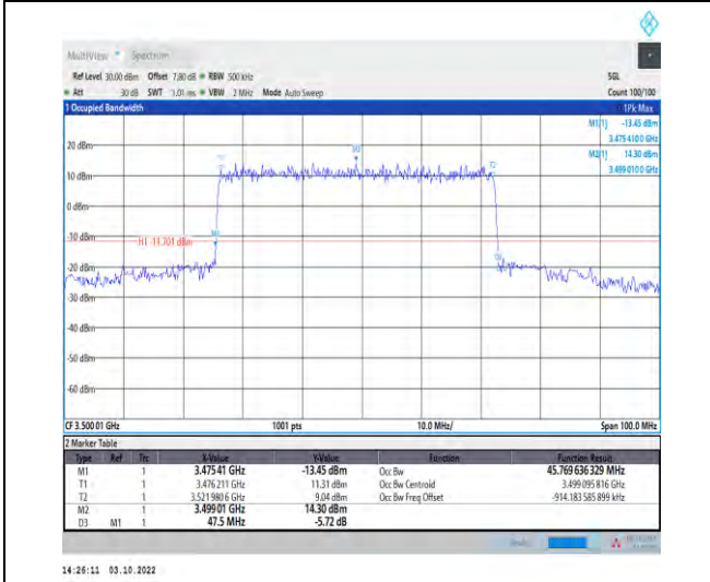
1-N78-3450-3550--30-50-M-1-DFT-QPSK-Outer_Full -128@0-Ant1-45.77-47.500-≤50-PASS
