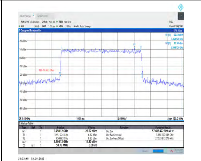
1-N78-3450-3550--30-60-L-4-DFT-64QAM-Outer_Full -162@0-Ant1-57.606-59.760-≤60-PASS
