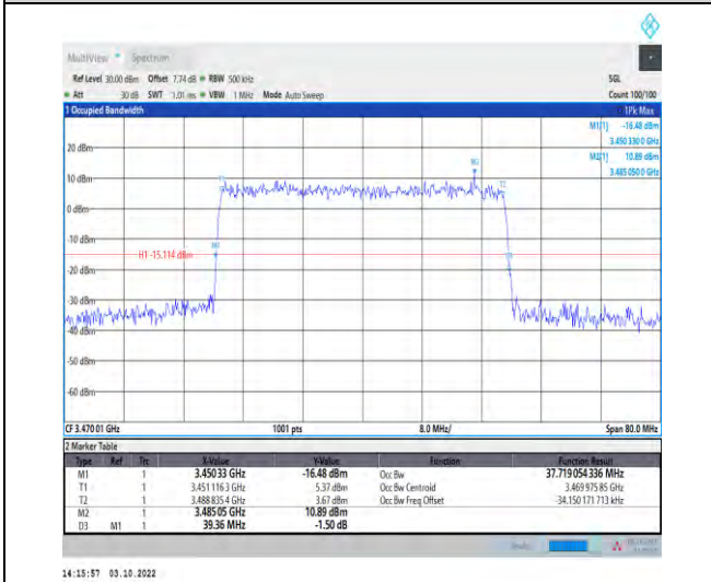
1-N78-3450-3550--30-40-L-9-CP-256QAM-Outer_Fu II-106@0-Ant1-37.719-39.360-≤40-PASS
