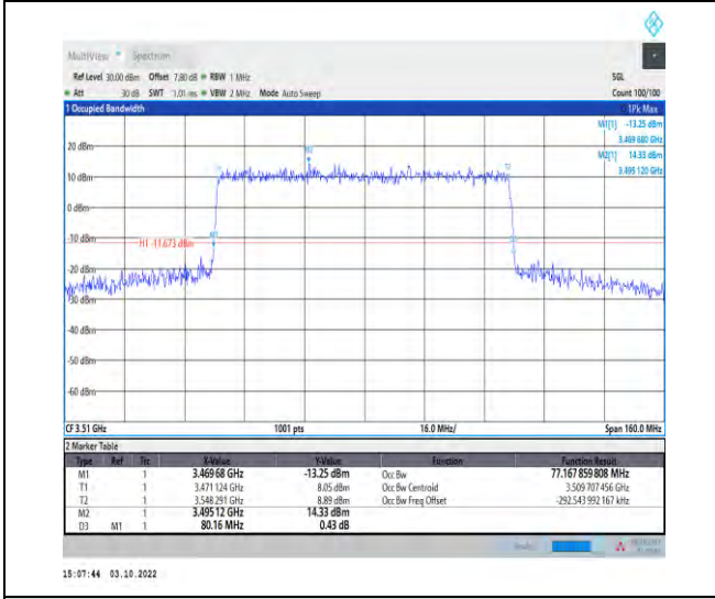
1-N78-3450-3550--30-80-H-3-DFT-16QAM-Outer_Full -216@0-Ant1-77.168-80.160-≤80-PASS
