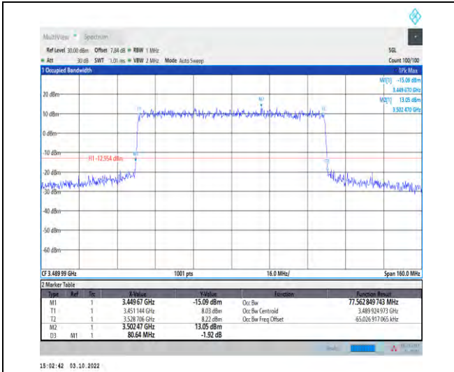
1-N78-3450-3550--30-80-L-7-CP-16QAM-Outer_Full -217@0-Ant1-77.563-80.640-≤80-PASS
