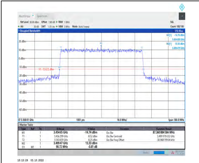
1-N78-3450-3550--30-90-M-7-CP-16QAM-Outer_Full I-245@0-Ant1-87.361-90.720-≤90-PASS
