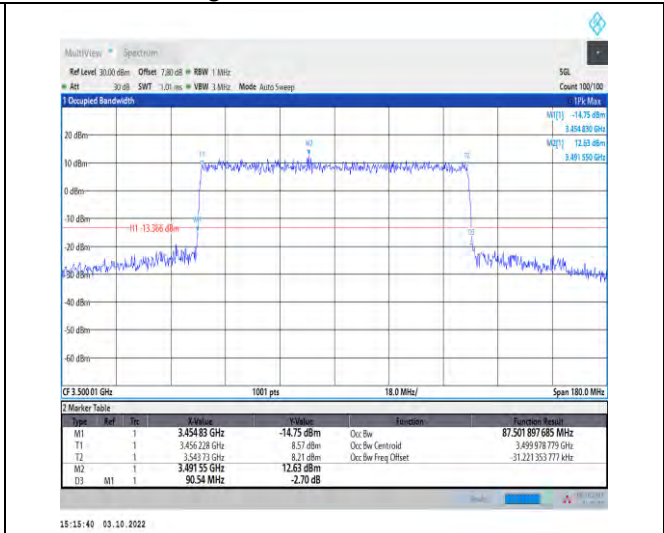
1-N78-3450-3550--30-90-M-8-CP-64QAM-Outer_Full -245@0-Ant1-87.502-90.540-≤90-PASS
