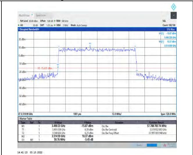
1-N78-3450-3550--30-60-H-8-CP-64QAM-Outer_Full -162@0-Ant1-57.789-59.760-≤60-PASS
