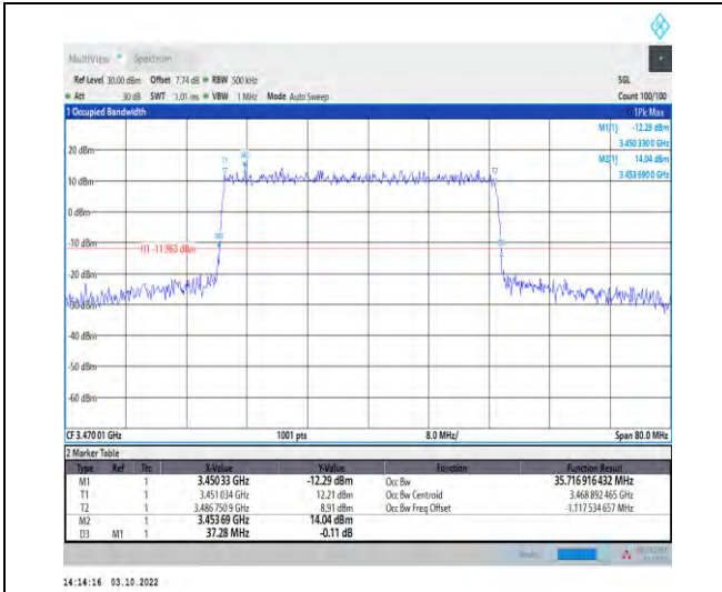
1-N78-3450-3550--30-40-L-3-DFT-16QAM-Outer_Fu II-100@0-Ant1-35.717-37.280-≤40-PASS
