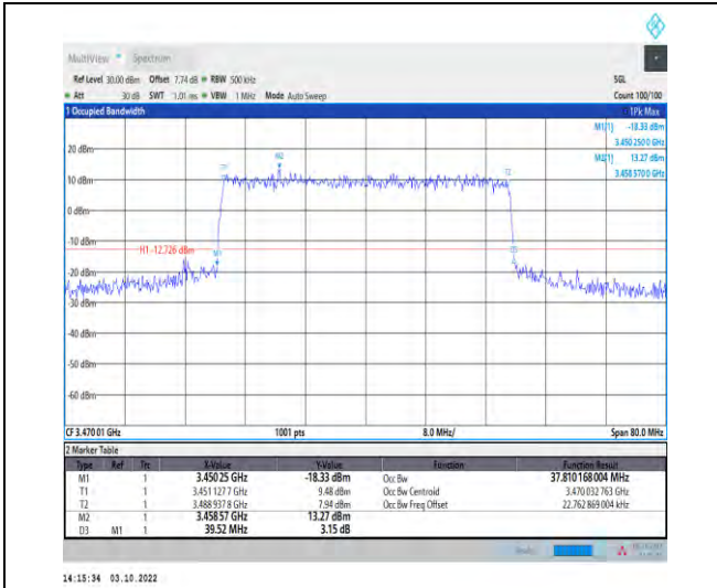
1-N78-3450-3550--30-40-L-7-CP-16QAM-Outer_Full -106@0-Ant1-37.81-39.520-≤40-PASS
