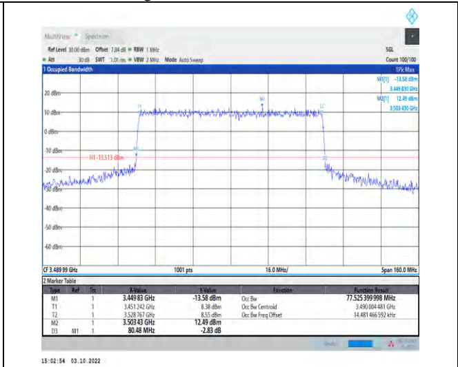
1-N78-3450-3550--30-80-L-8-CP-64QAM-Outer_Full 217@0-Ant1-77.525-80.480-≤80-PASS
