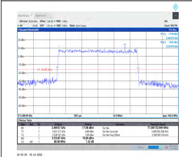
1-N78-3450-3550--30-80-L-9-CP-256QAM-Outer_Fu ll-217@0-Ant1-77.55-80.480-≤80-PASS
