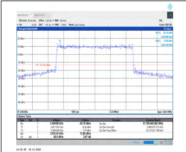
1-N78-3450-3550--30-60-L-1-DFT-QPSK-Outer_Full -162@0-Ant1-57.786-60.000-≤60-PASS
