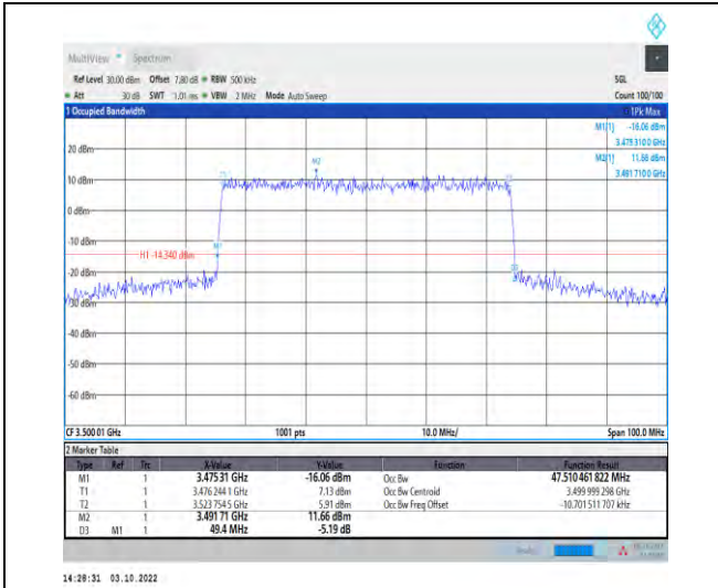
1-N78-3450-3550--30-50-M-7-CP-16QAM-Outer_Full I-133@0-Ant1-47.51-49.400-≤50-PASS
