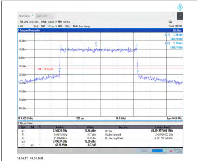
1-N78-3450-3550--30-70-M-1-DFT-QPSK-Outer_Full -180@0-Ant1-64.495-66.360-≤70-PASS
