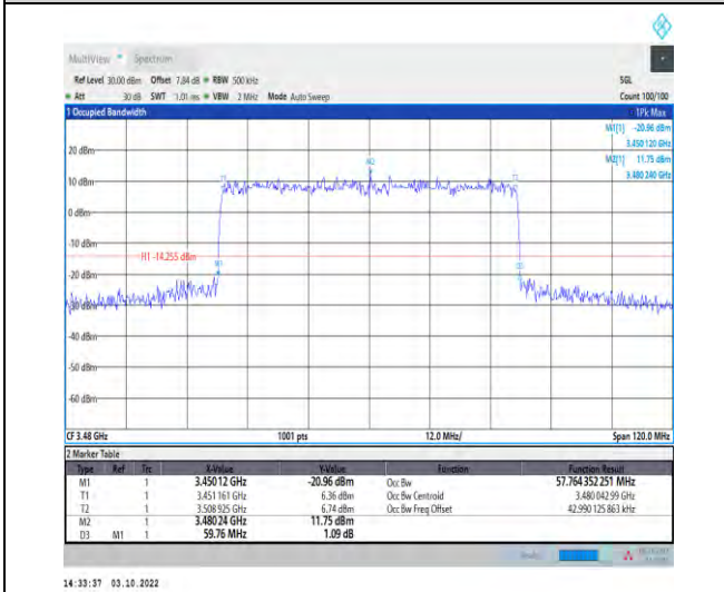
1-N78-3450-3550--30-60-L-3-DFT-16QAM-Outer_Full -162@0-Ant1-57.764-59.760-≤60-PASS
