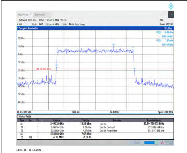
1-N78-3450-3550--30-60-H-9-CP-256QAM-Outer_Full -162@0-Ant1-57.644-59.760-≤60-PASS
