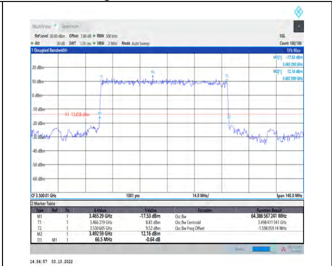
1-N78-3450-3550--30-70-M-2-DFT-PI2BPSK-Outer_Full -180@0-Ant1-64.387-66.500-≤70-PASS
