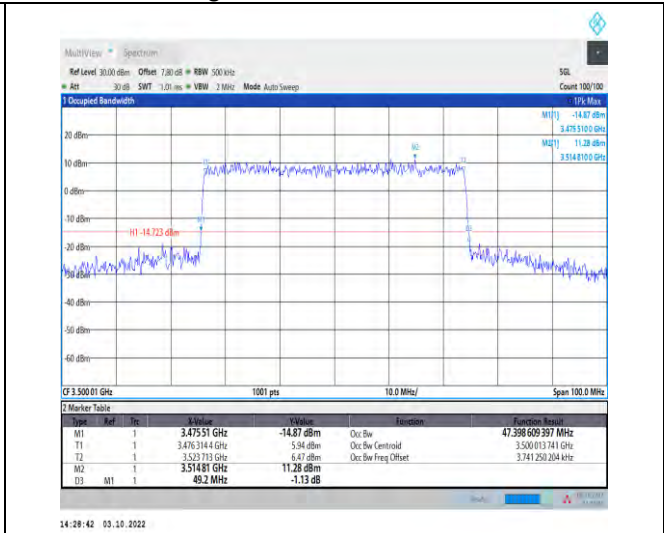
1-N78-3450-3550--30-50-M-8-CP-64QAM-Outer_Full -133@0-Ant1-47.399-49.200-≤50-PASS
