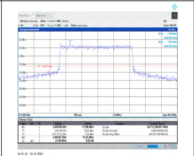
1-N78-3450-3550--30-30-L-1-DFT-QPSK-Outer_Full -75@0-Ant1-26.712-27.960-≤30-PASS
