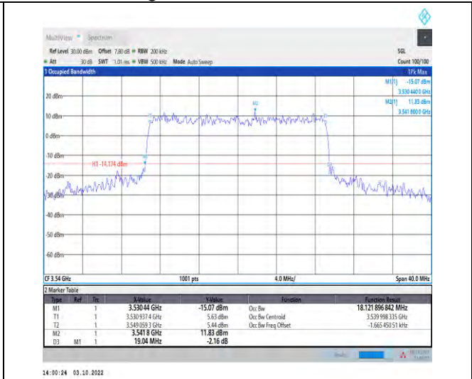
1-N78-3450-3550--30-20-H-8-CP-64QAM-Outer_Full -51@0-Ant1-18.122-19.040-≤20-PASS
