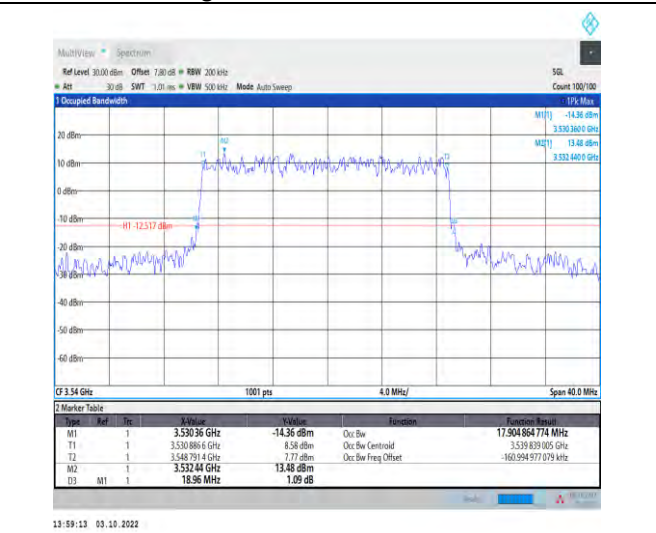
1-N78-3450-3550--30-20-H-4-DFT-64QAM-Outer_Full-50@0-Ant1-17.905-18.960-≤20-PASS
