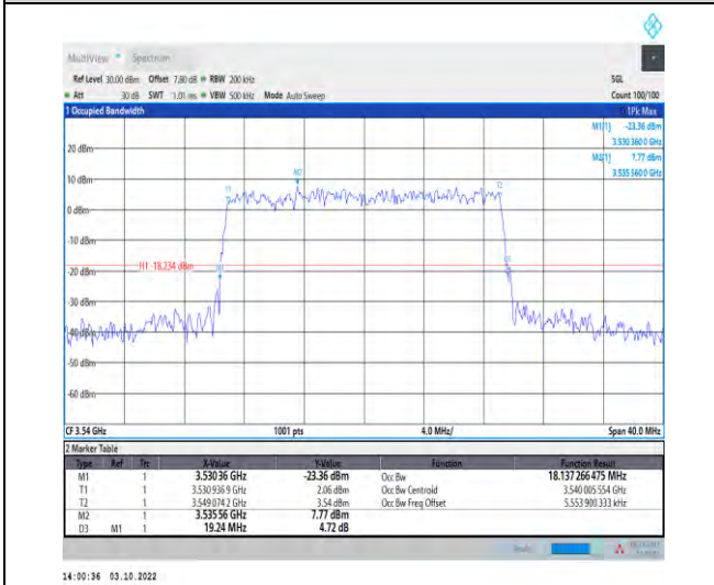
1-N78-3450-3550--30-20-H-9-CP-256QAM-Outer_Full -51@0-Ant1-18.137-19.240-≤20-PASS
