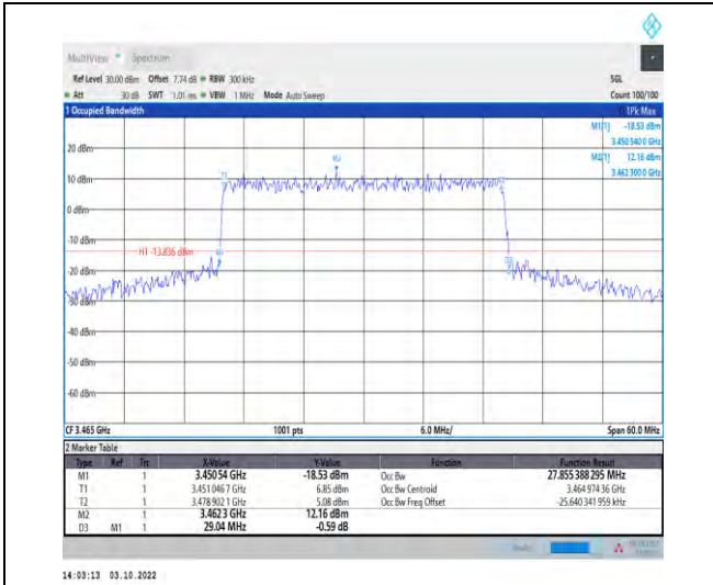
1-N78-3450-3550--30-30-L-6-CP-QPSK-Outer_Full-78@0-Ant1-27.855-29.040-≤30-PASS
