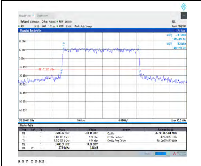
1-N78-3450-3550--30-30-M-3-DFT-16QAM-Outer_Full ull-75@0-Ant1-26.79-27.900-≤30-PASS
