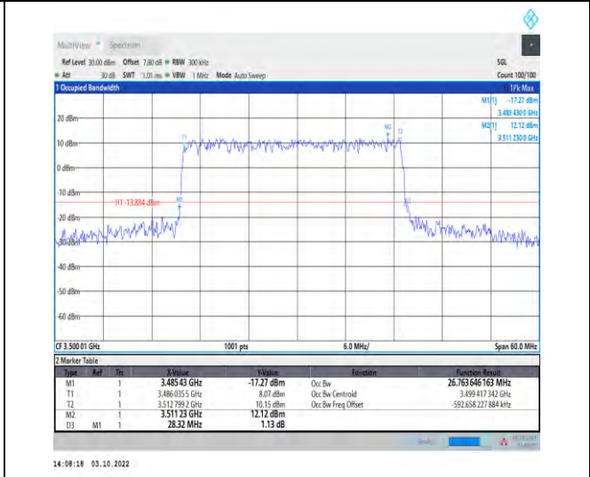
1-N78-3450-3550--30-30-M-4-DFT-64QAM-Outer_Full ll-75@0-Ant1-26.764-28.320-≤30-PASS
