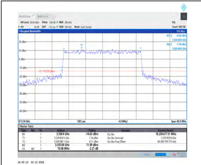
1-N78-3450-3550--30-20-H-7-CP-16QAM-Outer_Full -51@0-Ant1-18.251-19.080-≤20-PASS
