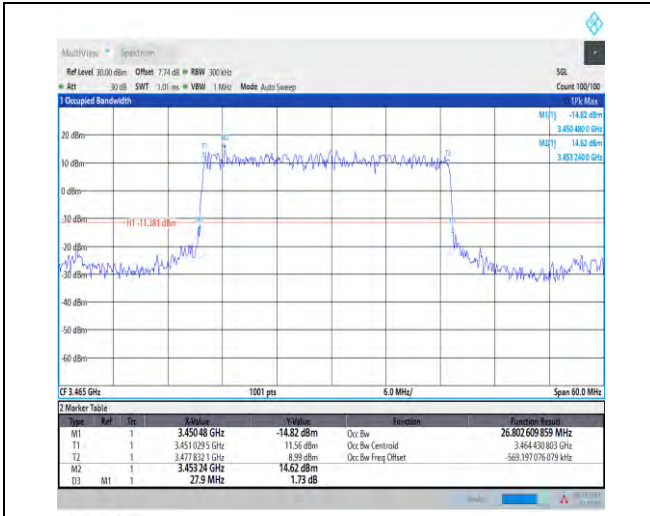
1-N78-3450-3550--30-30-L-2-DFT-PI2BPSK-Outer_Full-75@0-Ant1-26.803-27.900-≤30-PASS
