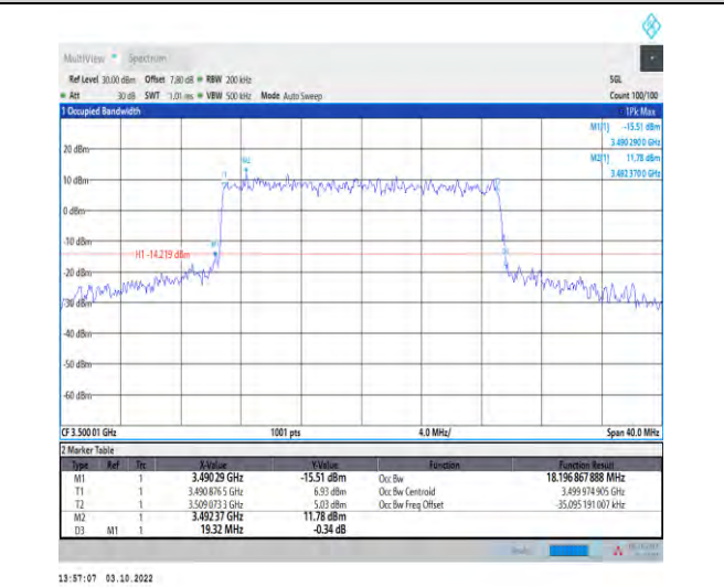
1-N78-3450-3550--30-20-M-7-CP-16QAM-Outer_Full-51@0-Ant1-18.197-19.320-≤20-PASS
