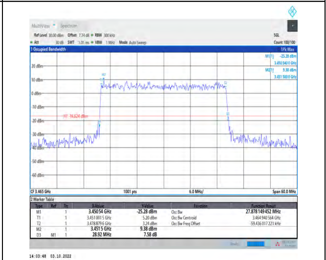
1-N78-3450-3550--30-30-L-9-CP-256QAM-Outer_Full-78@0-Ant1-27.878-28.920-≤30-PASS
