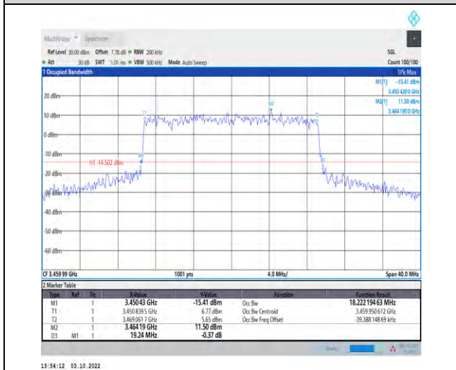
1-N78-3450-3550--30-20-L-7-CP-16QAM-Outer_Full-51@0-Ant1-18.222-19.240-<math>\leq 20</math>-PASS
