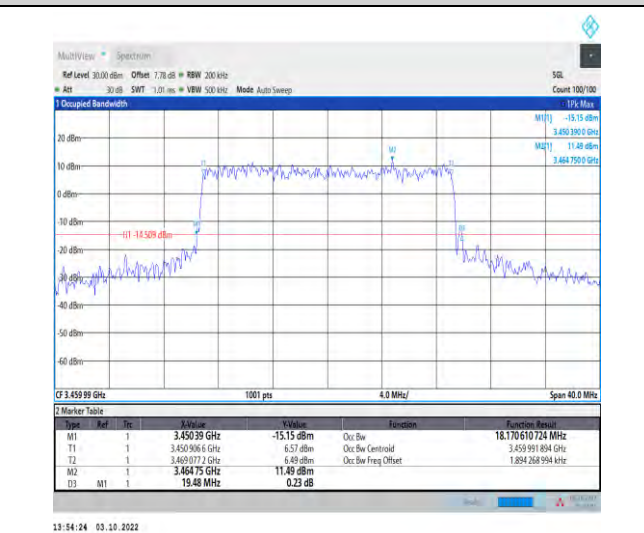
1-N78-3450-3550--30-20-L-8-CP-64QAM-Outer_Full-51@0-Ant1-18.171-19.480-<math>\leq 20</math>-PASS
