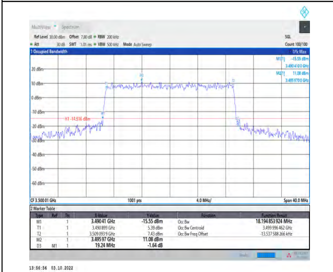
1-N78-3450-3550--30-20-M-6-CP-QPSK-Outer_Full-51@0-Ant1-18.195-19.240-≤20-PASS
