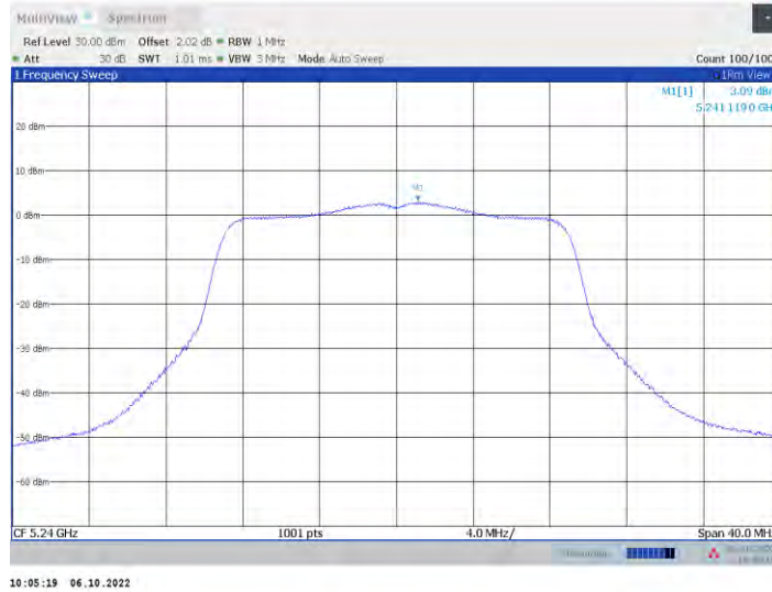
11n20MIMO Ant8 5240
