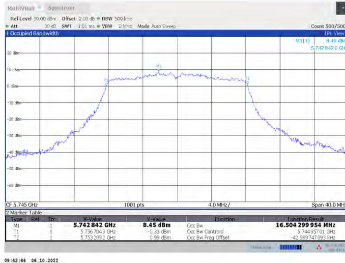
11a-CDD Ant8 5745
