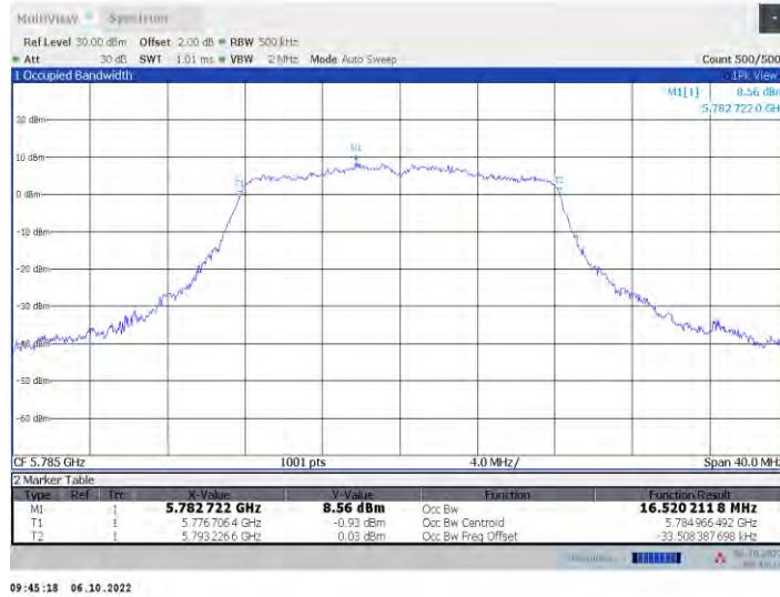
11a-CDD Ant8 5785
