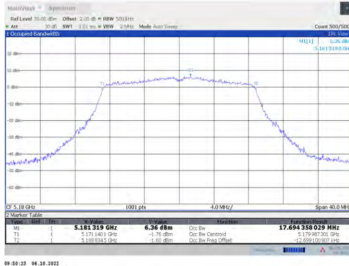
11n20MIMO Ant8 5180
