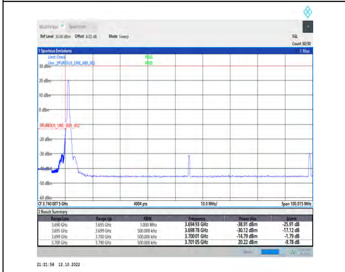
1-N77-3700-3980--30-90-L-4-CP-QPSK-Edge_1RB_Left-1@0-Ant1-1--PASS-see graph
