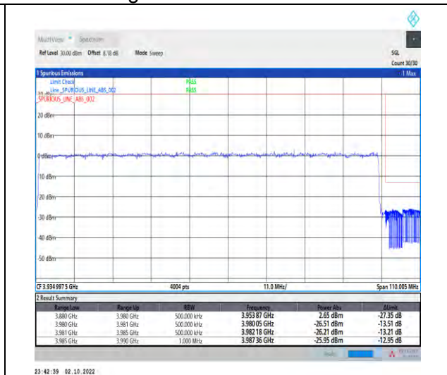
1-N77-3700-3980--30-100-H-3-DFT-PI2BPSK-Out er_Full-270@0-Ant1-1--PASS-see graph
