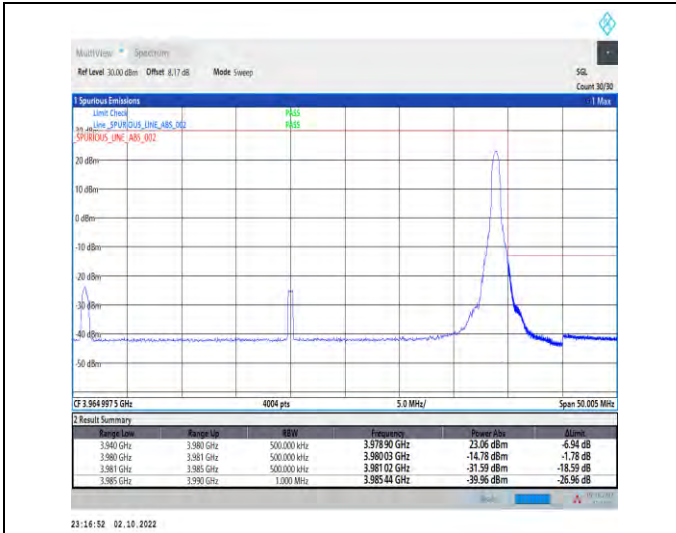
1-N77-3700-3980--30-40-H-2-DFT-PI2BPSK-Edge_1R_B_Right-1@105-Ant1-1--PASS-see graph
