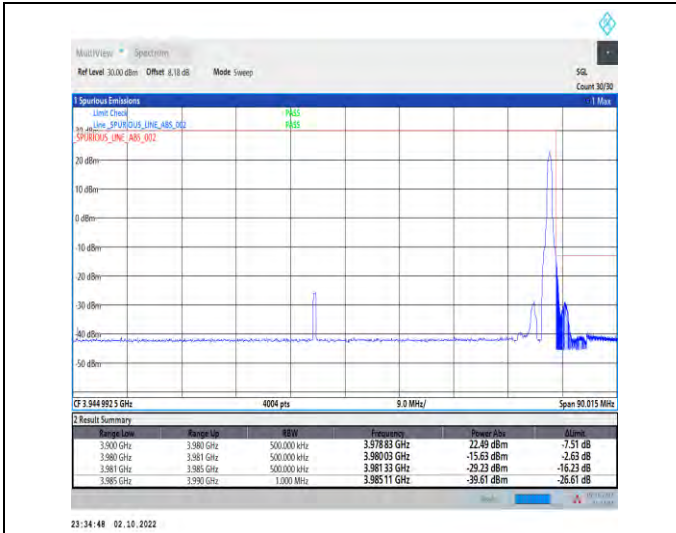
1-N77-3700-3980--30-80-H-2-DFT-PI2BPSK-Edge_1R_B_Right-1@216-Ant1-1--PASS-see graph
