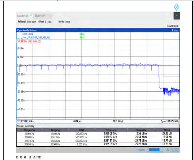
1-N77-3700-3980--30-90-H-3-DFT-PI2BPSK-Outer_Full-240@0-Ant1-1--PASS-see graph
