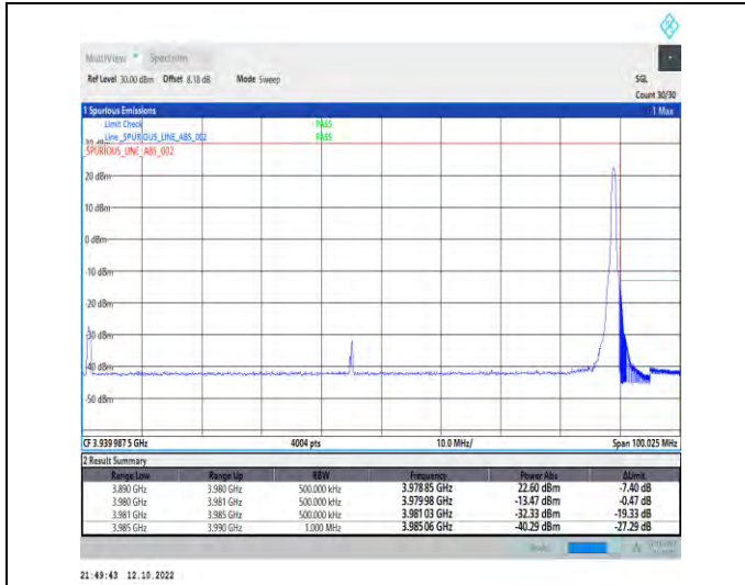
1-N77-3700-3980--30-90-H-2-DFT-PI2BPSK-Edge_1R_B_Right-1@244-Ant1-1--PASS-see graph
