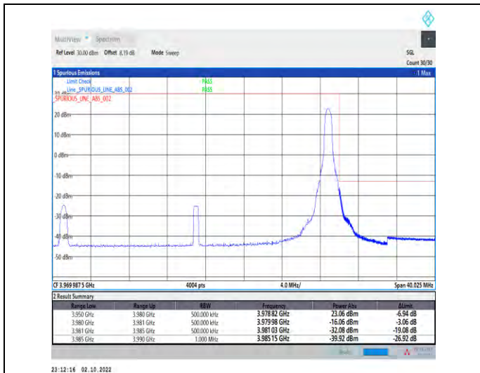
1-N77-3700-3980--30-30-H-2-DFT-PI2BPSK-Edge_1R_B_Right-1@77-Ant1-1--PASS-see graph
