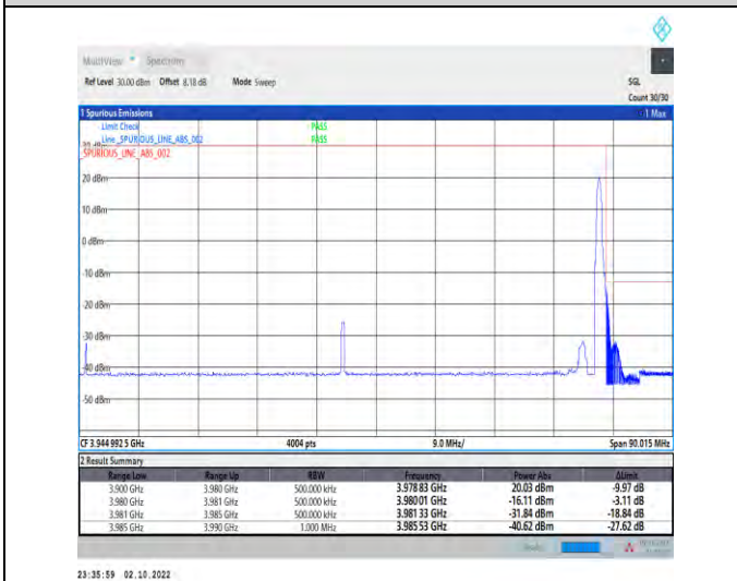
1-N77-3700-3980--30-80-H-5-CP-QPSK-Edge_1RB_R ight-1@216-Ant1-1--PASS-see graph
