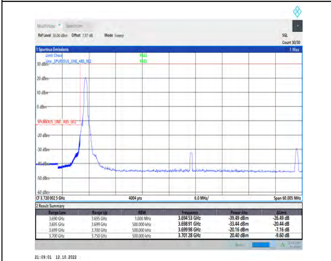
1-N77-3700-3980--30-50-L-4-CP-QPSK-Edge_1RB_Left-1@0-Ant1-1--PASS-see graph
