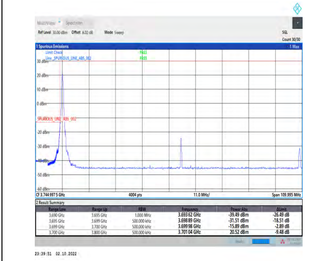
1-N77-3700-3980--30-100-L-4-CP-QPSK-Edge_1RB_Left-1@0-Ant1-1--PASS-see graph
