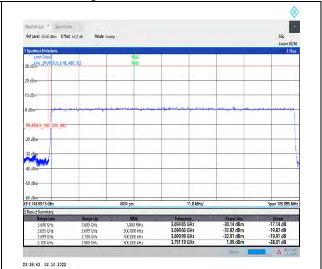
1-N77-3700-3980--30-100-L-3-DFT-PI2BPSK-Outer_Full-270@0-Ant1-1--PASS-see graph
