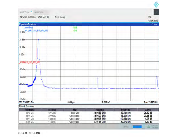
1-N77-3700-3980--30-70-L-4-CP-QPSK-Edge_1RB_Left-1@0-Ant1-1--PASS-see graph
