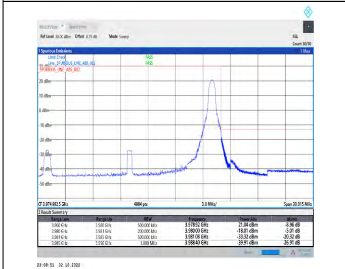
1-N77-3700-3980--30-20-H-5-CP-QPSK-Edge_1RB_Right-1@50-Ant1-1--PASS-see graph
