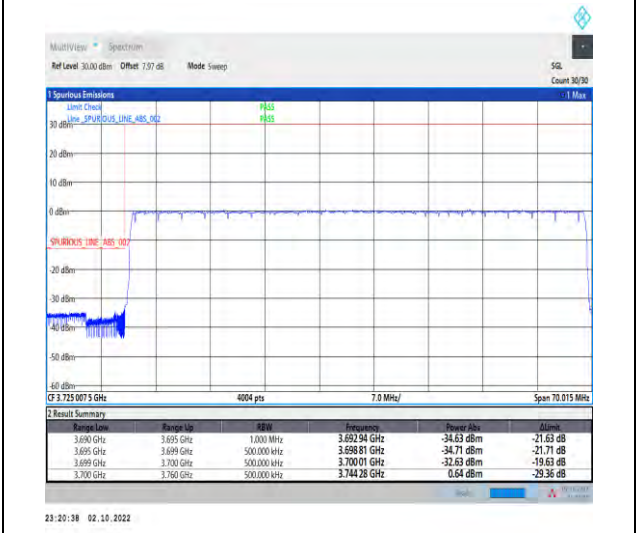
1-N77-3700-3980--30-60-L-6-CP-QPSK-Outer_Full-162@0-Ant1-1--PASS-see graph
