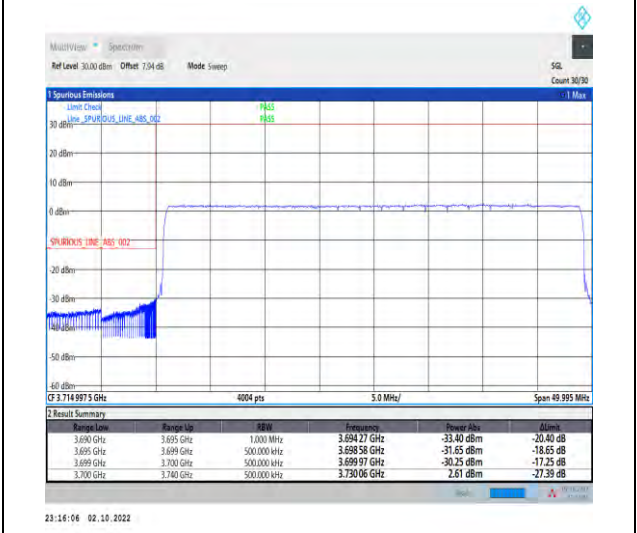
1-N77-3700-3980--30-40-L-6-CP-QPSK-Outer_Full-106@0-Ant1-1--PASS-see graph
