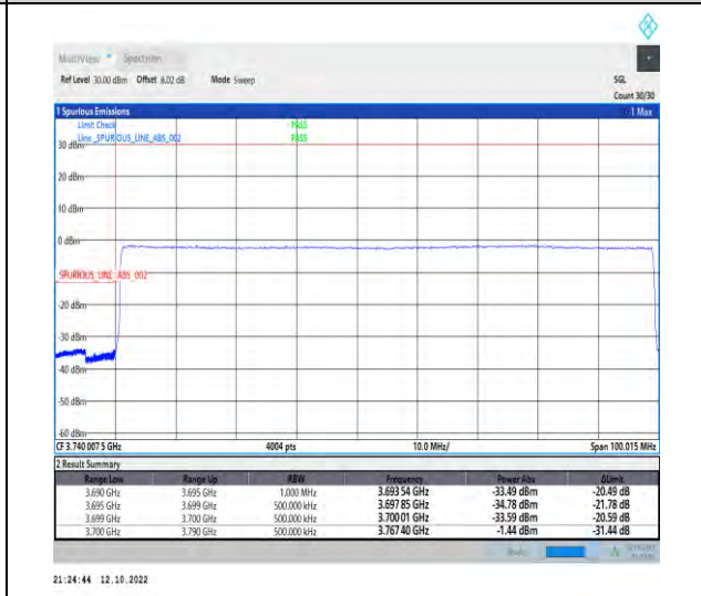
1-N77-3700-3980--30-90-L-6-CP-QPSK-Outer_Full-245@0-Ant1-1--PASS-see graph
