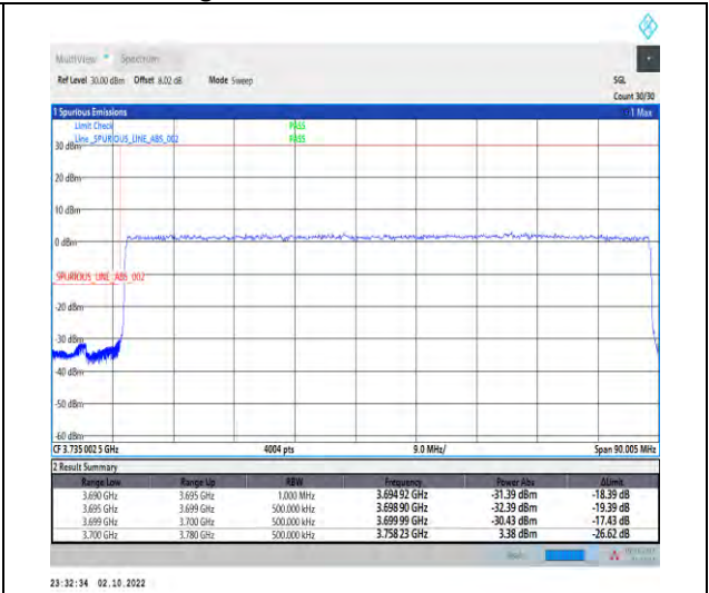
1-N77-3700-3980--30-80-L-3-DFT-PI2BPSK-Outer_Full-216@0-Ant1-1--PASS-see graph
