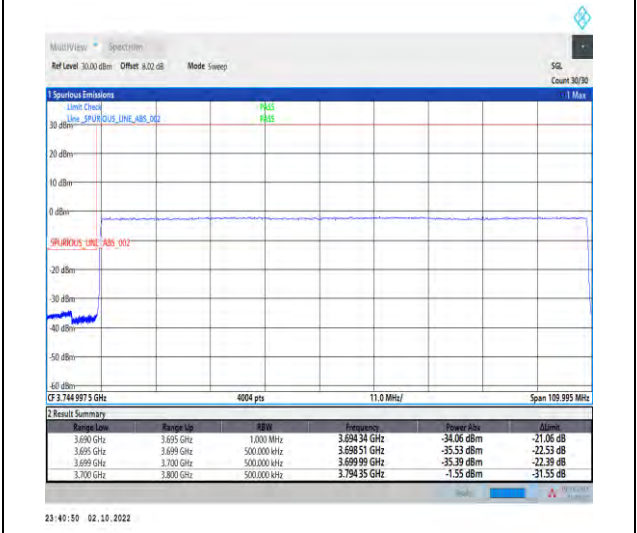
1-N77-3700-3980--30-100-L-6-CP-QPSK-Outer_Full-273@0-Ant1-1--PASS-see graph
