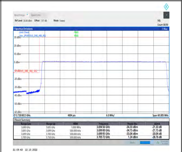
1-N77-3700-3980--30-50-L-6-CP-QPSK-Outer_Full-133@0-Ant1-1--PASS-see graph
