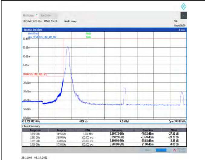
1-N77-3700-3980--30-30-L-4-CP-QPSK-Edge_1RB_Left-1@0-Ant1-1--PASS-see graph
