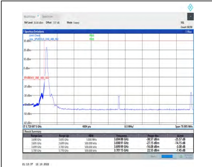
1-N77-3700-3980--30-70-L-1-DFT-PI2BPSK-Edge_1R_B_Left-1@0-Ant1-1--PASS-see graph
