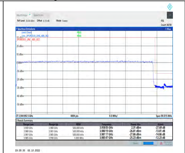
1-N77-3700-3980--30-80-H-3-DFT-PI2BPSK-Outer_Full-216@0-Ant1-1--PASS-see graph
