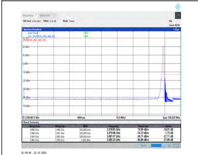
1-N77-3700-3980--30-90-H-5-CP-QPSK-Edge_1RB_Right-1@244-Ant1-1--PASS-see graph
