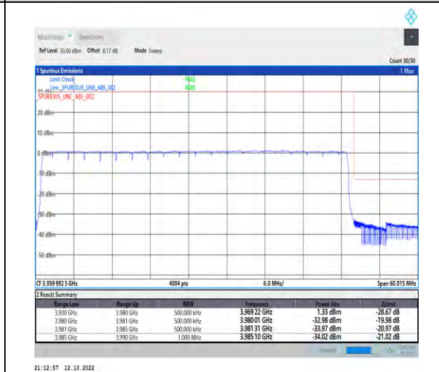
1-N77-3700-3980--30-50-H-6-CP-QPSK-Outer_Full-133@0-Ant1-1--PASS-see graph
