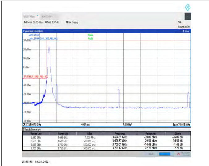
1-N77-3700-3980--30-60-L-1-DFT-PI2BPSK-Edge_1R_B_Left-1@0-Ant1-1--PASS-see graph
