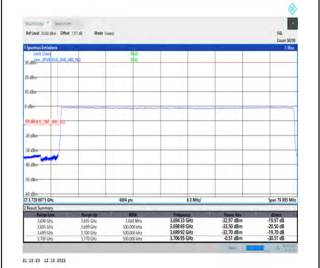
1-N77-3700-3980--30-70-L-6-CP-QPSK-Outer_Full-189@0-Ant1-1--PASS-see graph
