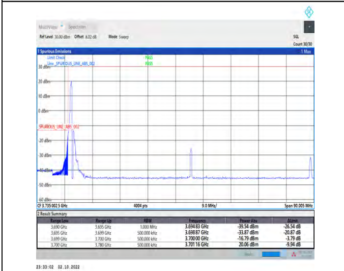
1-N77-3700-3980--30-80-L-4-CP-QPSK-Edge_1RB_Left-1@0-Ant1-1--PASS-see graph
