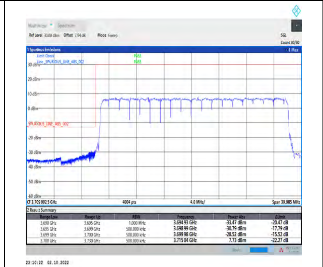
1-N77-3700-3980--30-30-L-3-DFT-PI2BPSK-Outer_Full-75@0-Ant1-1--PASS-see graph
