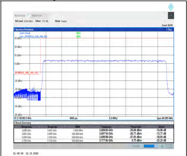
1-N77-3700-3980--30-50-L-3-DFT-PI2BPSK-Outer_Full-128@0-Ant1-1--PASS-see graph
