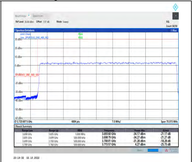
1-N77-3700-3980--30-60-L-3-DFT-PI2BPSK-Outer_Full-162@0-Ant1-1--PASS-see graph
