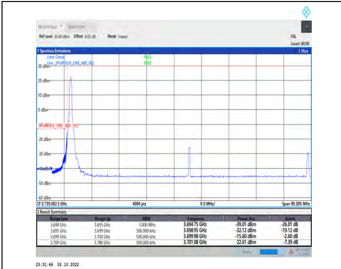
1-N77-3700-3980--30-80-L-1-DFT-PI2BPSK-Edge_1R_B_Left-1@0-Ant1-1--PASS-see graph
