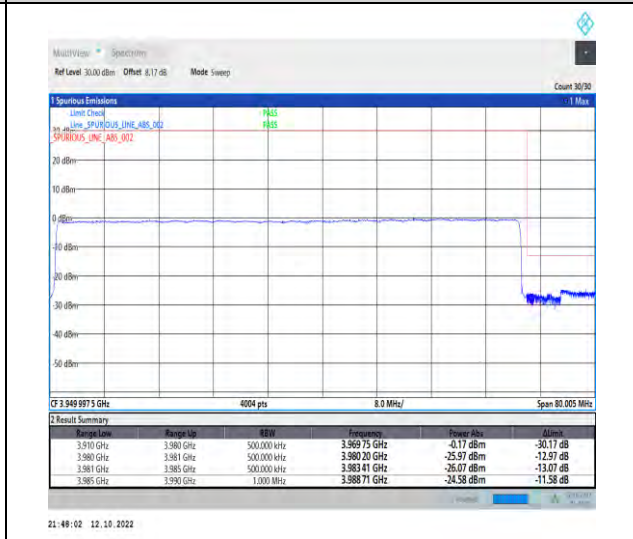
1-N77-3700-3980--30-70-H-6-CP-QPSK-Outer_Full-189@0-Ant1-1--PASS-see graph
