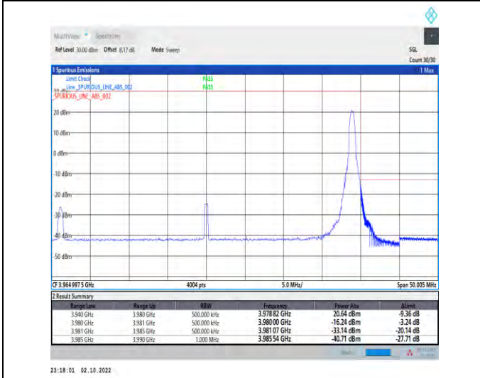
1-N77-3700-3980--30-40-H-5-CP-QPSK-Edge_1RB_Right-1@105-Ant1-1--PASS-see graph
