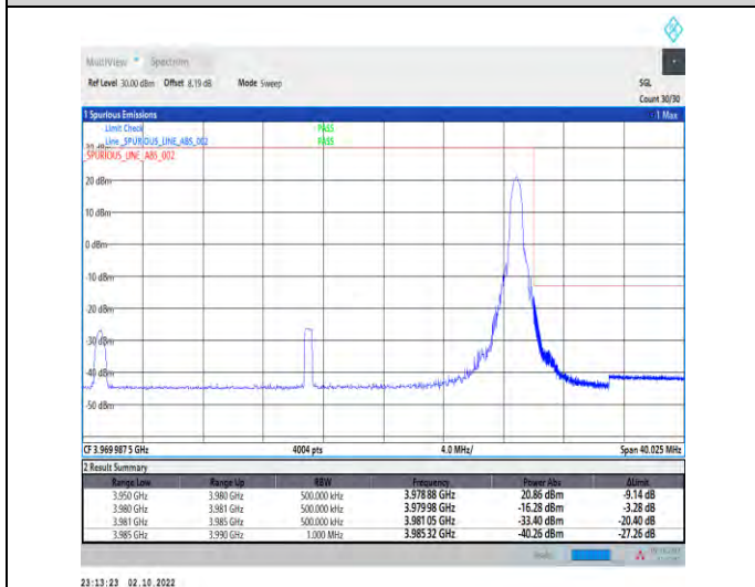
1-N77-3700-3980--30-30-H-5-CP-QPSK-Edge_1RB_Right-1@77-Ant1-1--PASS-see graph
