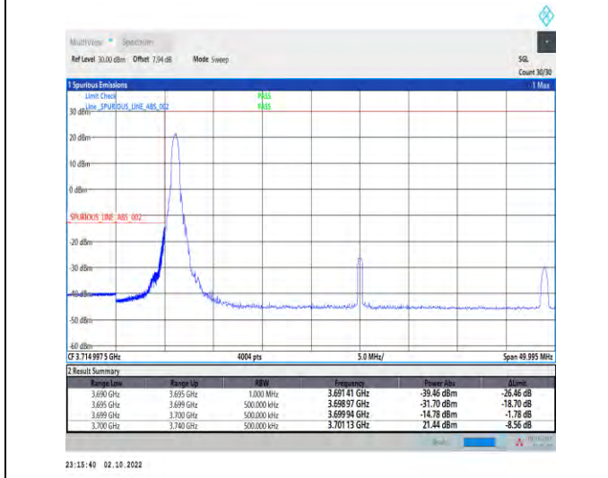
1-N77-3700-3980--30-40-L-4-CP-QPSK-Edge_1RB_Left-1@0-Ant1-1--PASS-see graph
