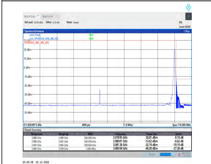
1-N77-3700-3980--30-100-H-5-CP-QPSK-Edge_1RB_Right-1@272-Ant1-1--PASS-see graph
