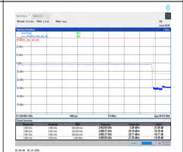
1-N77-3700-3980--30-80-H-6-CP-QPSK-Outer_Ful I-217@0-Ant1-1--PASS-see graph
