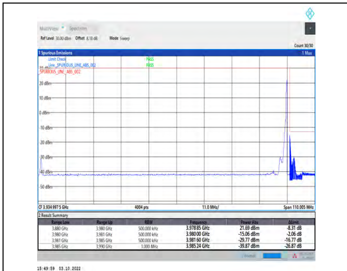
1-N77-3700-3980--30-100-H-2-DFT-PI2BPSK-Edge_1 RB_Right-1@272-Ant1-1--PASS-see graph
