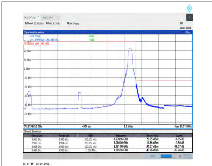
1-N77-3700-3980--30-20-H-2-DFT-PI2BPSK-Edge_1R_B_Right-1@50-Ant1-1--PASS-see graph
