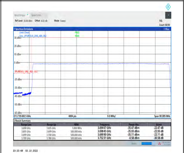
1-N77-3700-3980--30-80-L-6-CP-QPSK-Outer_Full-217@0-Ant1-1--PASS-see graph
