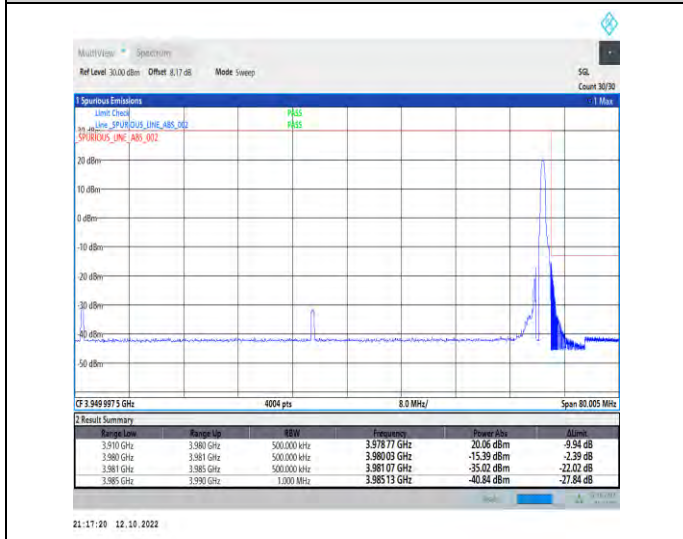
1-N77-3700-3980--30-70-H-5-CP-QPSK-Edge_1RB_Right-1@188-Ant1-1--PASS-see graph
