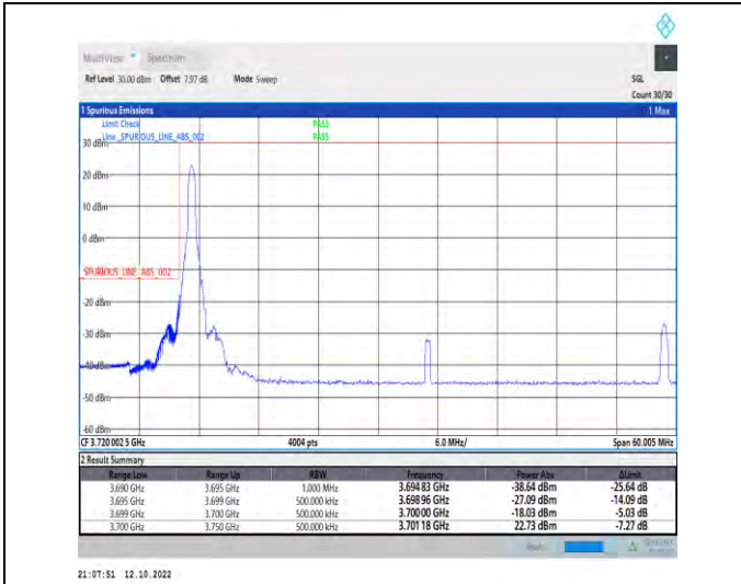
1-N77-3700-3980--30-50-L-1-DFT-PI2BPSK-Edge_1R_B_Left-1@0-Ant1-1--PASS-see graph
