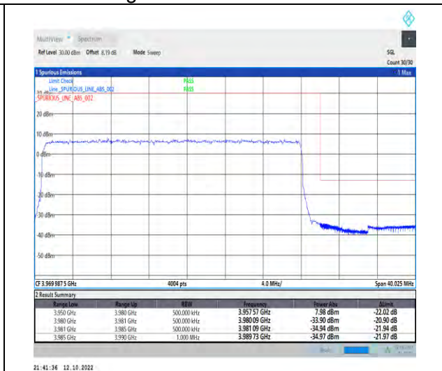
1-N77-3700-3980--30-30-H-3-DFT-PI2BPSK-Outer_Full-75@0-Ant1-1--PASS-see graph
