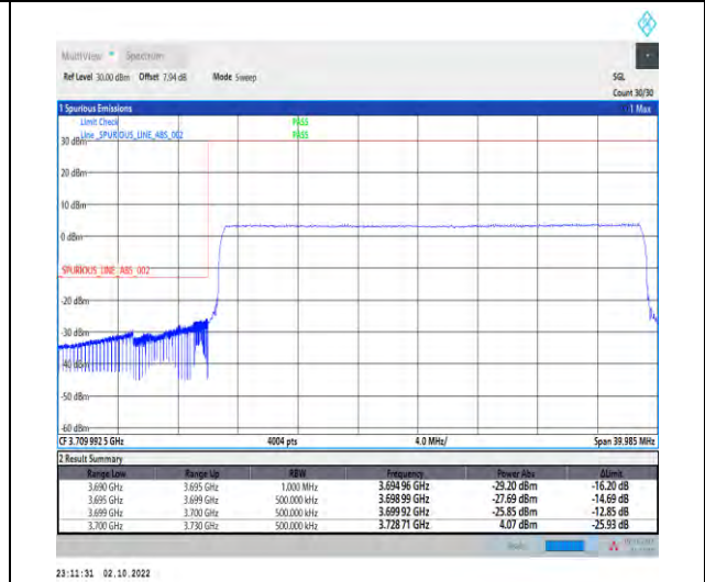
1-N77-3700-3980--30-30-L-6-CP-QPSK-Outer_Full-78@0-Ant1-1--PASS-see graph
