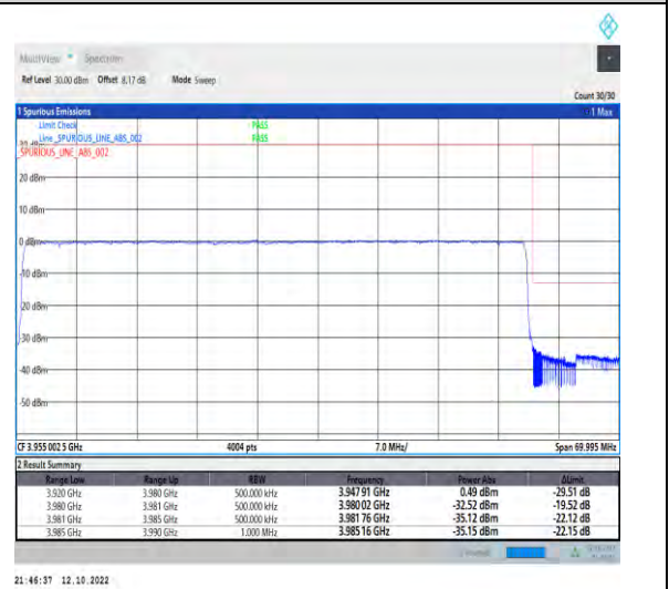
1-N77-3700-3980--30-60-H-6-CP-QPSK-Outer_Full-162@0-Ant1-1--PASS-see graph
