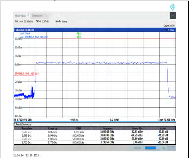
1-N77-3700-3980--30-70-L-3-DFT-PI2BPSK-Outer_Full-180@0-Ant1-1--PASS-see graph
