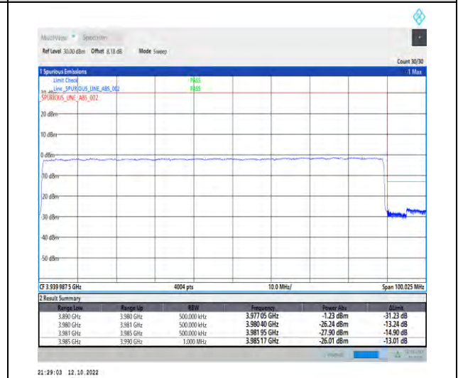
1-N77-3700-3980--30-90-H-6-CP-QPSK-Outer_Full-245@0-Ant1-1--PASS-see graph
