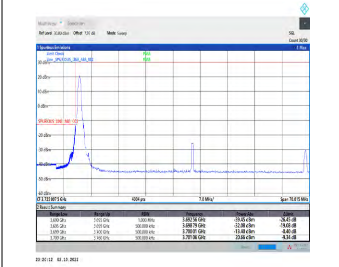
1-N77-3700-3980--30-60-L-4-CP-QPSK-Edge_1RB_Left-1@0-Ant1-1--PASS-see graph
