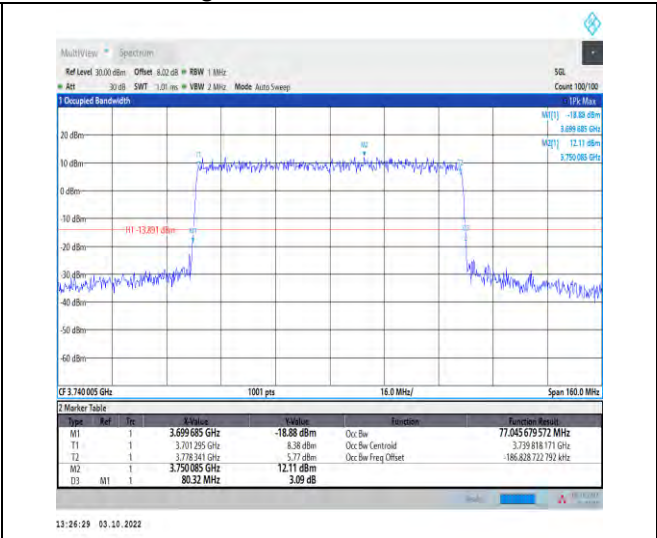
1-N77-3700-3980--30-80-L-4-DFT-64QAM-Outer_Fu II-216@0-Ant1-77.046-80.320-≤80-PASS
