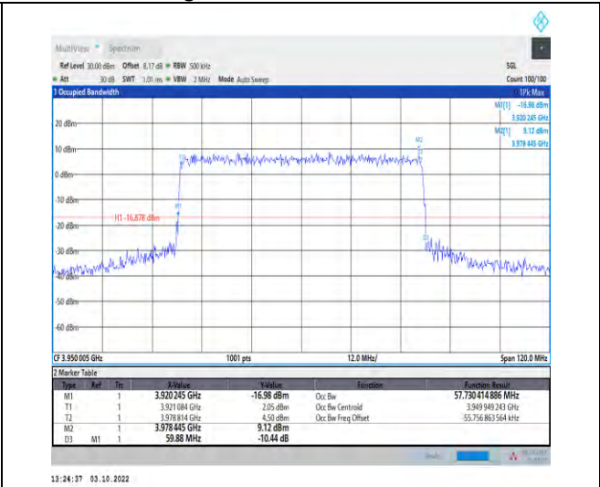
1-N77-3700-3980--30-60-H-8-CP-64QAM-Outer_Full -162@0-Ant1-57.73-59.880-≤60-PASS
