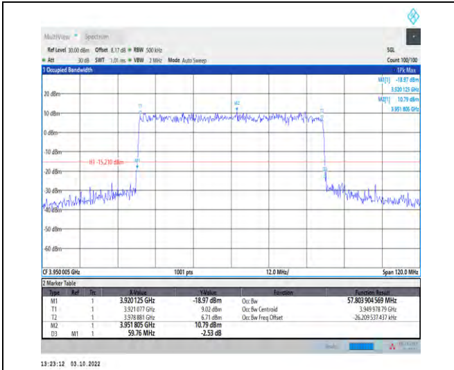
1-N77-3700-3980--30-60-H-3-DFT-16QAM-Outer_Fu ll-162@0-Ant1-57.804-59.760-≤60-PASS
