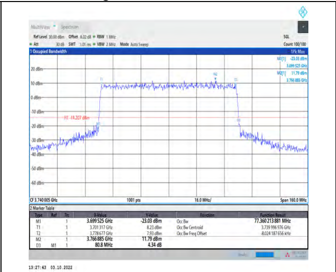
1-N77-3700-3980--30-80-L-8-CP-64QAM-Outer_Full-217@0-Ant1-77.36-80.800-<math>\leq 80</math>-PASS
