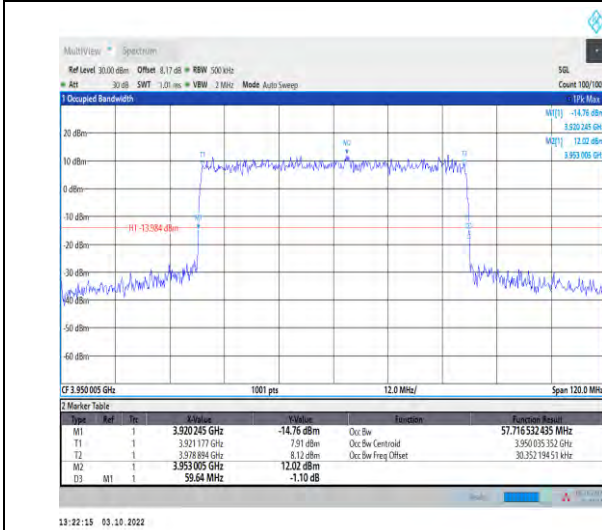
1-N77-3700-3980--30-60-H-1-DFT-QPSK-Outer_Full -162@0-Ant1-57.717-59.640-≤60-PASS
