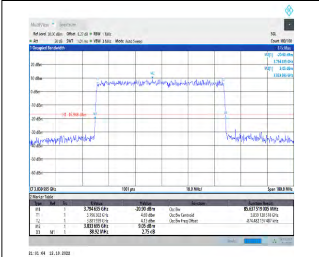
1-N77-3700-3980--30-90-M-5-DFT-256QAM-Outer_F ull-240@0-Ant1-85.638-88.920-<=90-PASS
