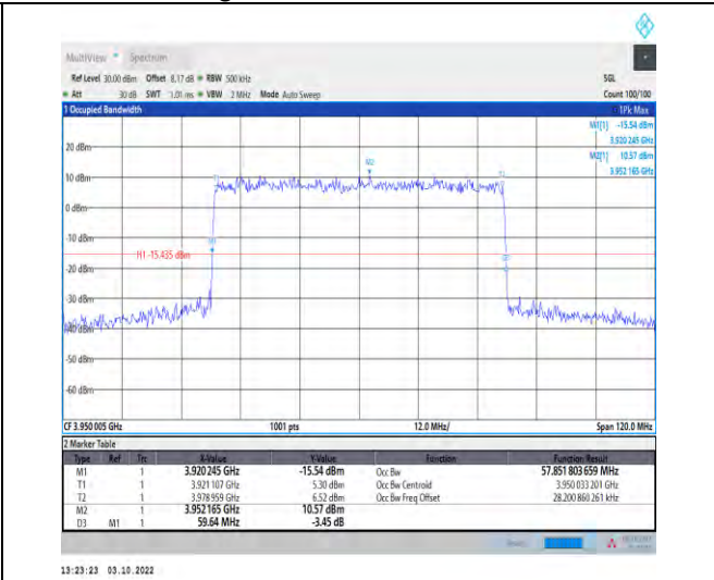
1-N77-3700-3980--30-60-H-4-DFT-64QAM-Outer_F ull-162@0-Ant1-57.852-59.640-≤60-PASS
