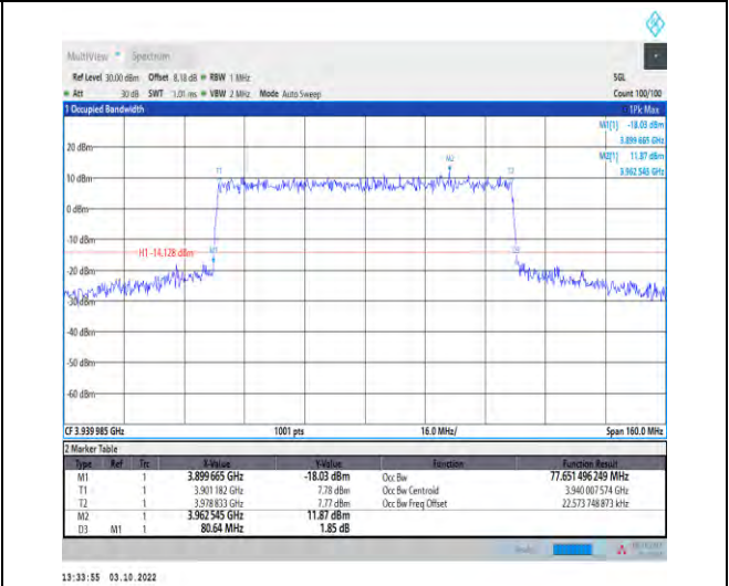
1-N77-3700-3980--30-80-H-8-CP-64QAM-Outer_Full-217@0-Ant1-77.651-80.640-≤80-PASS
