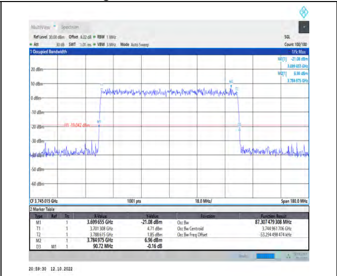
1-N77-3700-3980--30-90-L-9-CP-256QAM-Outer_Fu-II-245@0-Ant1-87.307-90.720-<math>\leq</math>90-PASS
