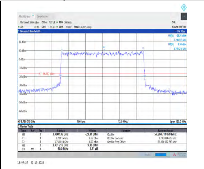
1-N77-3700-3980--30-60-L-6-CP-QPSK-Outer_Full-162@0-Ant1-57.869-60.000-≤60-PASS
