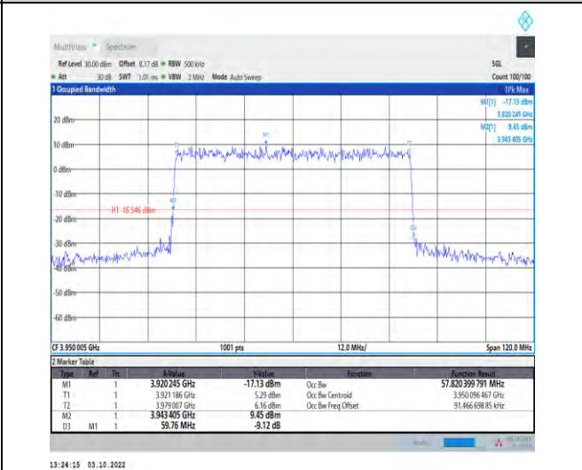
1-N77-3700-3980--30-60-H-6-CP-QPSK-Outer_Full- 162@0-Ant1-57.82-59.760-≤60-PASS
