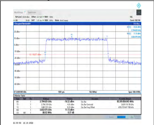
1-N77-3700-3980--30-90-M-4-DFT-64QAM-Outer_F ull-240@0-Ant1-85.596-88.920-<=90-PASS
