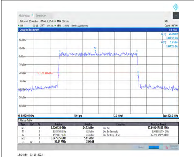
1-N77-3700-3980--30-60-H-9-CP-256QAM-Outer_Fu II-162@0-Ant1-57.649-59.640-≤60-PASS
