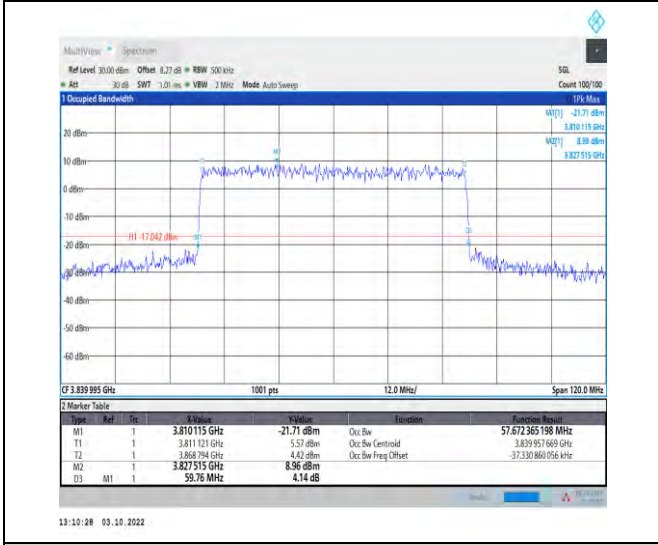
1-N77-3700-3980--30-60-M-6-CP-QPSK-Outer_Full-162@0-Ant1-57.672-59.760-<math>\leq 60</math>-PASS
