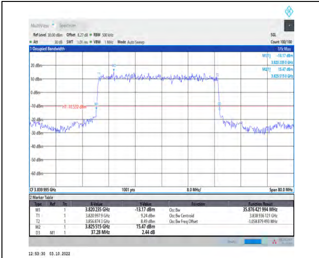
1-N77-3700-3980--30-40-M-2-DFT-PI2BPSK-Outer_Full-100@0-Ant1-35.876-37.280-≤40-PASS
