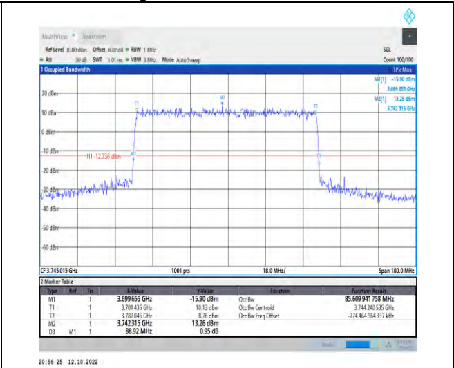
1-N77-3700-3980--30-90-L-1-DFT-QPSK-Outer_Full -240@0-Ant1-85.61-88.920-<math>\leq 90</math>-PASS
