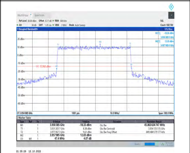
1-N77-3700-3980--30-50-H-1-DFT-QPSK-Outer_Full -128@0-Ant1-45.864-47.400-≤50-PASS
