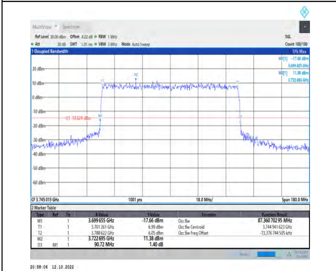
1-N77-3700-3980--30-90-L-6-CP-QPSK-Outer_Full-245@0-Ant1-87.361-90.720-≤90-PASS
