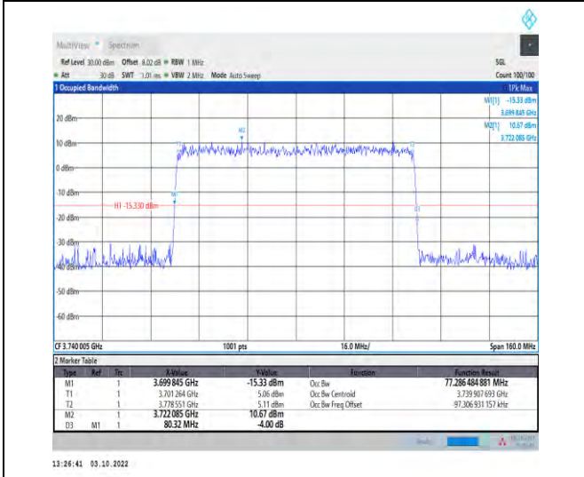
1-N77-3700-3980--30-80-L-5-DFT-256QAM-Outer_Full-216@0-Ant1-77.286-80.320-≤80-PASS
