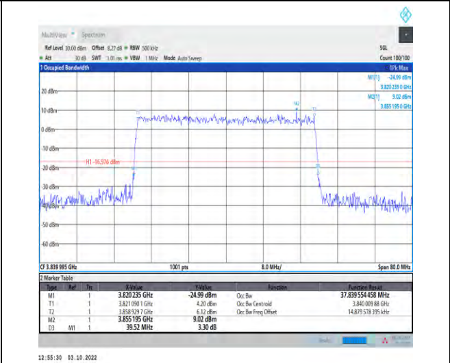
1-N77-3700-3980--30-40-M-9-CP-256QAM-Outer_Full-106@0-Ant1-37.84-39.520-≤40-PASS
