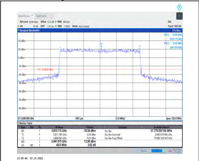
1-N77-3700-3980--30-60-M-1-DFT-QPSK-Outer_Full -162@0-Ant1-57.779-60.000-≤60-PASS
