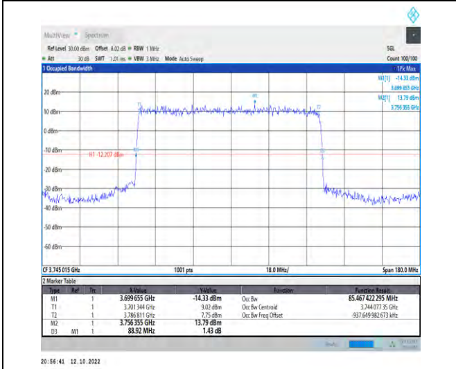
1-N77-3700-3980--30-90-L-2-DFT-PI2BPSK-Outer_Full -240@0-Ant1-85.467-88.920-<math>\leq 90</math>-PASS
