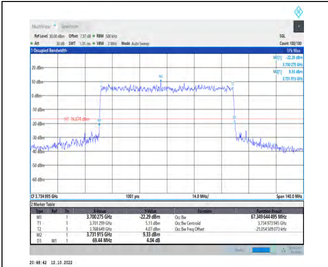
1-N77-3700-3980--30-70-L-6-CP-QPSK-Outer_Full-189@0-Ant1-67.35-69.440-<math>\leq 70</math>-PASS
