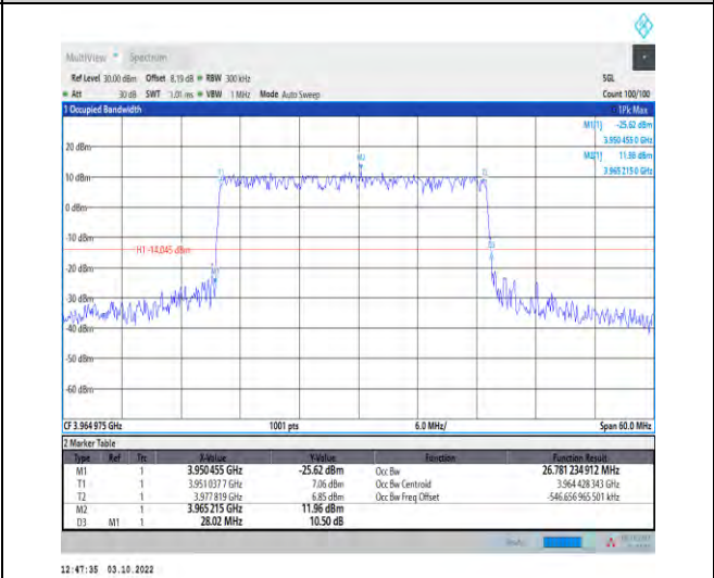
1-N77-3700-3980--30-30-H-3-DFT-16QAM-Outer_Full-75@0-Ant1-26.781-28.020-<=30-PASS
