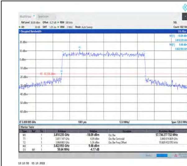
1-N77-3700-3980--30-60-M-8-CP-64QAM-Outer_Full -162@0-Ant1-57.736-59.640-≤60-PASS
