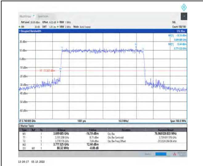
1-N77-3700-3980--30-80-L-3-DFT-16QAM-Outer_Ful I-216@0-Ant1-76.969-80.320-≤80-PASS
