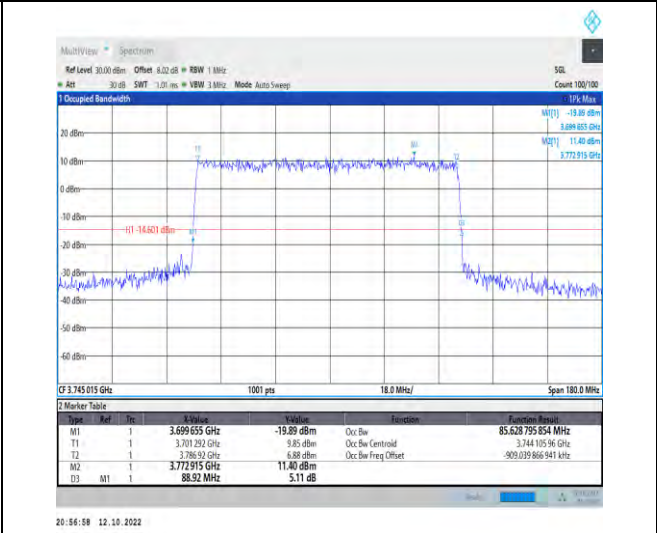
1-N77-3700-3980--30-90-L-3-DFT-16QAM-Outer_Full -240@0-Ant1-85.629-88.920-<math>\leq 90</math>-PASS
