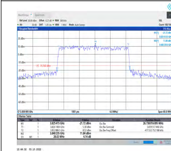
1-N77-3700-3980--30-30-M-3-DFT-16QAM-Outer_Full II-75@0-Ant1-26.738-28.020-≤30-PASS
