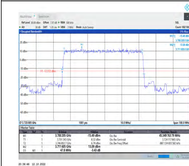
1-N77-3700-3980--30-50-L-2-DFT-PI2BPSK-Outer_Full-128@0-Ant1-45.55-47.800-≤50-PASS
