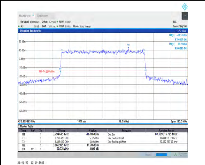
1-N77-3700-3980--30-90-M-6-CP-QPSK-Outer_Full-245@0-Ant1-87.189-90.720-<=90-PASS
