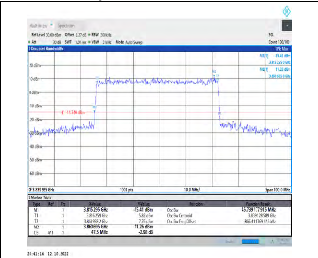
1-N77-3700-3980--30-50-M-4-DFT-64QAM-Outer_F ull-128@0-Ant1-45.739-47.500-≤50-PASS
