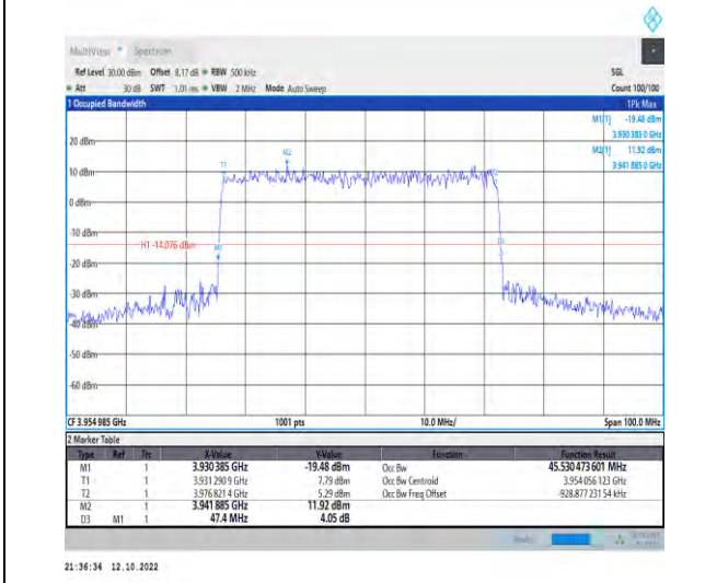
1-N77-3700-3980--30-50-H-4-DFT-64QAM-Outer_Full-128@0-Ant1-45.53-47.400-≤50-PASS
