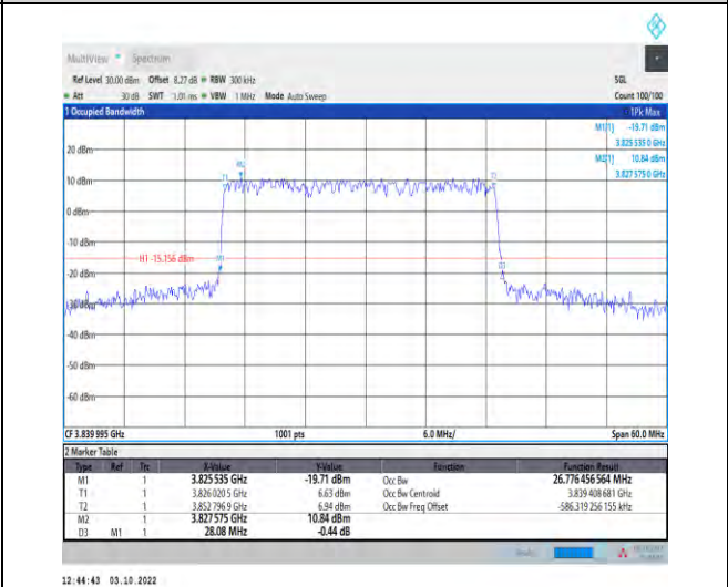
1-N77-3700-3980--30-30-M-4-DFT-64QAM-Outer_Full ull-75@0-Ant1-26.776-28.080-≤30-PASS
