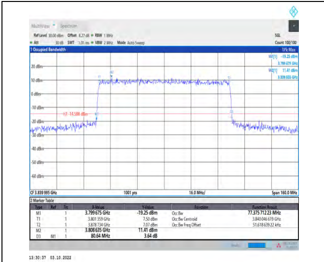
1-N77-3700-3980--30-80-M-6-CP-QPSK-Outer_Full-217@0-Ant1-77.376-80.640-<math>\leq 80</math>-PASS
