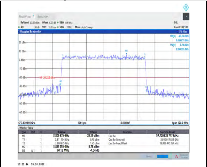
1-N77-3700-3980--30-60-M-9-CP-256QAM-Outer_Full-162@0-Ant1-57.721-60.120-≤60-PASS
