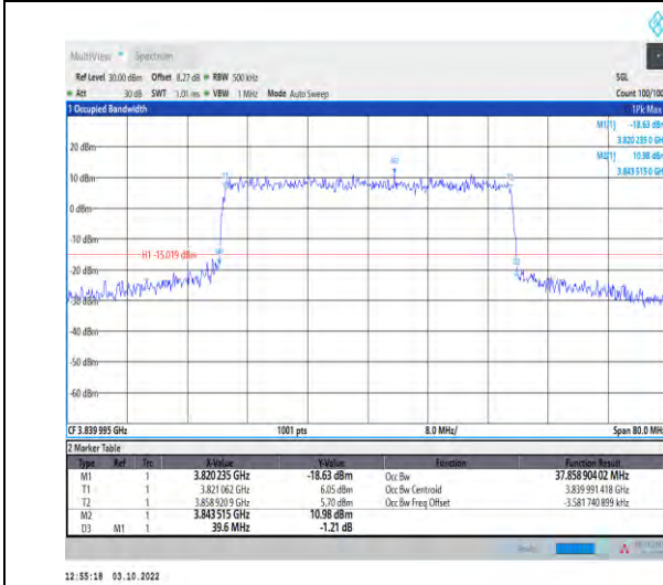
1-N77-3700-3980--30-40-M-8-CP-64QAM-Outer_Full-106@0-Ant1-37.859-39.600-≤40-PASS
