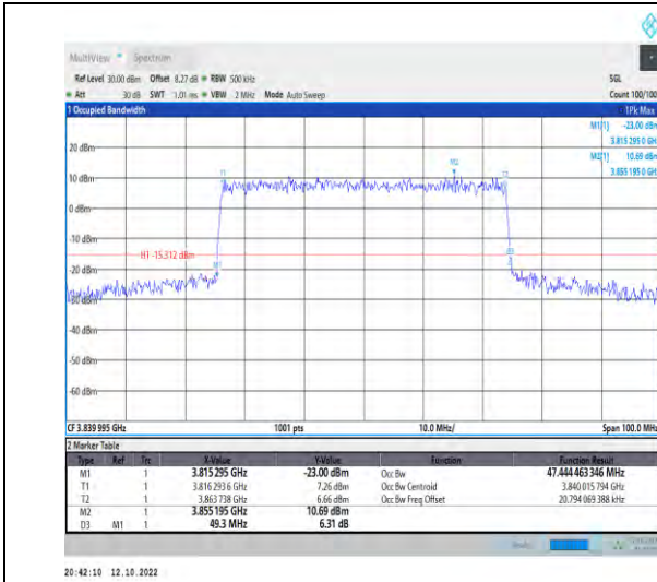
1-N77-3700-3980--30-50-M-7-CP-16QAM-Outer_Full -133@0-Ant1-47.444-49.300-≤50-PASS
