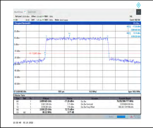
1-N77-3700-3980--30-80-H-4-DFT-64QAM-Outer_Full -216@0-Ant1-76.953-80.320-≤80-PASS
