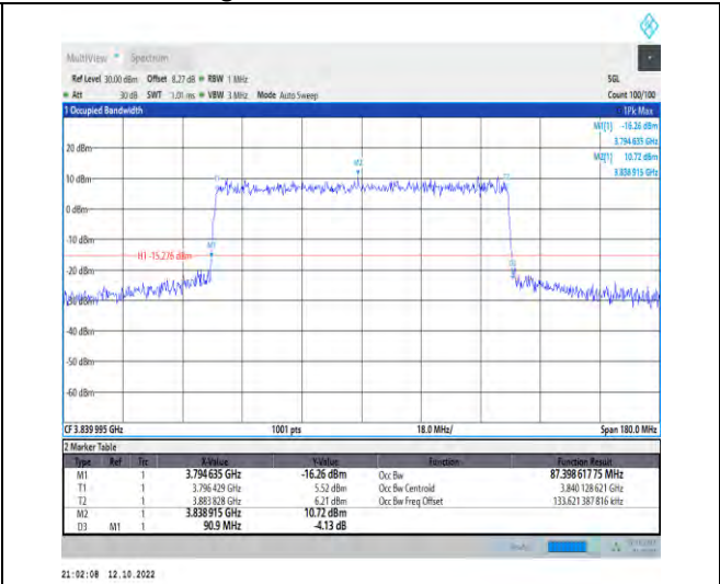
1-N77-3700-3980--30-90-M-8-CP-64QAM-Outer_Ful I-245@0-Ant1-87.399-90.900-≤90-PASS
