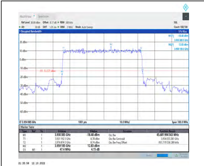
1-N77-3700-3980--30-50-H-2-DFT-PI2BPSK-Outer_Full-128@0-Ant1-45.682-47.400-≤50-PASS
