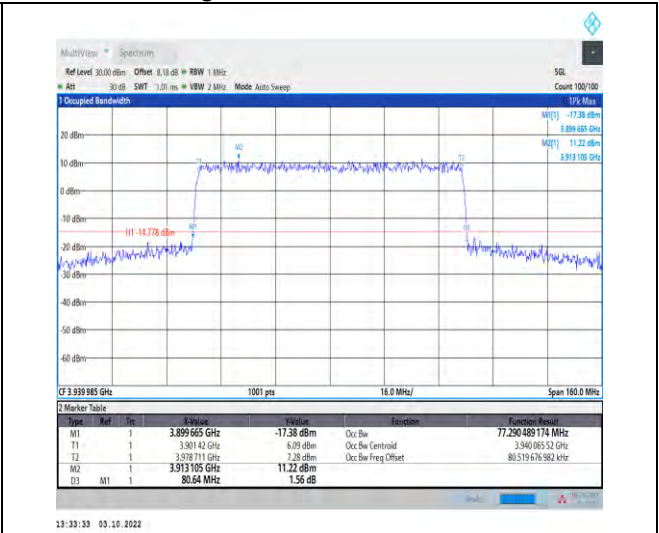
1-N77-3700-3980--30-80-H-6-CP-QPSK-Outer_Full-217@0-Ant1-77.29-80.640-≤80-PASS
