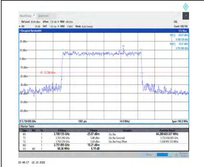
1-N77-3700-3980--30-70-L-4-DFT-64QAM-Outer_Full-180@0-Ant1-64.281-66.360-≤70-PASS
