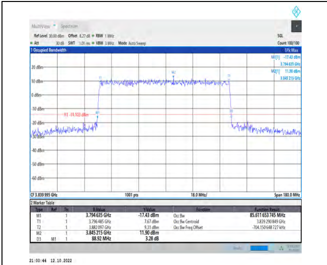
1-N77-3700-3980--30-90-M-3-DFT-16QAM-Outer_Fu ll-240@0-Ant1-85.612-88.920-<=90-PASS
