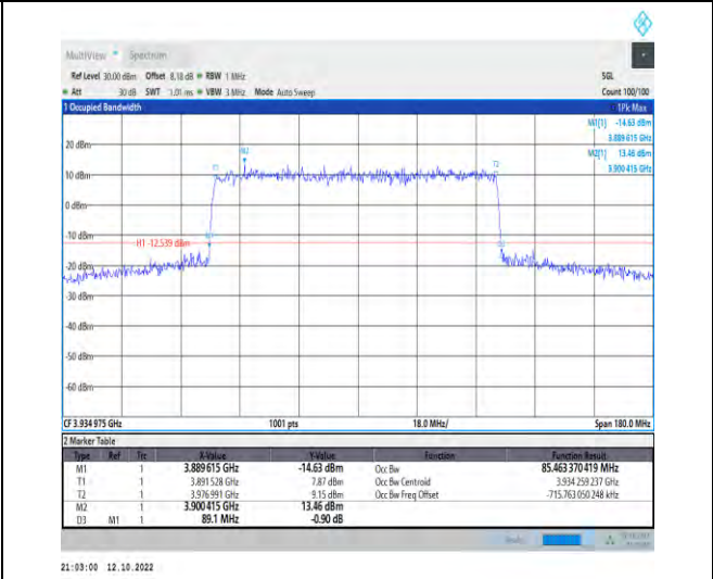
1-N77-3700-3980--30-90-H-1-DFT-QPSK-Outer_Full -240@0-Ant1-85.463-89.100-≤90-PASS
