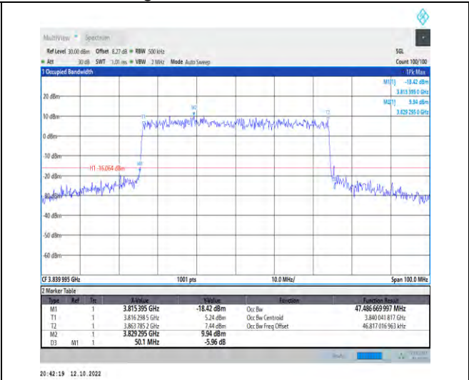
1-N77-3700-3980--30-50-M-8-CP-64QAM-Outer_Ful I-133@0-Ant1-47.487-50.100-≤50-PASS
