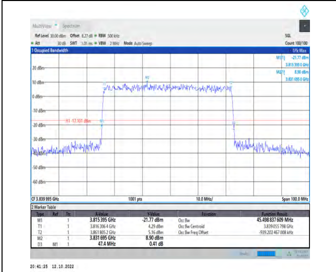
1-N77-3700-3980--30-50-M-5-DFT-256QAM-Outer_F ull-128@0-Ant1-45.499-47.400-≤50-PASS
