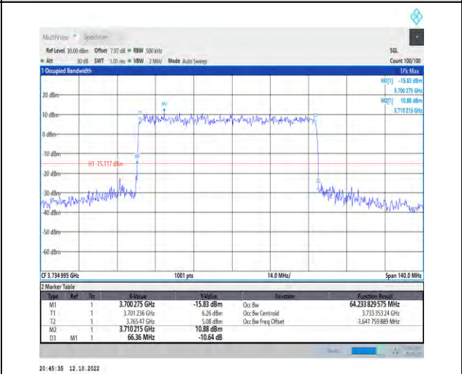
1-N77-3700-3980--30-70-L-1-DFT-QPSK-Outer_Full -180@0-Ant1-64.234-66.360-≤70-PASS
