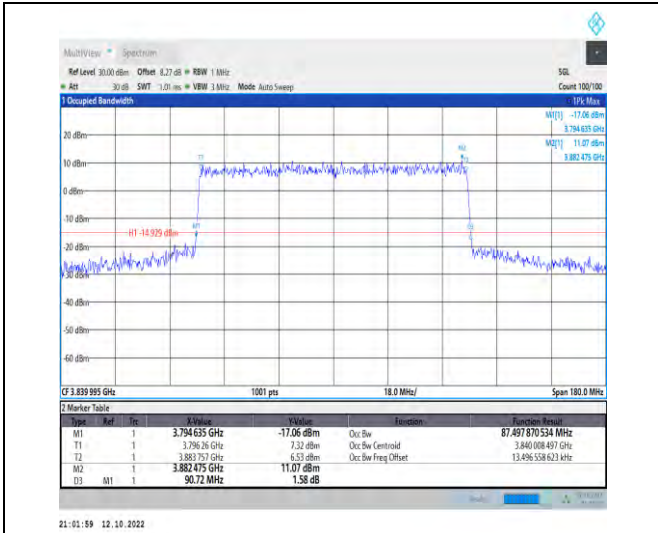
1-N77-3700-3980--30-90-M-7-CP-16QAM-Outer_Full -245@0-Ant1-87.498-90.720-≤90-PASS
