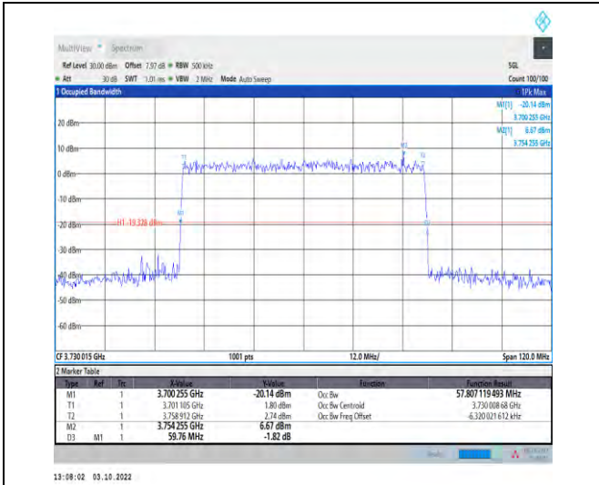
1-N77-3700-3980--30-60-L-9-CP-256QAM-Outer_Ful I-162@0-Ant1-57.807-59.760-≤60-PASS
