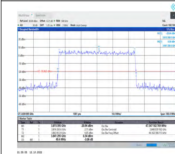
1-N77-3700-3980--30-50-M-9-CP-256QAM-Outer_F ull-133@0-Ant1-47.547-49.400-≤50-PASS
