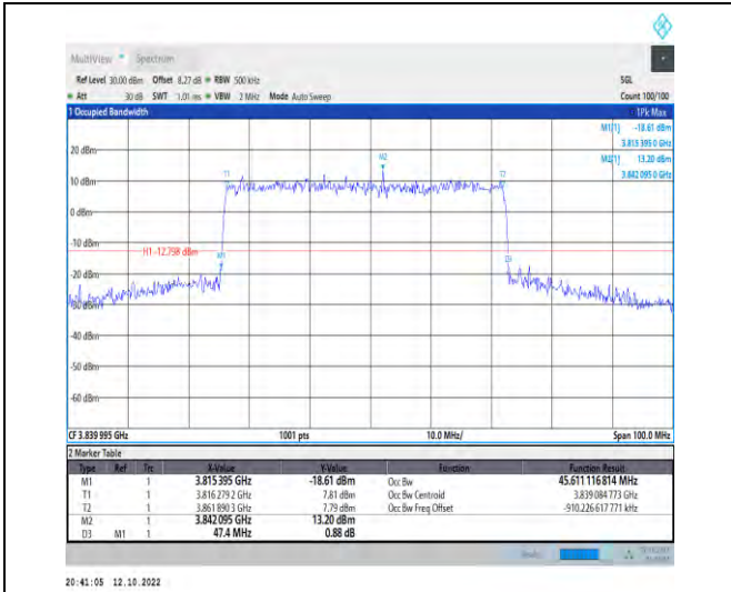
1-N77-3700-3980--30-50-M-3-DFT-16QAM-Outer_Fu ll-128@0-Ant1-45.611-47.400-≤50-PASS
