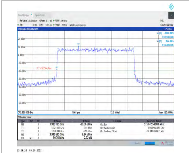
1-N77-3700-3980--30-60-H-7-CP-16QAM-Outer_Full -162@0-Ant1-57.762-59.760-≤60-PASS
